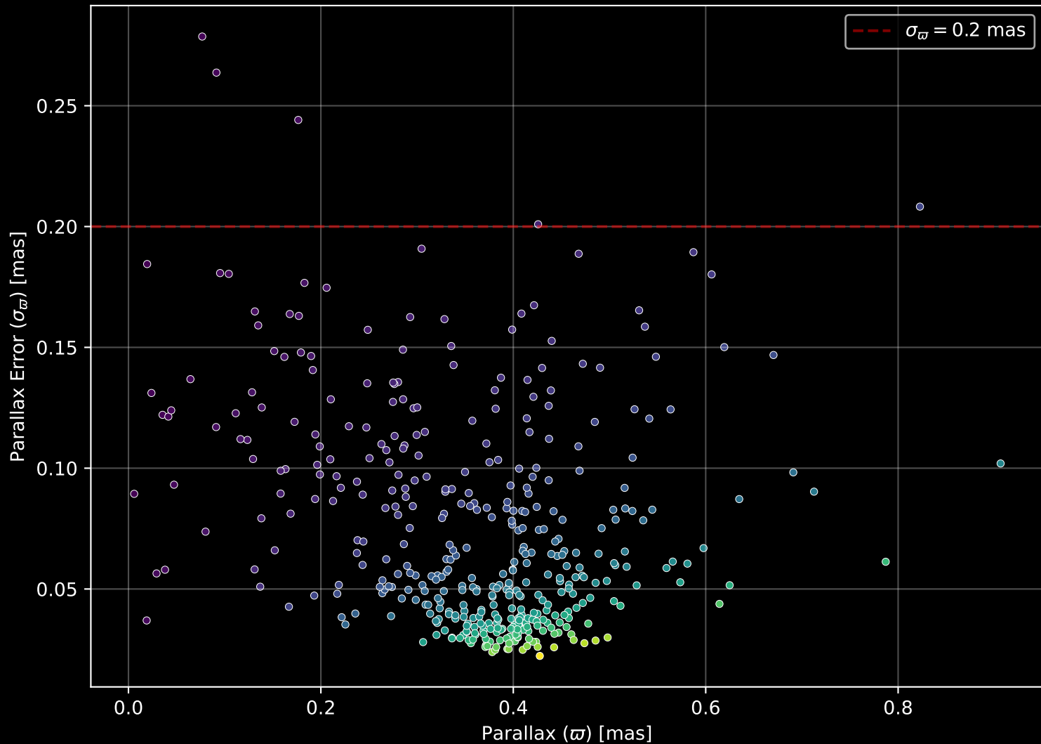
Gaia Cluster: [Ruprecht_134] Parallax Quality (n= 413)
