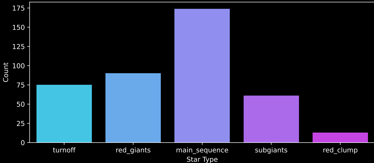
Gaia Cluster: [Ruprecht_134] Count plot of Star Type
