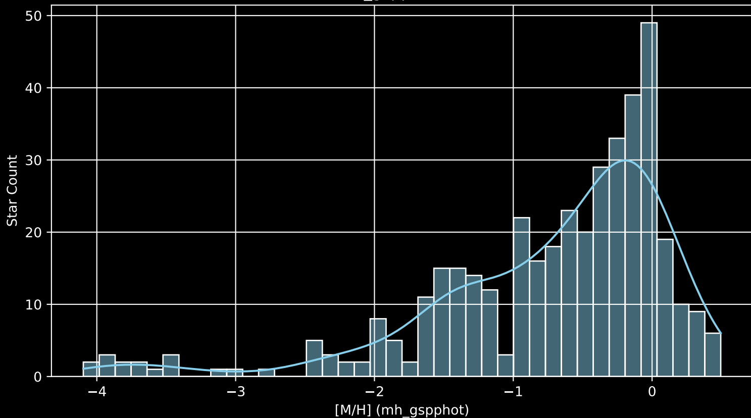
Gaia Cluster: [Ruprecht_134 [M/H] (mh_gspphot) (n= 406)
