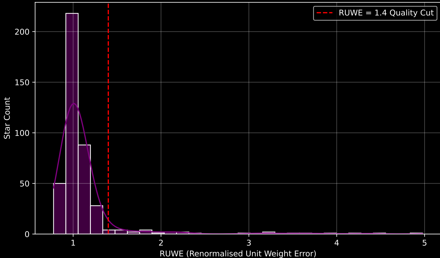
Gaia Cluster: [Ruprecht_134] RUWE Distribution (n= 413)
