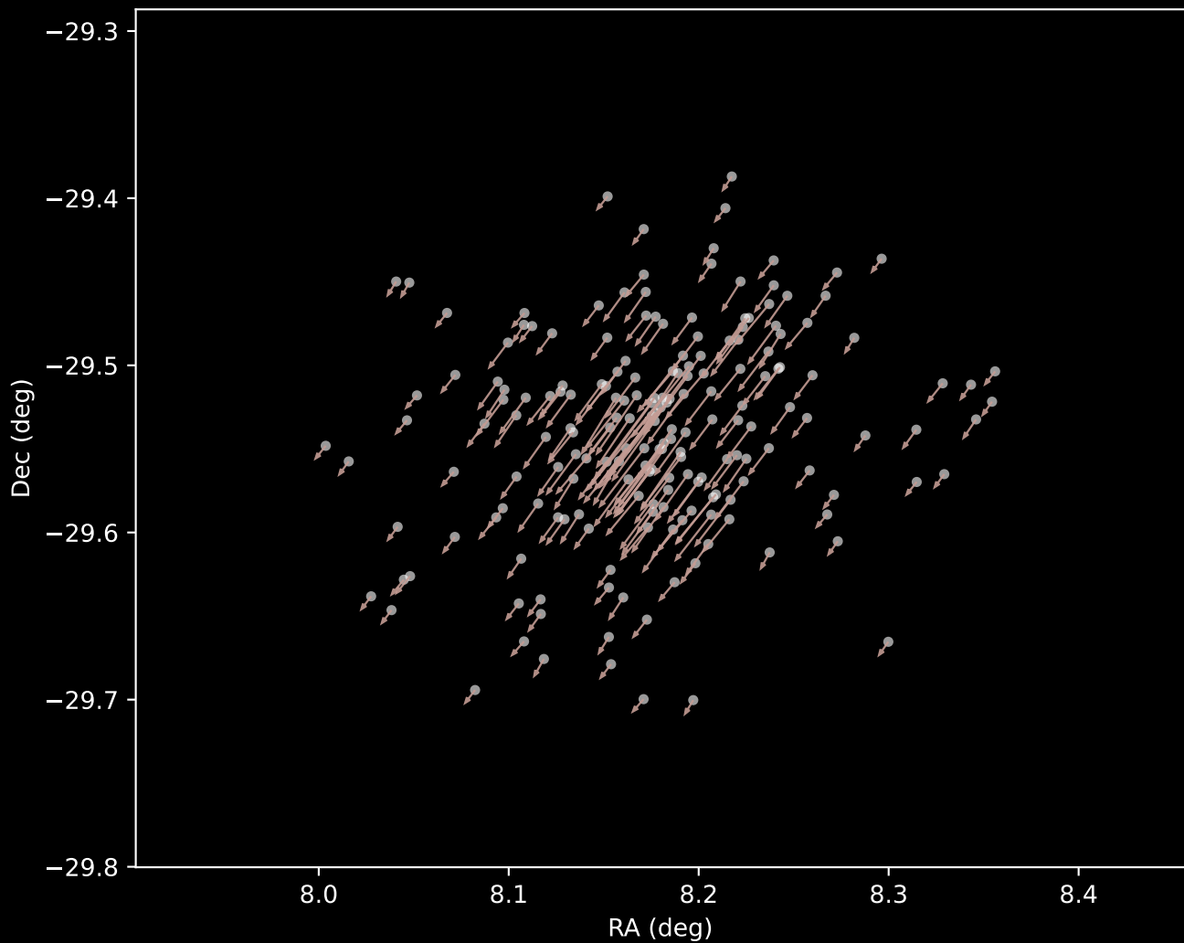
Gaia DR3 Cluster 11 Proper Motion Vectors (n=191)
