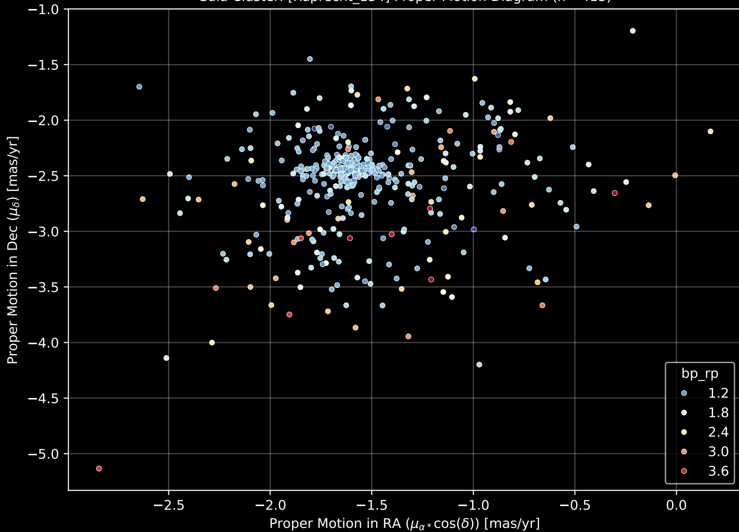
Gaia Cluster: [Ruprecht_134] Proper Motion Diagram (n= 413)
