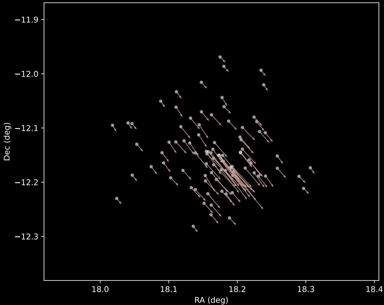
Gaia DR3 Cluster 11 Proper Motion Vectors (n=91)
