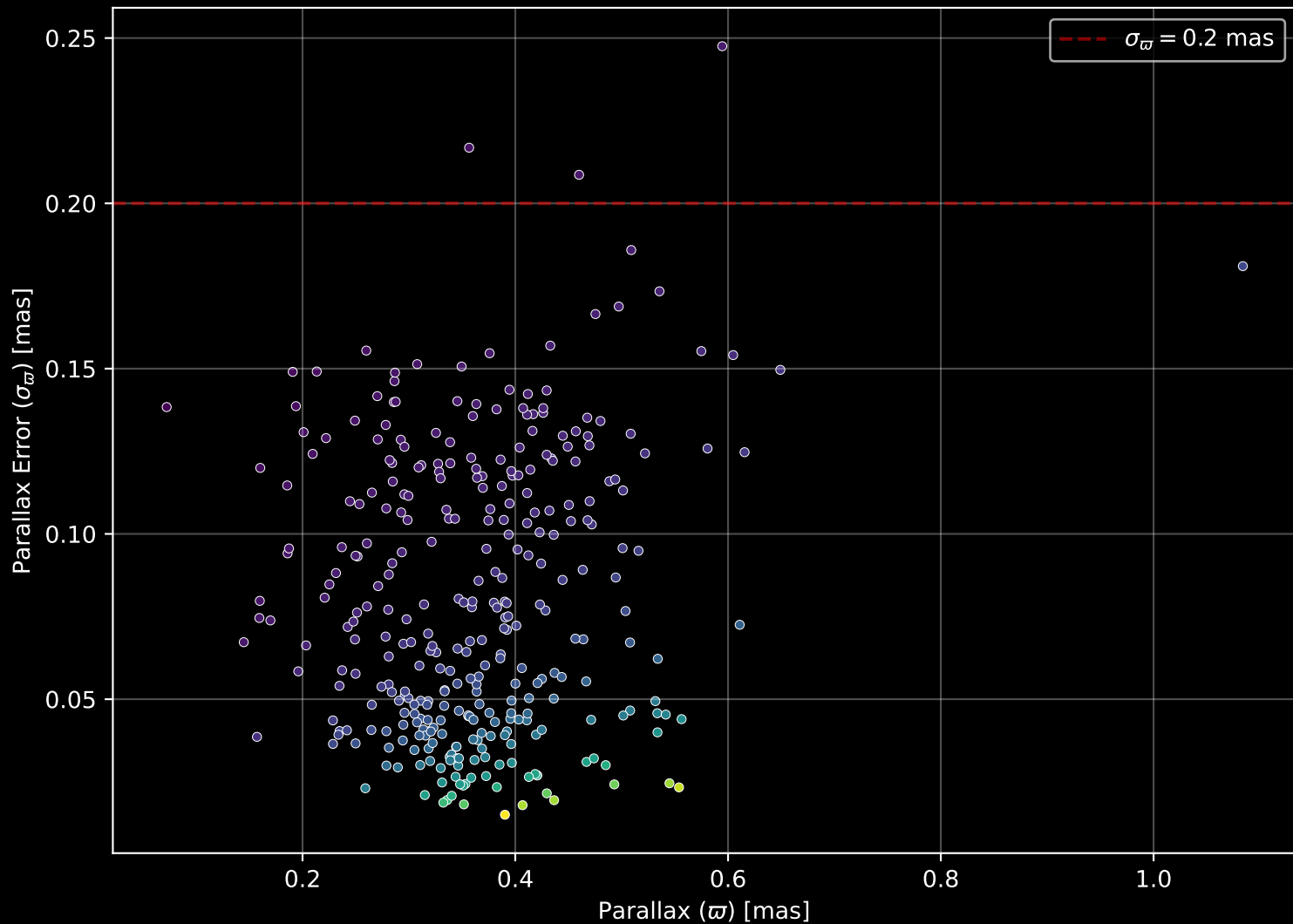
Gaia Cluster: [Ruprecht_143] Parallax Quality (n= 332)
