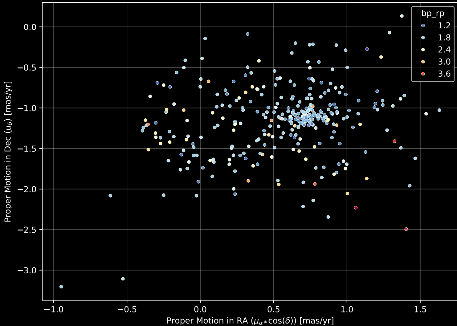
Gaia Cluster: [Ruprecht_143] Proper Motion Diagram (n= 332)
