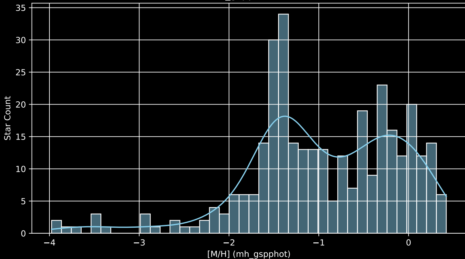
Gaia Cluster: [Ruprecht_143 [M/H] (mh_gspphot) (n= 329)
