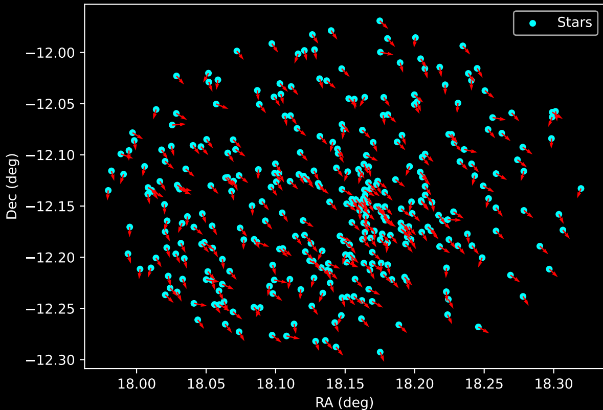
Gaia Cluster: [Ruprecht_143] Proper Motion Vectors for Gaia Star Field (n= 332)
