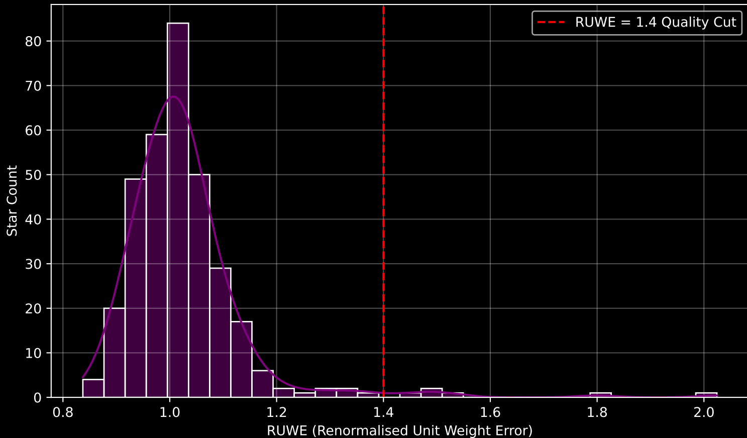
Gaia Cluster: [Ruprecht_143] RUWE Distribution (n= 332)
