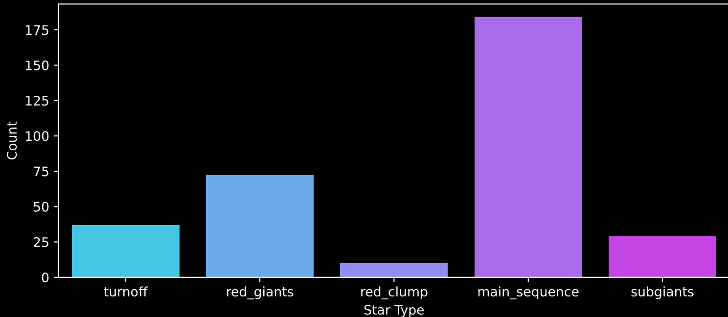
Gaia Cluster: [Ruprecht_143] Count plot of Star Type
