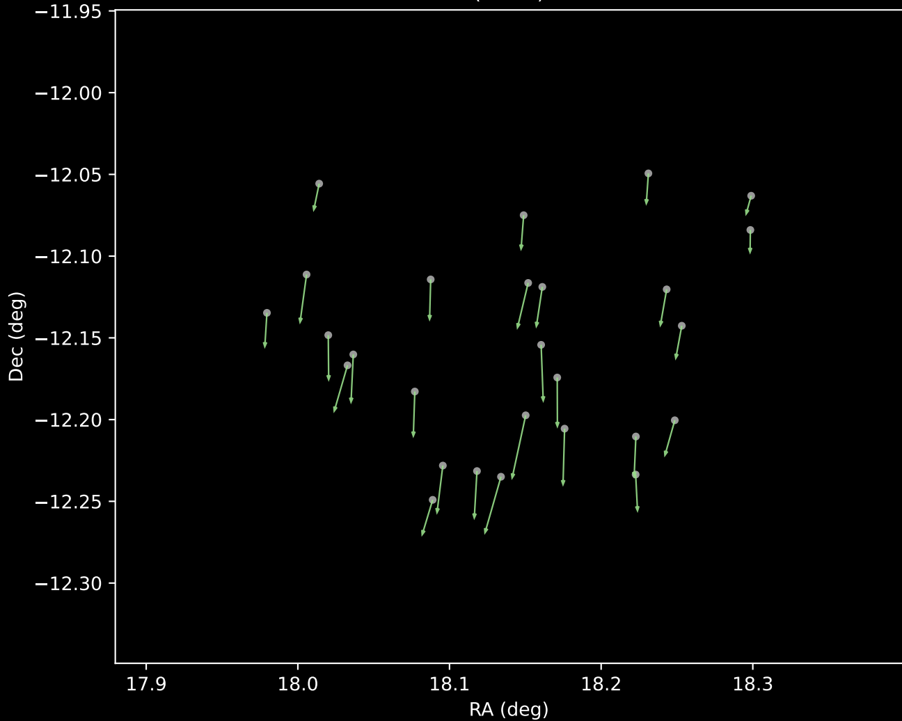
Gaia DR3 Cluster 5 Proper Motion Vectors (n=27)
