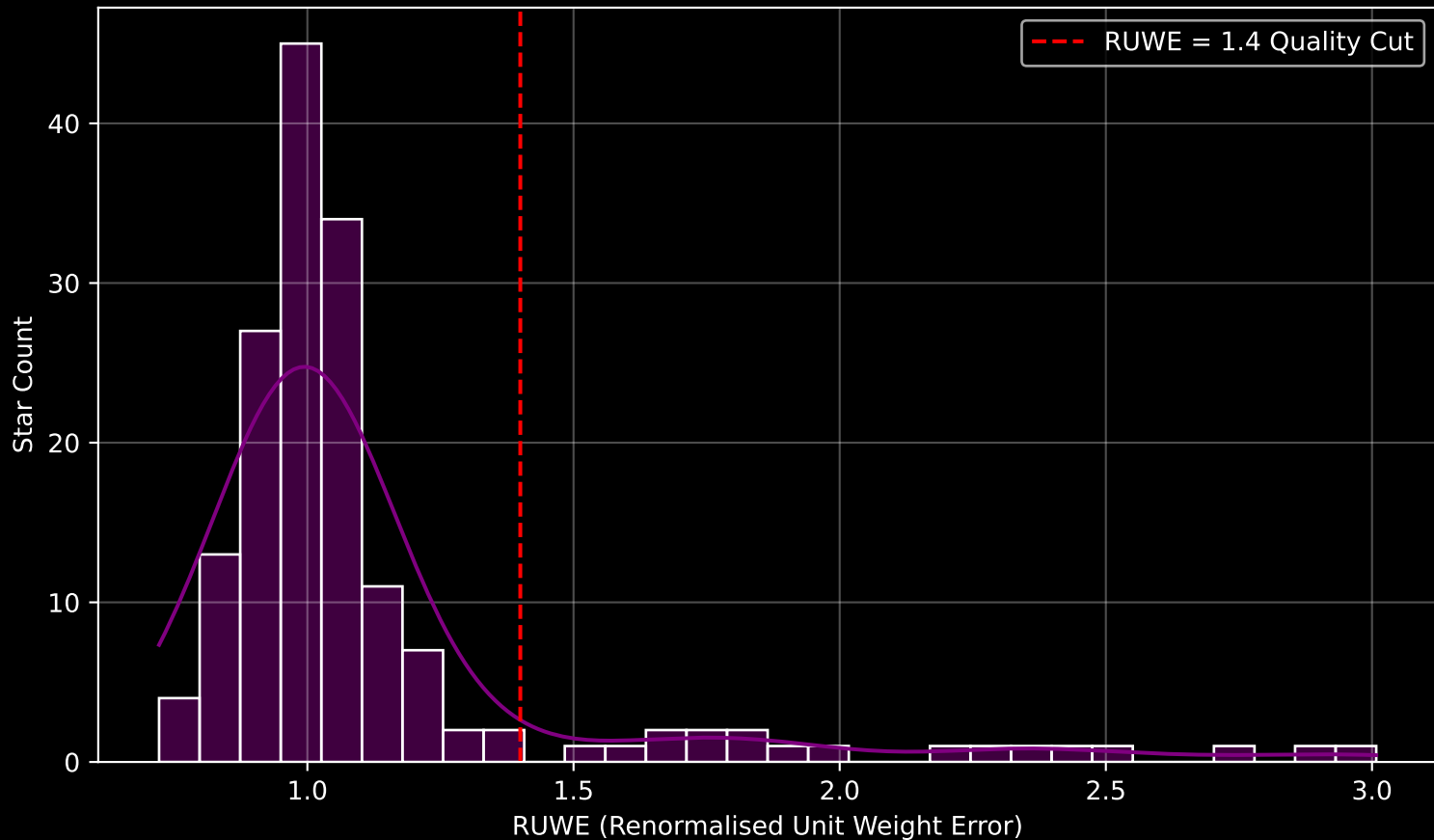
Gaia Cluster: [Ruprecht_147] RUWE Distribution (n= 163)
