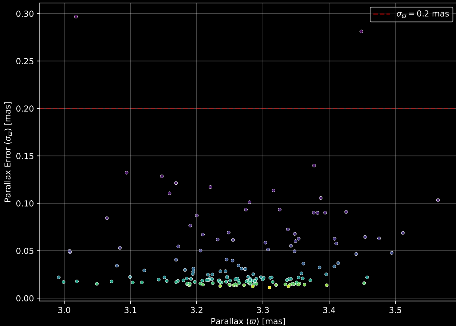
Gaia Cluster: [Ruprecht_147] Parallax Quality (n= 166)
