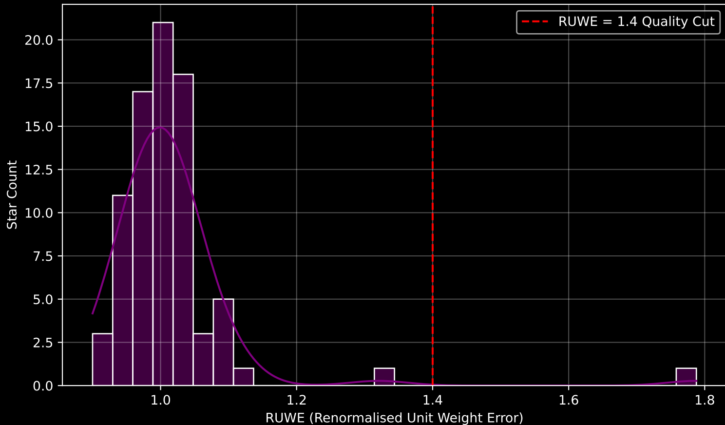
Gaia Cluster: [Ruprecht_148] RUWE Distribution (n= 81)
