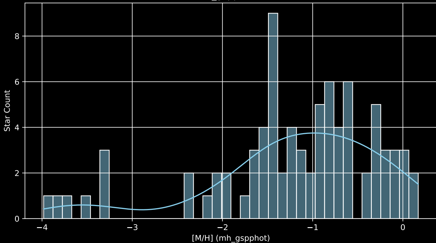
Gaia Cluster: [Ruprecht_148 [M/H] (mh_gspphot) (n= 81)
