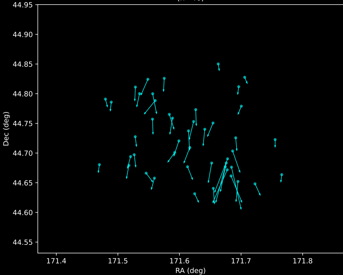
Gaia DR3 Noise Stream Proper Motion Vectors (n=46)
