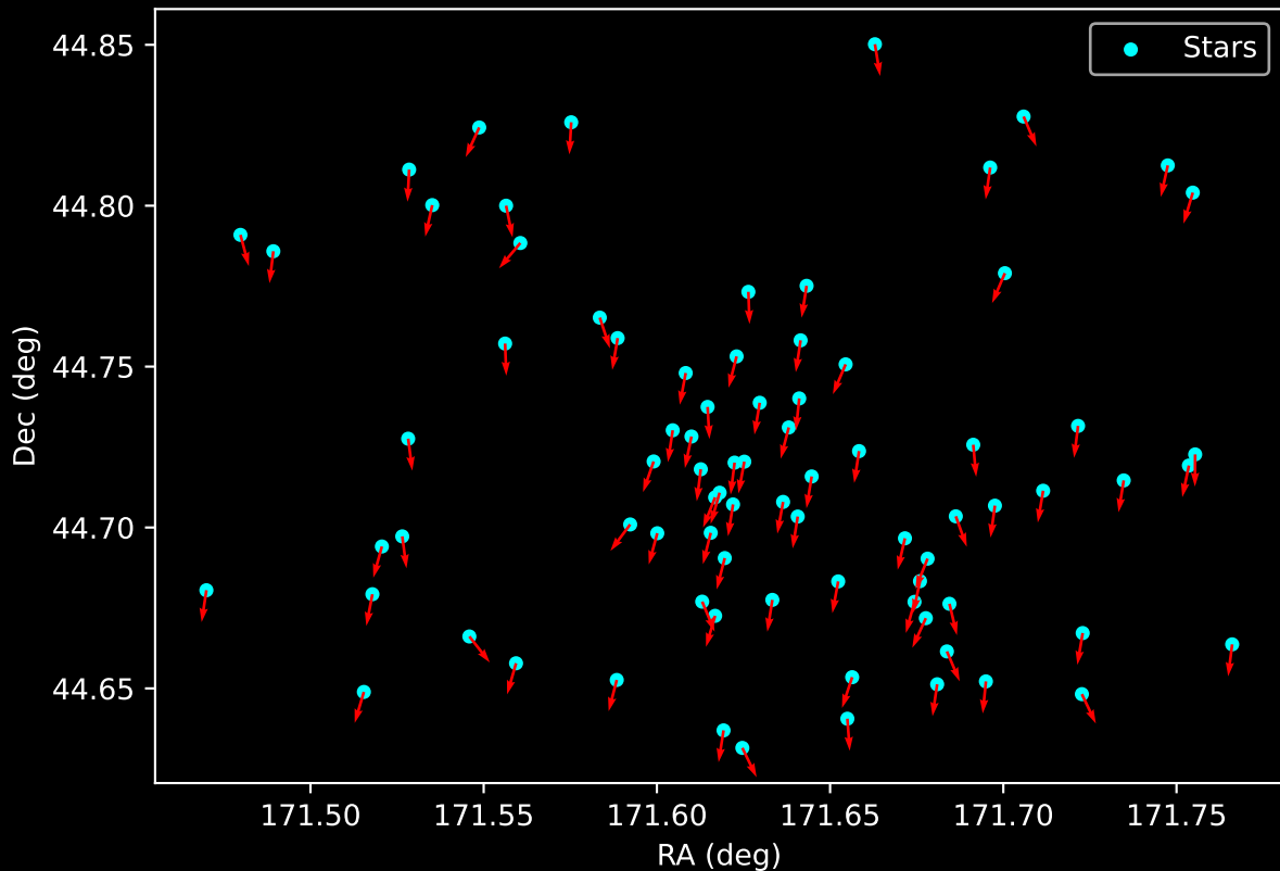
Gaia Cluster: [Ruprecht_148] Proper Motion Vectors for Gaia Star Field (n= 81)
