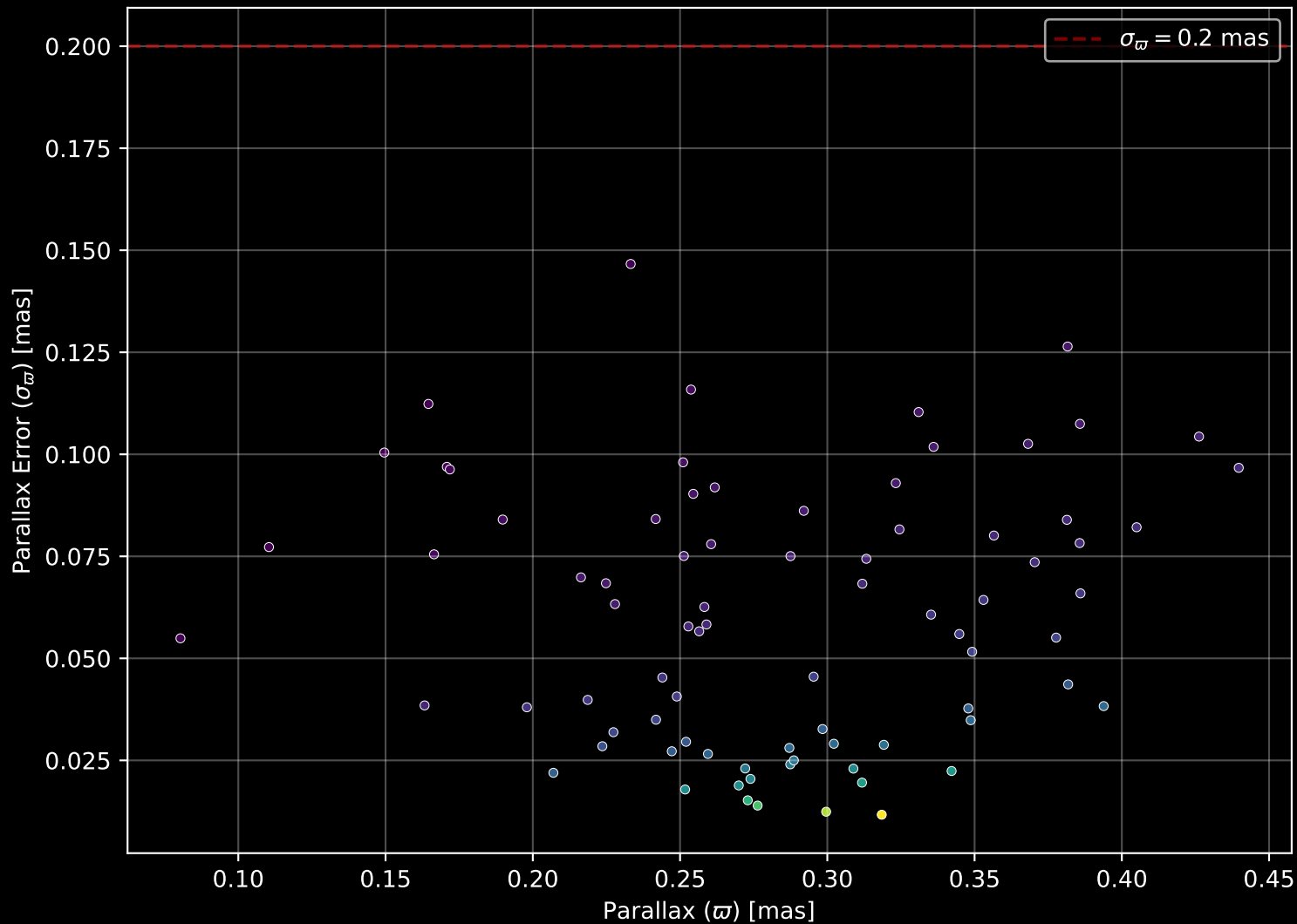
Gaia Cluster: [Ruprecht_148] Parallax Quality (n= 81)
