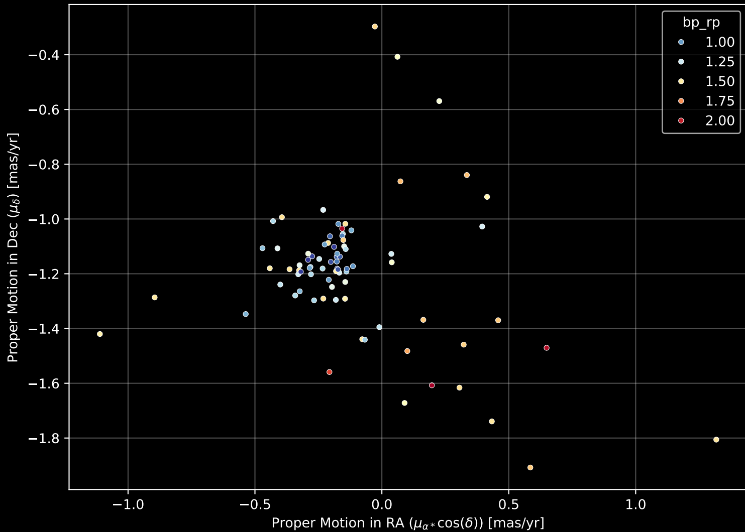
Gaia Cluster: [Ruprecht_148] Proper Motion Diagram (n= 81)
