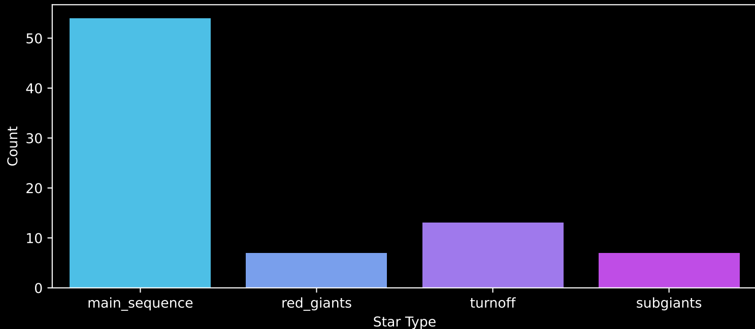
Gaia Cluster: [Ruprecht_148] Count plot of Star Type
