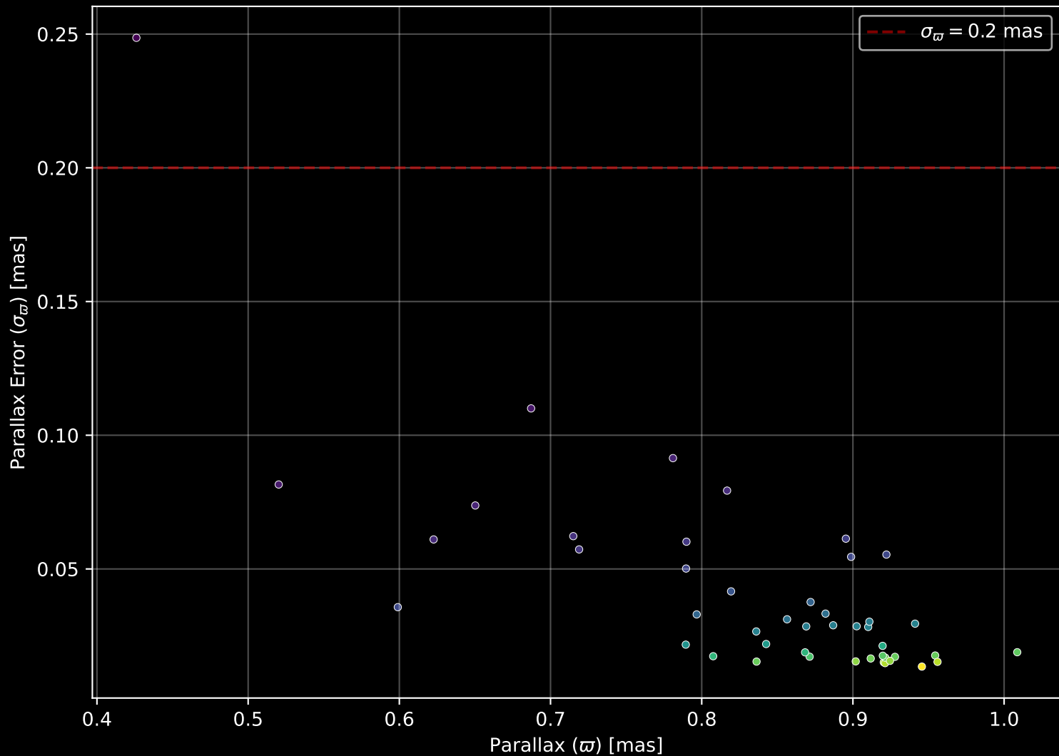
Gaia Cluster: [Ruprecht_151] Parallax Quality (n= 46)
