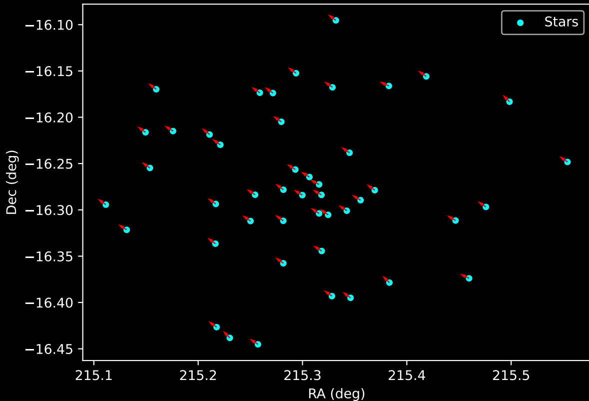
Gaia Cluster: [Ruprecht_151] Proper Motion Vectors for Gaia Star Field (n= 46)
