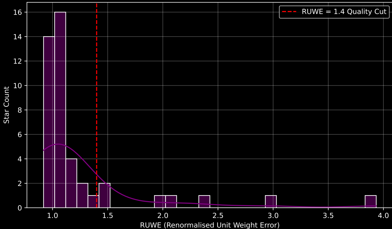
Gaia Cluster: [Ruprecht_151] RUWE Distribution (n= 44)
