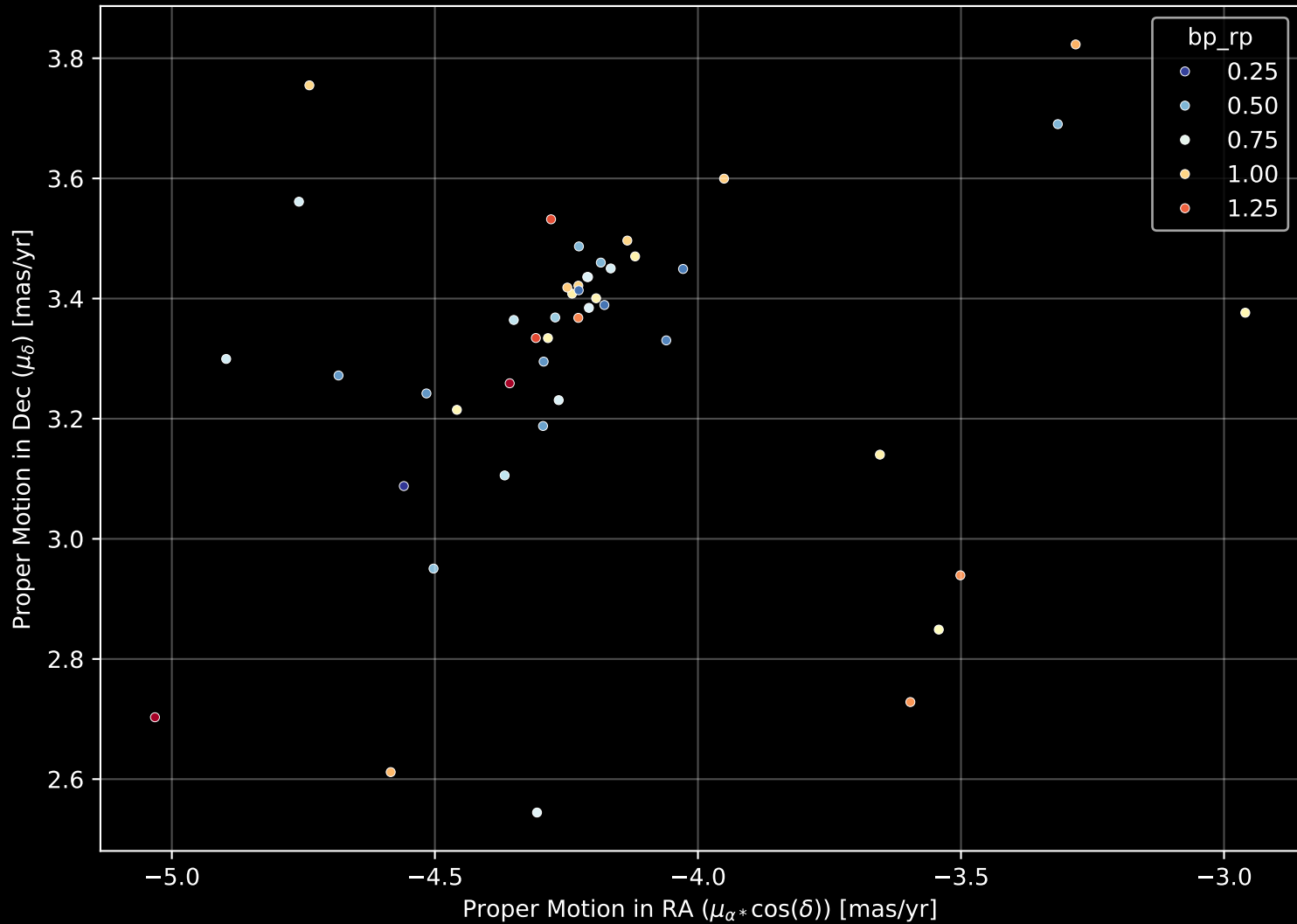
Gaia Cluster: [Ruprecht_151] Proper Motion Diagram (n= 46)
