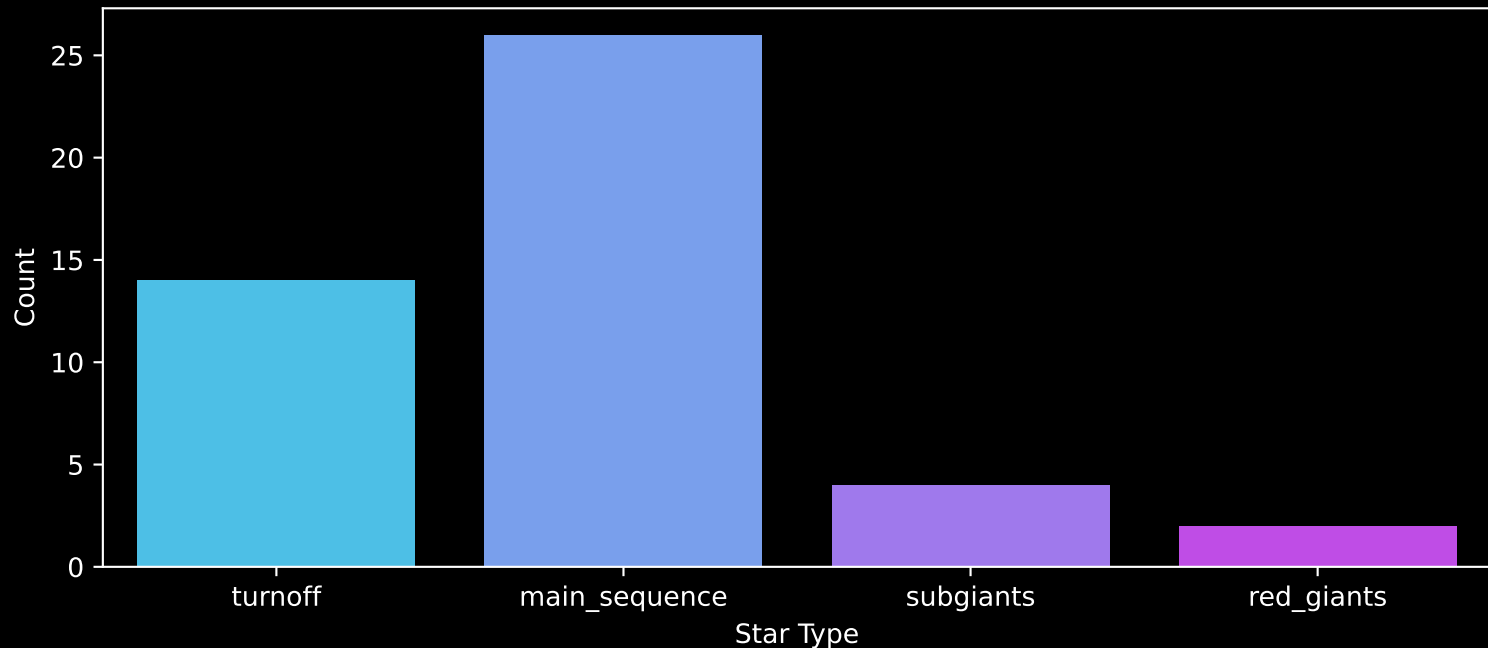
Gaia Cluster: [Ruprecht_151] Count plot of Star Type
