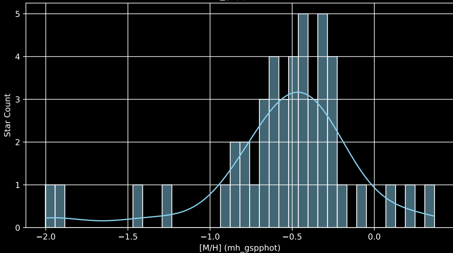
Gaia Cluster: [Ruprecht_151 [M/H] (mh_gspphot) (n= 46)
