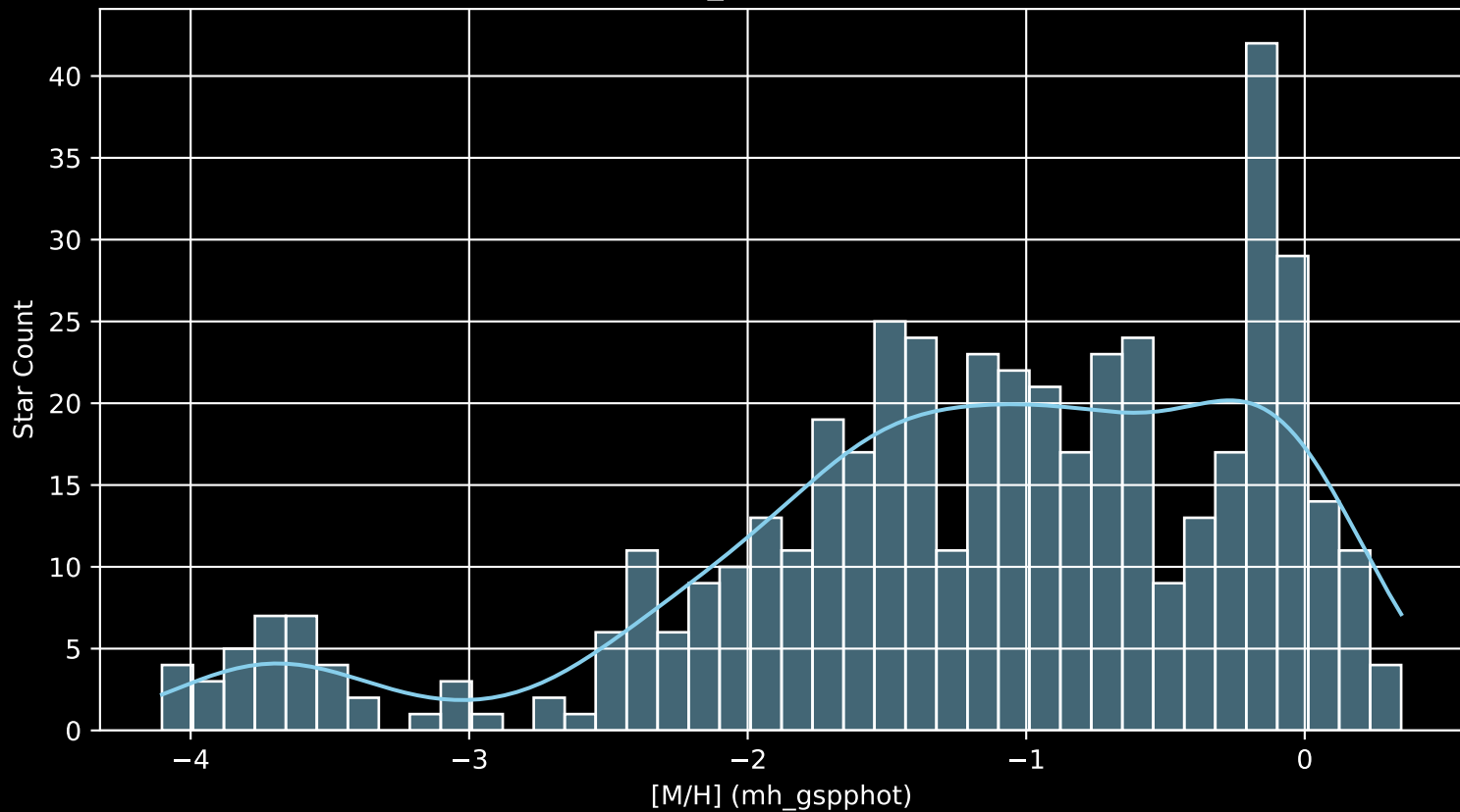
Gaia Cluster: [Ruprecht_164 [M/H] (mh_gspphot) (n= 471)
