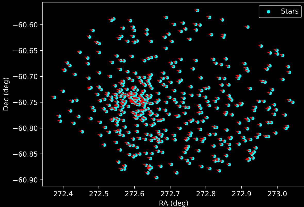
Gaia Cluster: [Ruprecht_164] Proper Motion Vectors for Gaia Star Field (n= 473)
