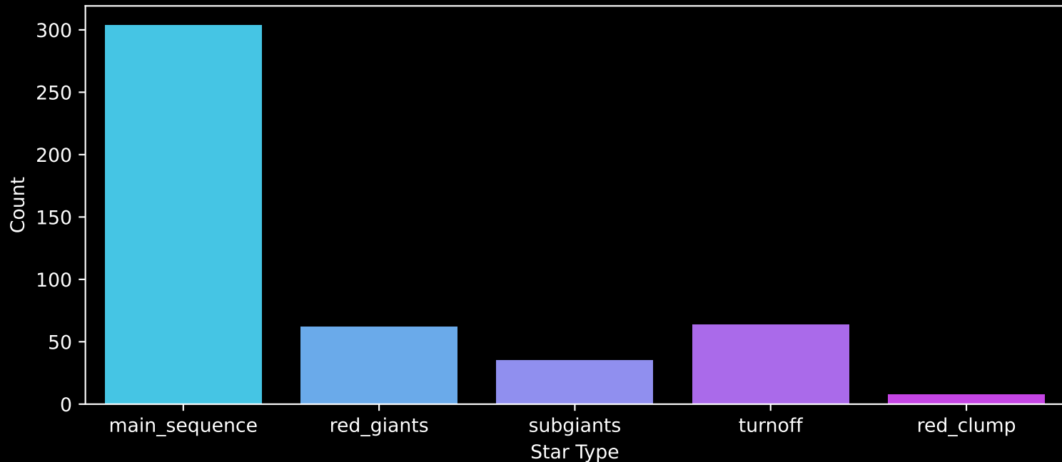
Gaia Cluster: [Ruprecht_164] Count plot of Star Type
