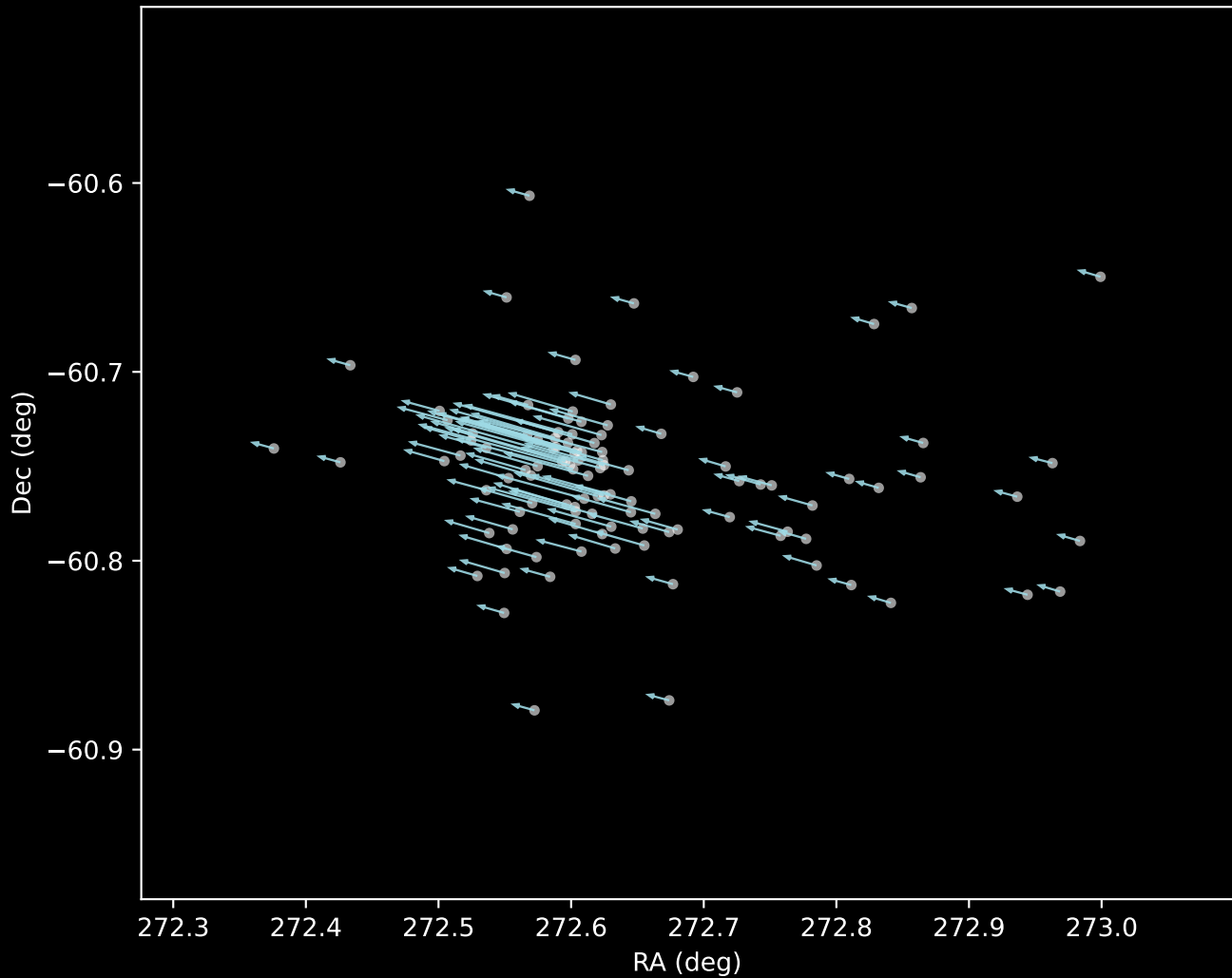
Gaia DR3 Cluster 19 Proper Motion Vectors (n=109)
