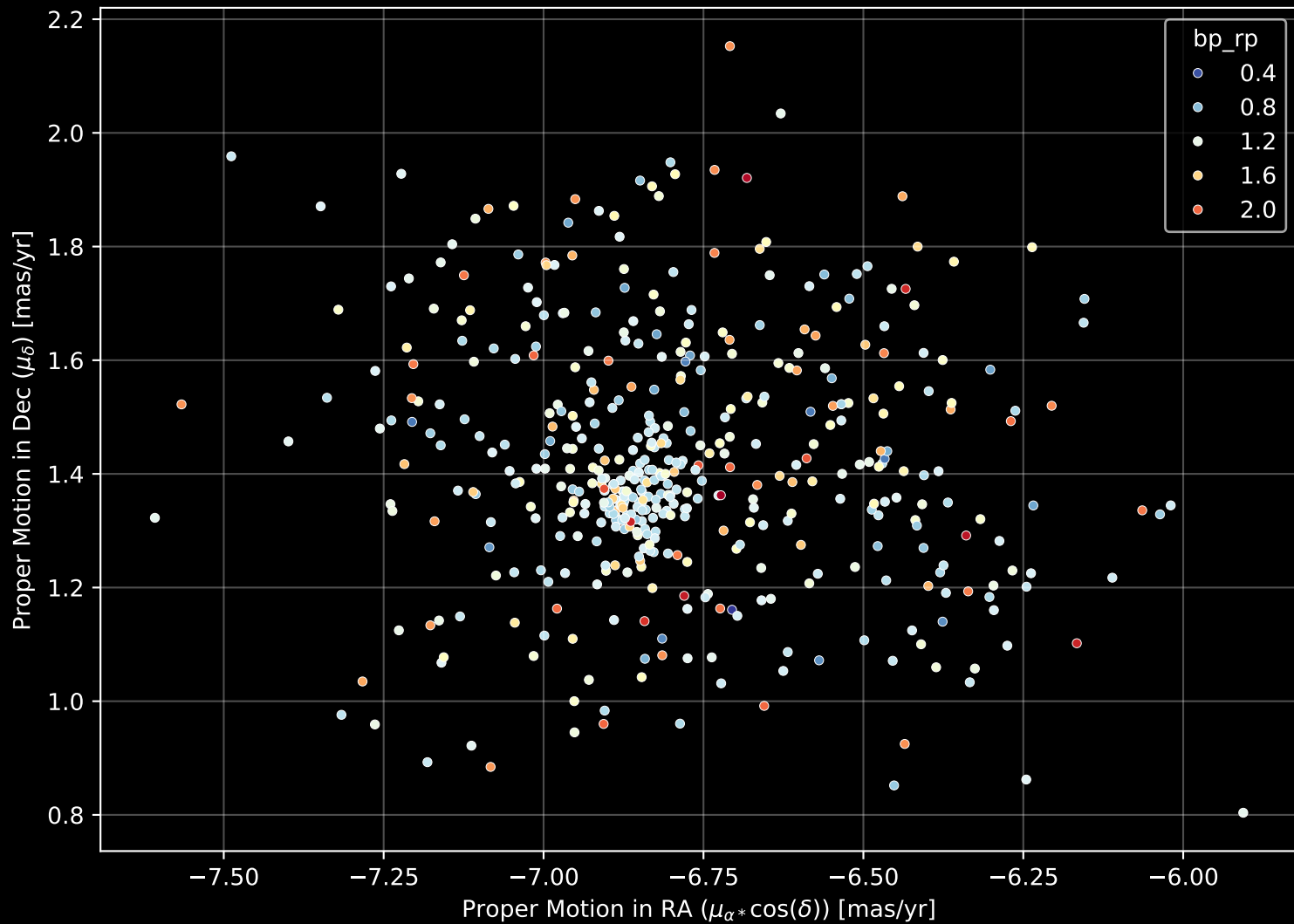
Gaia Cluster: [Ruprecht_164] Proper Motion Diagram (n= 473)
