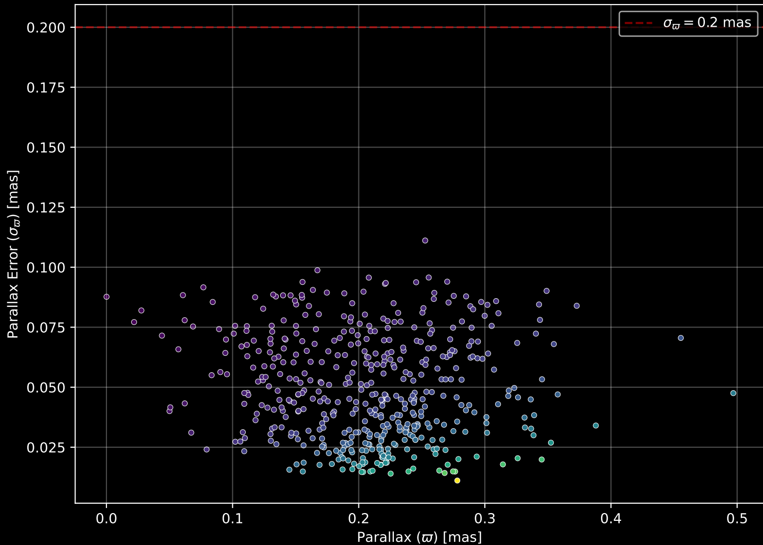
Gaia Cluster: [Ruprecht_164] Parallax Quality (n= 473)
