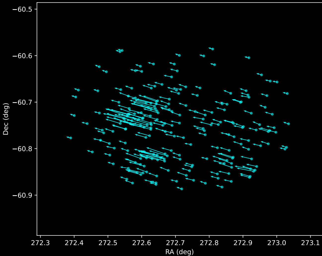
Gaia DR3 Noise Stream Proper Motion Vectors (n=212)
