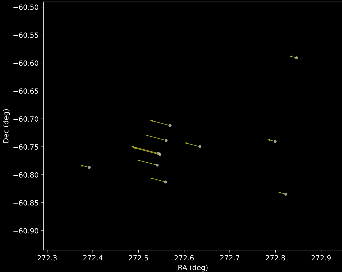
Gaia DR3 Cluster 16 Proper Motion Vectors (n=11)
