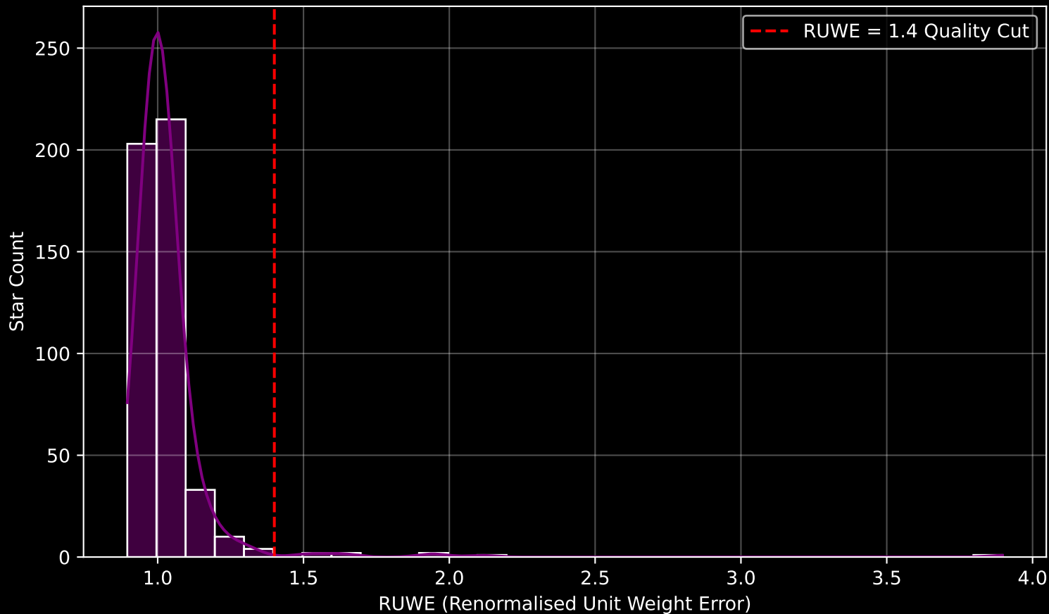
Gaia Cluster: [Ruprecht_164] RUWE Distribution (n= 473)
