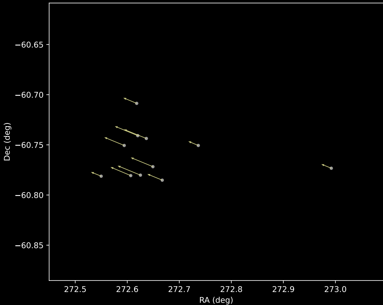
Gaia DR3 Cluster 17 Proper Motion Vectors (n=11)
