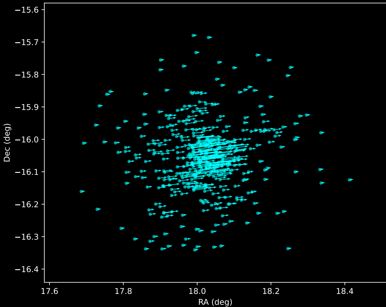
Gaia DR3 Noise Stream Proper Motion Vectors (n=375)
