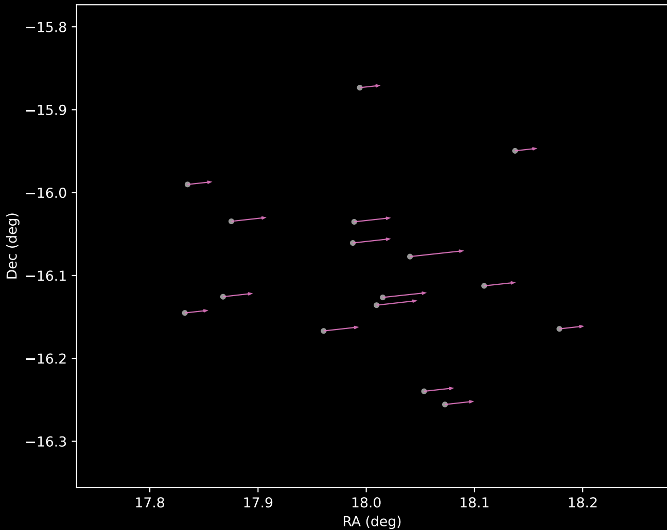
Gaia DR3 Cluster 32 Proper Motion Vectors (n=16)
