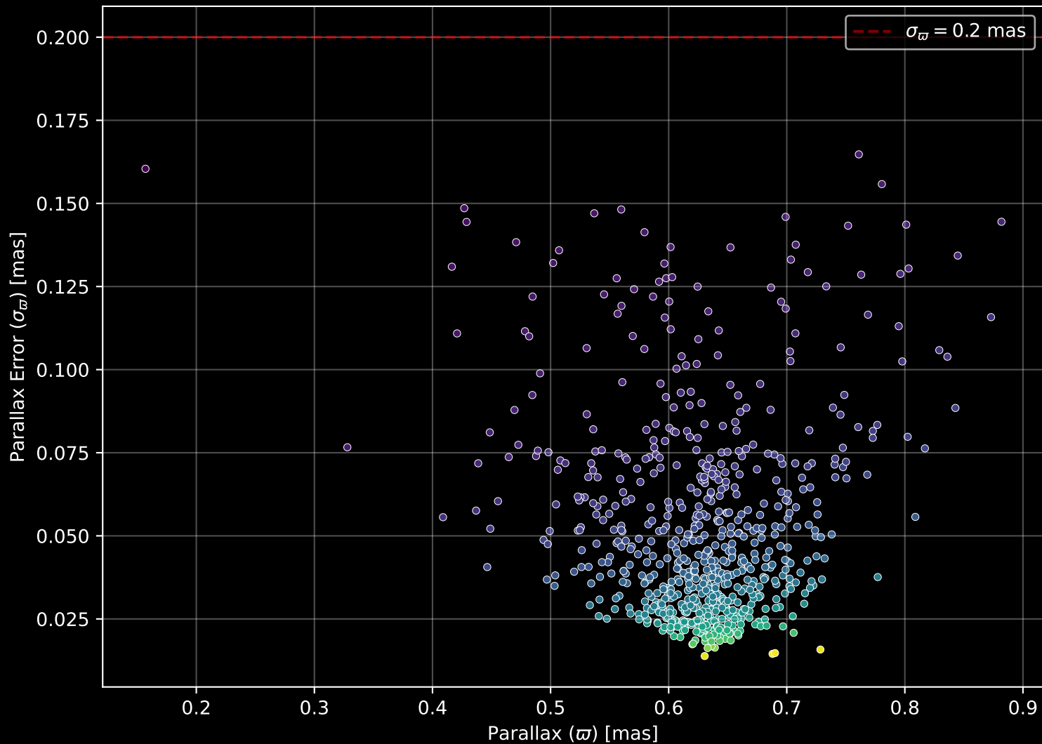
Gaia Cluster: [Ruprecht_171] Parallax Quality (n= 701)
