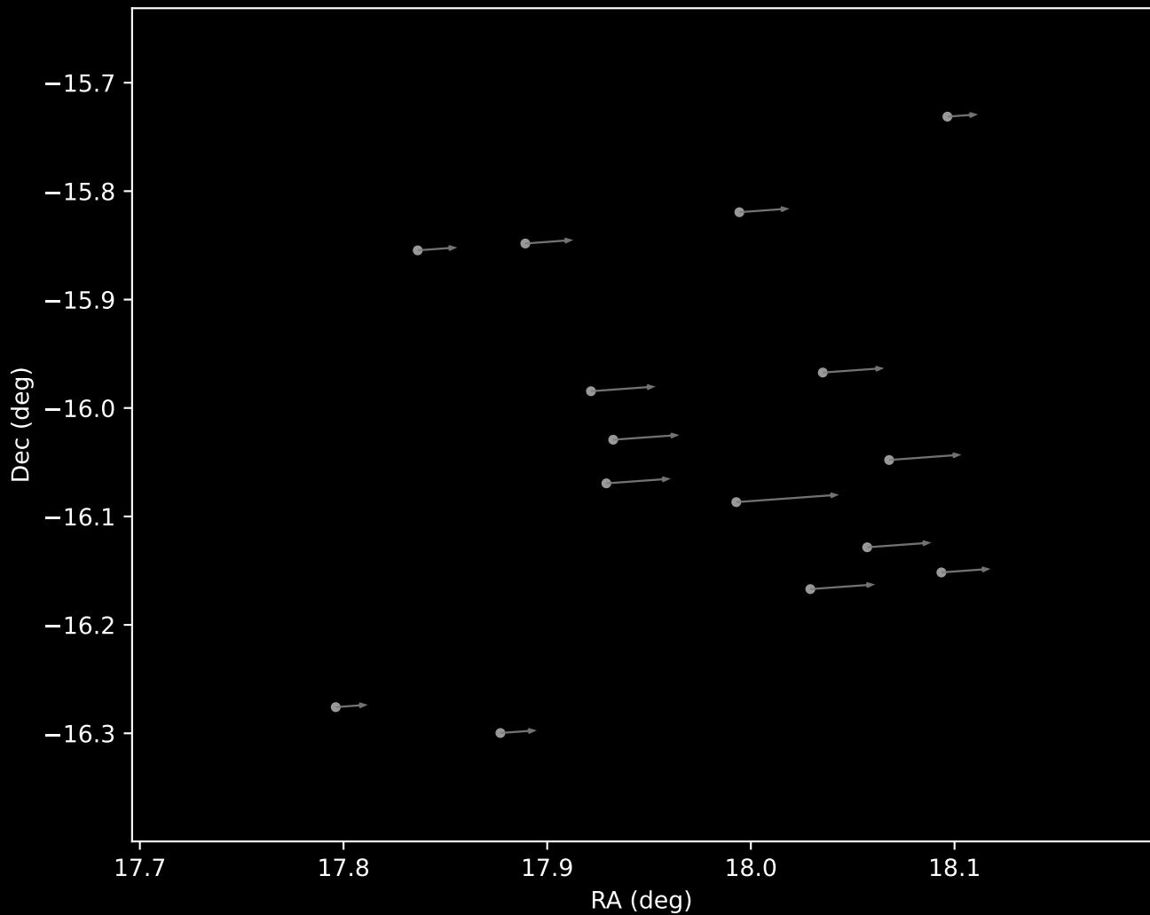
Gaia DR3 Cluster 34 Proper Motion Vectors (n=15)
