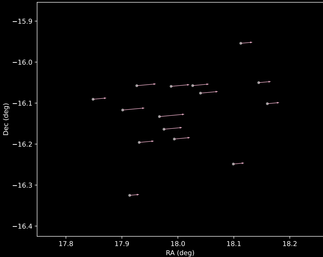
Gaia DR3 Cluster 13 Proper Motion Vectors (n=15)
