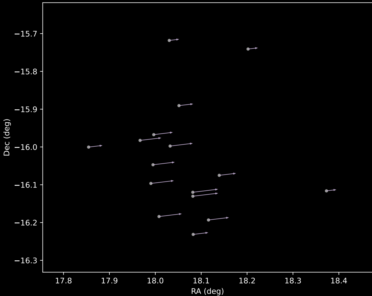
Gaia DR3 Cluster 29 Proper Motion Vectors (n=16)
