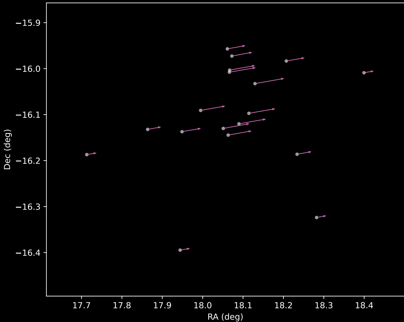
Gaia DR3 Cluster 12 Proper Motion Vectors (n=18)
