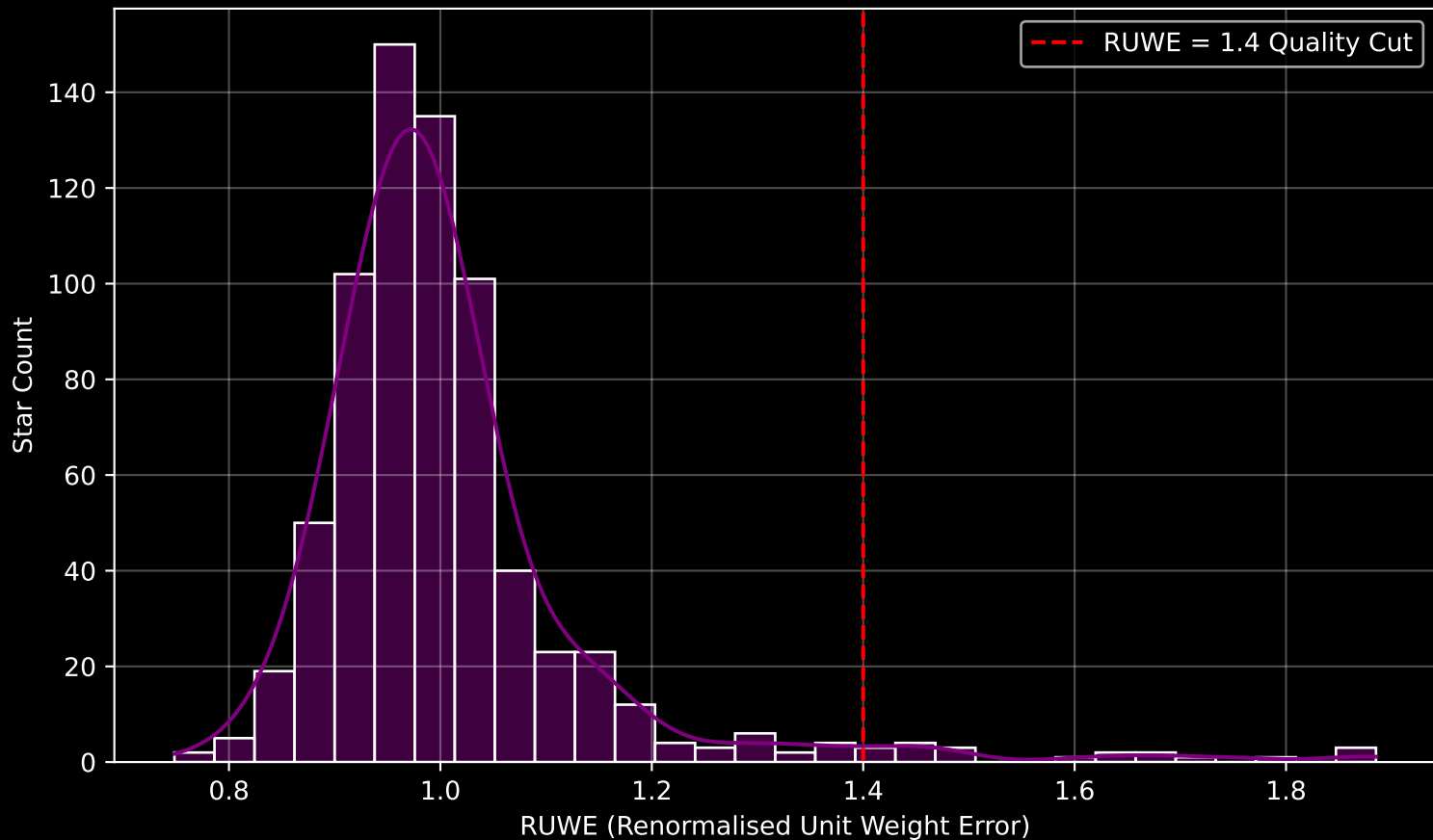
Gaia Cluster: [Ruprecht_171] RUWE Distribution (n= 701)
