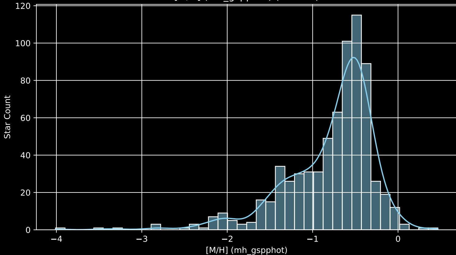
Gaia Cluster: [Ruprecht_171 [M/H] (mh_gspphot) (n= 701)
