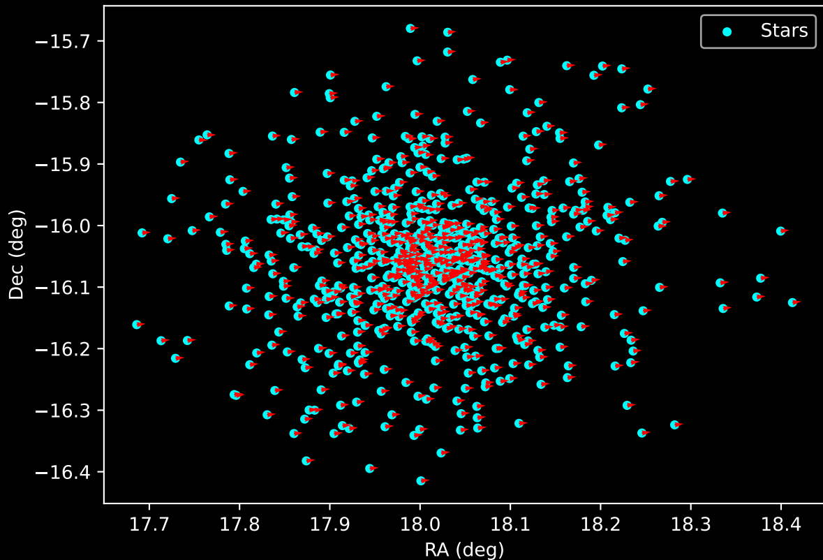
Gaia Cluster: [Ruprecht_171] Proper Motion Vectors for Gaia Star Field (n= 701)
