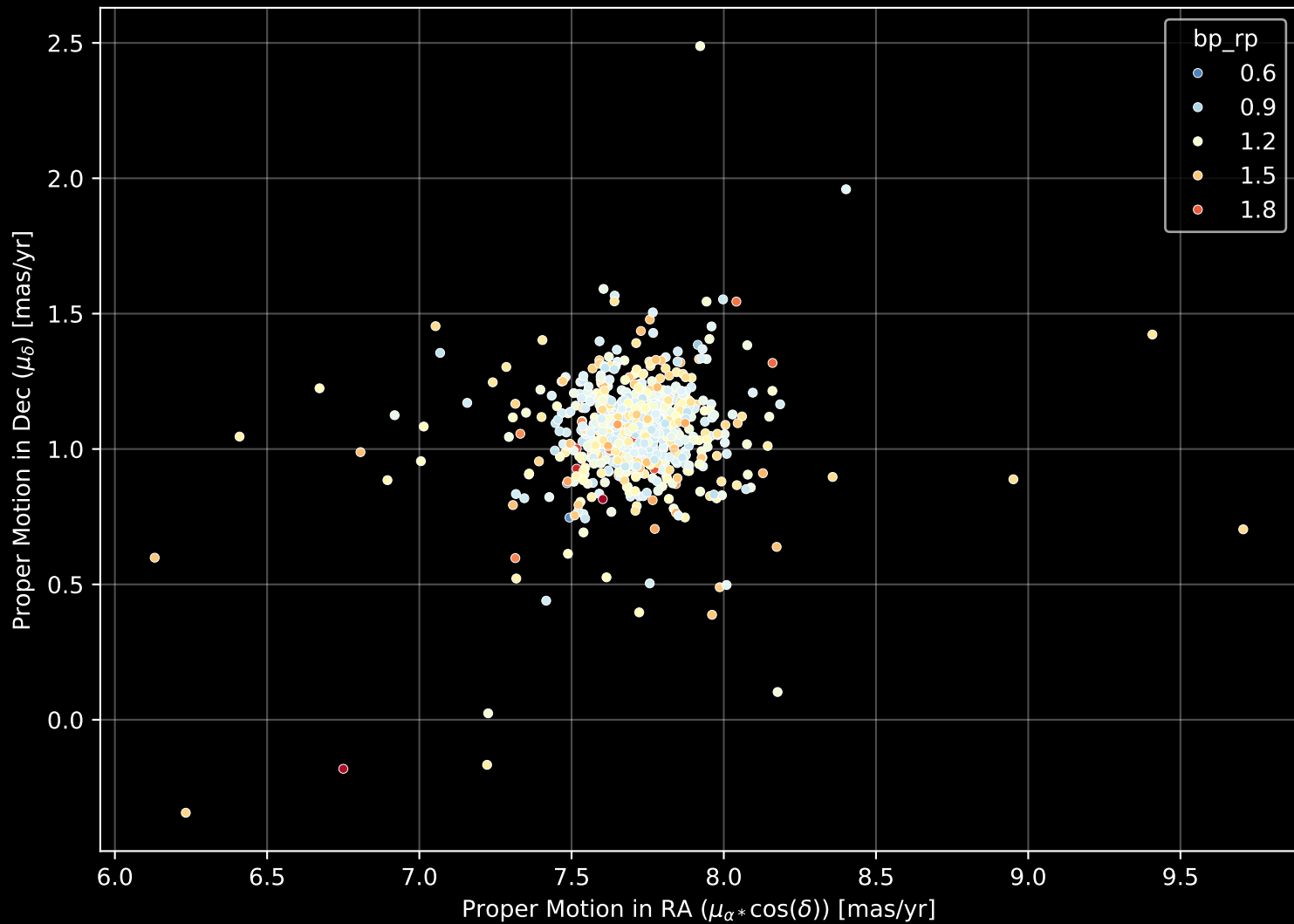
Gaia Cluster: [Ruprecht_171] Proper Motion Diagram (n= 701)
