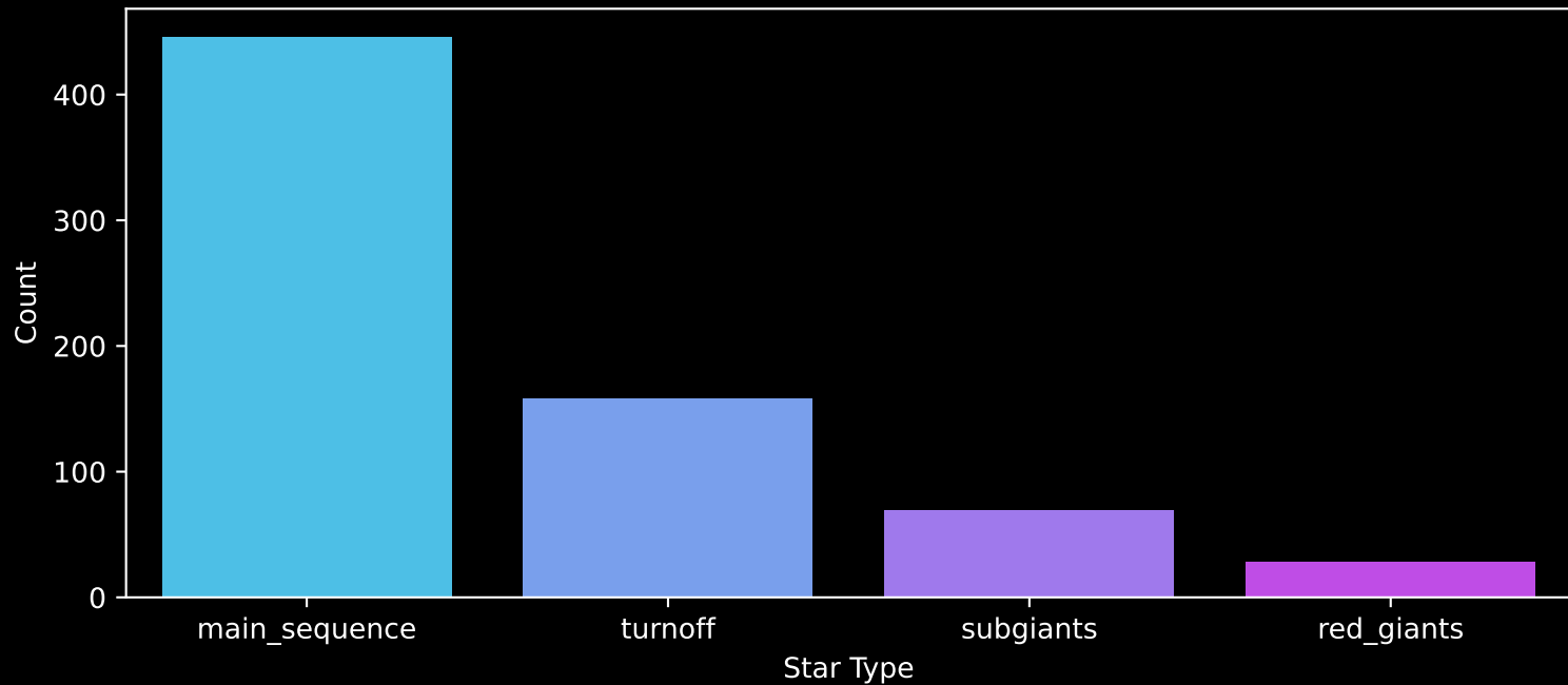
Gaia Cluster: [Ruprecht_171] Count plot of Star Type
