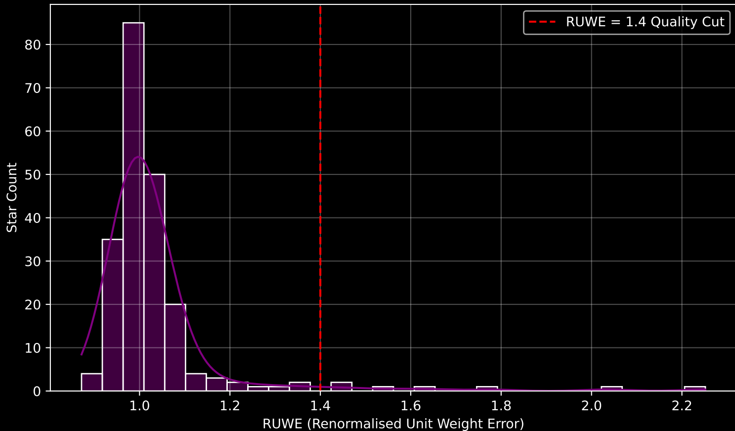
Gaia Cluster: [Ruprecht_176] RUWE Distribution (n= 214)
