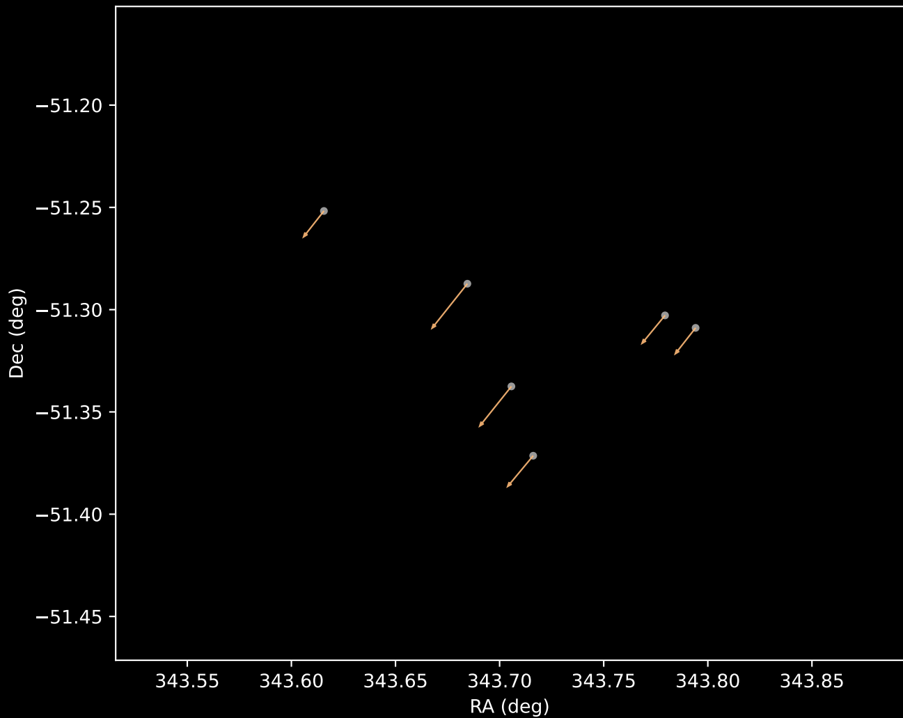
Gaia DR3 Cluster 3 Proper Motion Vectors (n=6)
