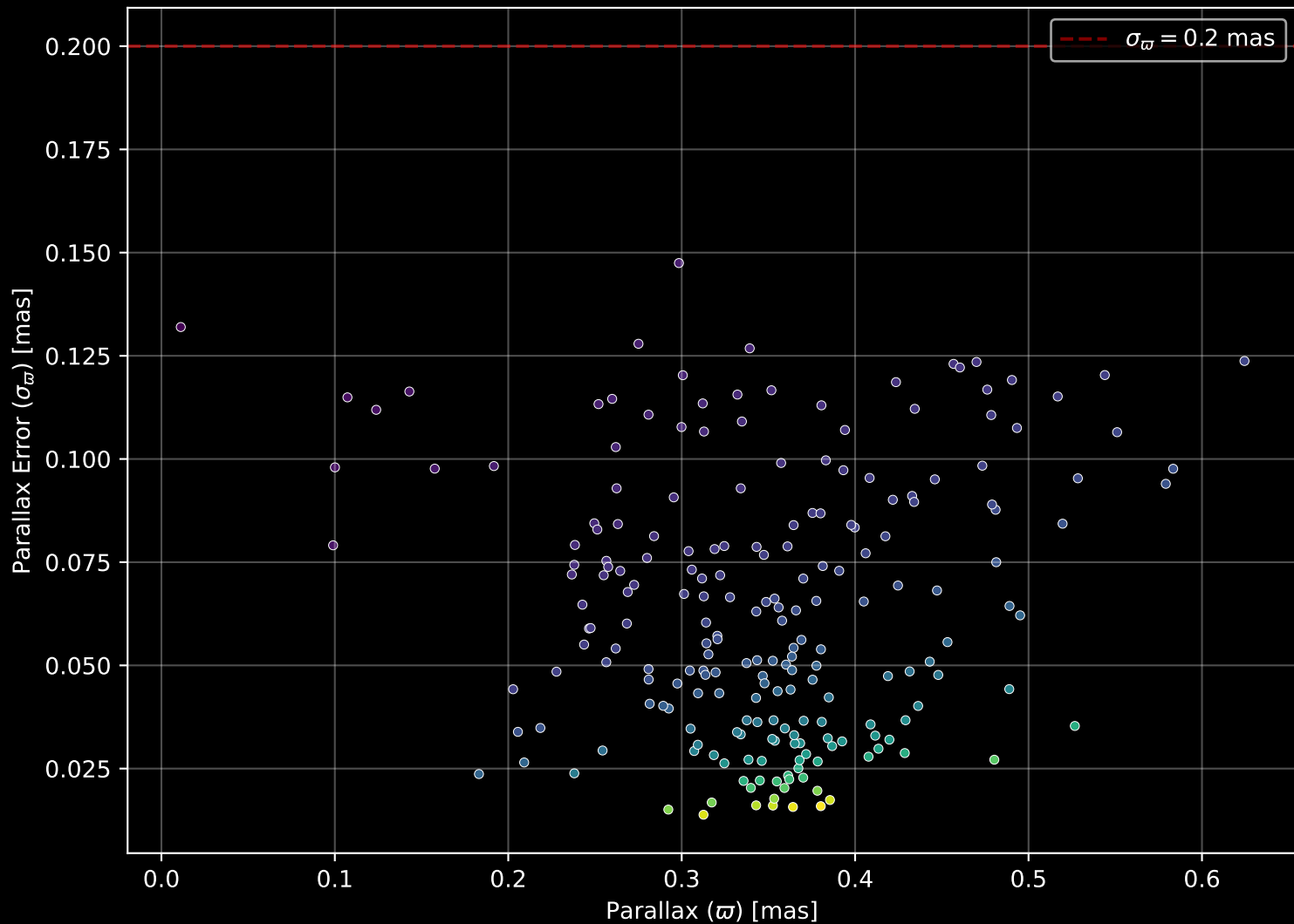
Gaia Cluster: [Ruprecht_176] Parallax Quality (n= 214)
