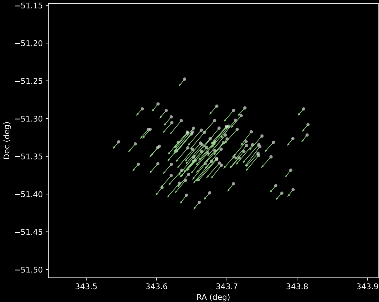
Gaia DR3 Cluster 5 Proper Motion Vectors (n=92)
