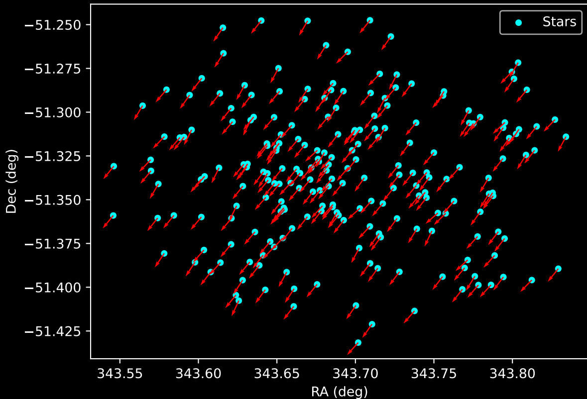
Gaia Cluster: [Ruprecht_176] Proper Motion Vectors for Gaia Star Field (n= 214)
