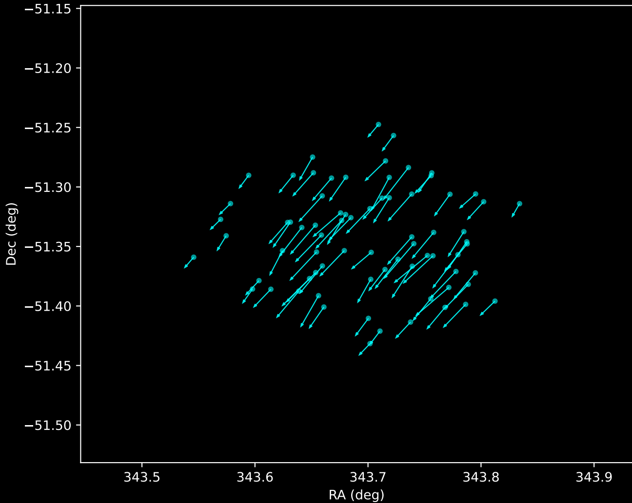
Gaia DR3 Noise Stream Proper Motion Vectors (n=73)
