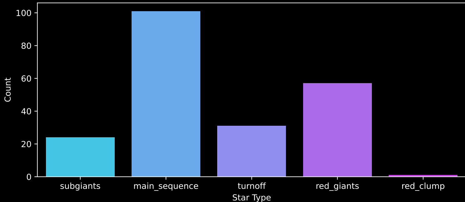
Gaia Cluster: [Ruprecht_176] Count plot of Star Type
