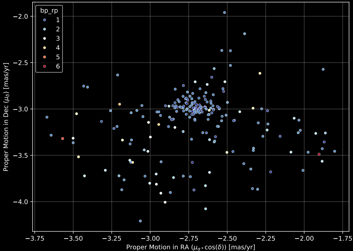
Gaia Cluster: [Ruprecht_176] Proper Motion Diagram (n= 214)
