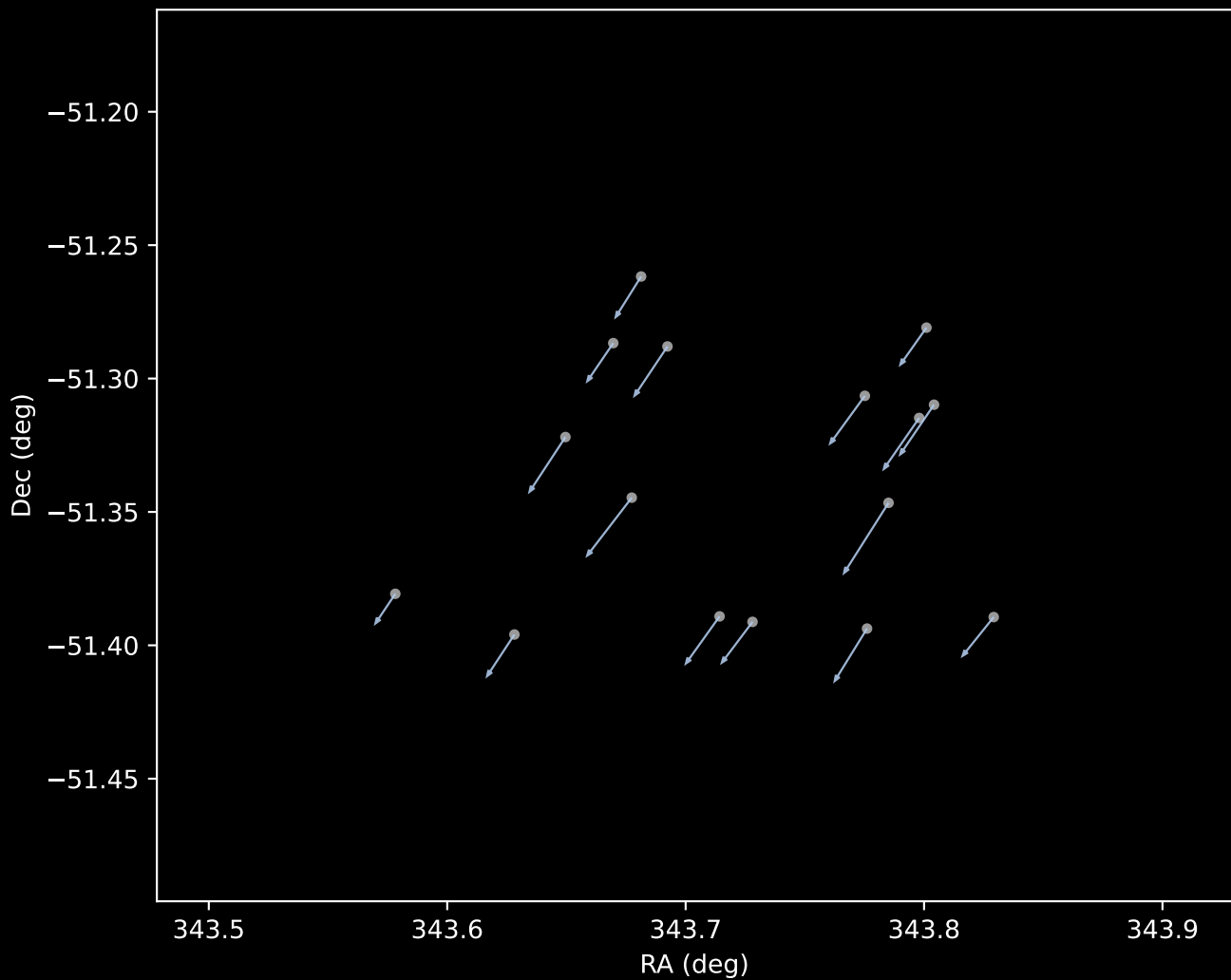
Gaia DR3 Cluster 1 Proper Motion Vectors (n=16)
