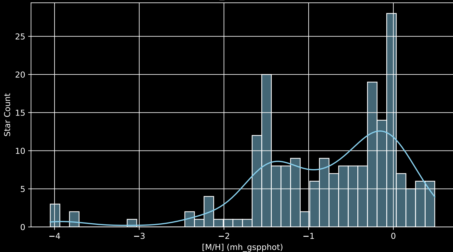
Gaia Cluster: [Ruprecht_176 [M/H] (mh_gspphot) (n= 207)
