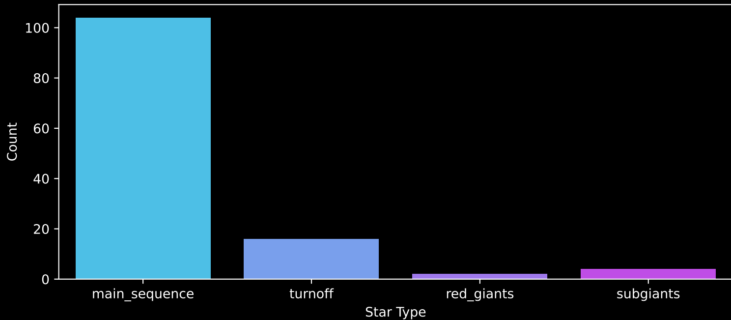
Gaia Cluster: [Ruprecht_19] Count plot of Star Type
