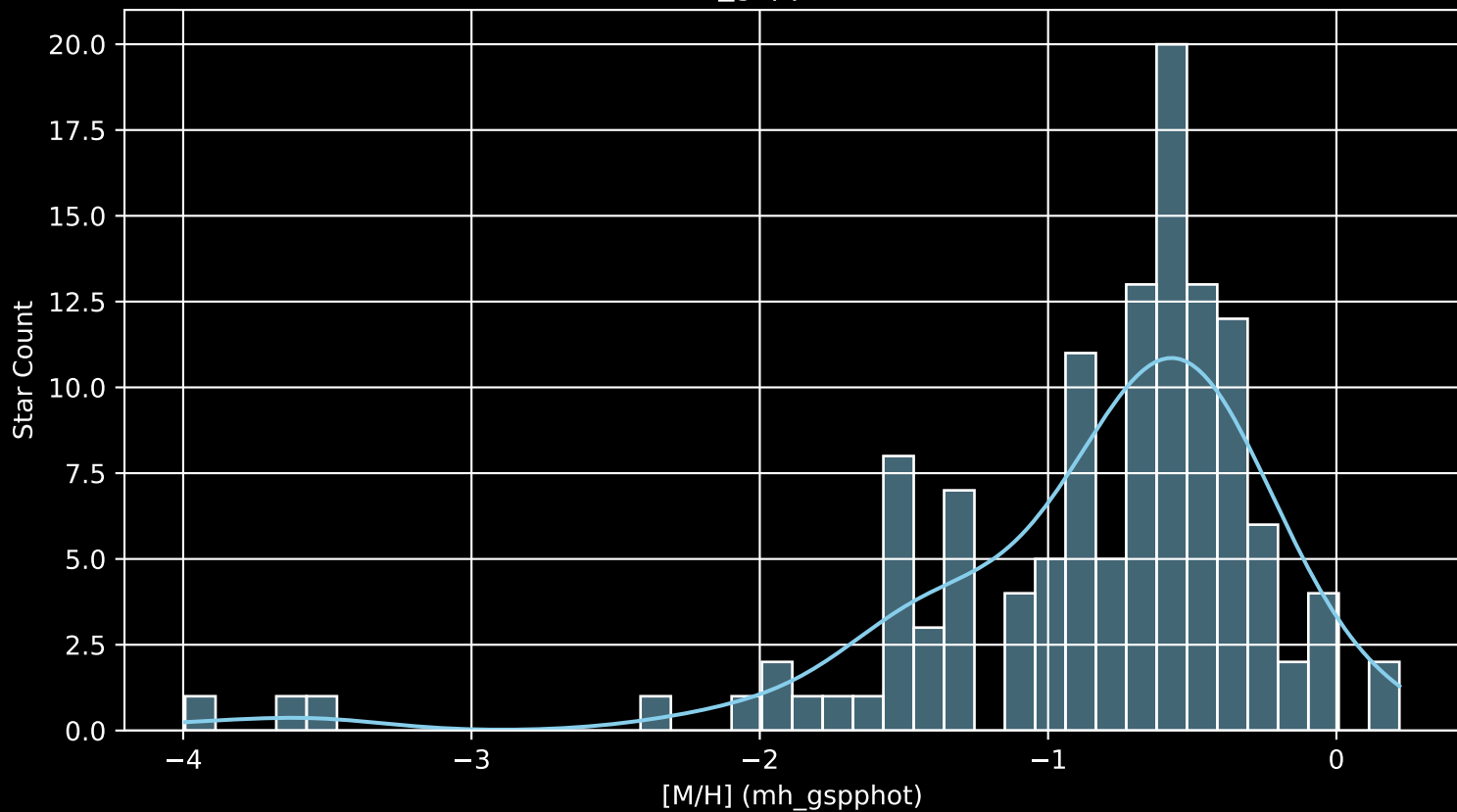
Gaia Cluster: [Ruprecht_19 [M/H] (mh_gspphot) (n= 125)
