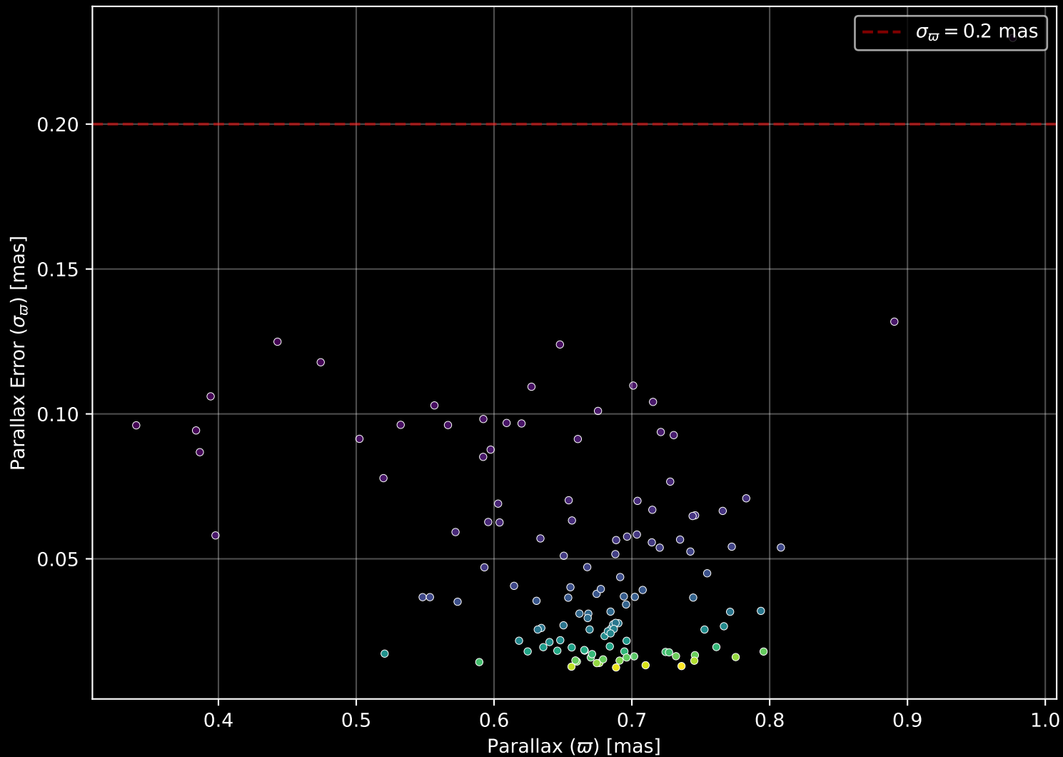
Gaia Cluster: [Ruprecht_19] Parallax Quality (n= 126)
