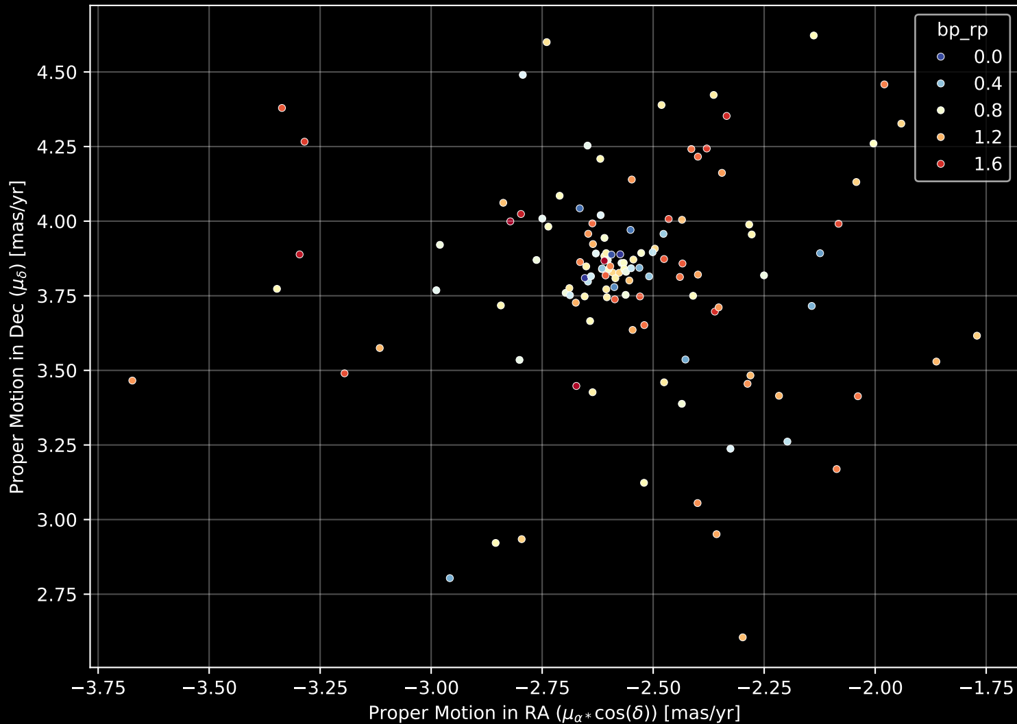
Gaia Cluster: [Ruprecht_19] Proper Motion Diagram (n= 126)
