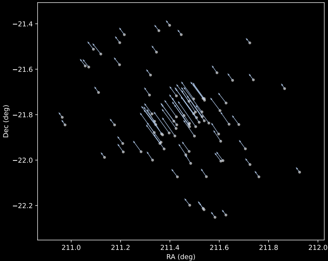
Gaia DR3 Cluster 1 Proper Motion Vectors (n=84)
