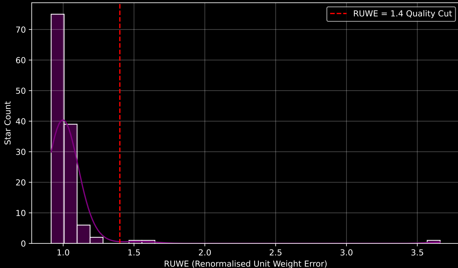
Gaia Cluster: [Ruprecht_19] RUWE Distribution (n= 125)
