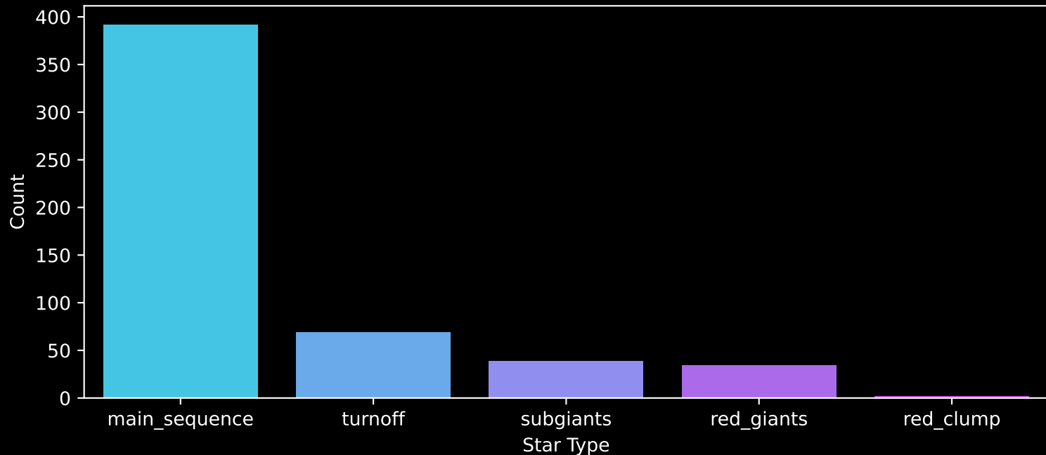
Gaia Cluster: [Ruprecht_23] Count plot of Star Type
