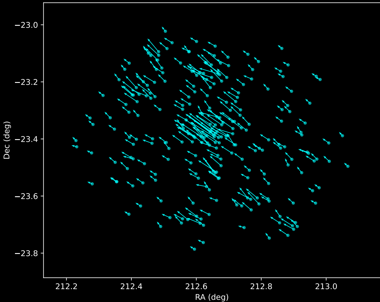
Gaia DR3 Noise Stream Proper Motion Vectors (n=239)
