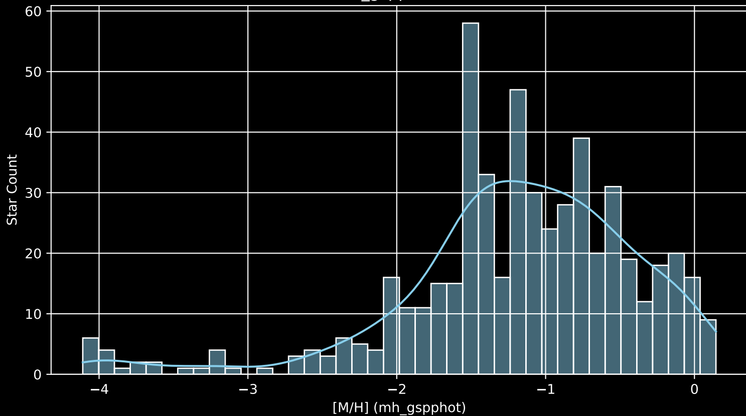
Gaia Cluster: [Ruprecht_23 [M/H] (mh_gspphot) (n= 536)
