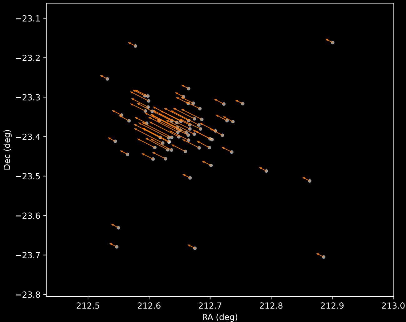
Gaia DR3 Cluster 22 Proper Motion Vectors (n=69)
