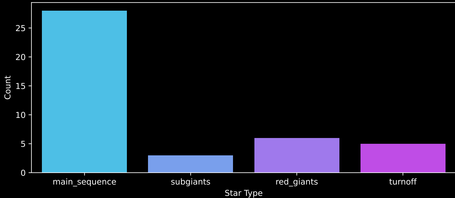
Gaia Cluster: [Ruprecht_25] Count plot of Star Type
