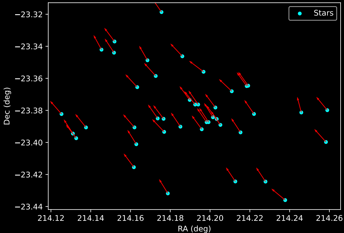
Gaia Cluster: [Ruprecht_25] Proper Motion Vectors for Gaia Star Field (n= 42)
