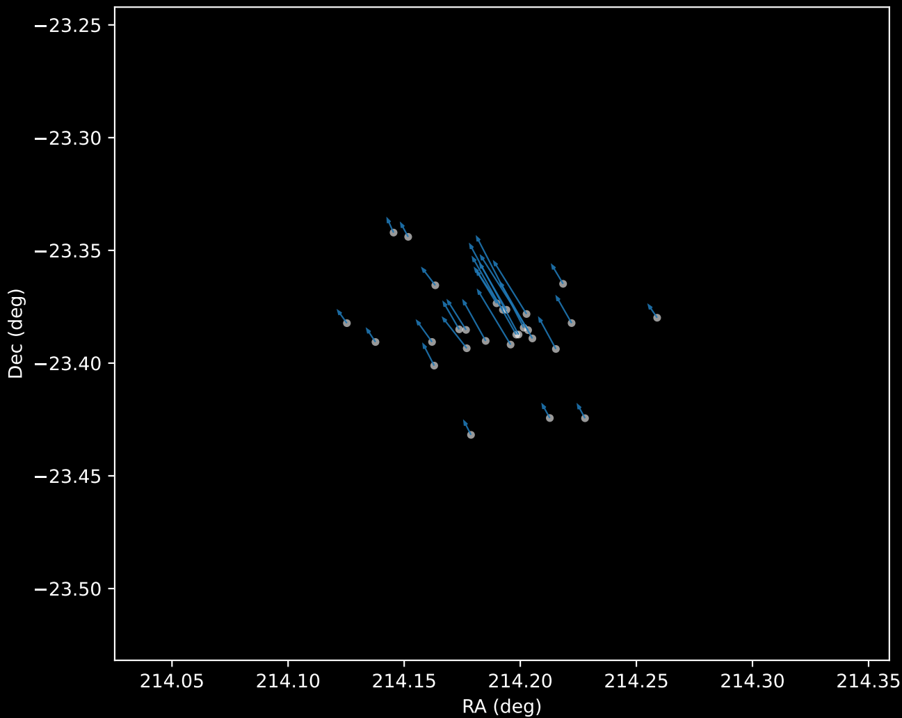
Gaia DR3 Cluster 0 Proper Motion Vectors (n=28)
