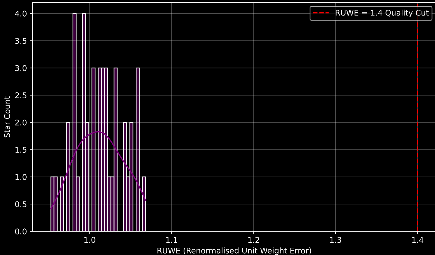
Gaia Cluster: [Ruprecht_25] RUWE Distribution (n= 42)
