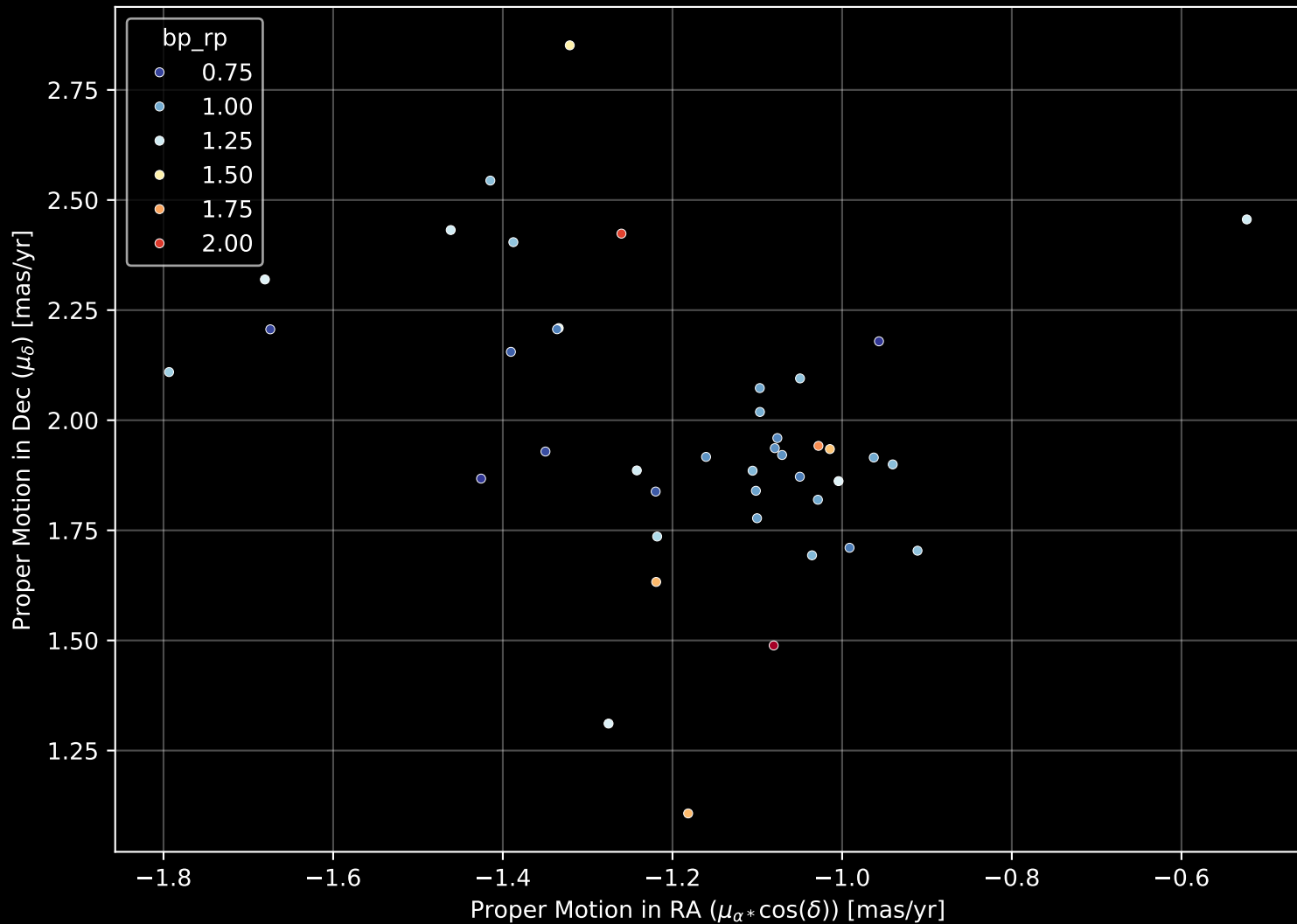
Gaia Cluster: [Ruprecht_25] Proper Motion Diagram (n= 42)
