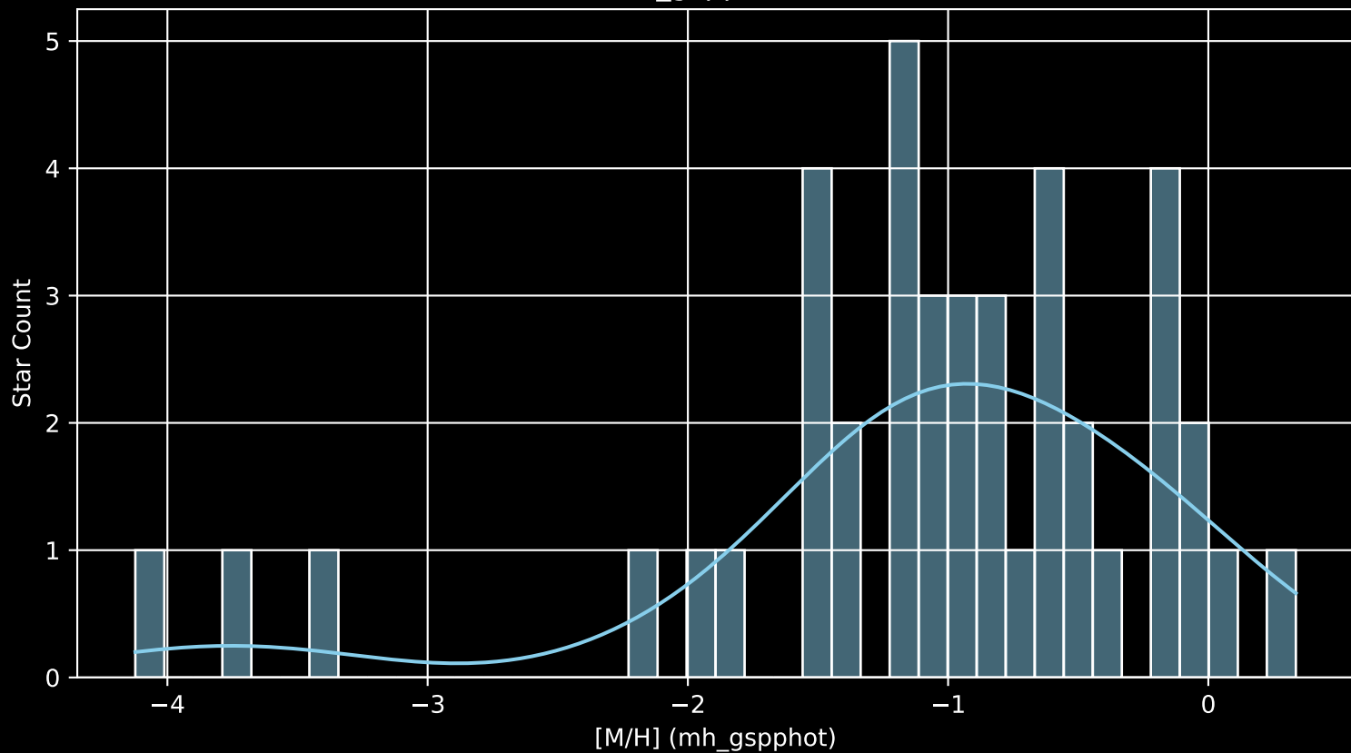
Gaia Cluster: [Ruprecht_25 [M/H] (mh_gspphot) (n= 42)
