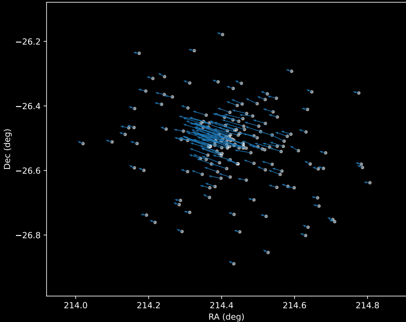
Gaia DR3 Cluster 0 Proper Motion Vectors (n=166)
