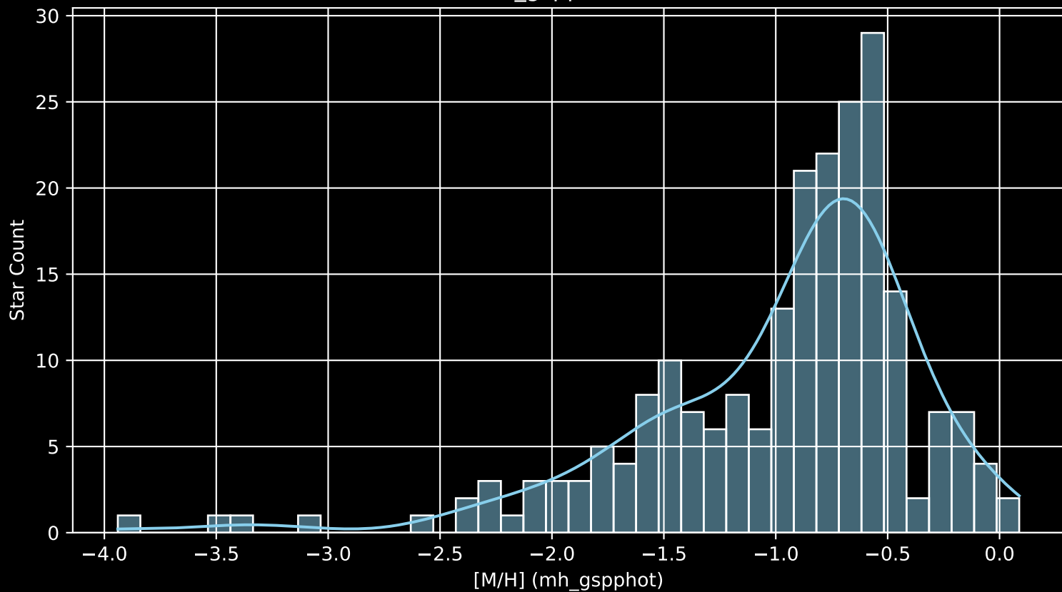
Gaia Cluster: [Ruprecht_27 [M/H] (mh_gspphot) (n= 220)
