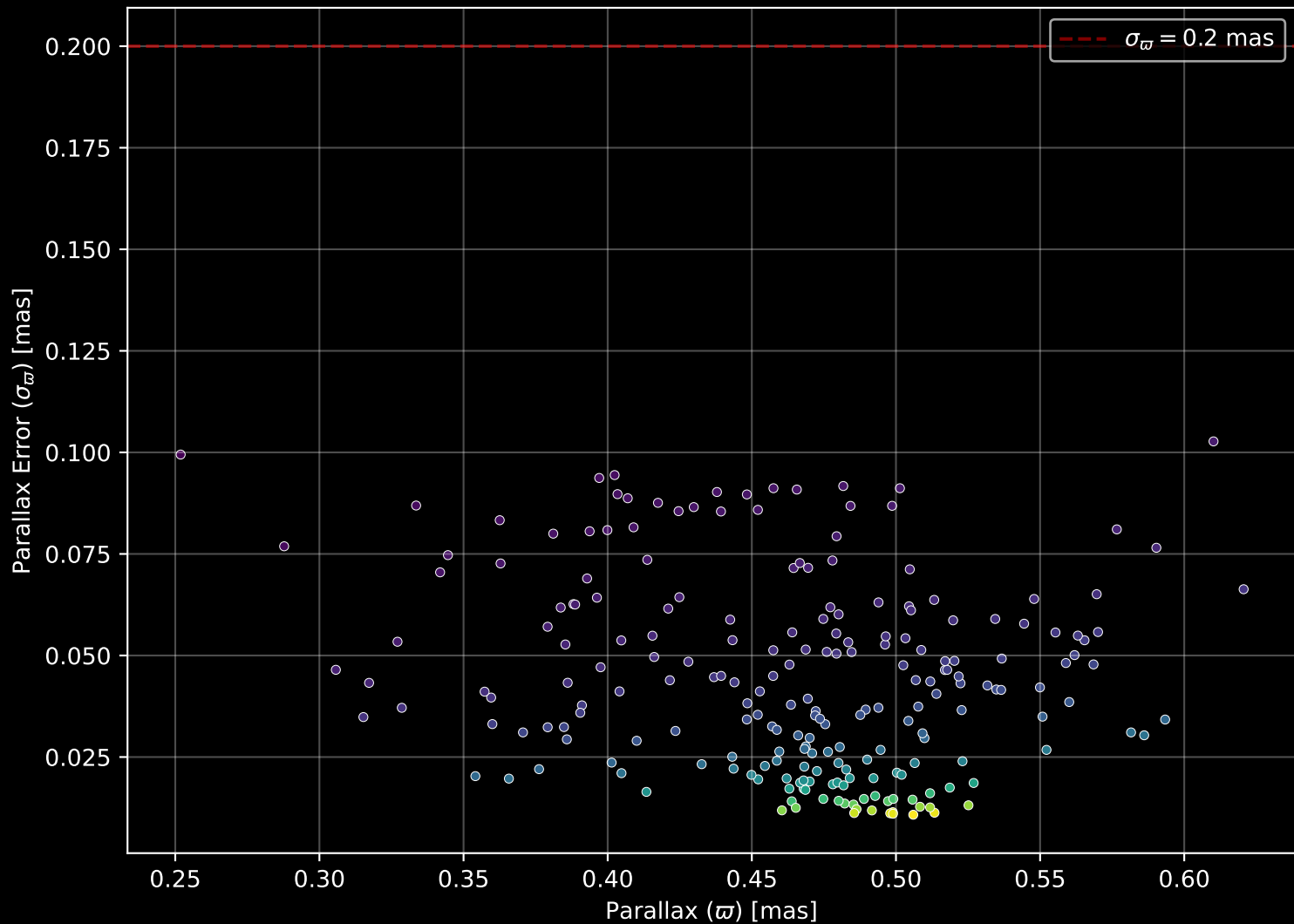
Gaia Cluster: [Ruprecht_27] Parallax Quality (n= 220)
