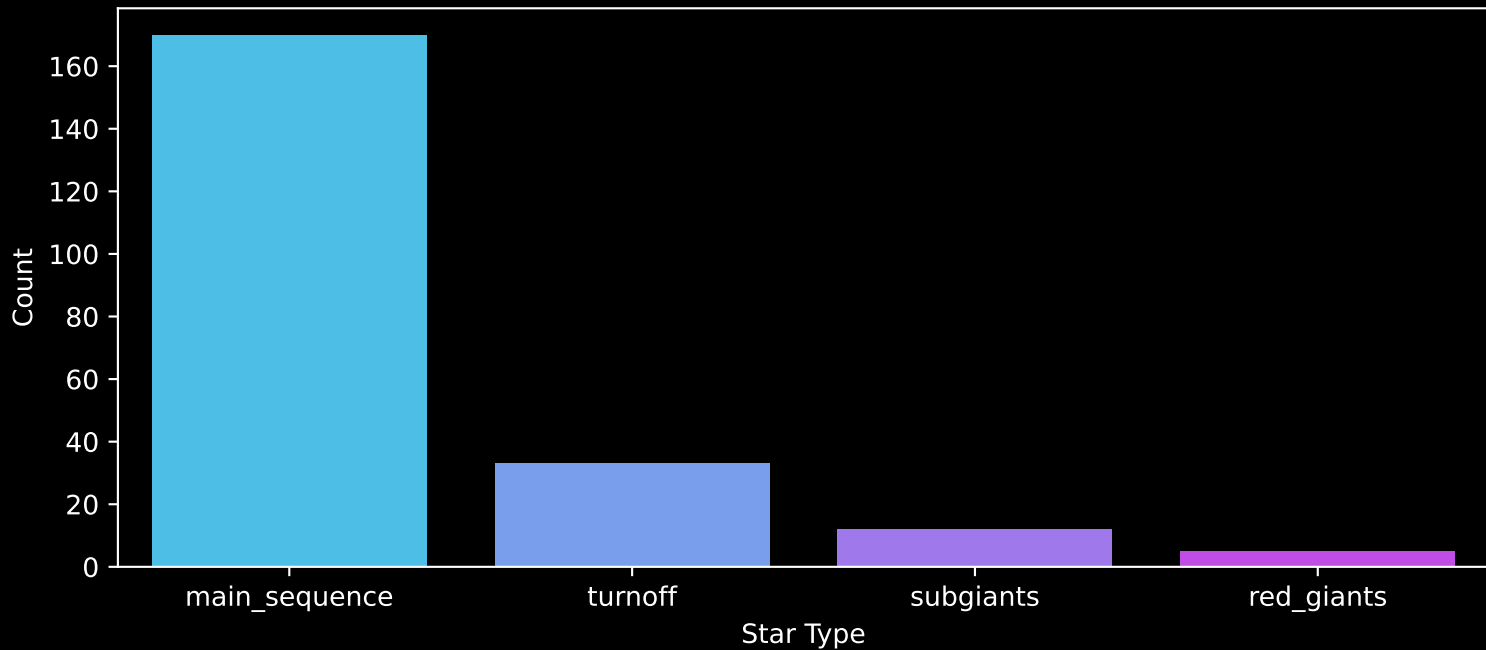
Gaia Cluster: [Ruprecht_27] Count plot of Star Type
