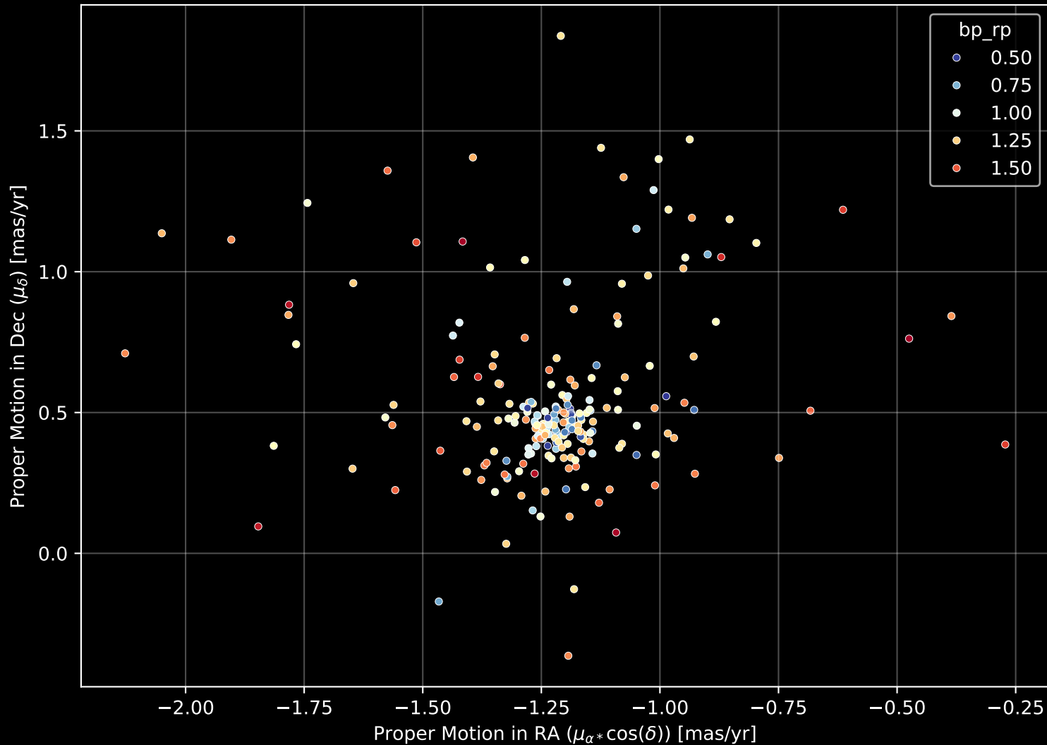
Gaia Cluster: [Ruprecht_27] Proper Motion Diagram (n= 220)
