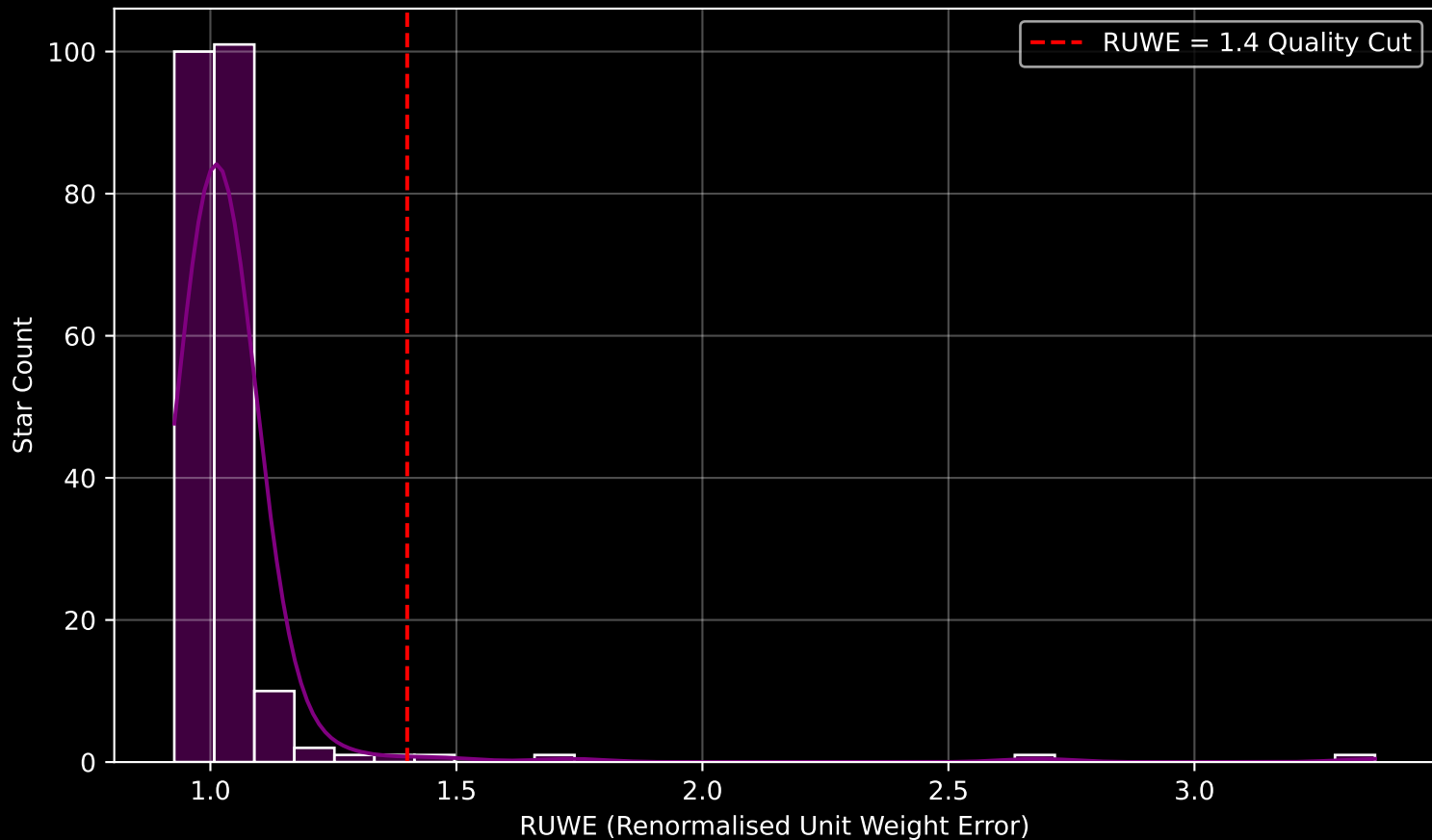
Gaia Cluster: [Ruprecht_27] RUWE Distribution (n= 219)
