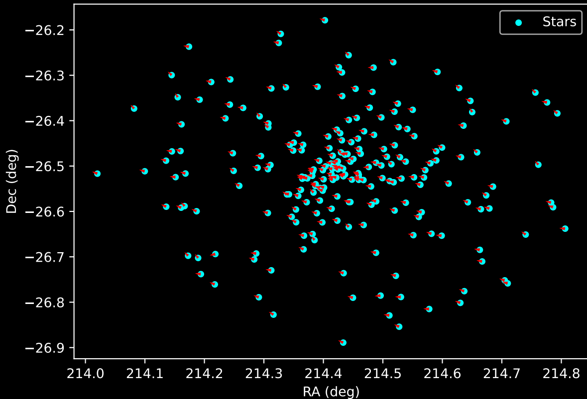
Gaia Cluster: [Ruprecht_27] Proper Motion Vectors for Gaia Star Field (n= 220)
