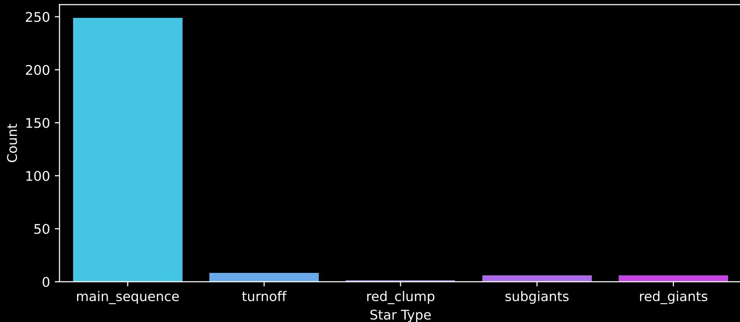
Gaia Cluster: [Ruprecht_28] Count plot of Star Type
