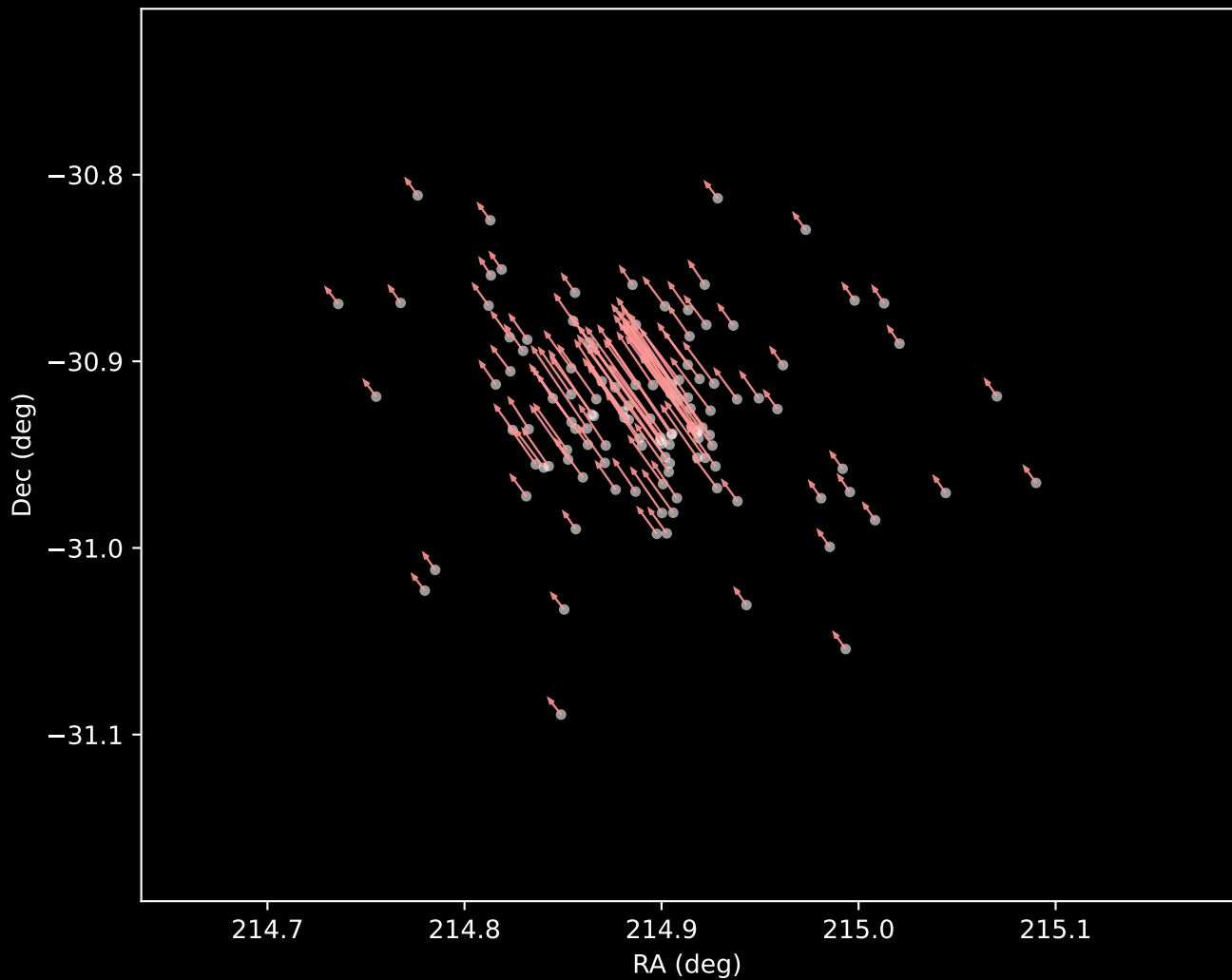
Gaia DR3 Cluster 7 Proper Motion Vectors (n=122)
