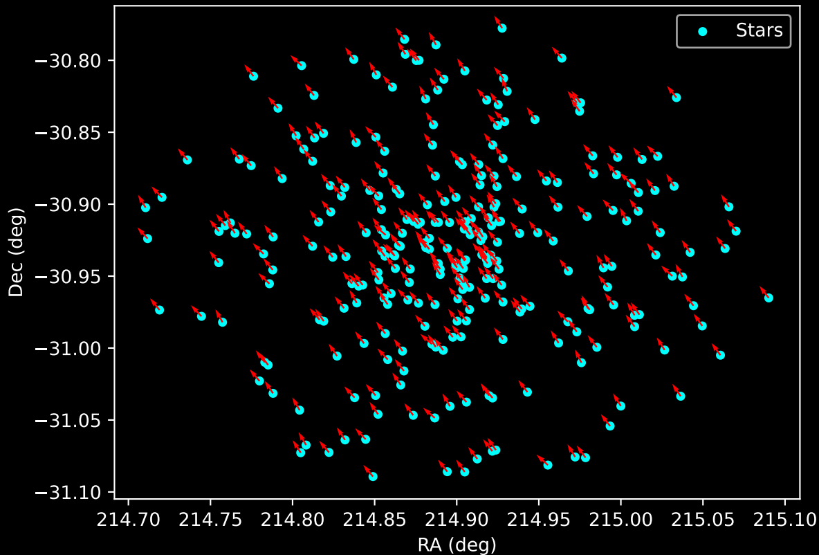
Gaia Cluster: [Ruprecht_28] Proper Motion Vectors for Gaia Star Field (n= 270)
