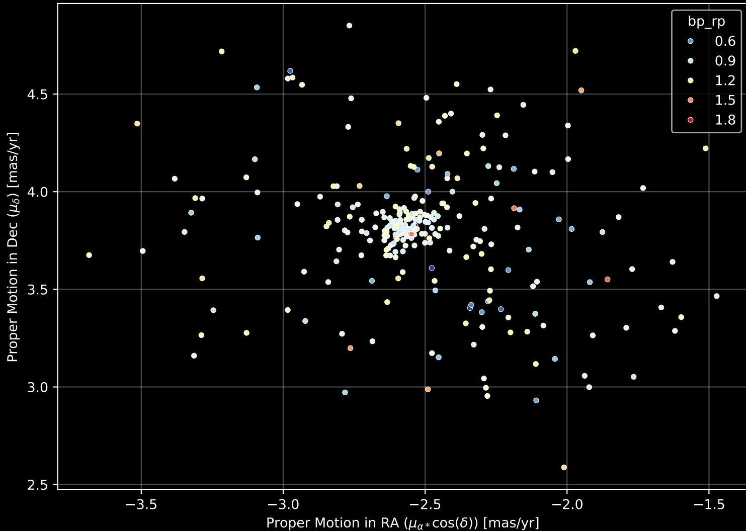
Gaia Cluster: [Ruprecht_28] Proper Motion Diagram (n= 270)
