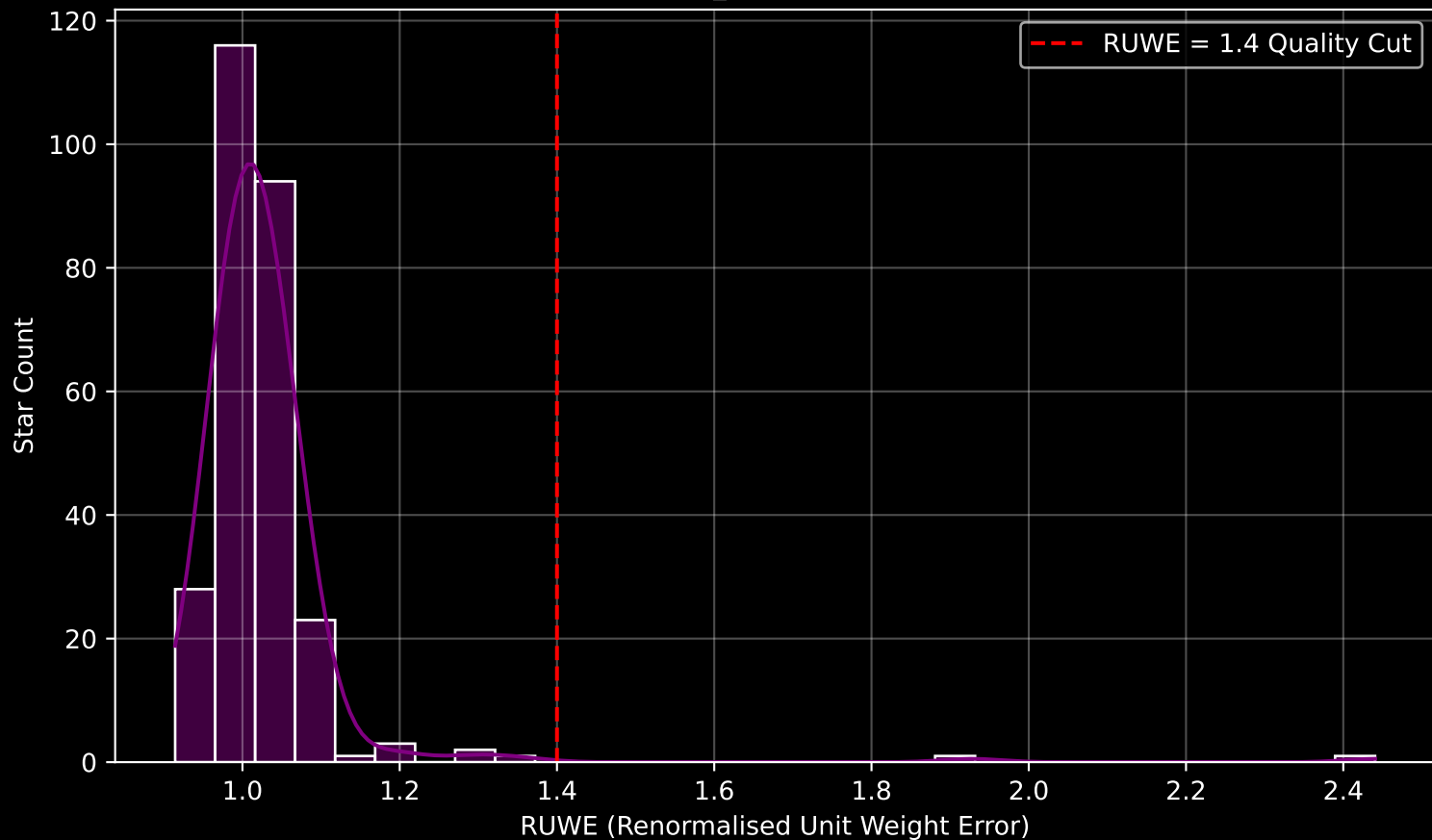
Gaia Cluster: [Ruprecht_28] RUWE Distribution (n= 270)
