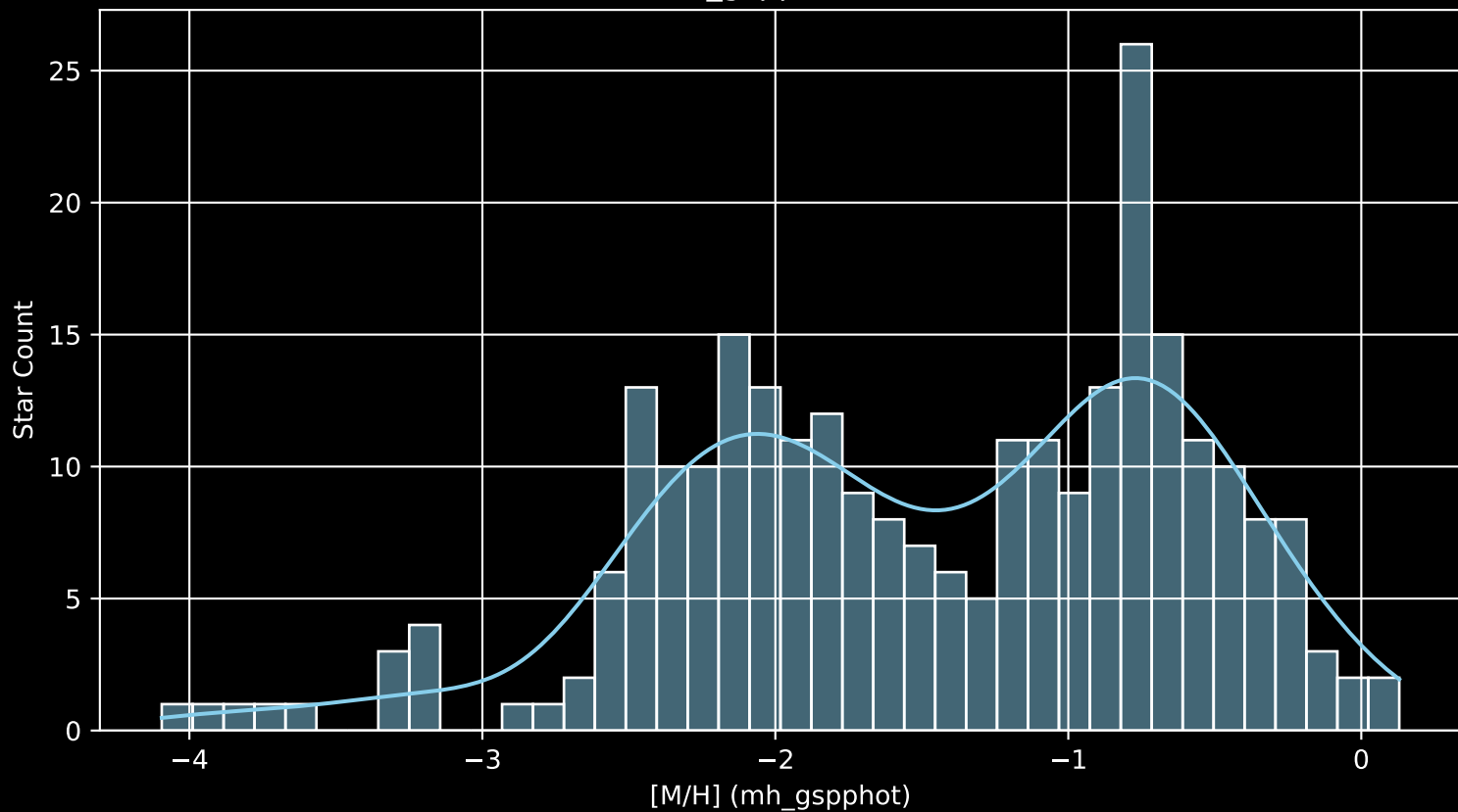
Gaia Cluster: [Ruprecht_28 [M/H] (mh_gspphot) (n= 270)
