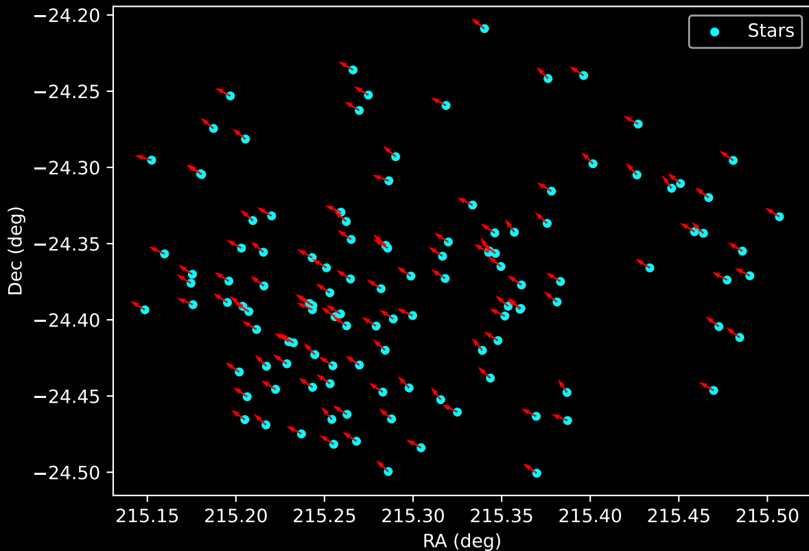
Gaia Cluster: [Ruprecht_29] Proper Motion Vectors for Gaia Star Field (n= 120)
