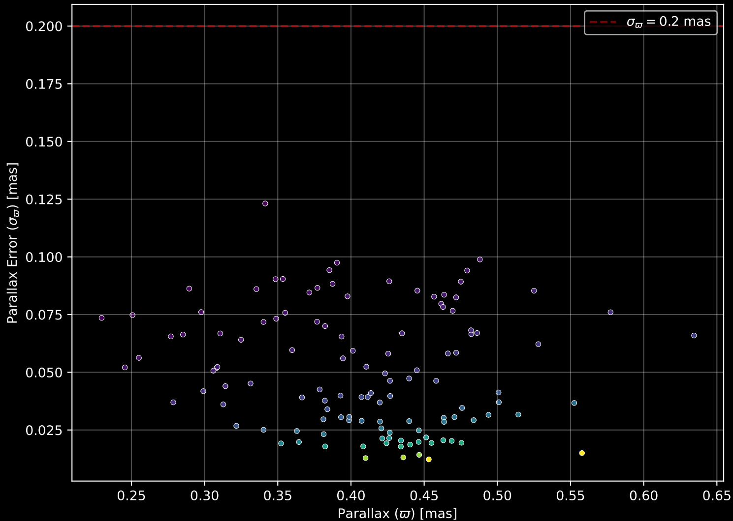
Gaia Cluster: [Ruprecht_29] Parallax Quality (n= 120)
