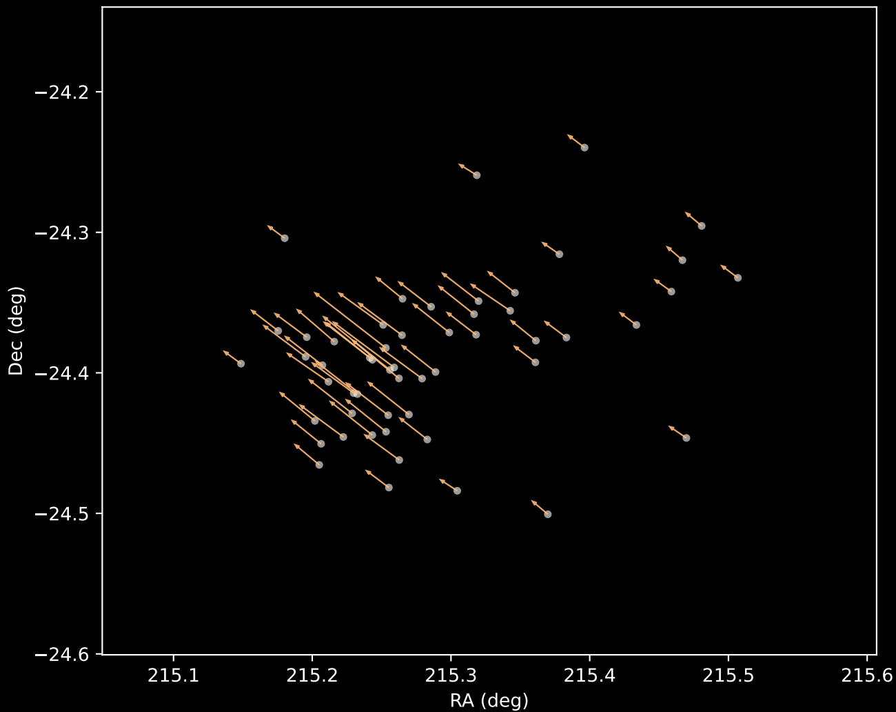
Gaia DR3 Cluster 3 Proper Motion Vectors (n=54)
