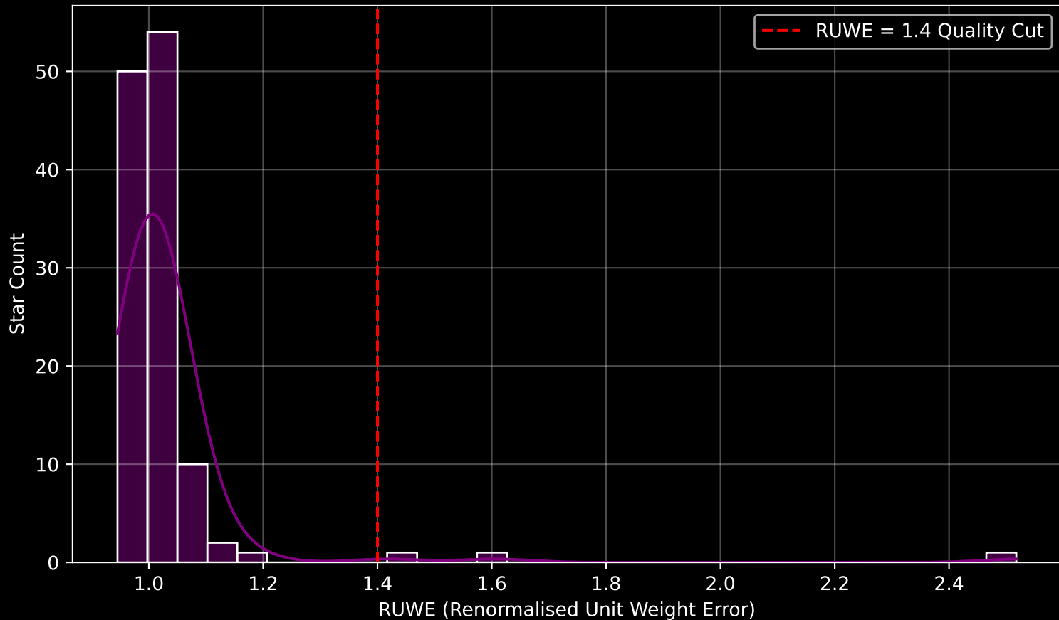
Gaia Cluster: [Ruprecht_29] RUWE Distribution (n= 120)
