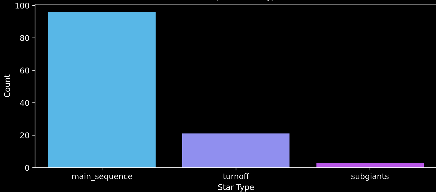
Gaia Cluster: [Ruprecht_29] Count plot of Star Type
