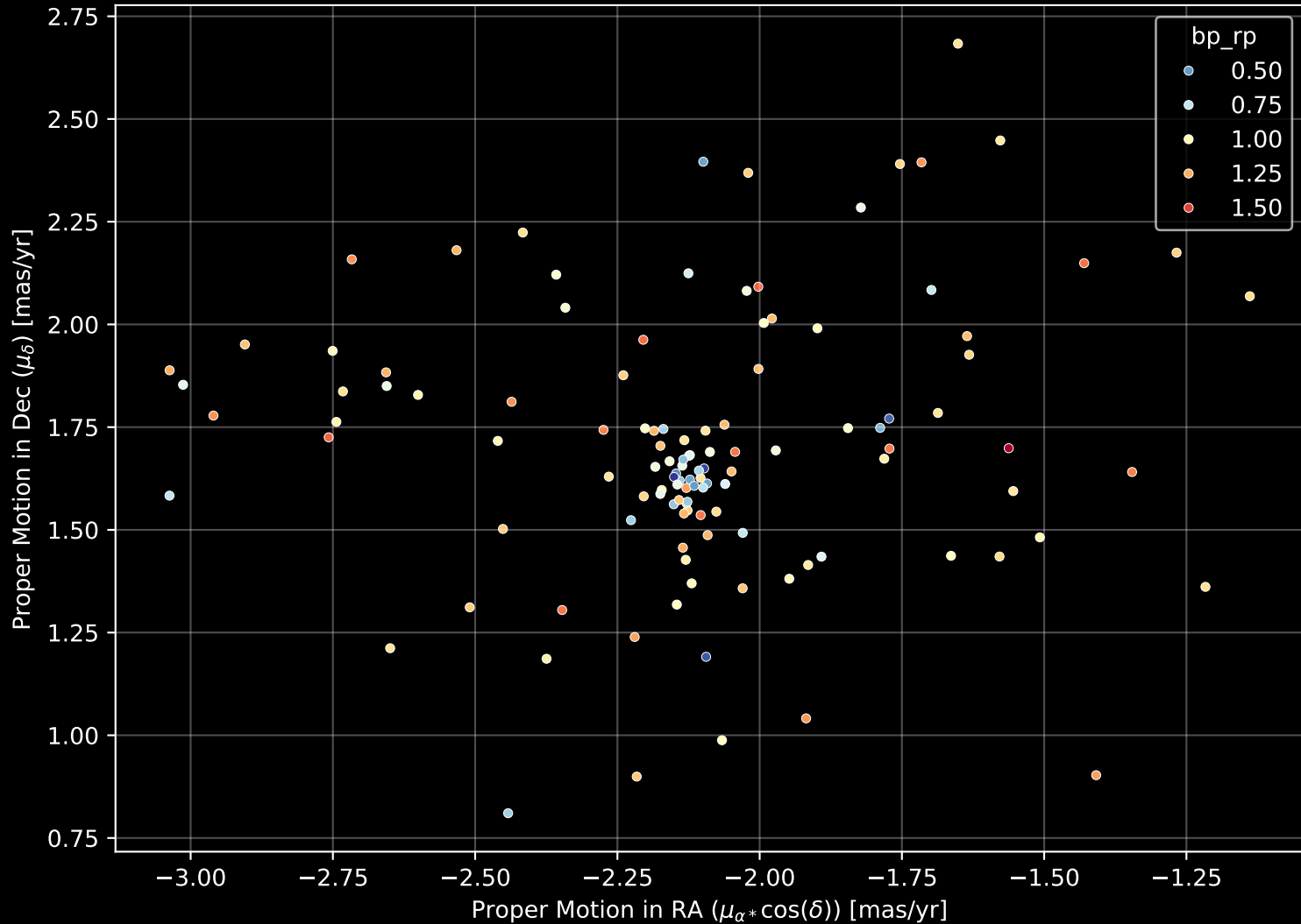
Gaia Cluster: [Ruprecht_29] Proper Motion Diagram (n= 120)
