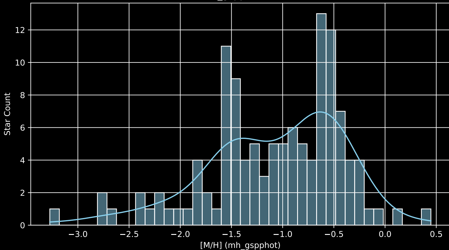
Gaia Cluster: [Ruprecht_29 [M/H] (mh_gspphot) (n= 120)
