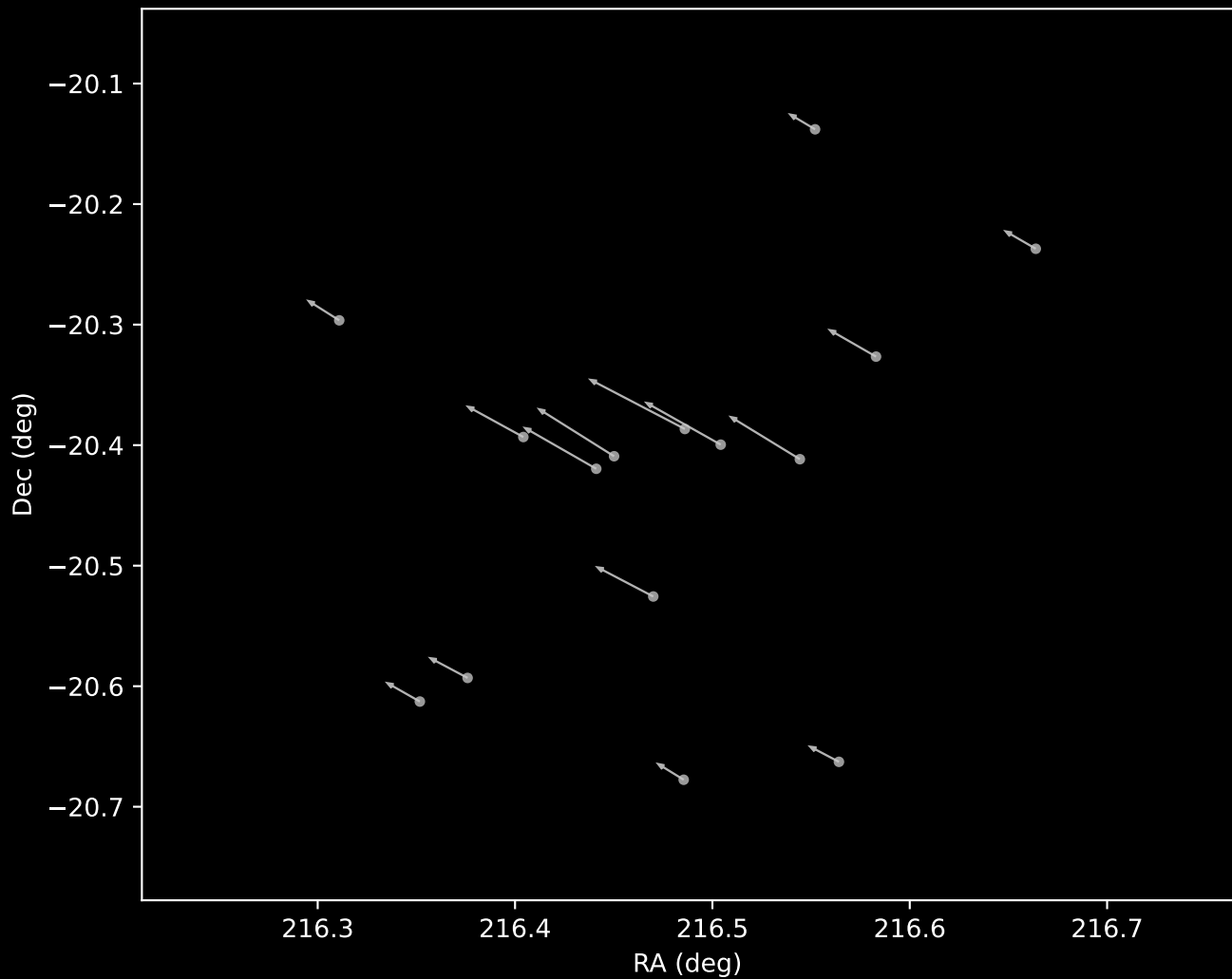
Gaia DR3 Cluster 15 Proper Motion Vectors (n=15)
