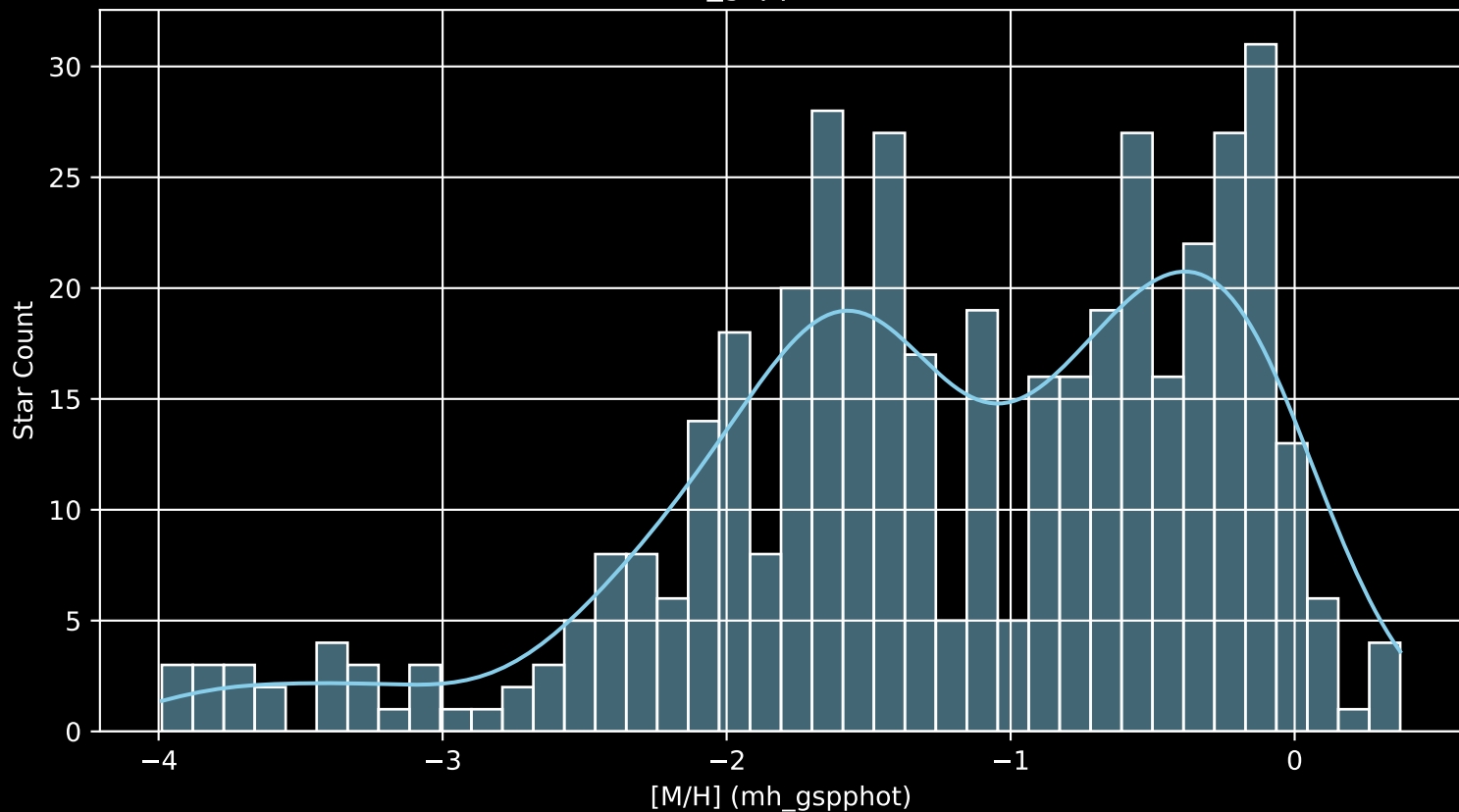
Gaia Cluster: [Ruprecht_34 [M/H] (mh_gspphot) (n= 435)
