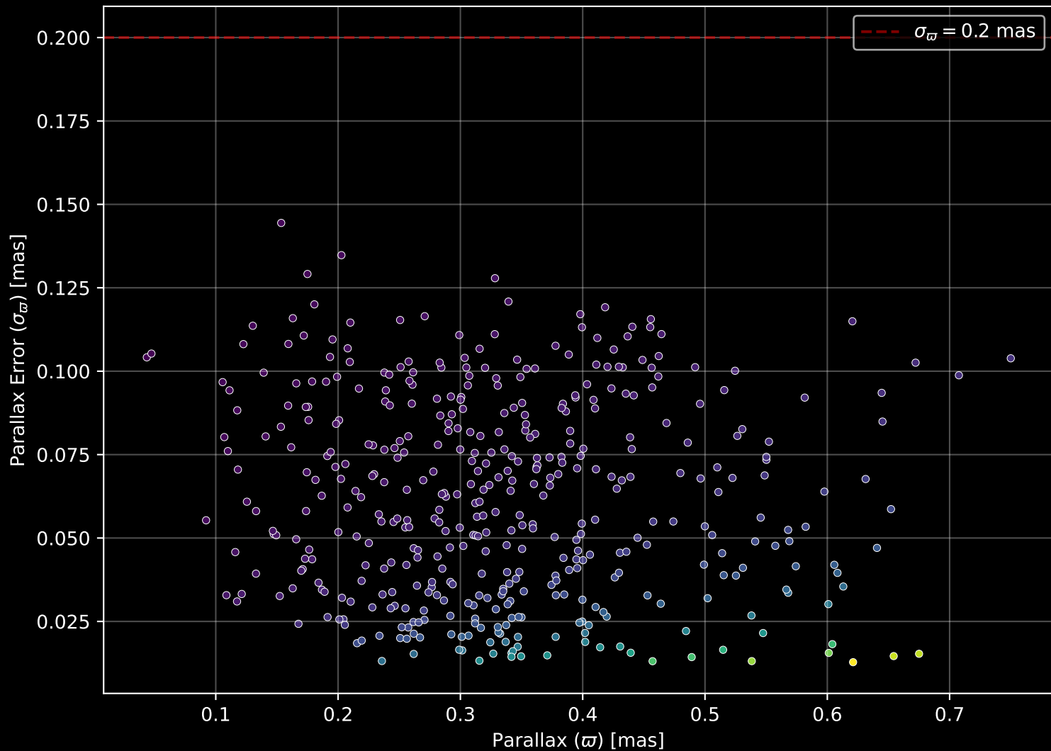
Gaia Cluster: [Ruprecht_34] Parallax Quality (n= 438)
