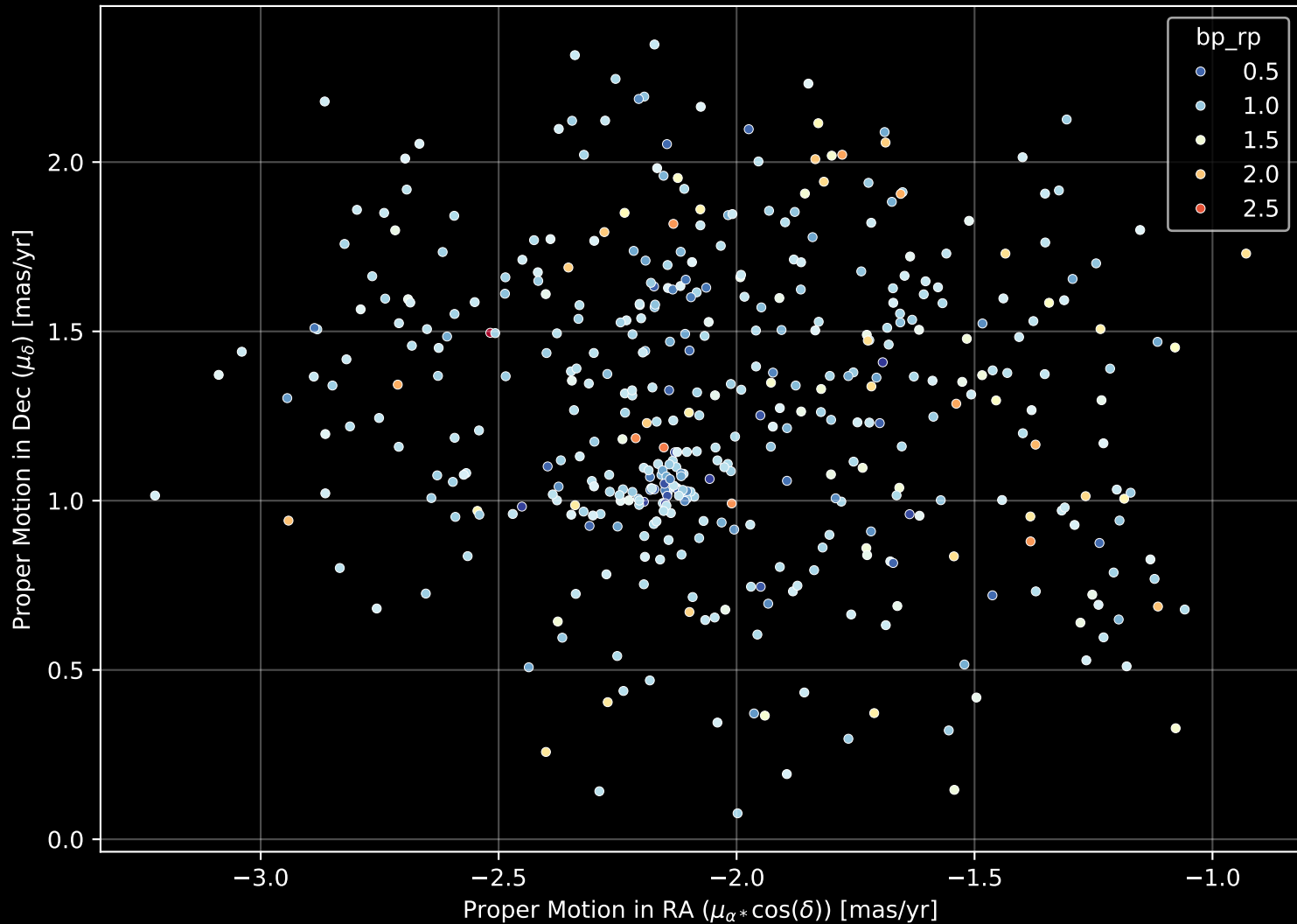
Gaia Cluster: [Ruprecht_34] Proper Motion Diagram (n= 438)
