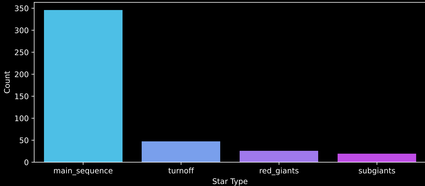
Gaia Cluster: [Ruprecht_34] Count plot of Star Type
