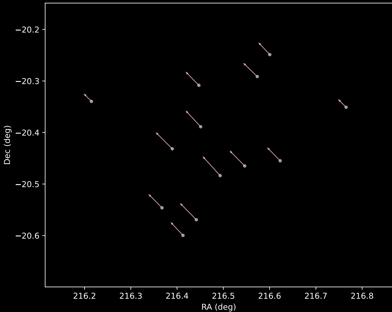
Gaia DR3 Cluster 13 Proper Motion Vectors (n=13)
