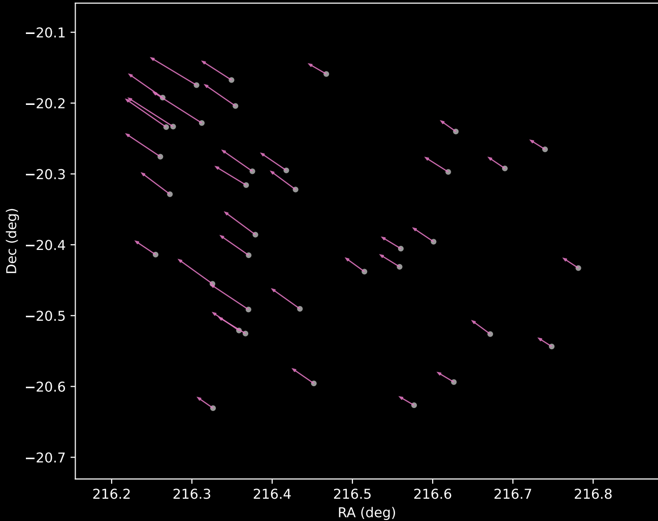
Gaia DR3 Cluster 12 Proper Motion Vectors (n=37)
