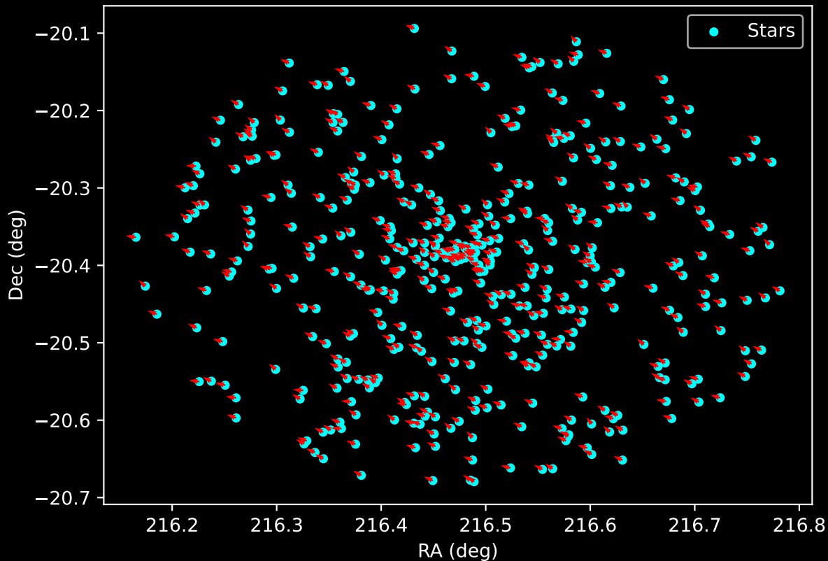
Gaia Cluster: [Ruprecht_34] Proper Motion Vectors for Gaia Star Field (n= 438)
