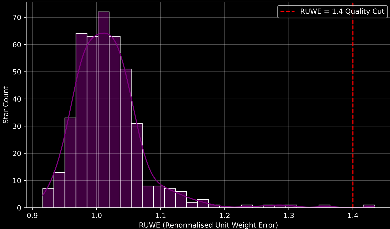
Gaia Cluster: [Ruprecht_34] RUWE Distribution (n= 438)
