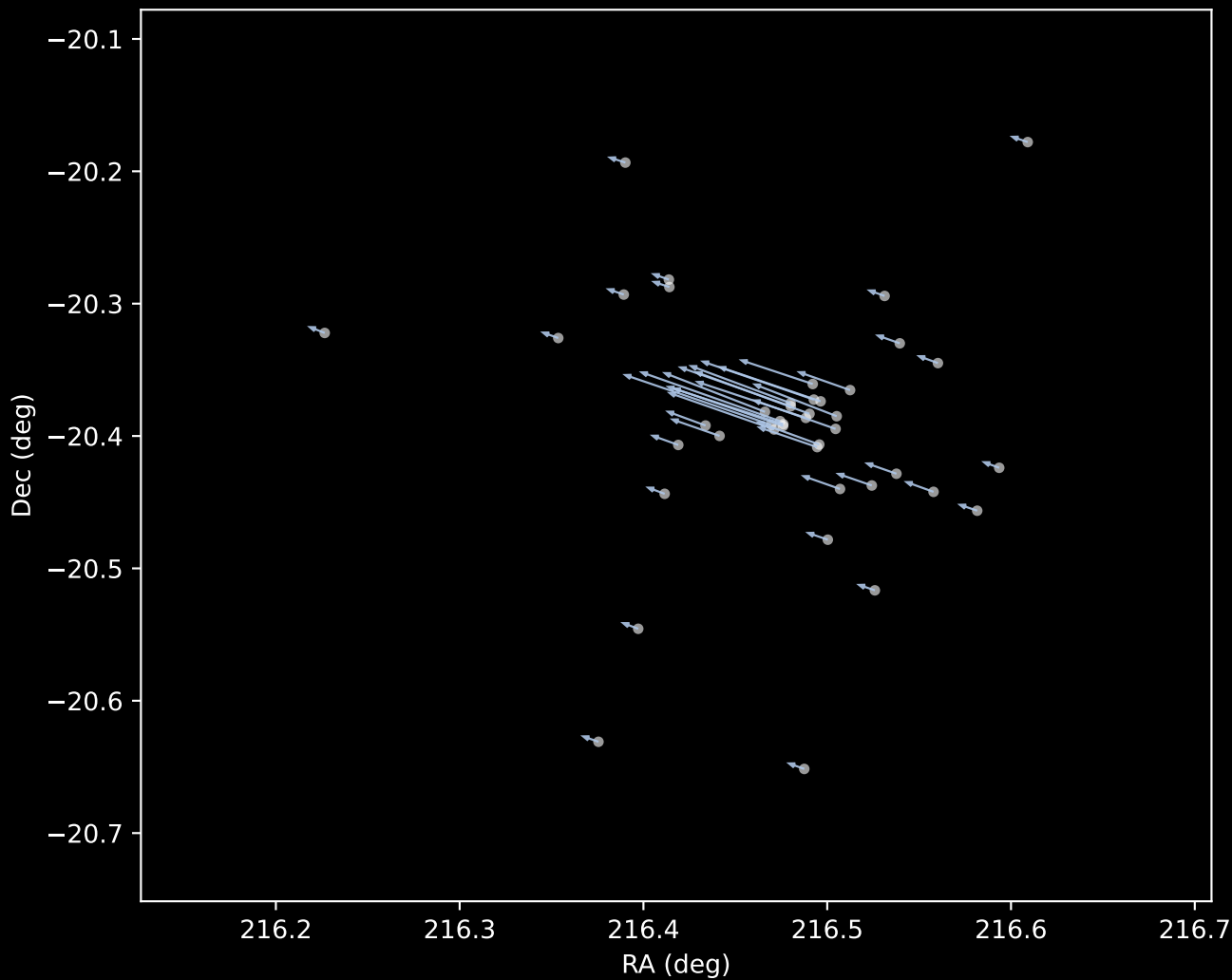
Gaia DR3 Cluster 21 Proper Motion Vectors (n=43)
