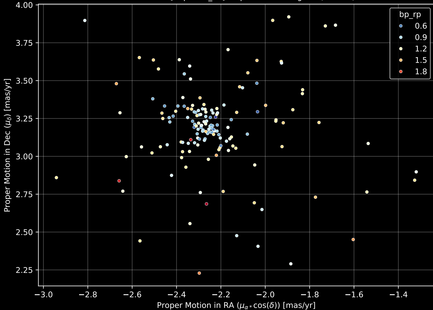
Gaia Cluster: [Ruprecht_35] Proper Motion Diagram (n= 158)
