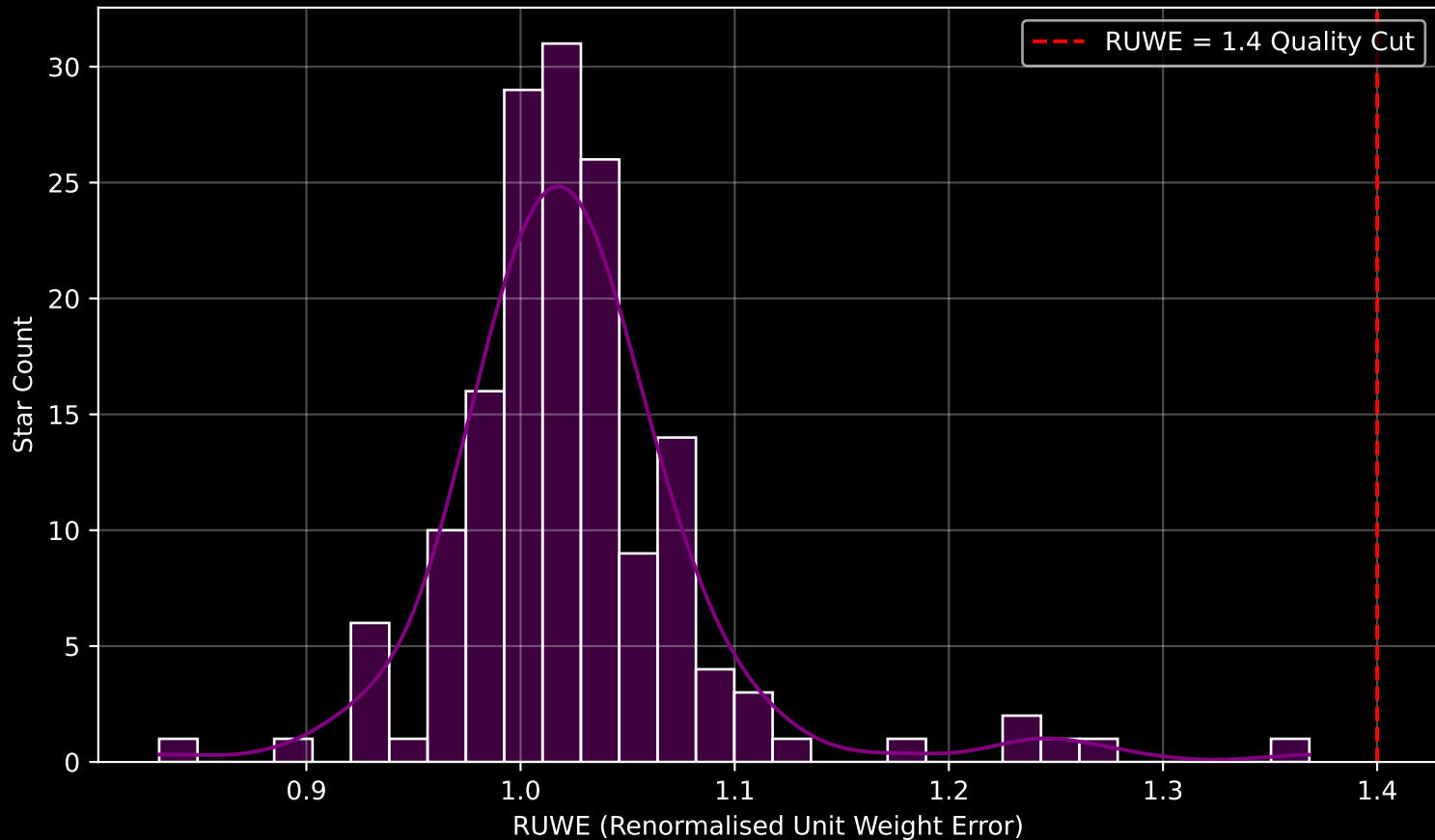
Gaia Cluster: [Ruprecht_35] RUWE Distribution (n= 158)
