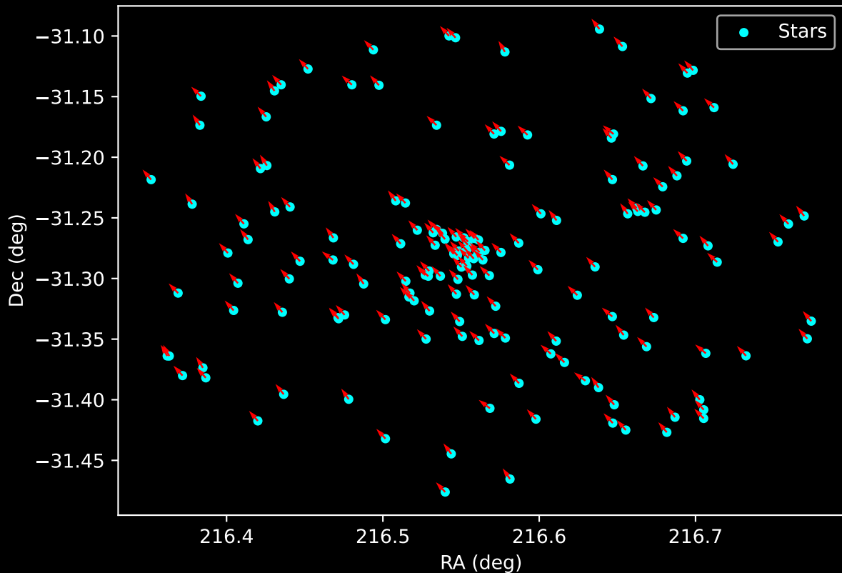
Gaia Cluster: [Ruprecht_35] Proper Motion Vectors for Gaia Star Field (n= 158)
