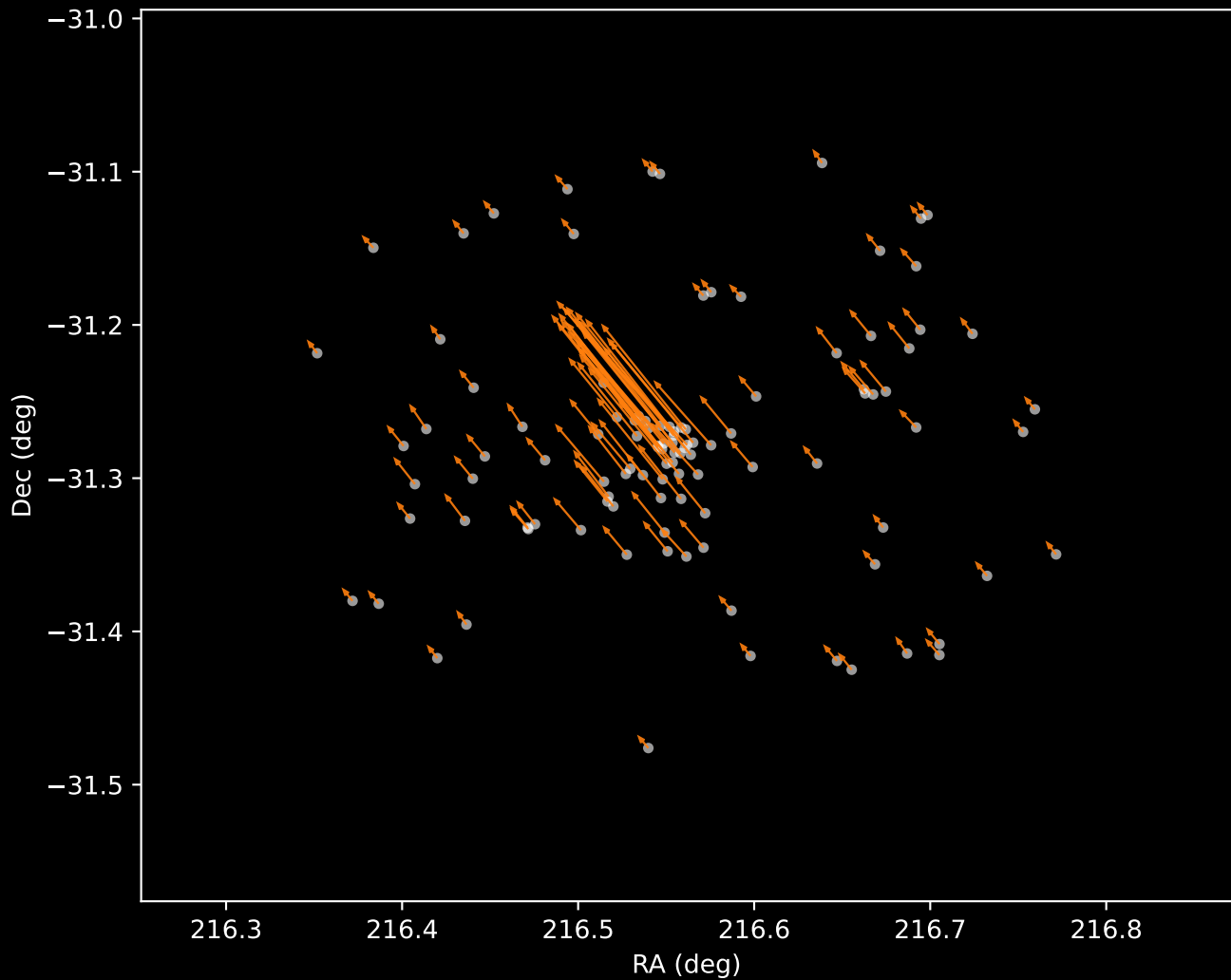
Gaia DR3 Cluster 2 Proper Motion Vectors (n=109)
