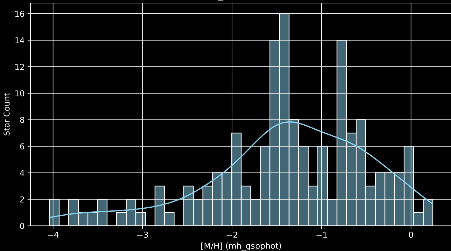
Gaia Cluster: [Ruprecht_35 [M/H] (mh_gspphot) (n= 158)
