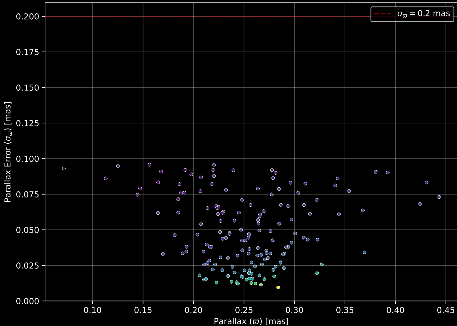
Gaia Cluster: [Ruprecht_35] Parallax Quality (n= 158)
