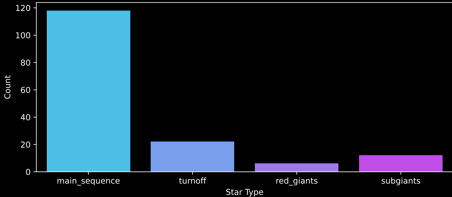
Gaia Cluster: [Ruprecht_35] Count plot of Star Type
