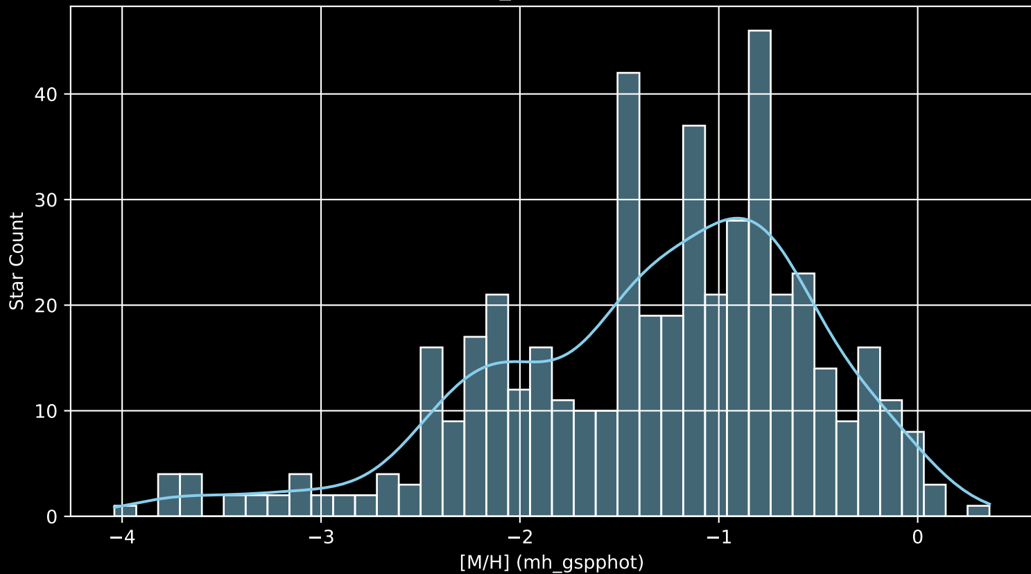
Gaia Cluster: [Ruprecht_41 [M/H] (mh_gspphot) (n= 472)
