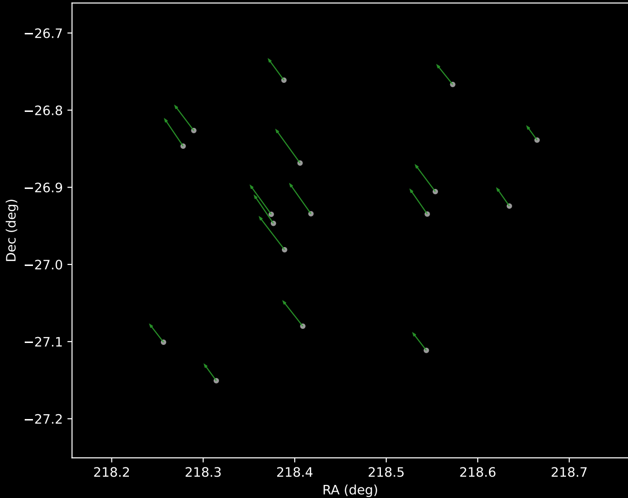
Gaia DR3 Cluster 4 Proper Motion Vectors (n=17)
