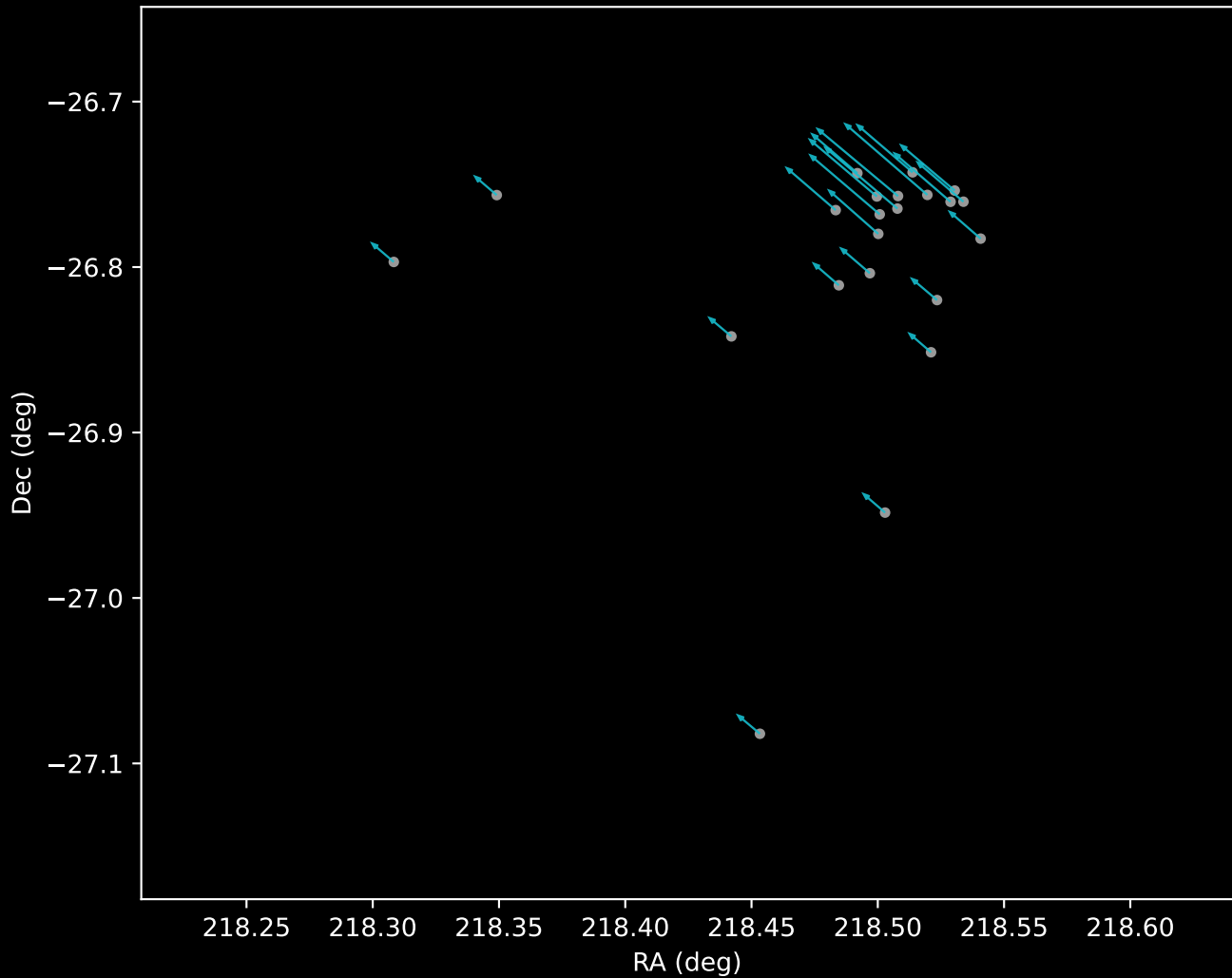
Gaia DR3 Cluster 18 Proper Motion Vectors (n=22)
