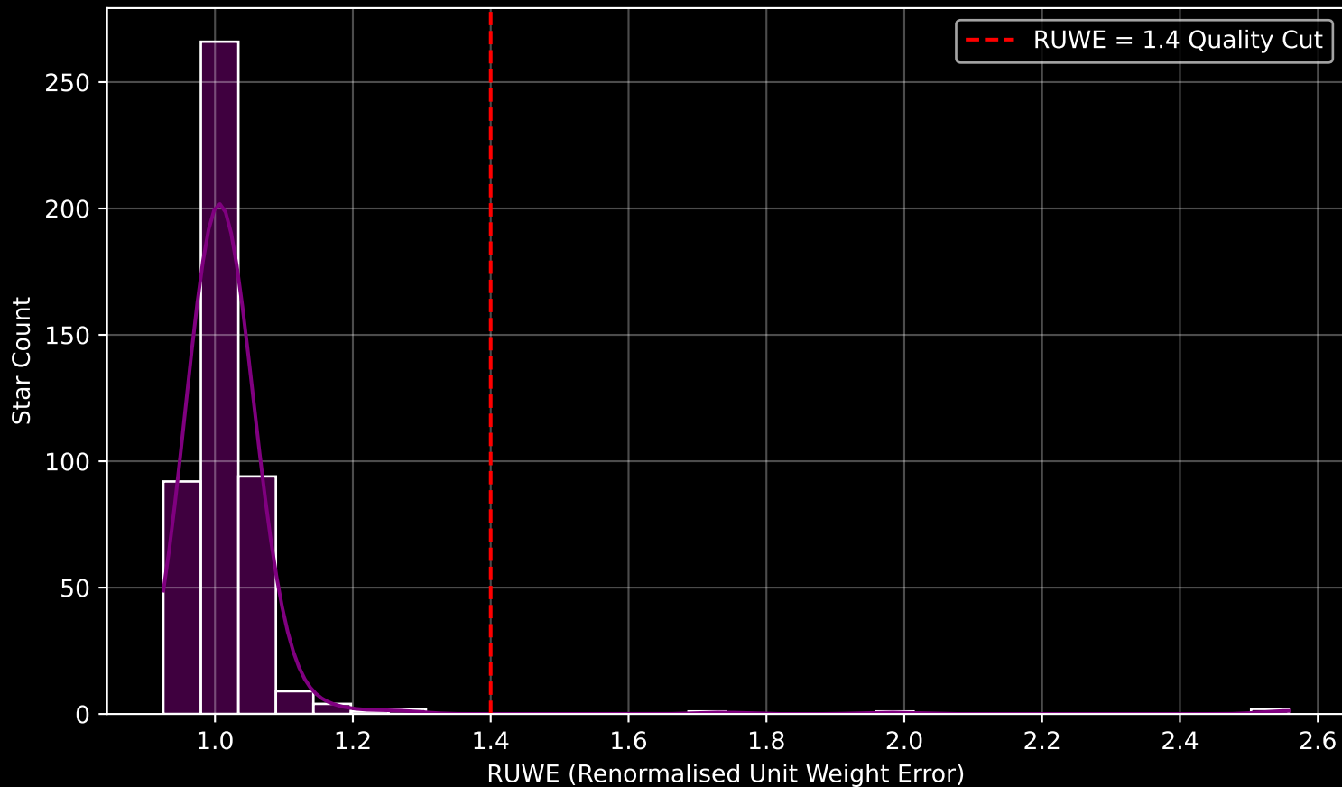
Gaia Cluster: [Ruprecht_41] RUWE Distribution (n= 472)
