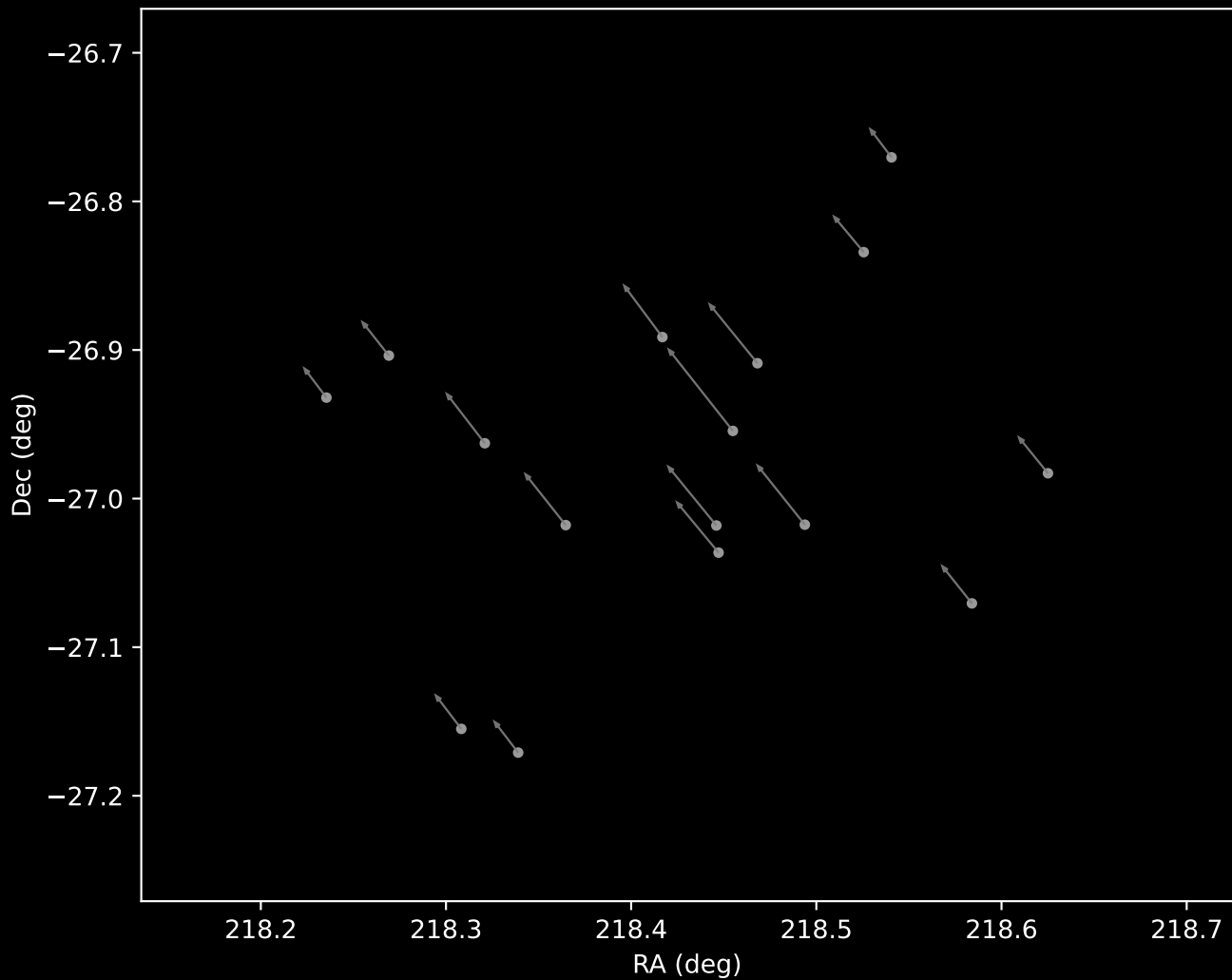
Gaia DR3 Cluster 14 Proper Motion Vectors (n=16)
