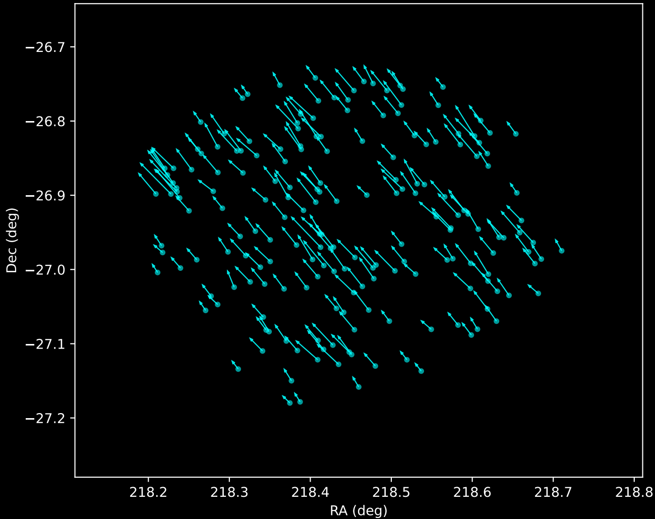
Gaia DR3 Noise Stream Proper Motion Vectors (n=188)
