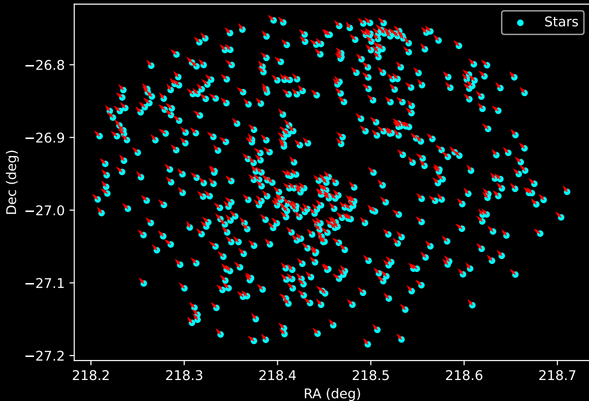
Gaia Cluster: [Ruprecht_41] Proper Motion Vectors for Gaia Star Field (n= 472)
