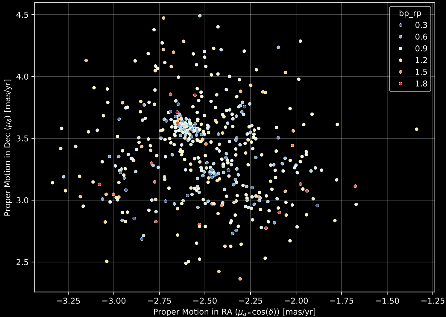
Gaia Cluster: [Ruprecht_41] Proper Motion Diagram (n= 472)
