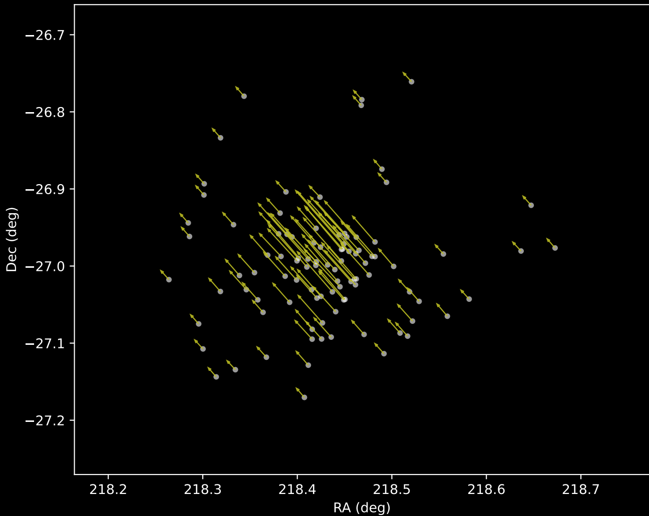
Gaia DR3 Cluster 16 Proper Motion Vectors (n=96)
