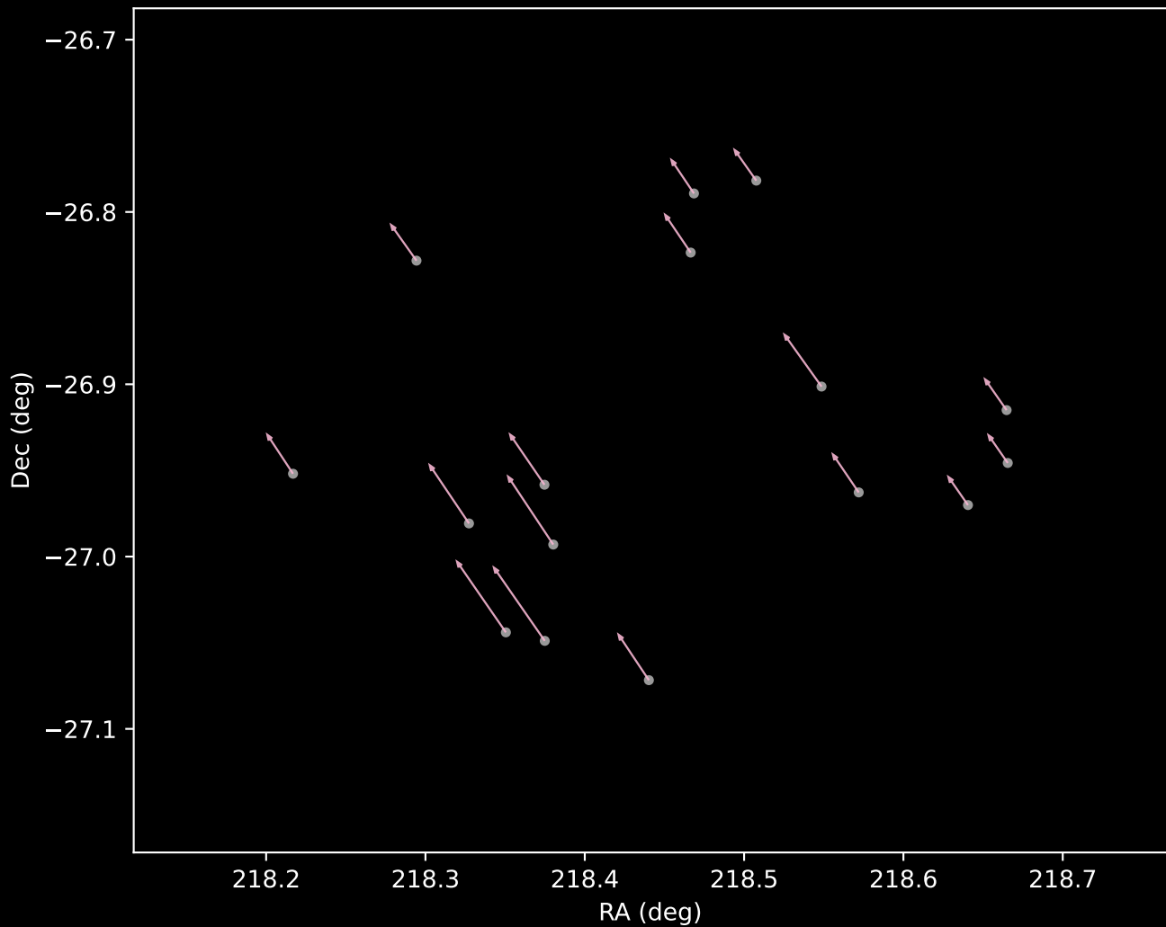
Gaia DR3 Cluster 13 Proper Motion Vectors (n=16)
