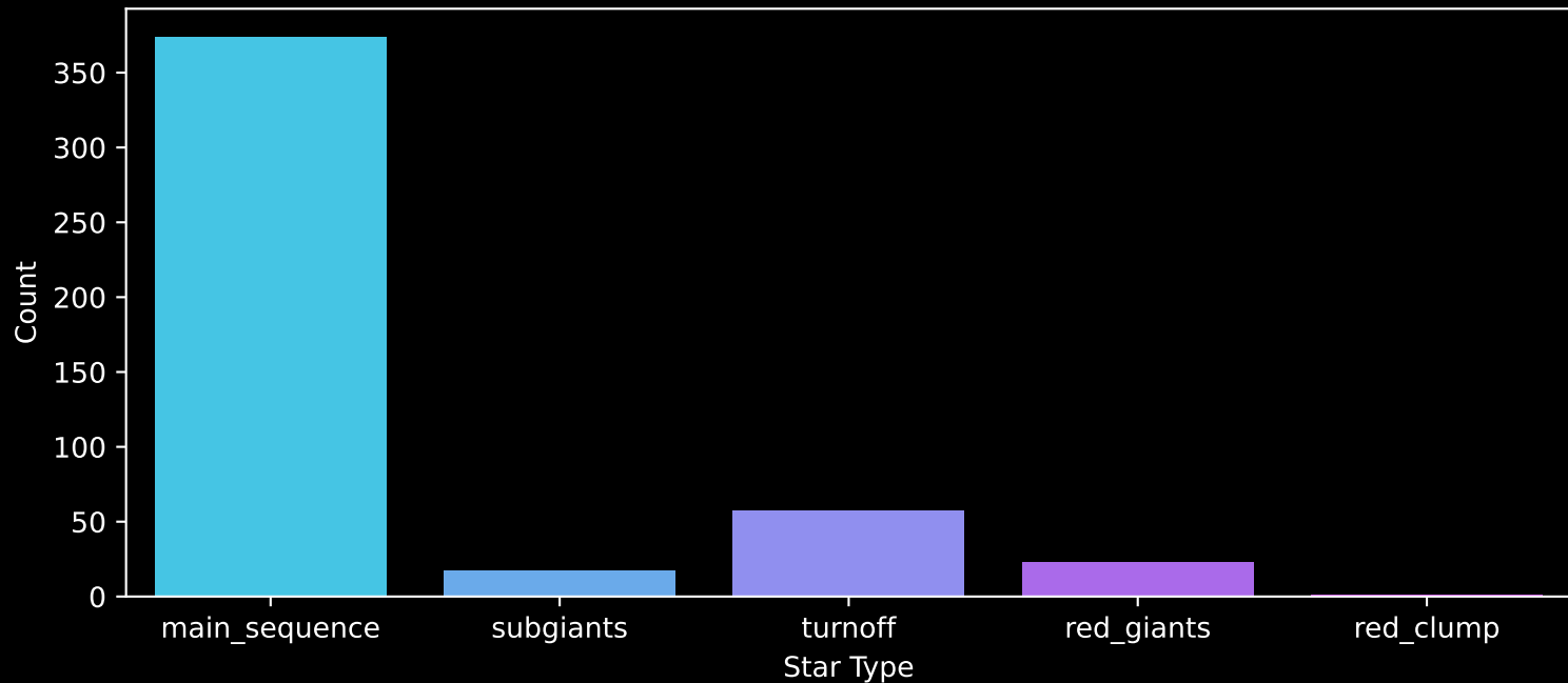
Gaia Cluster: [Ruprecht_41] Count plot of Star Type
