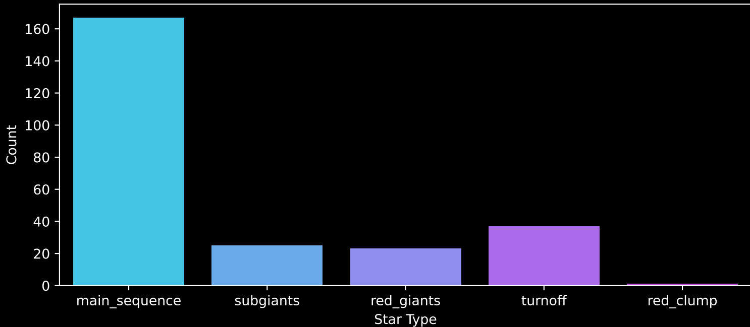
Gaia Cluster: [Ruprecht_43] Count plot of Star Type
