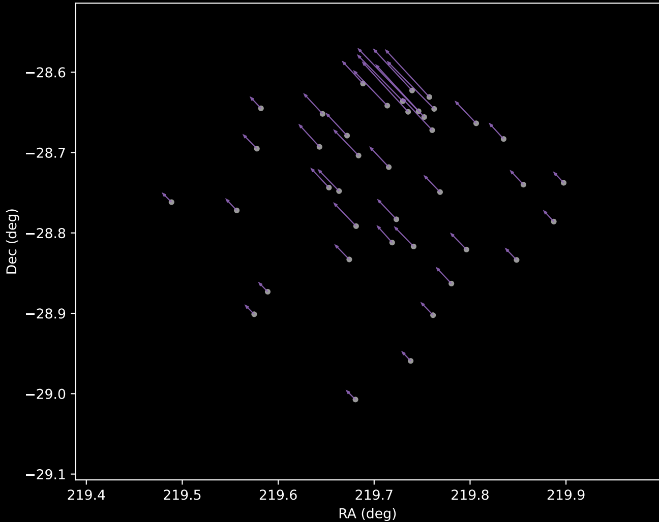
Gaia DR3 Cluster 8 Proper Motion Vectors (n=40)
