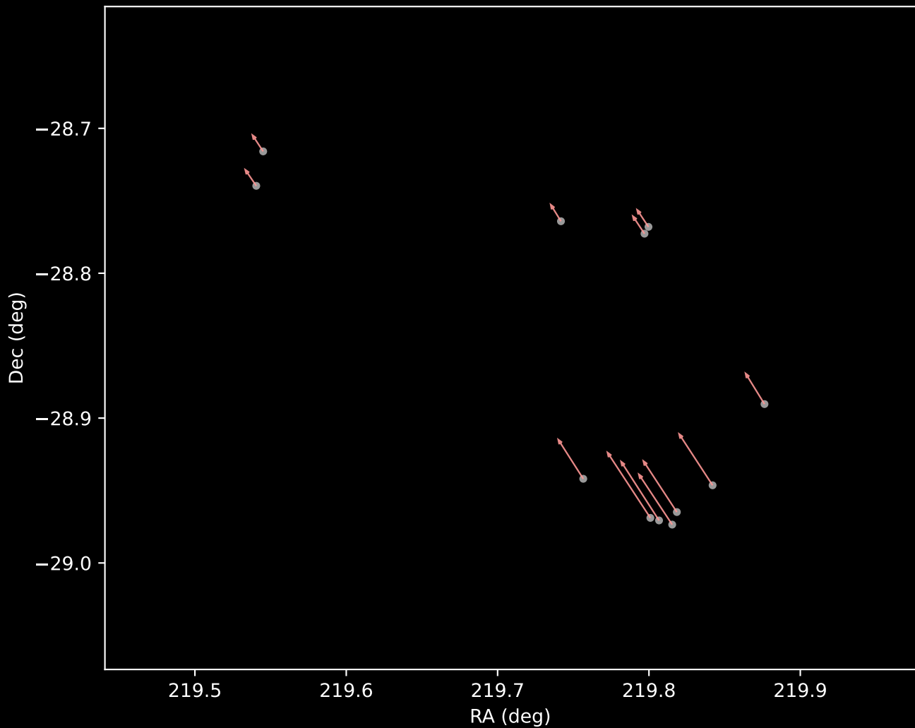
Gaia DR3 Cluster 7 Proper Motion Vectors (n=12)
