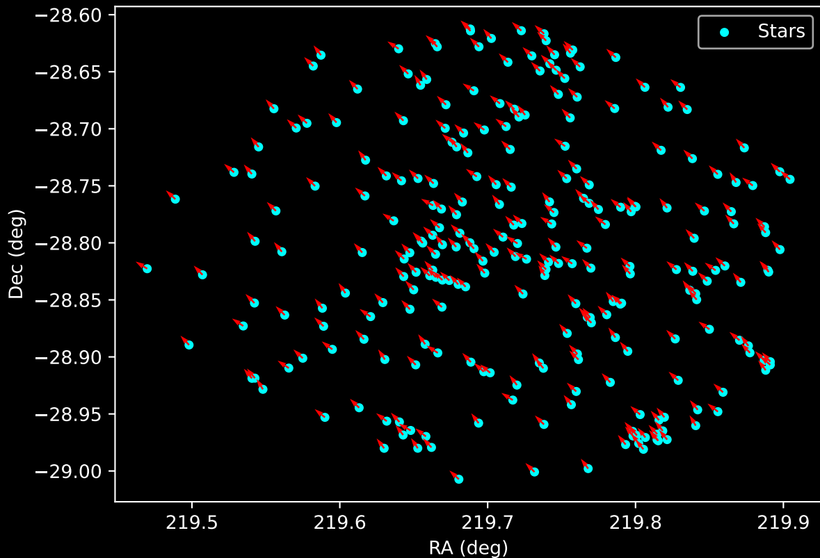
Gaia Cluster: [Ruprecht_43] Proper Motion Vectors for Gaia Star Field (n= 253)
