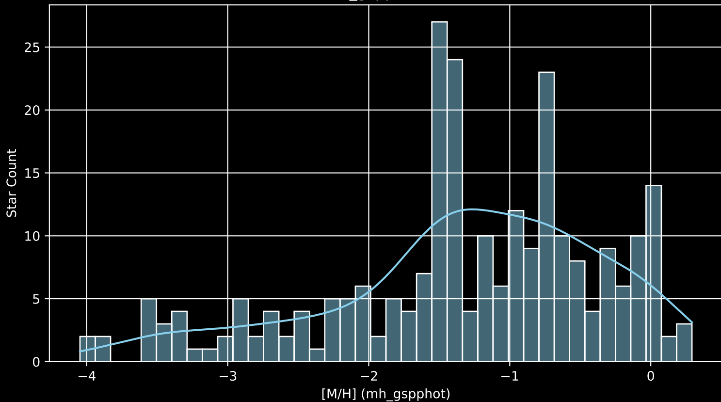
Gaia Cluster: [Ruprecht_43 [M/H] (mh_gspphot) (n= 253)
