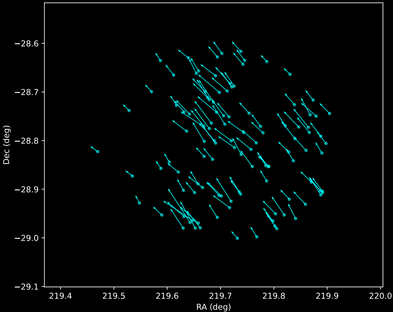
Gaia DR3 Noise Stream Proper Motion Vectors (n=111)
