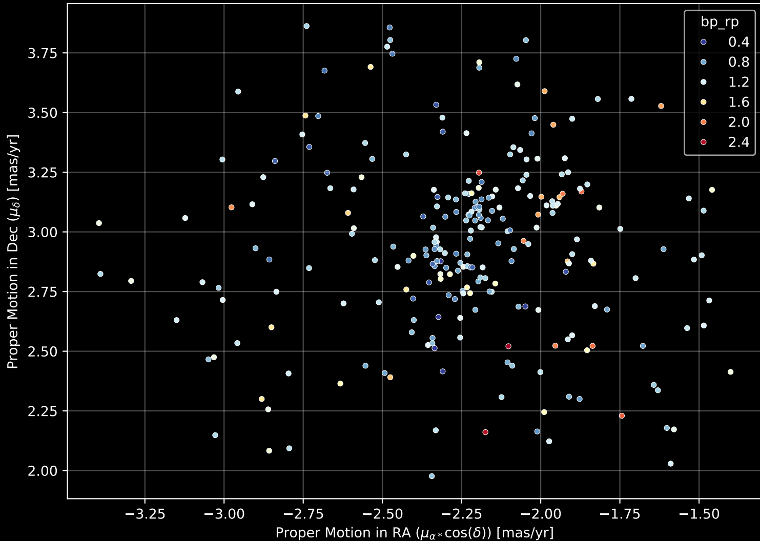
Gaia Cluster: [Ruprecht_43] Proper Motion Diagram (n= 253)
