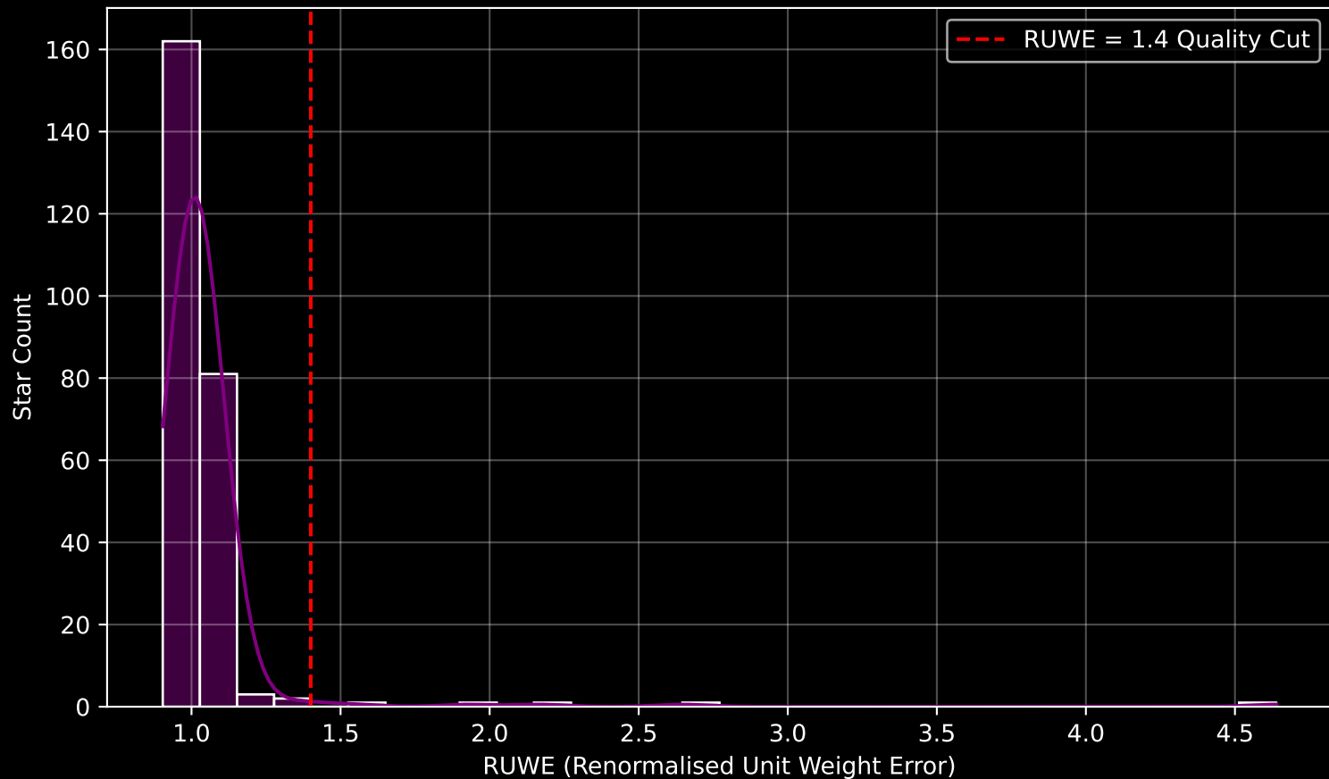
Gaia Cluster: [Ruprecht_43] RUWE Distribution (n= 253)
