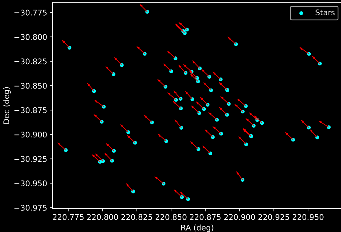
Gaia Cluster: [Ruprecht_50] Proper Motion Vectors for Gaia Star Field (n= 68)
