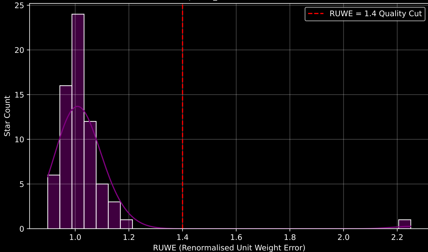
Gaia Cluster: [Ruprecht_50] RUWE Distribution (n= 68)
