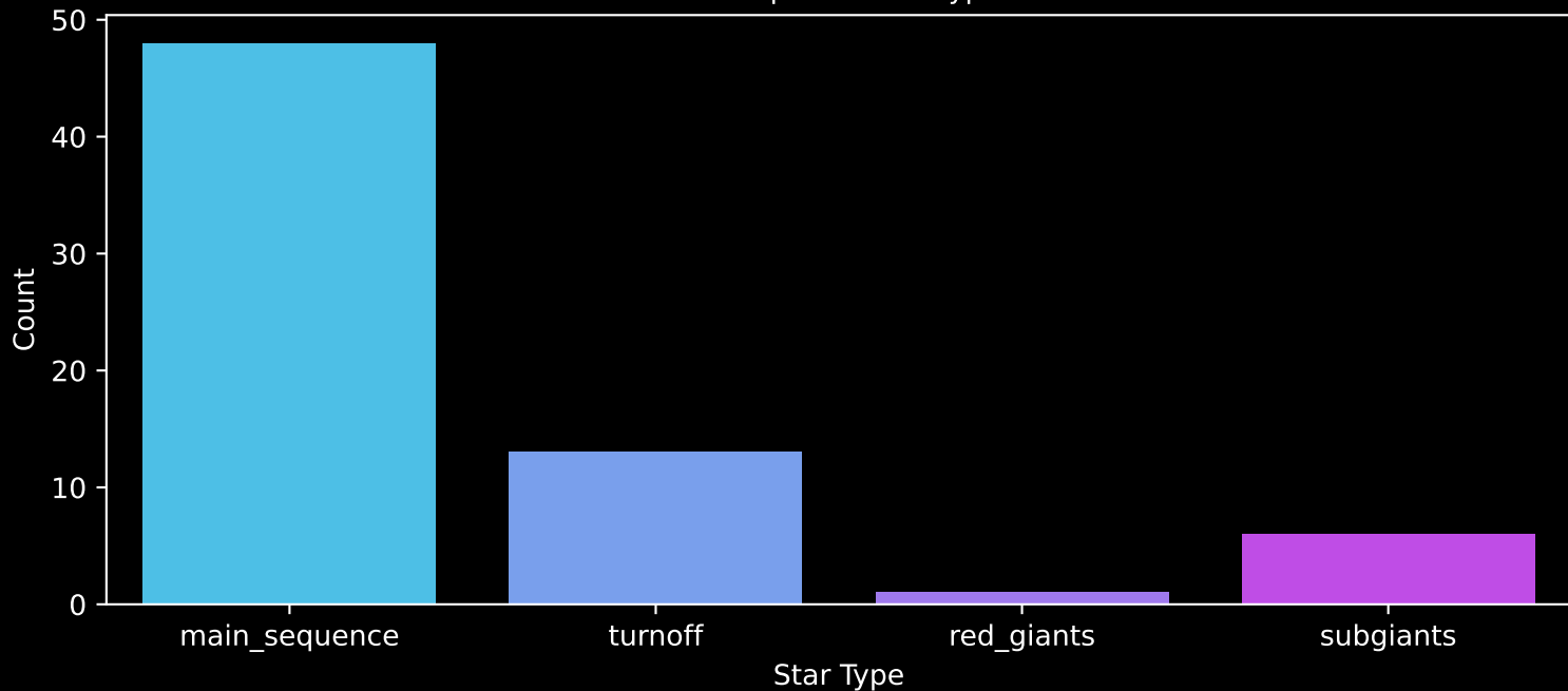
Gaia Cluster: [Ruprecht_50] Count plot of Star Type
