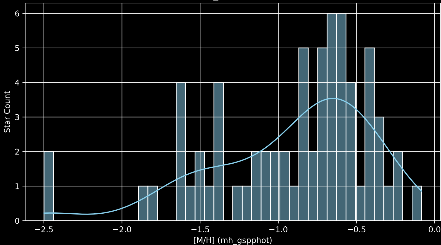
Gaia Cluster: [Ruprecht_50 [M/H] (mh_gspphot) (n= 68)
