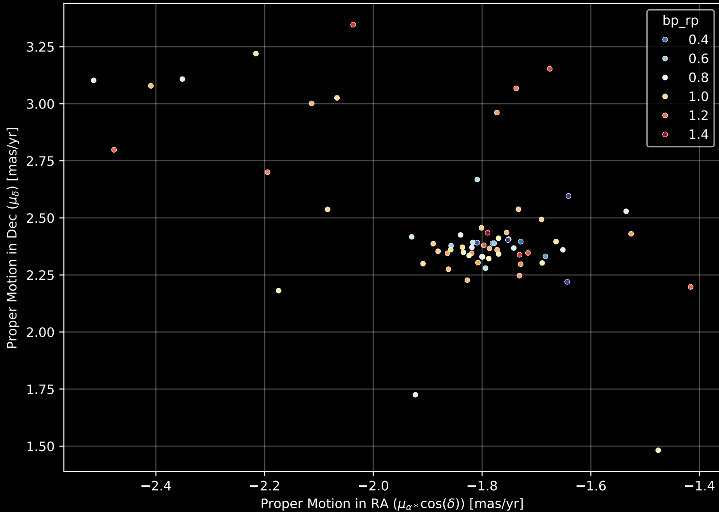
Gaia Cluster: [Ruprecht_50] Proper Motion Diagram (n= 68)
