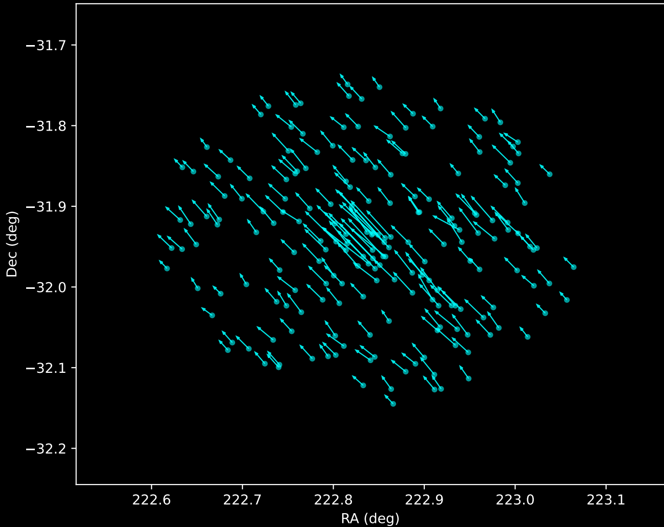
Gaia DR3 Noise Stream Proper Motion Vectors (n=194)
