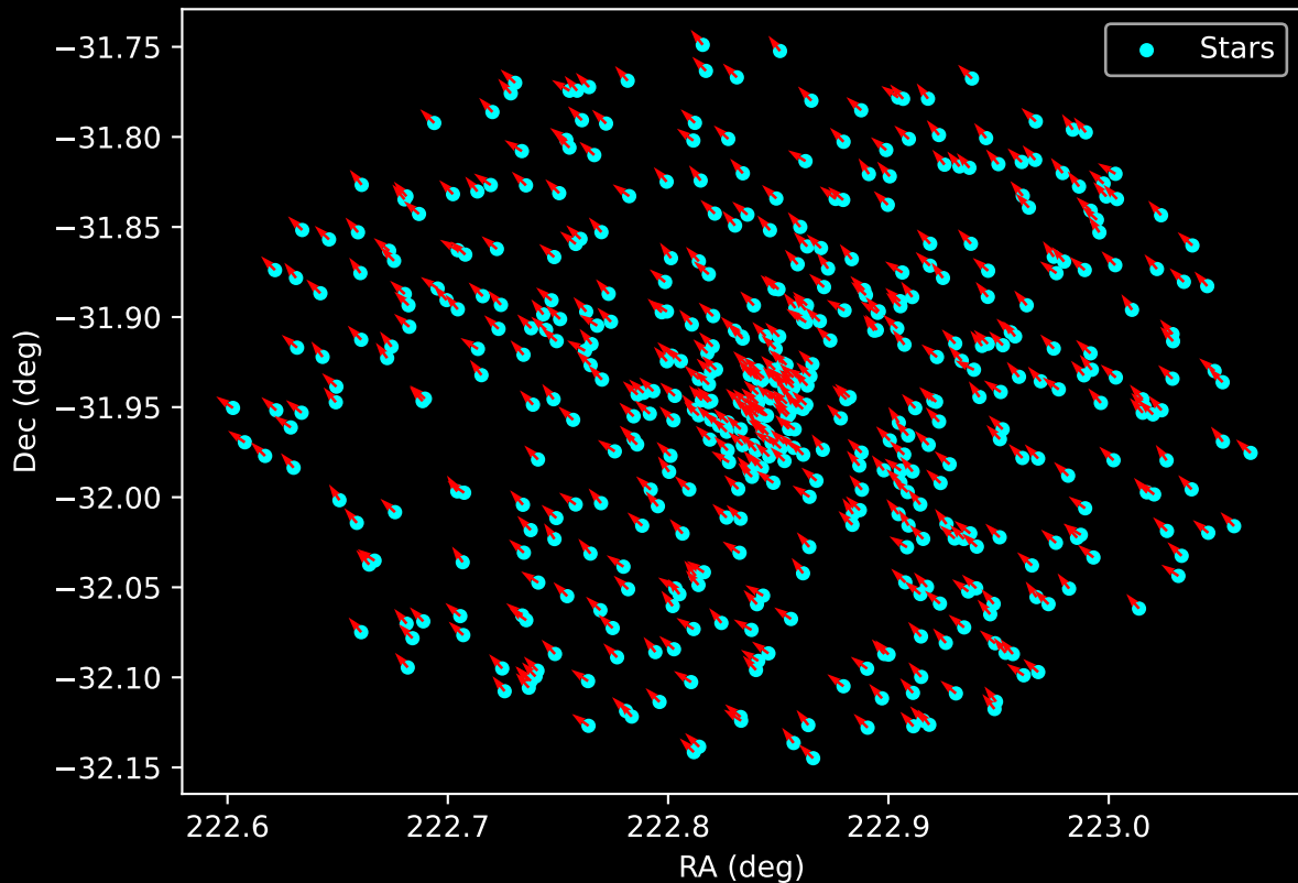
Gaia Cluster: [Ruprecht_54] Proper Motion Vectors for Gaia Star Field (n= 505)
