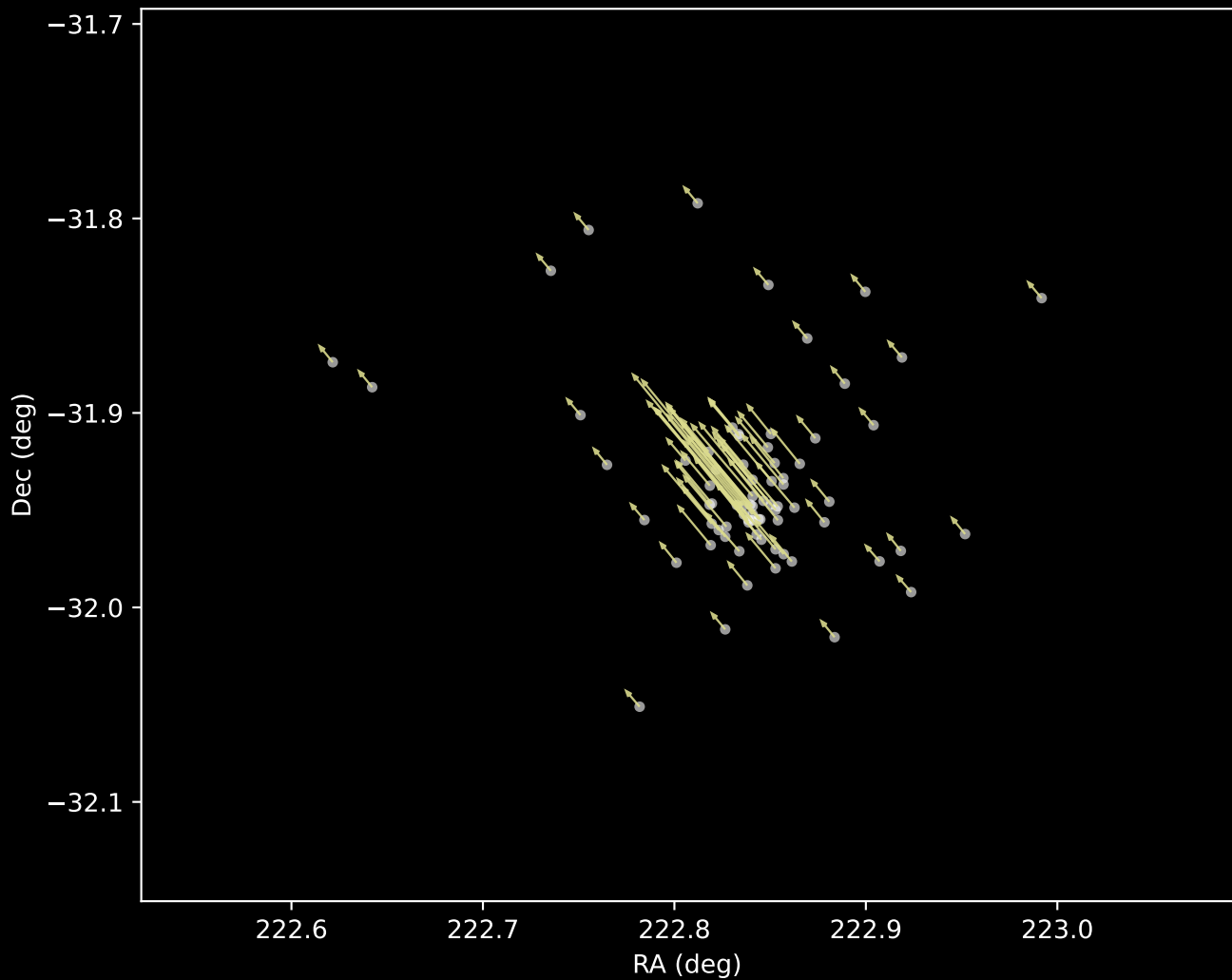
Gaia DR3 Cluster 17 Proper Motion Vectors (n=75)
