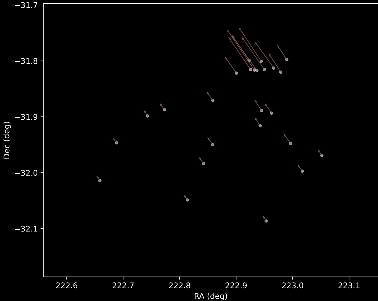
Gaia DR3 Cluster 10 Proper Motion Vectors (n=25)
