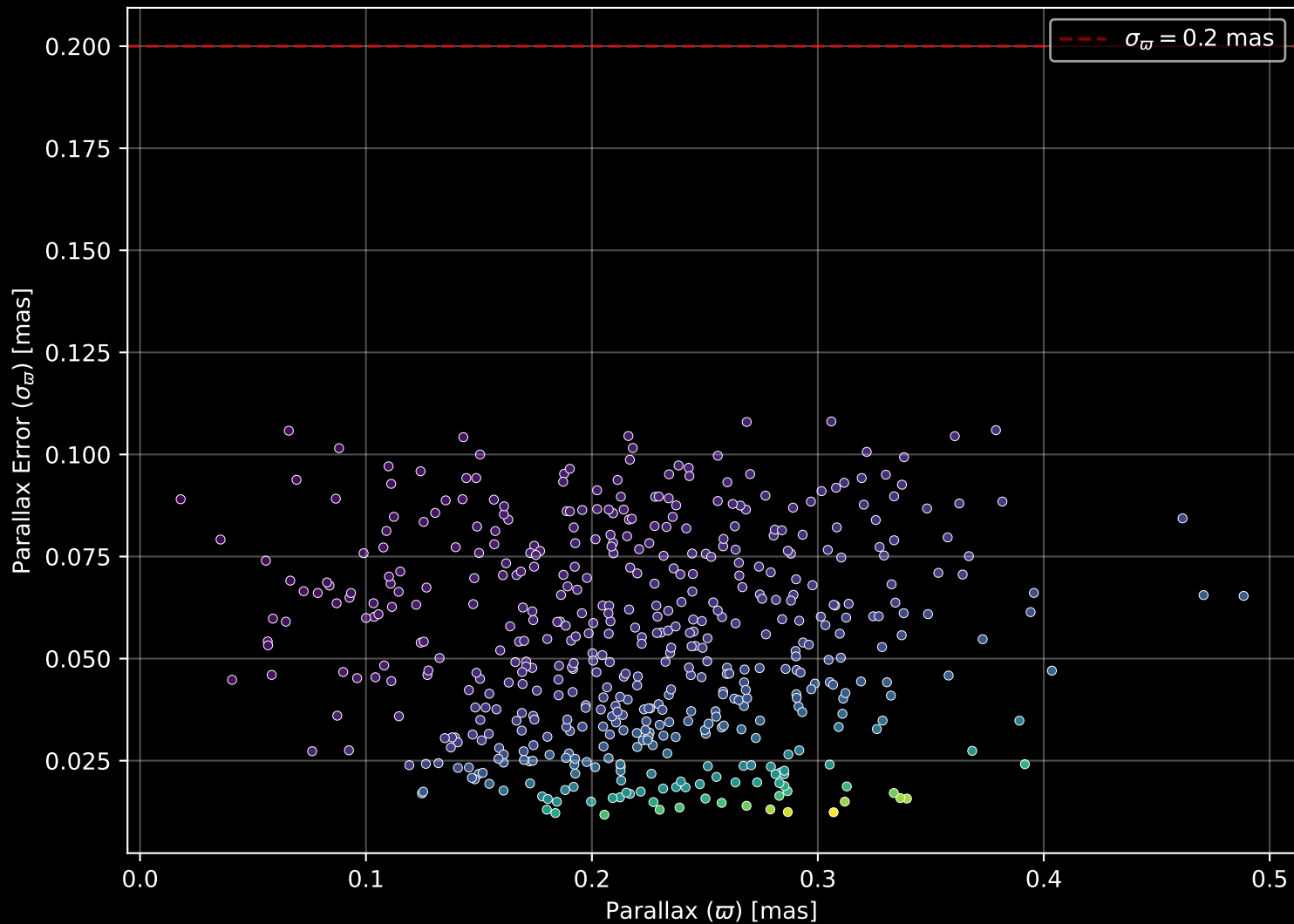
Gaia Cluster: [Ruprecht_54] Parallax Quality (n= 505)
