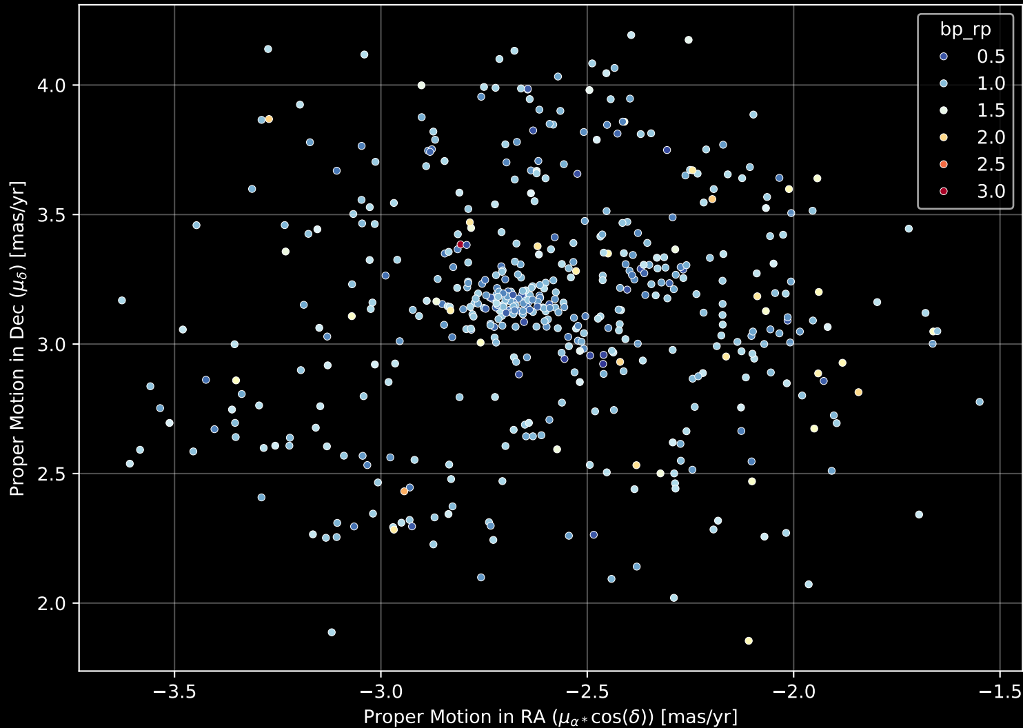
Gaia Cluster: [Ruprecht_54] Proper Motion Diagram (n= 505)
