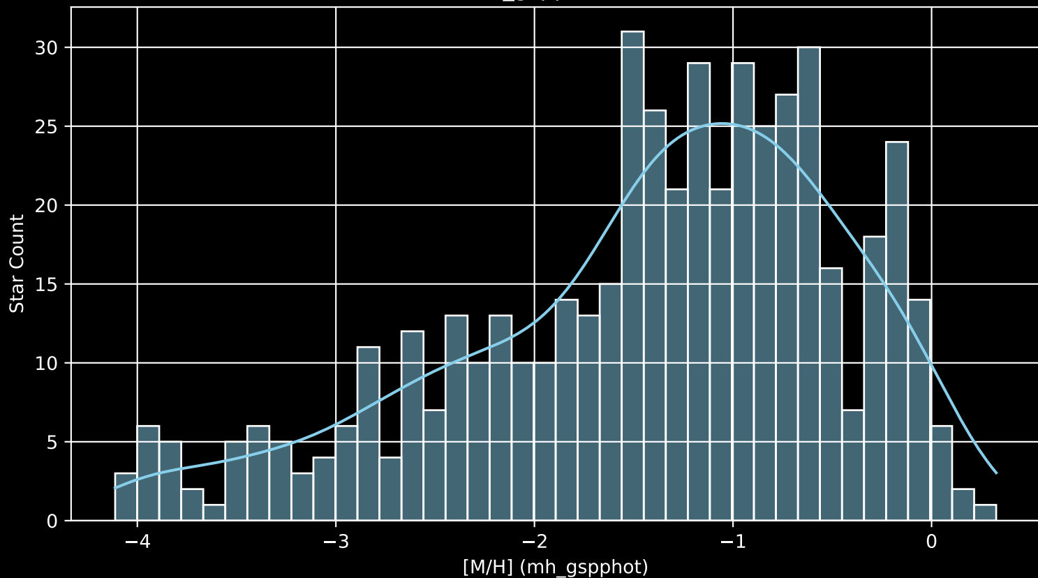
Gaia Cluster: [Ruprecht_54 [M/H] (mh_gspphot) (n= 505)
