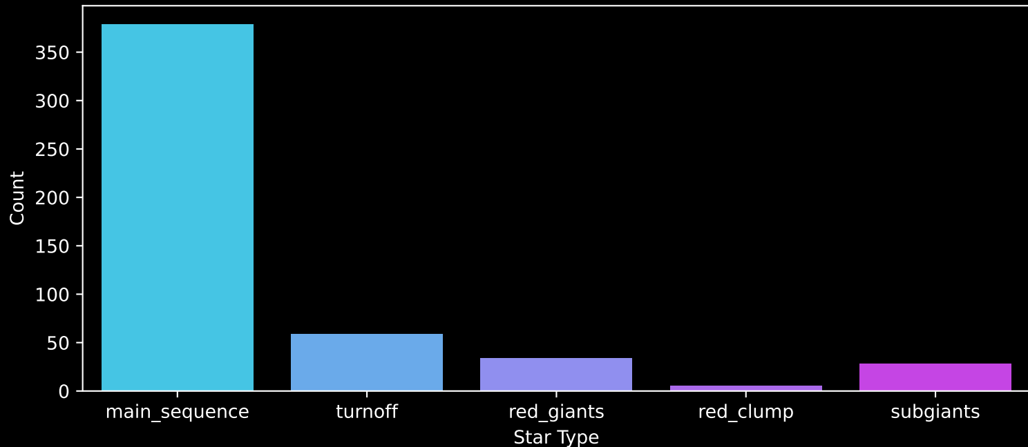
Gaia Cluster: [Ruprecht_54] Count plot of Star Type
