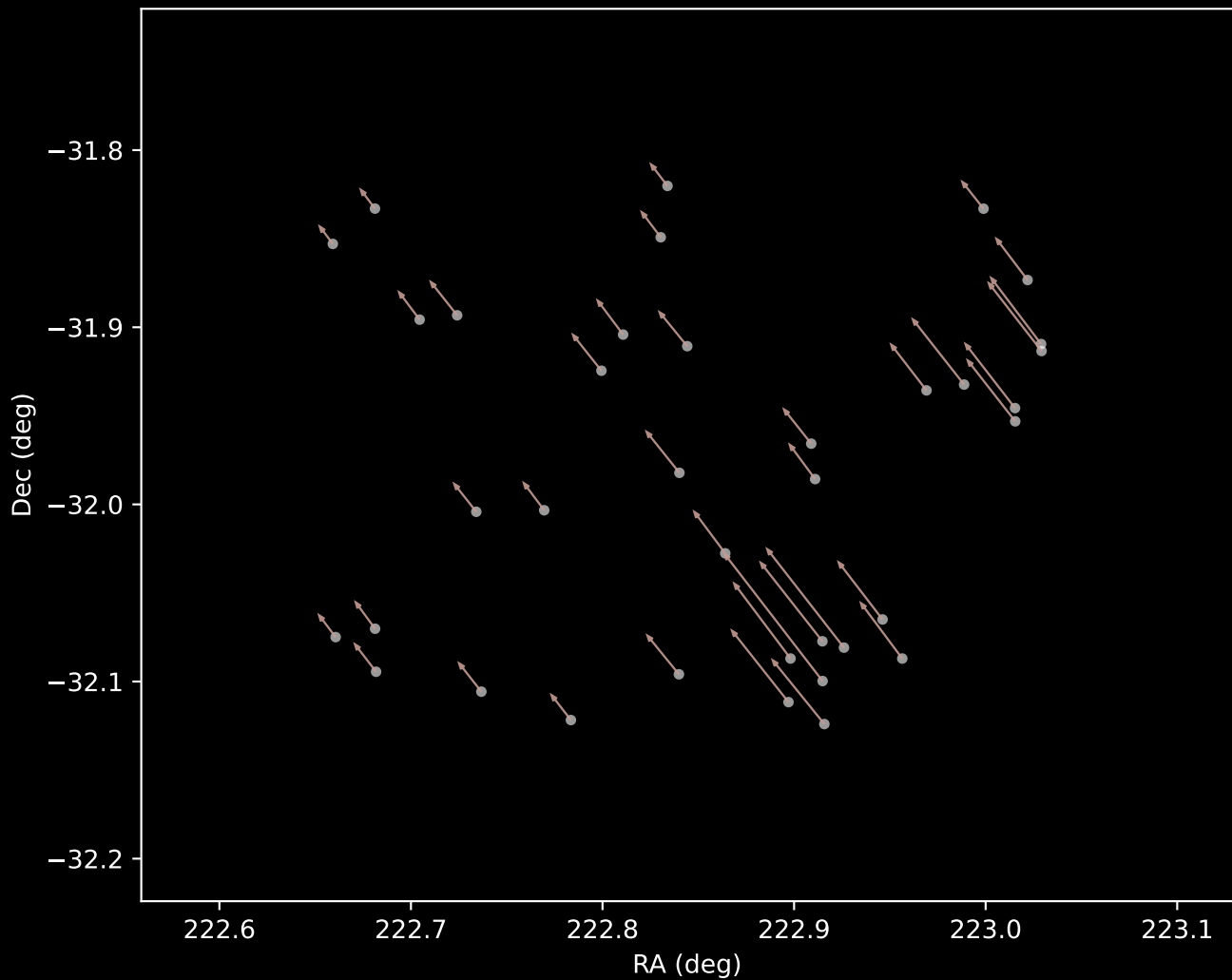
Gaia DR3 Cluster 11 Proper Motion Vectors (n=37)
