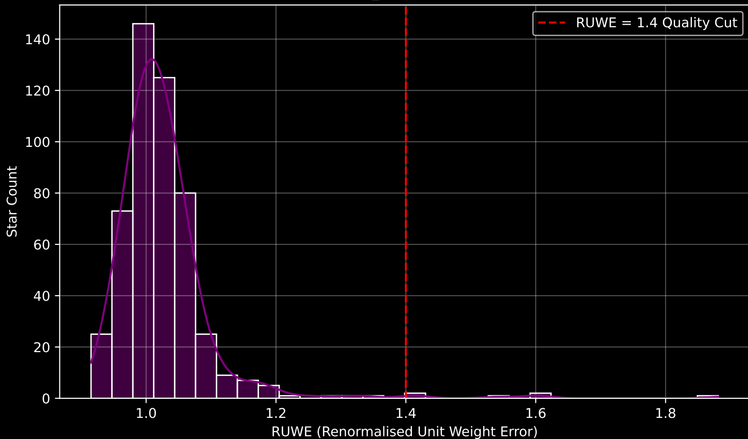
Gaia Cluster: [Ruprecht_54] RUWE Distribution (n= 505)
