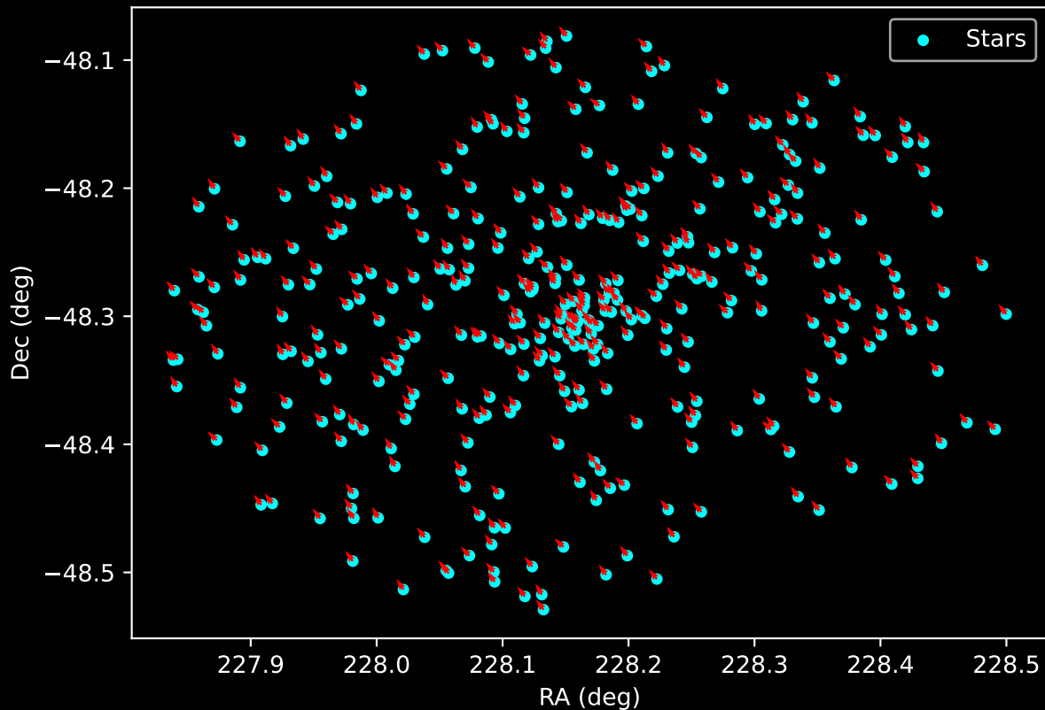
Gaia Cluster: [Ruprecht_63] Proper Motion Vectors for Gaia Star Field (n= 361)
