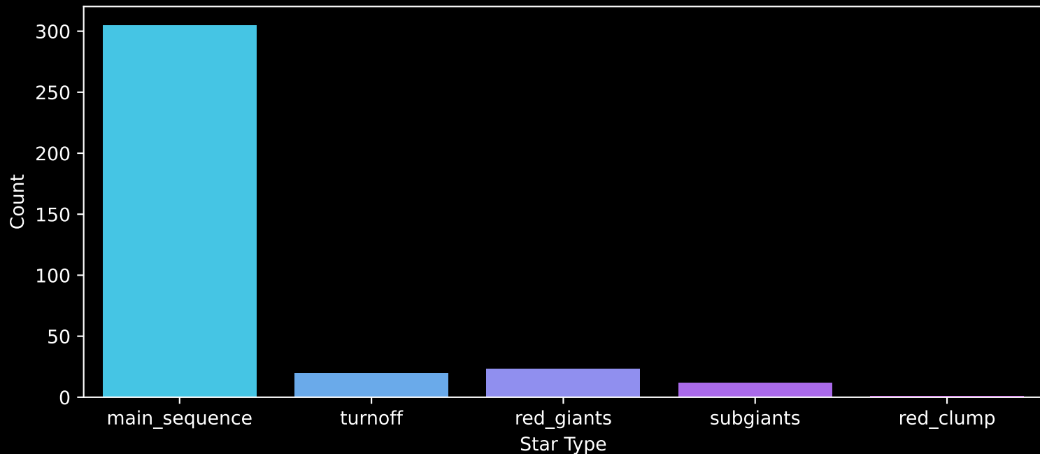
Gaia Cluster: [Ruprecht_63] Count plot of Star Type
