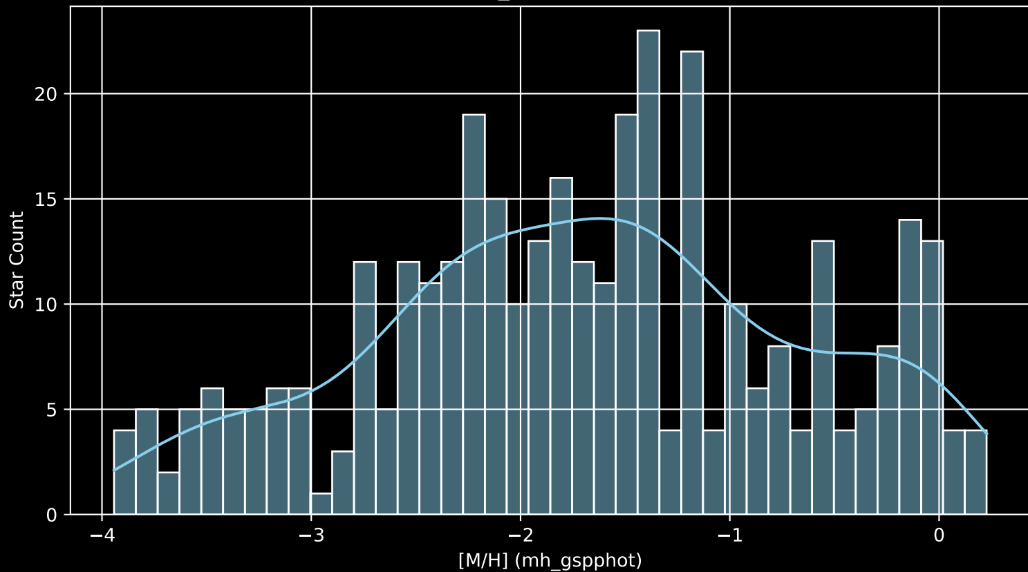
Gaia Cluster: [Ruprecht_63 [M/H] (mh_gspphot) (n= 361)
