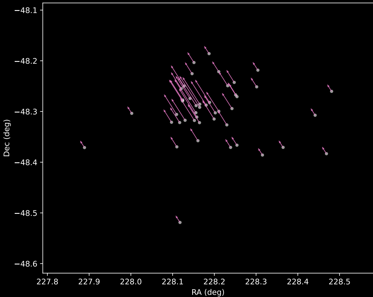
Gaia DR3 Cluster 12 Proper Motion Vectors (n=45)
