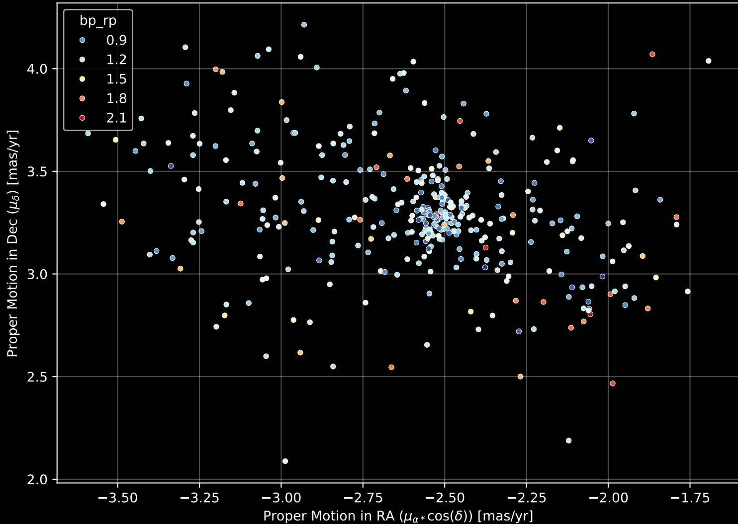
Gaia Cluster: [Ruprecht_63] Proper Motion Diagram (n= 361)
