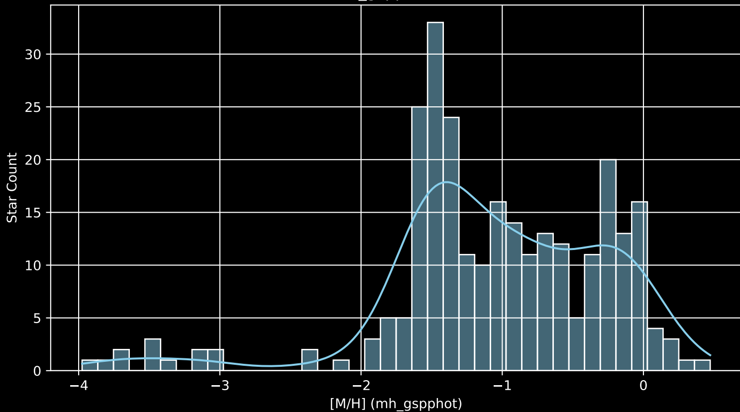
Gaia Cluster: [Ruprecht_65 [M/H] (mh_gspphot) (n= 271)
