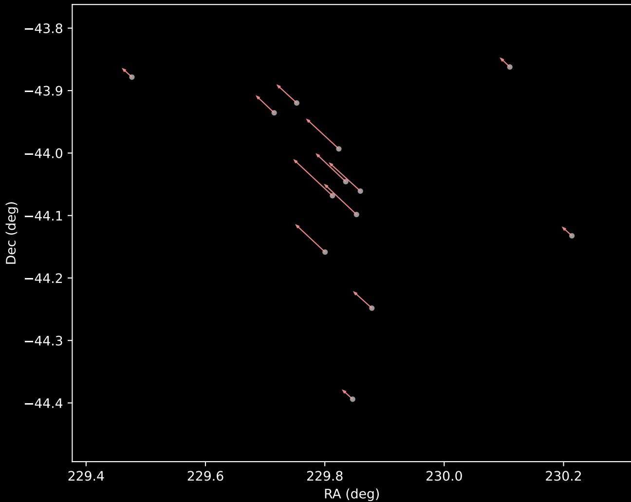
Gaia DR3 Cluster 7 Proper Motion Vectors (n=13)
