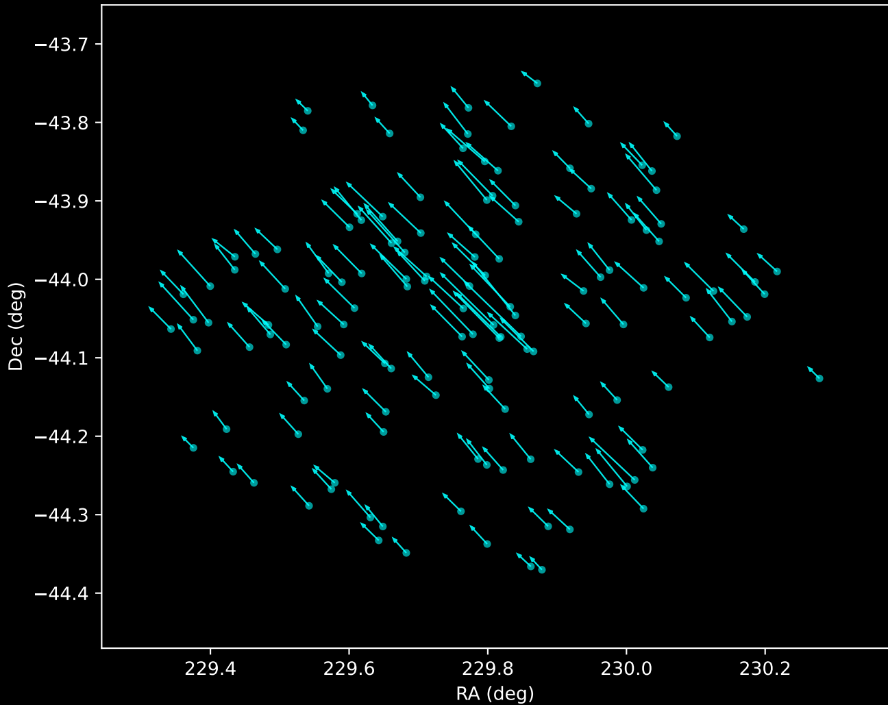
Gaia DR3 Noise Stream Proper Motion Vectors (n=137)
