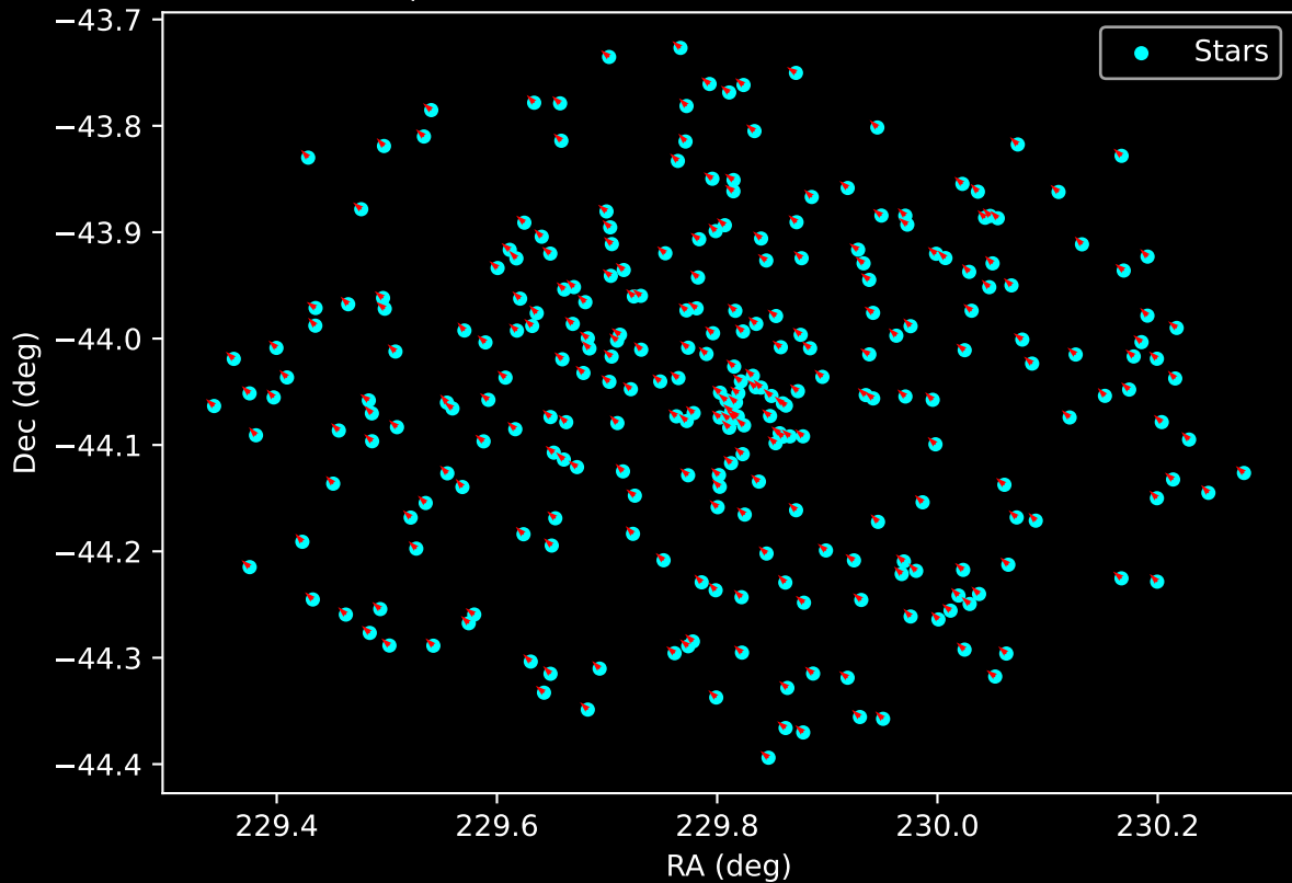
Gaia Cluster: [Ruprecht_65] Proper Motion Vectors for Gaia Star Field (n= 272)
