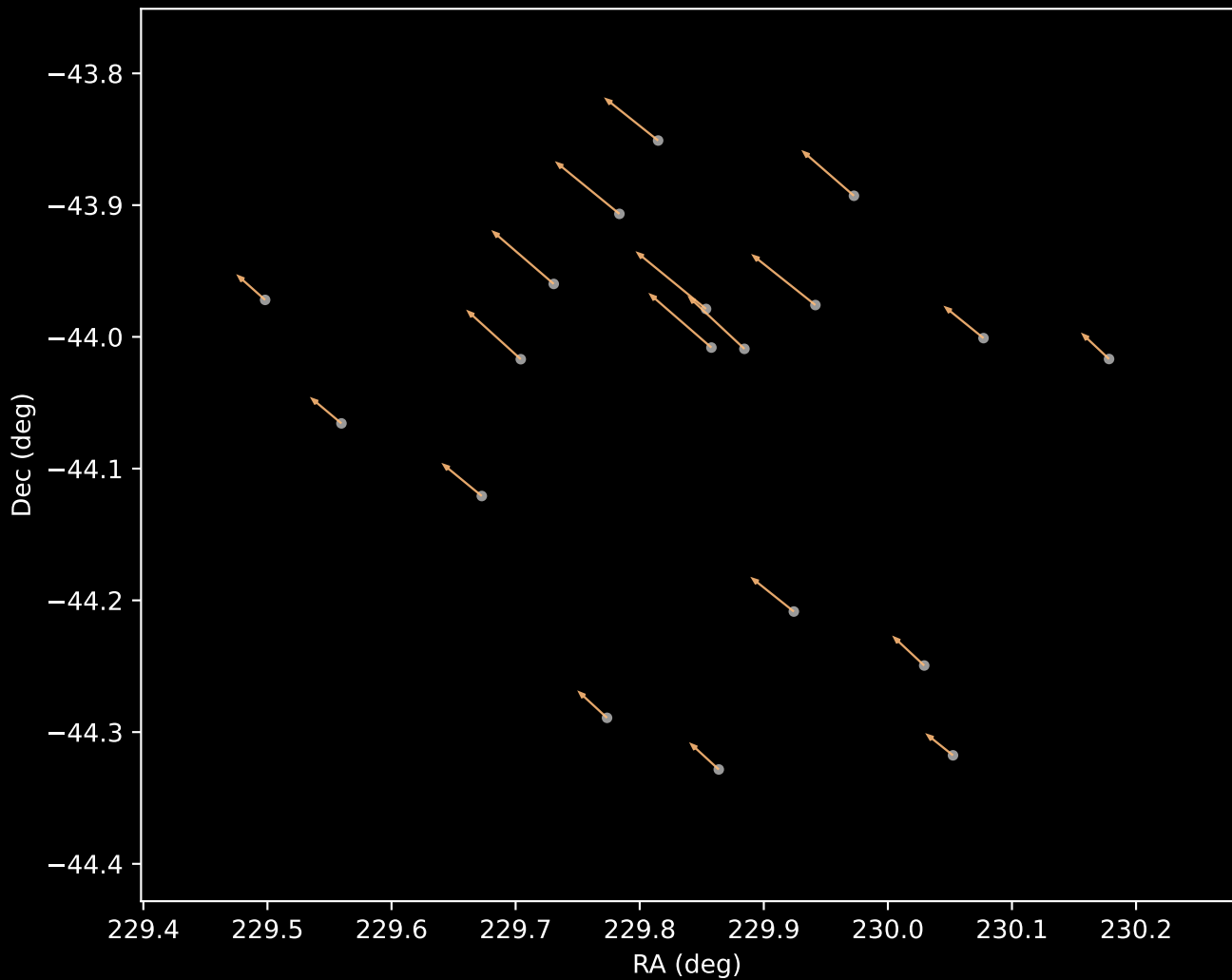
Gaia DR3 Cluster 3 Proper Motion Vectors (n=19)
