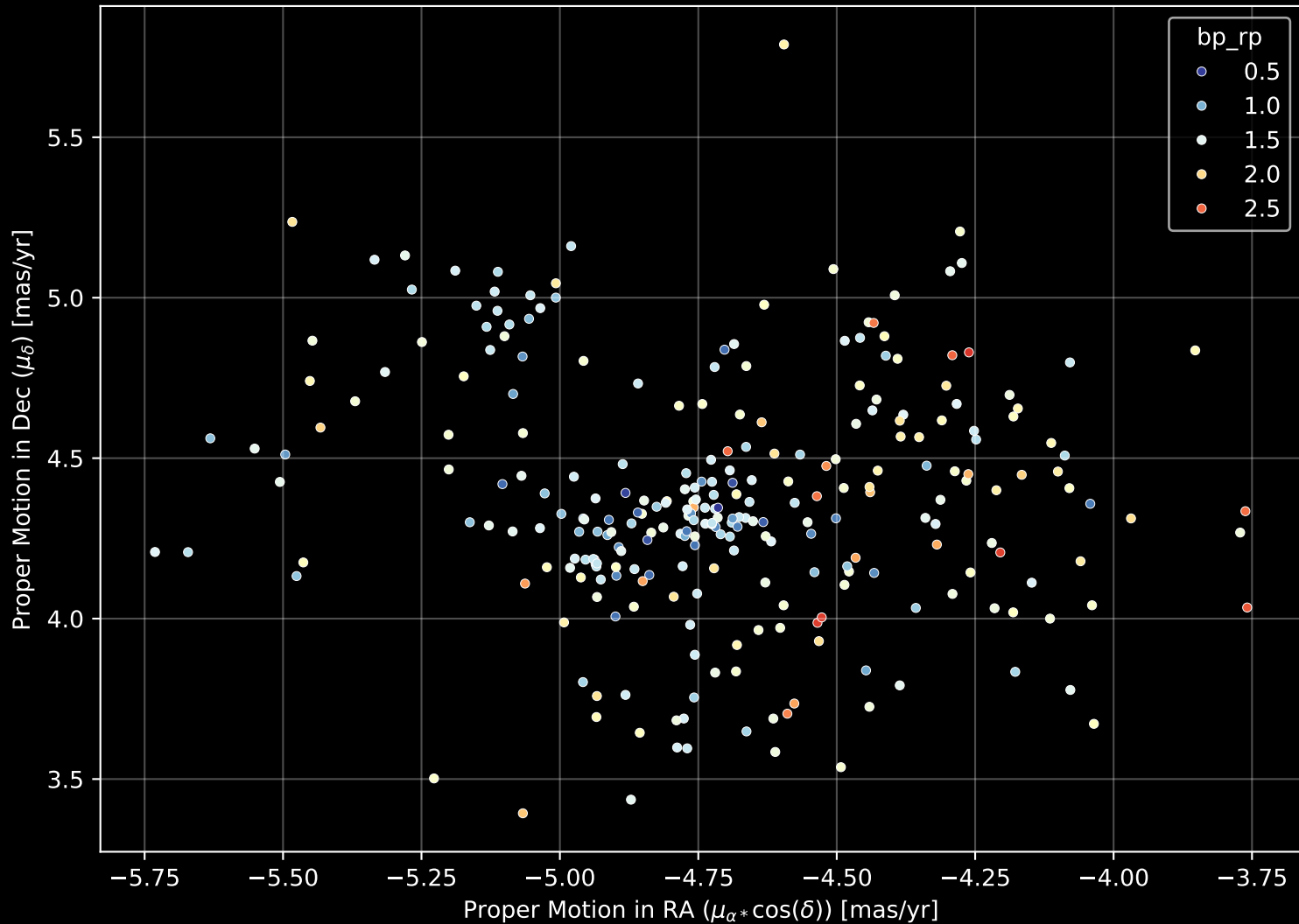
Gaia Cluster: [Ruprecht_65] Proper Motion Diagram (n= 272)
