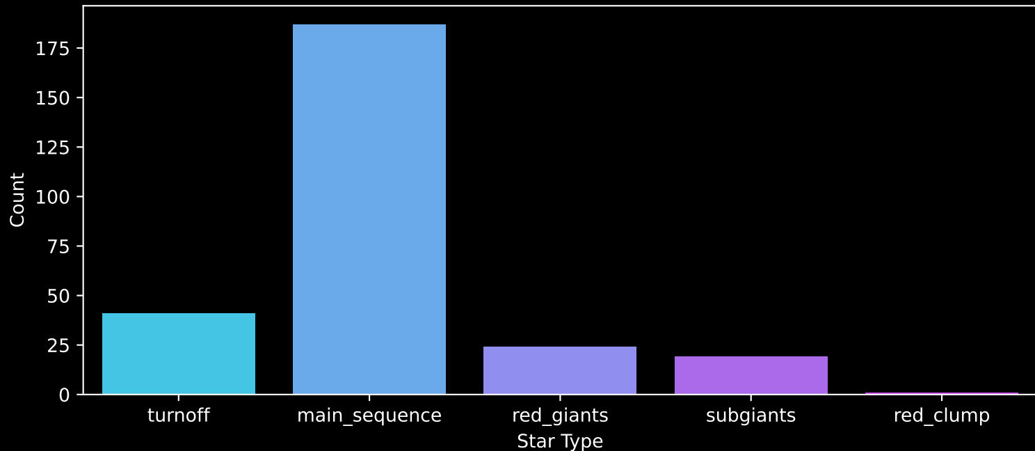
Gaia Cluster: [Ruprecht_65] Count plot of Star Type
