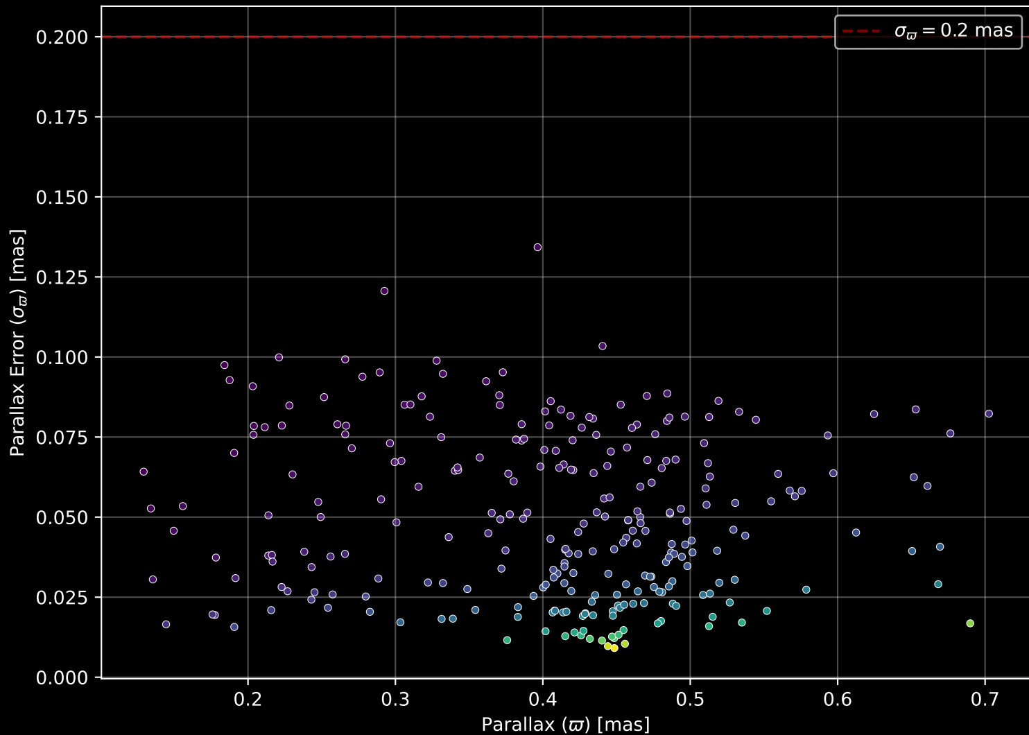
Gaia Cluster: [Ruprecht_65] Parallax Quality (n= 272)
