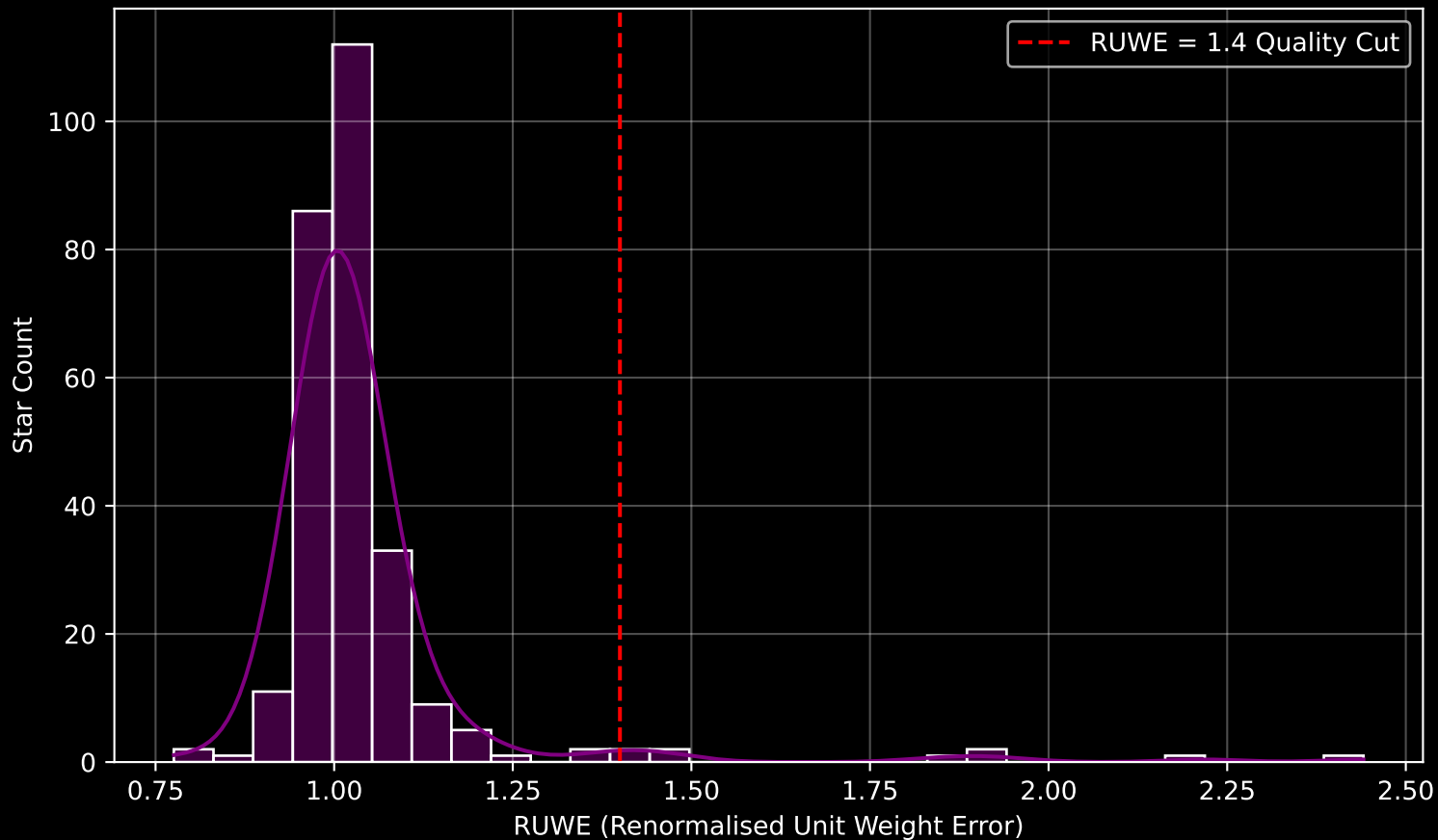
Gaia Cluster: [Ruprecht_65] RUWE Distribution (n= 271)
