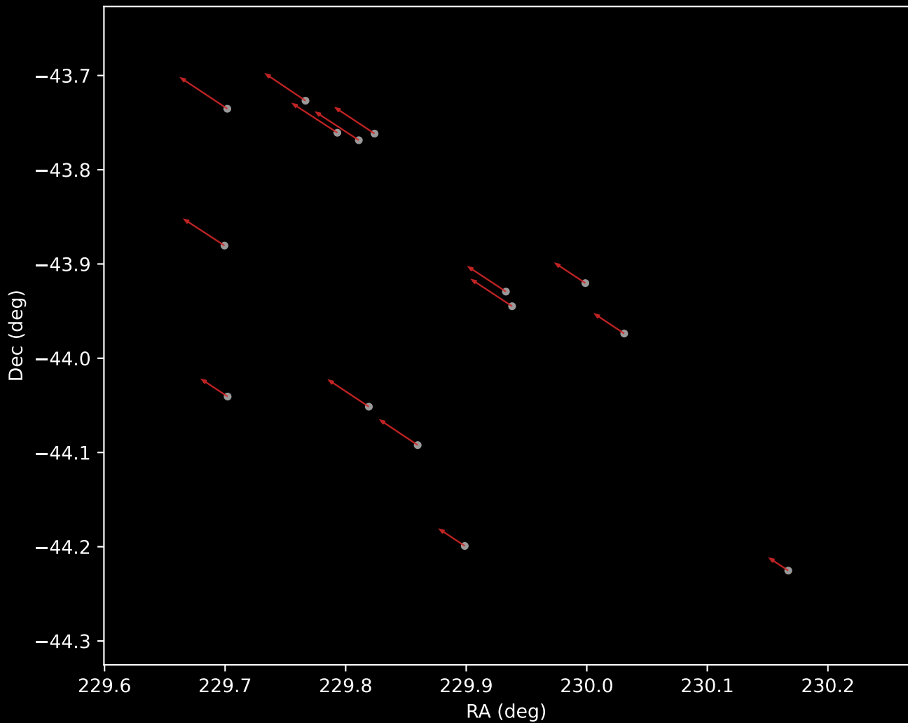
Gaia DR3 Cluster 6 Proper Motion Vectors (n=15)
