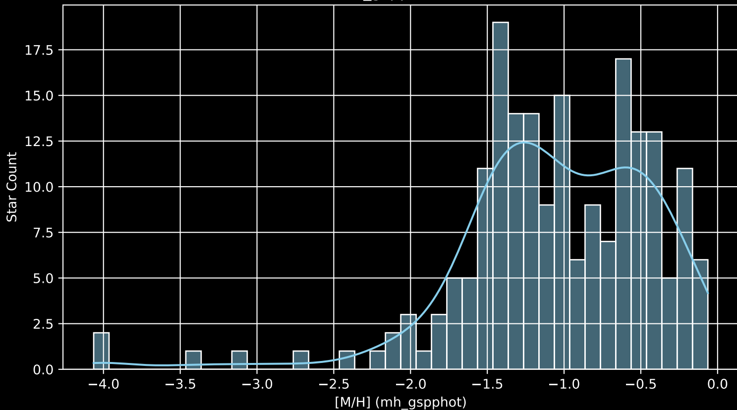
Gaia Cluster: [Ruprecht_71 [M/H] (mh_gspphot) (n= 195)
