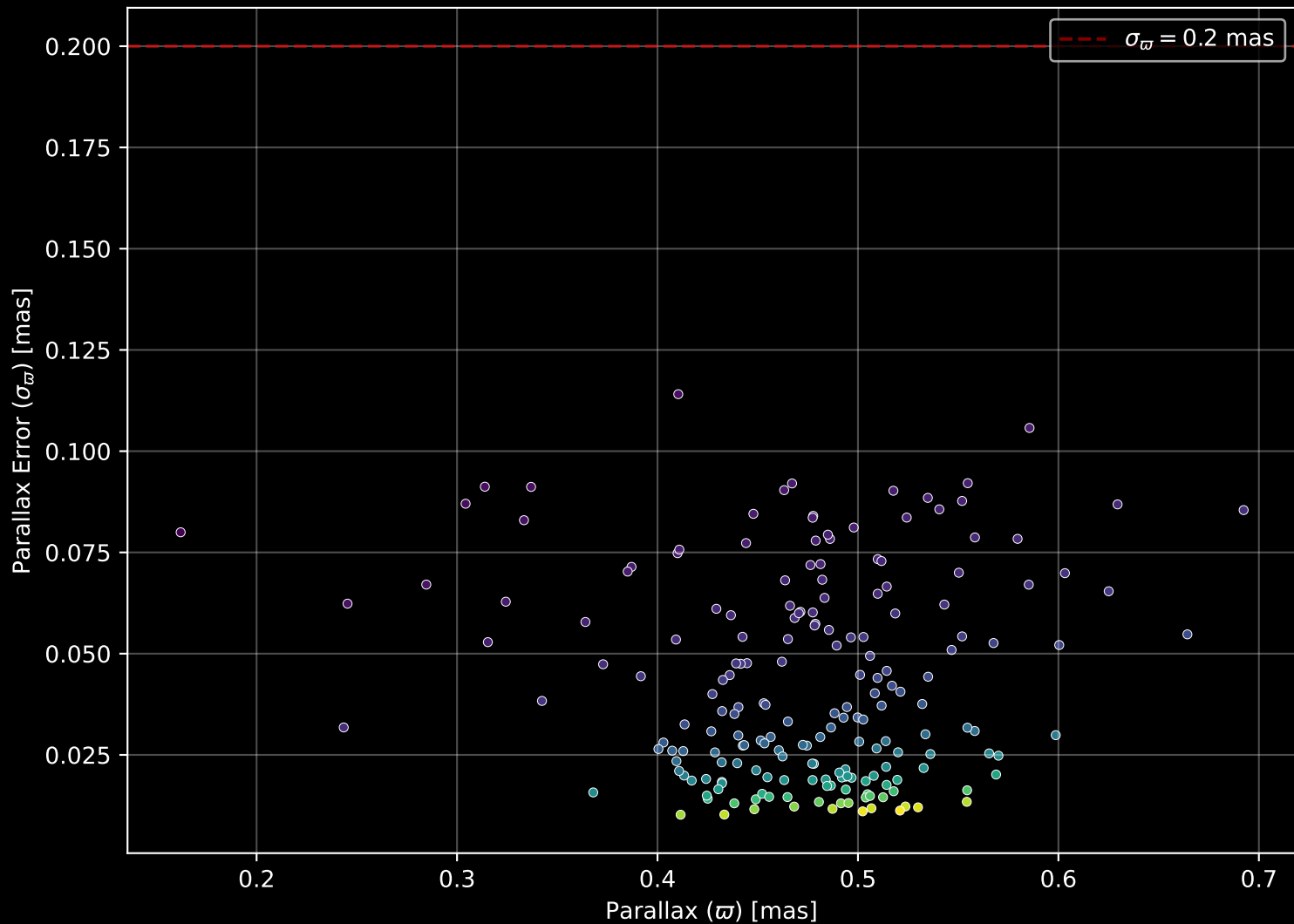
Gaia Cluster: [Ruprecht_71] Parallax Quality (n= 195)
