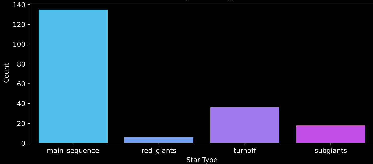
Gaia Cluster: [Ruprecht_71] Count plot of Star Type
