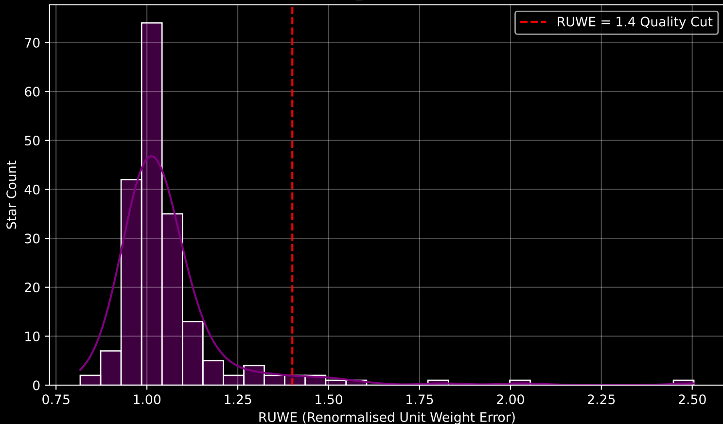
Gaia Cluster: [Ruprecht_71] RUWE Distribution (n= 195)
