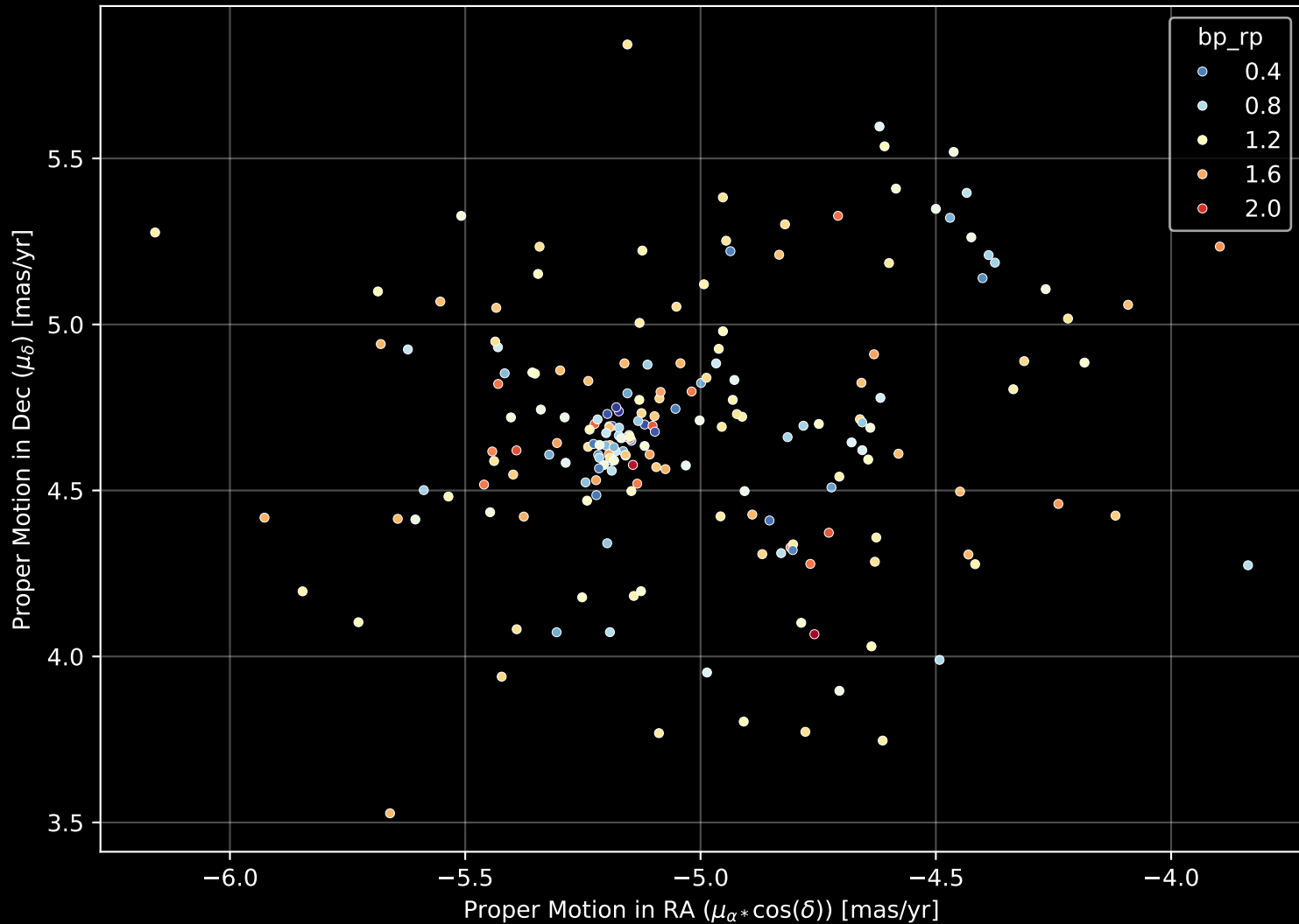
Gaia Cluster: [Ruprecht_71] Proper Motion Diagram (n= 195)
