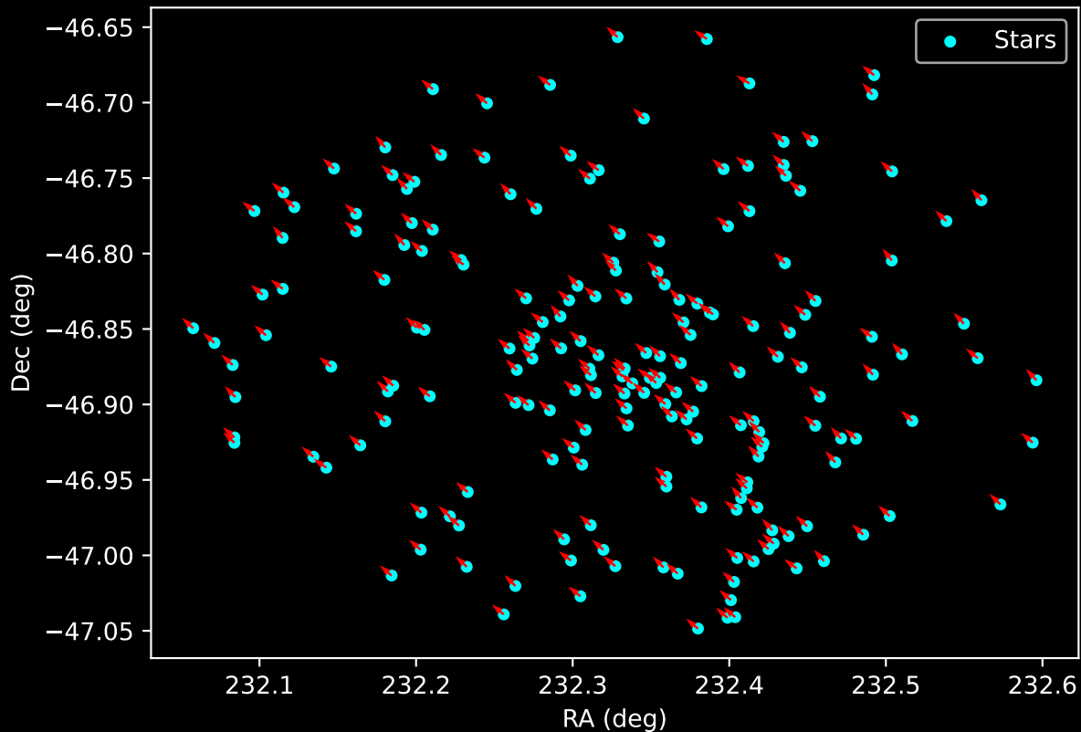
Gaia Cluster: [Ruprecht_71] Proper Motion Vectors for Gaia Star Field (n= 195)
