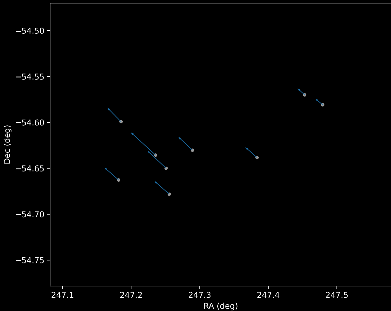
Gaia DR3 Cluster 0 Proper Motion Vectors (n=9)
