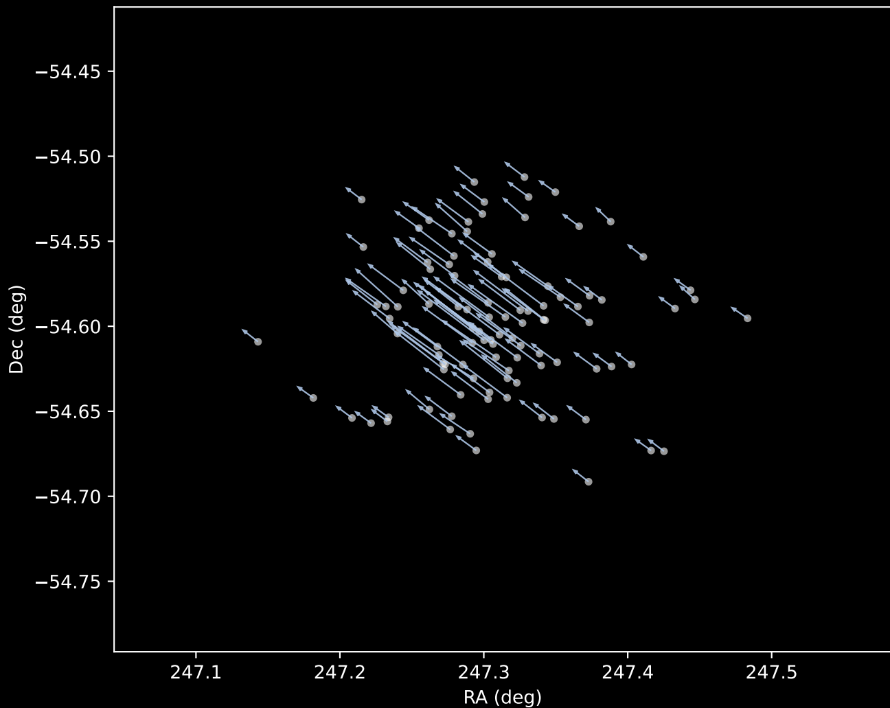
Gaia DR3 Cluster 1 Proper Motion Vectors (n=102)
