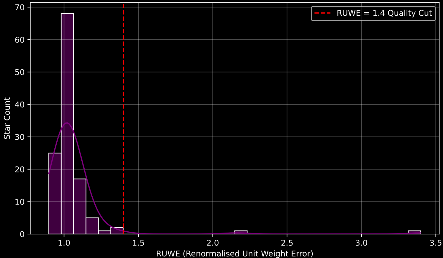
Gaia Cluster: [Ruprecht_83] RUWE Distribution (n= 120)
