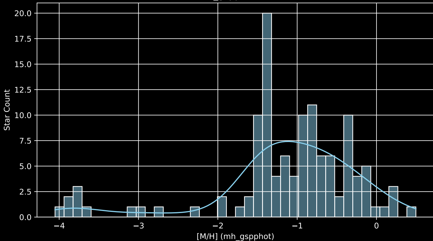
Gaia Cluster: [Ruprecht_83 [M/H] (mh_gspphot) (n= 120)
