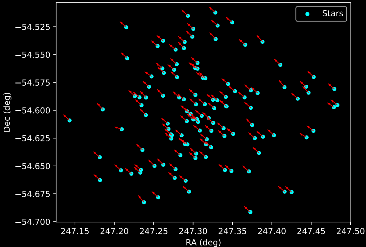
Gaia Cluster: [Ruprecht_83] Proper Motion Vectors for Gaia Star Field (n= 120)
