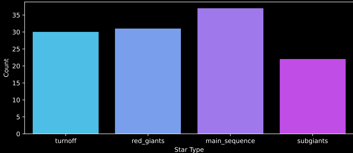
Gaia Cluster: [Ruprecht_83] Count plot of Star Type
