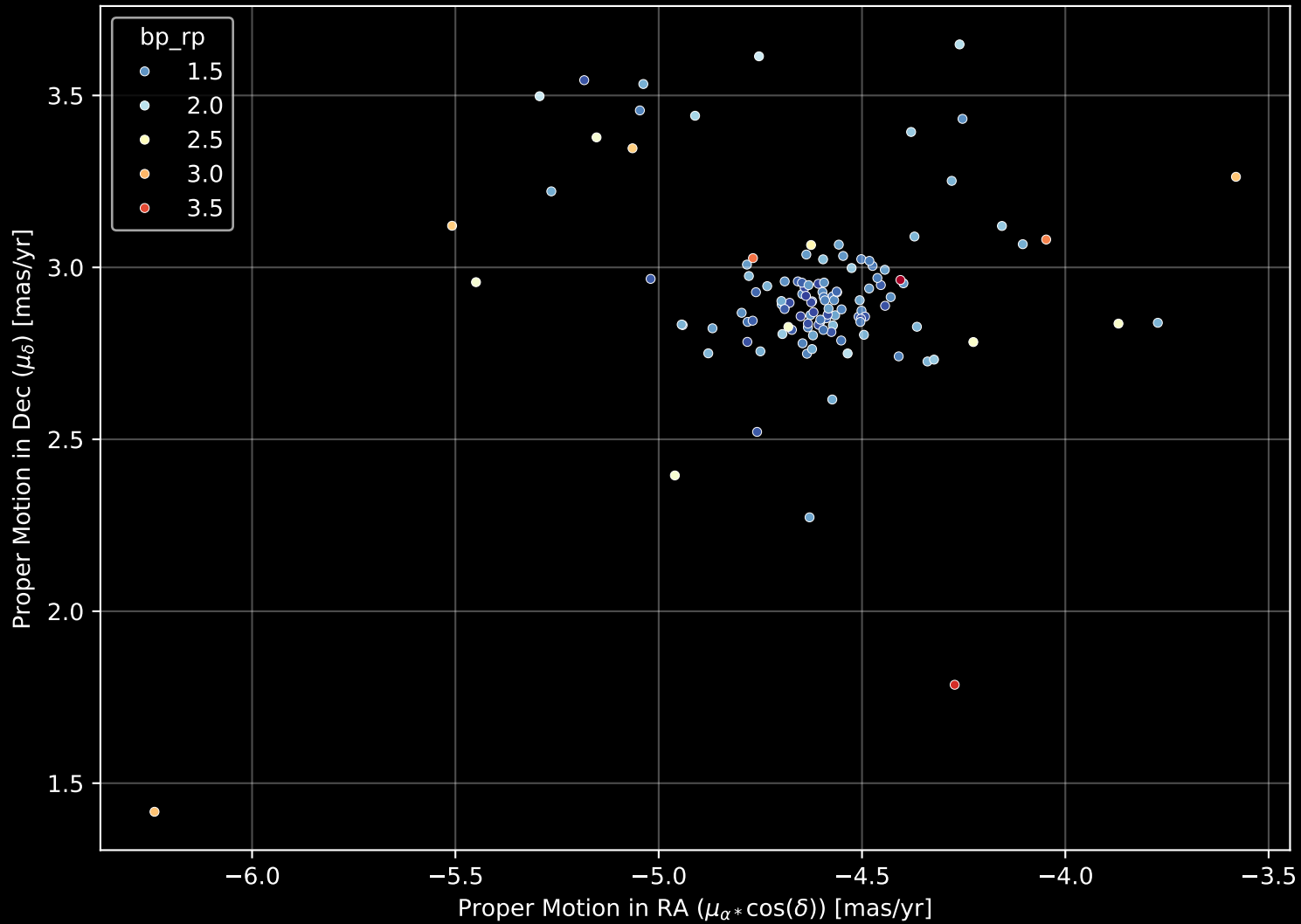
Gaia Cluster: [Ruprecht_83] Proper Motion Diagram (n= 120)
