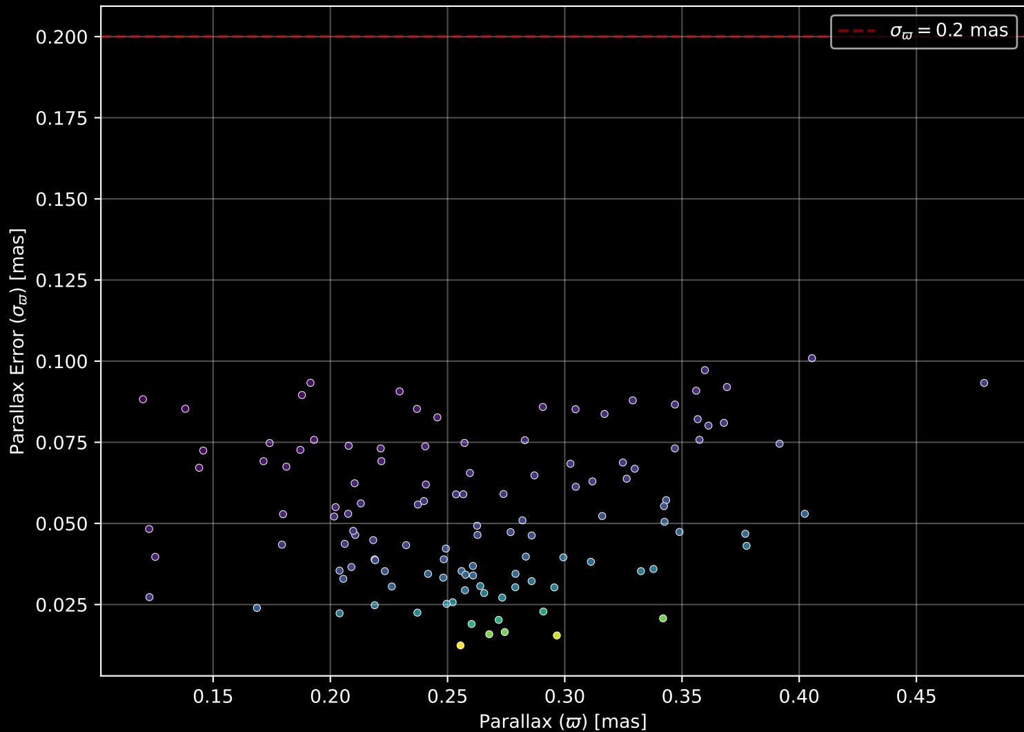
Gaia Cluster: [Ruprecht_83] Parallax Quality (n= 120)
