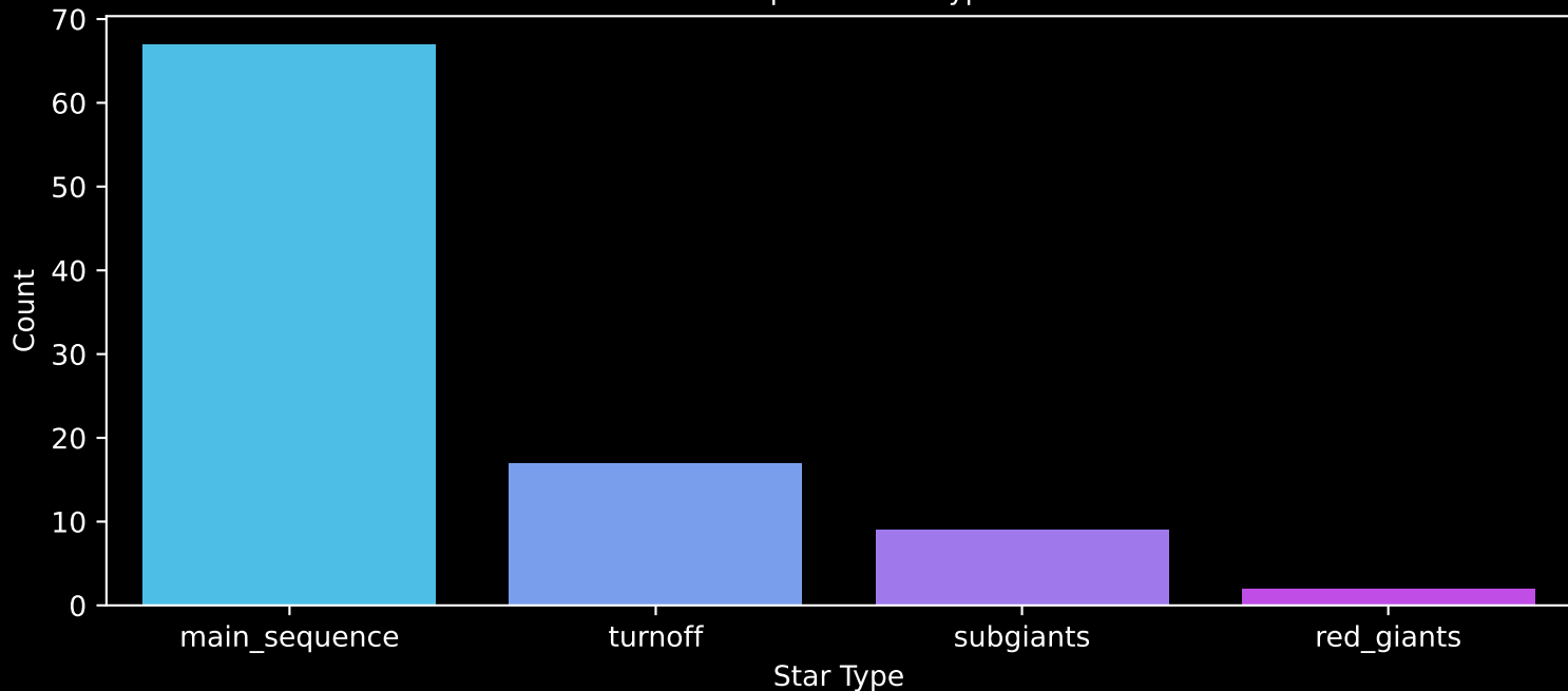
Gaia Cluster: [Ruprecht_84] Count plot of Star Type
