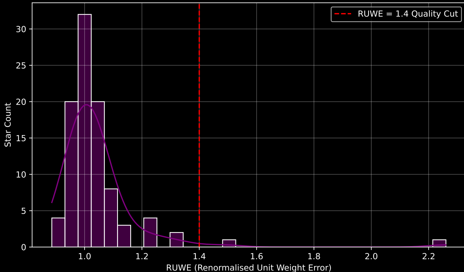
Gaia Cluster: [Ruprecht_84] RUWE Distribution (n= 95)
