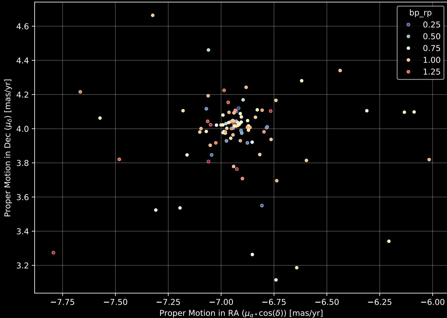
Gaia Cluster: [Ruprecht_84] Proper Motion Diagram (n= 95)
