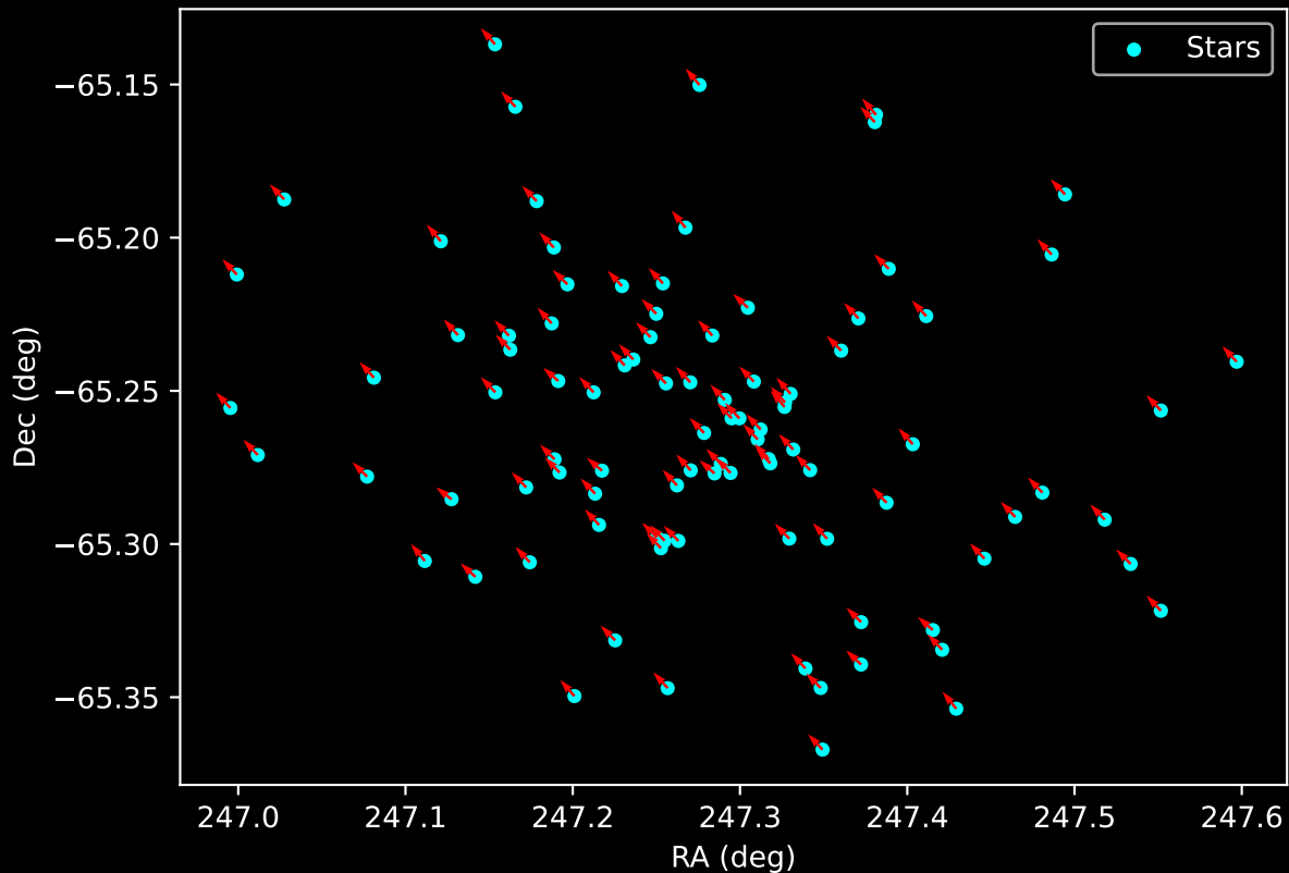
Gaia Cluster: [Ruprecht_84] Proper Motion Vectors for Gaia Star Field (n= 95)
