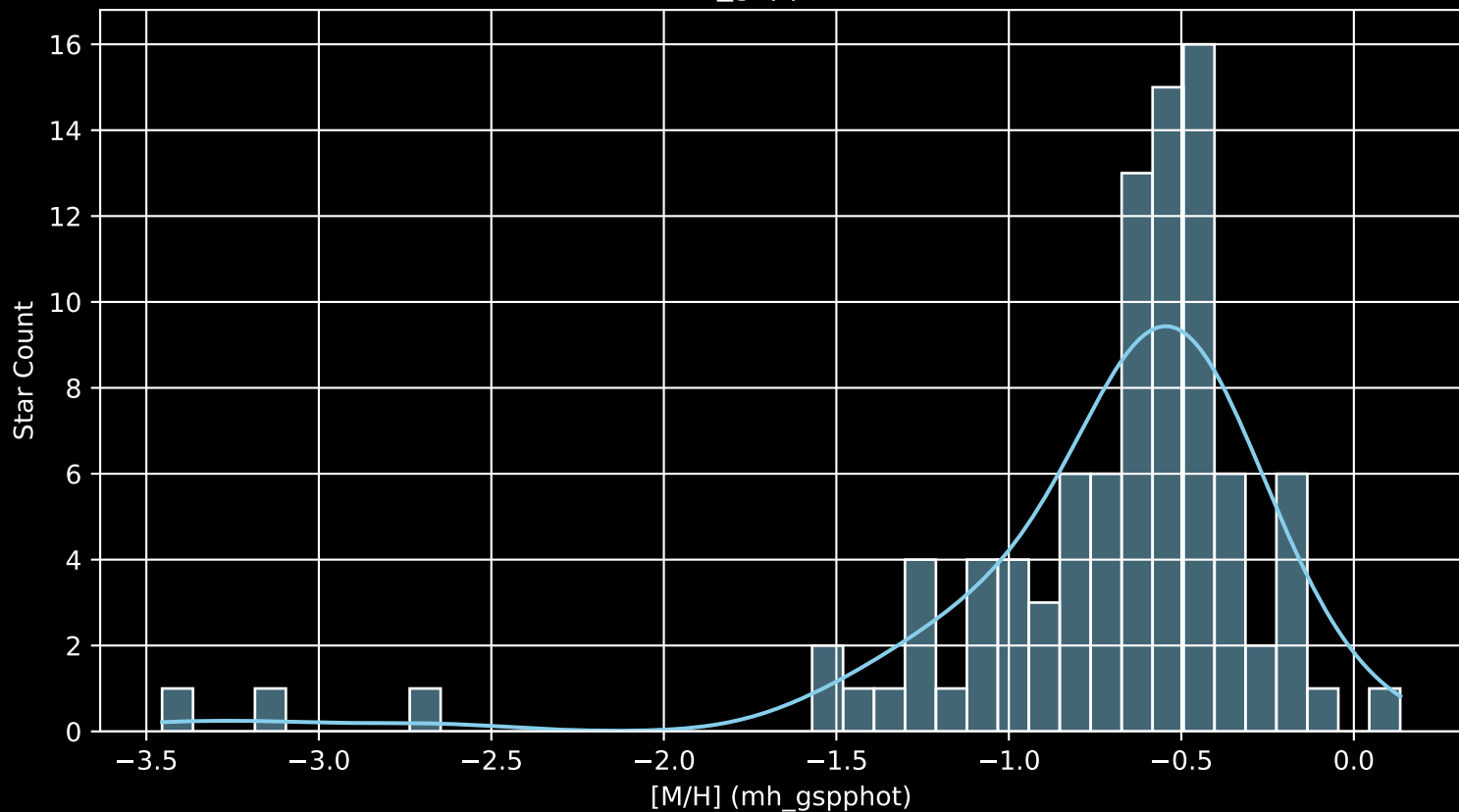
Gaia Cluster: [Ruprecht_84 [M/H] (mh_gspphot) (n= 95)
