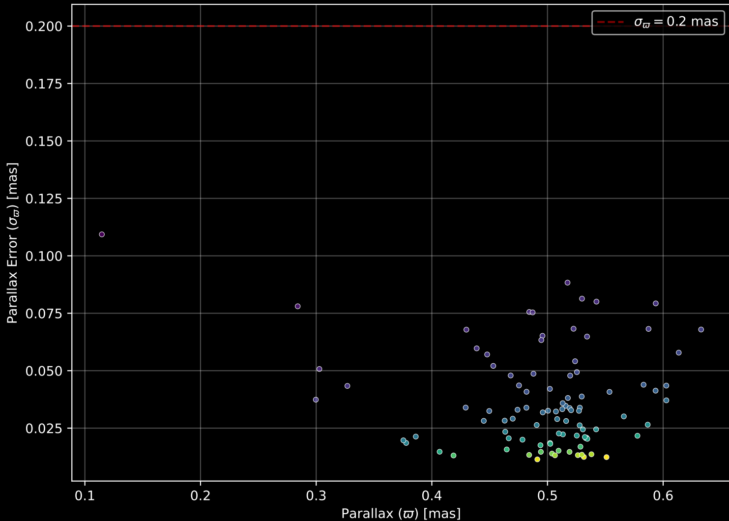
Gaia Cluster: [Ruprecht_84] Parallax Quality (n= 95)
