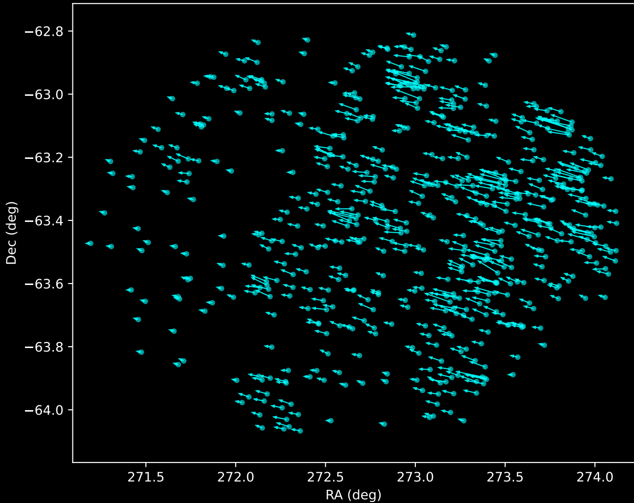
Gaia DR3 Noise Stream Proper Motion Vectors (n=550)
