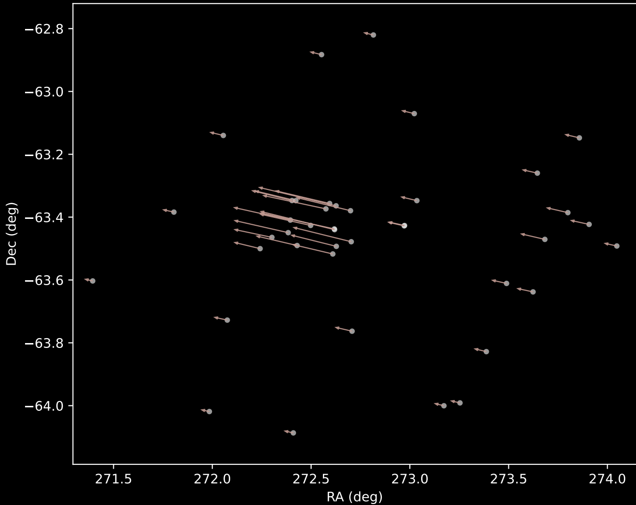
Gaia DR3 Cluster 71 Proper Motion Vectors (n=41)
