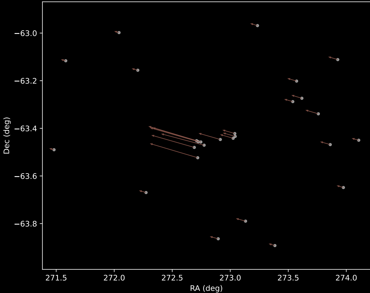
Gaia DR3 Cluster 50 Proper Motion Vectors (n=27)
