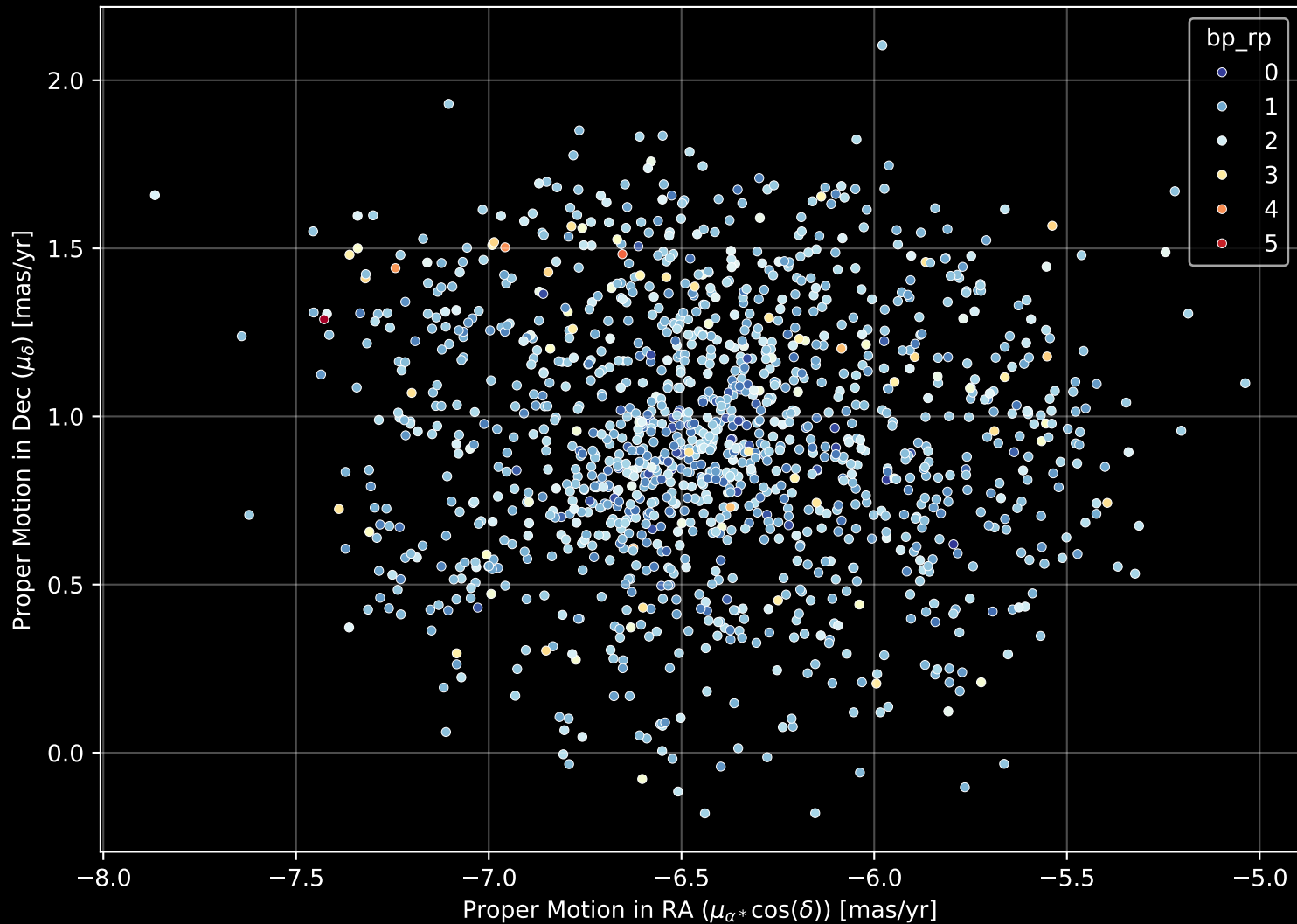
Gaia Cluster: [Ruprecht_94] Proper Motion Diagram (n= 1331)
