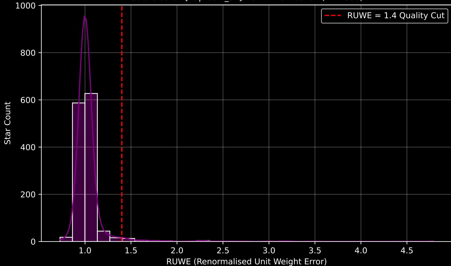
Gaia Cluster: [Ruprecht_94] RUWE Distribution (n= 1330)
