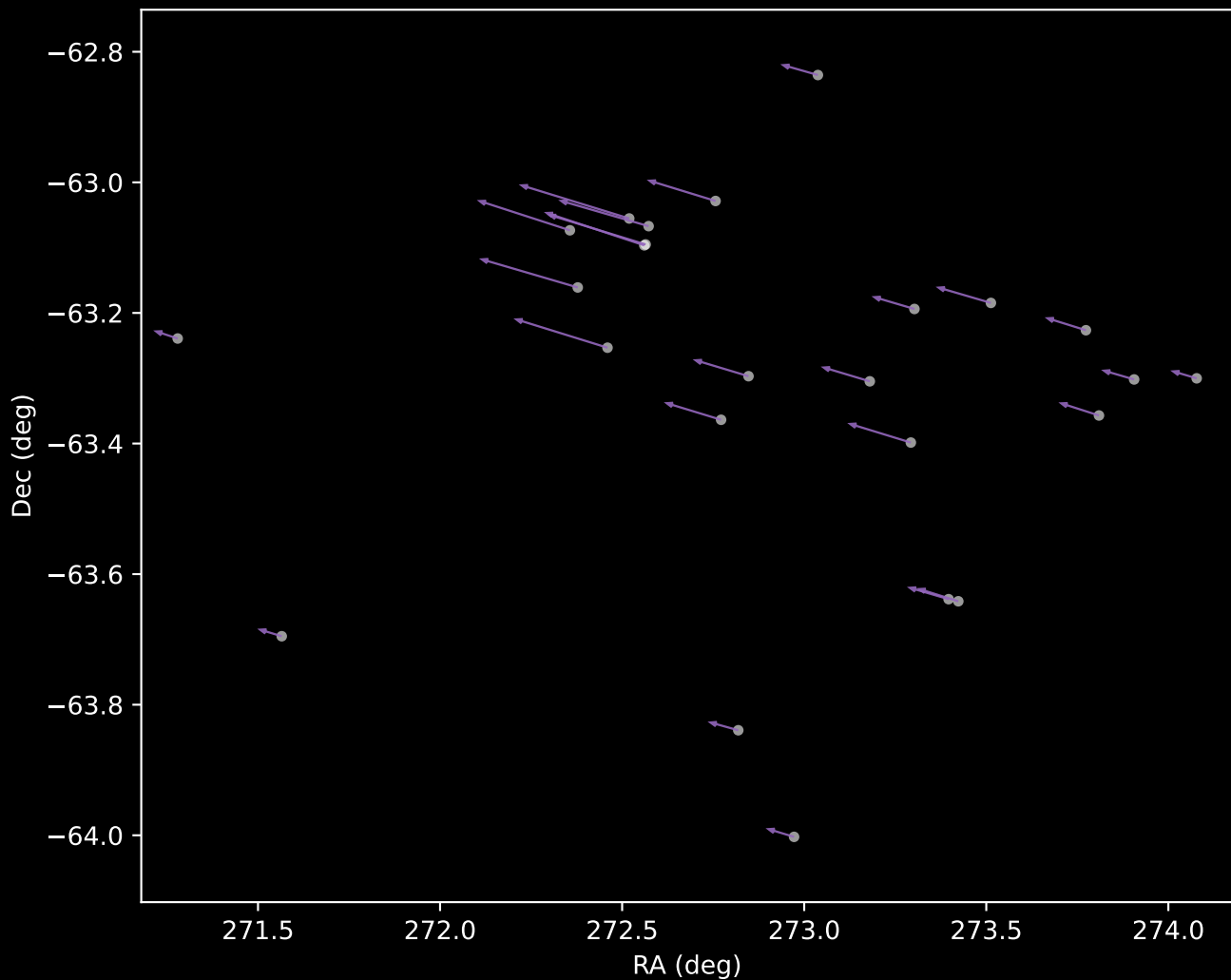
Gaia DR3 Cluster 68 Proper Motion Vectors (n=25)
