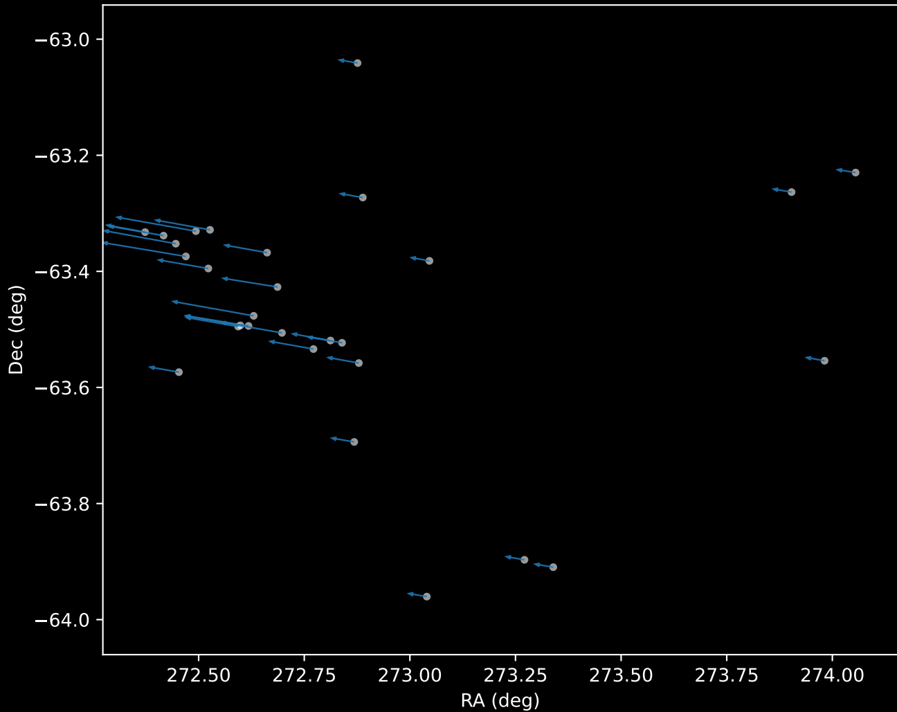
Gaia DR3 Cluster 60 Proper Motion Vectors (n=29)
