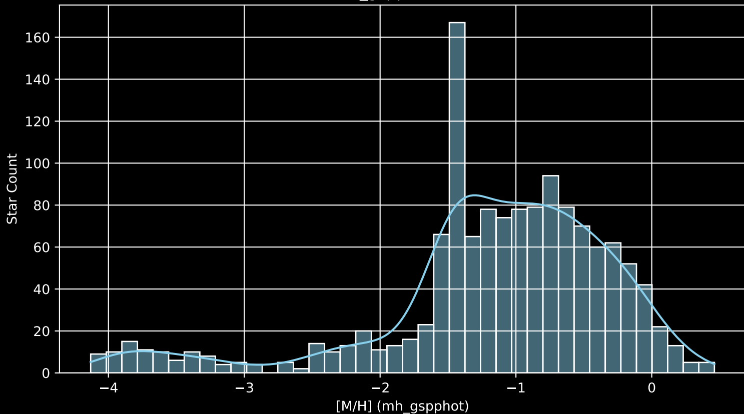
Gaia Cluster: [Ruprecht_94 [M/H] (mh_gspphot) (n= 1330)
