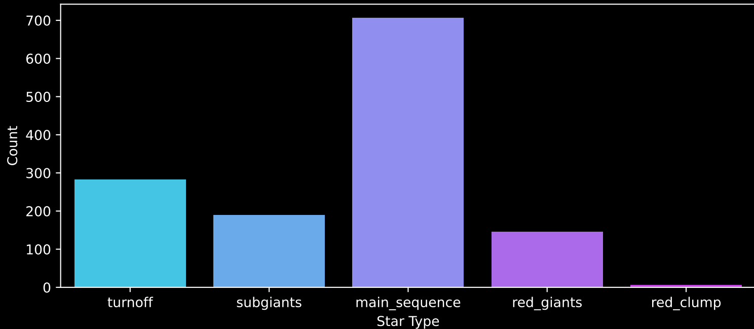
Gaia Cluster: [Ruprecht_94] Count plot of Star Type
