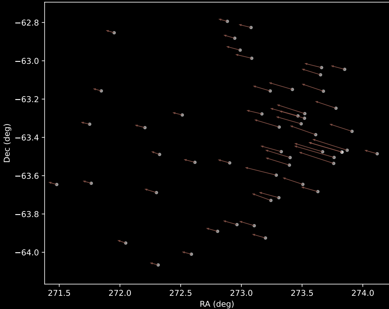
Gaia DR3 Cluster 10 Proper Motion Vectors (n=53)
