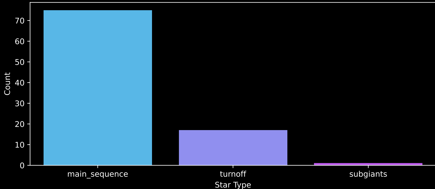
Gaia Cluster: [Ruprecht_98] Count plot of Star Type
