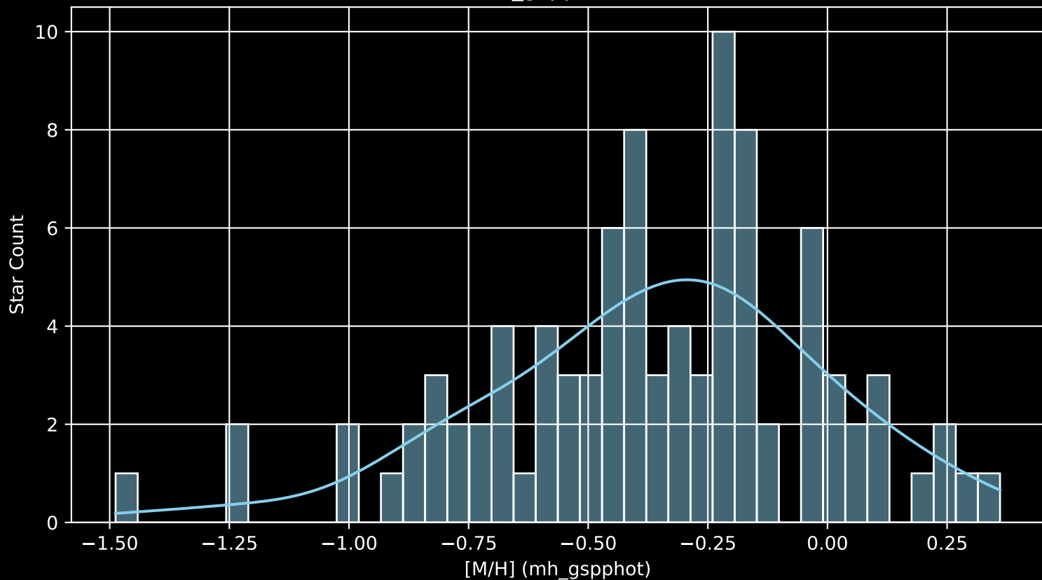
Gaia Cluster: [Ruprecht_98 [M/H] (mh_gspphot) (n= 93)
