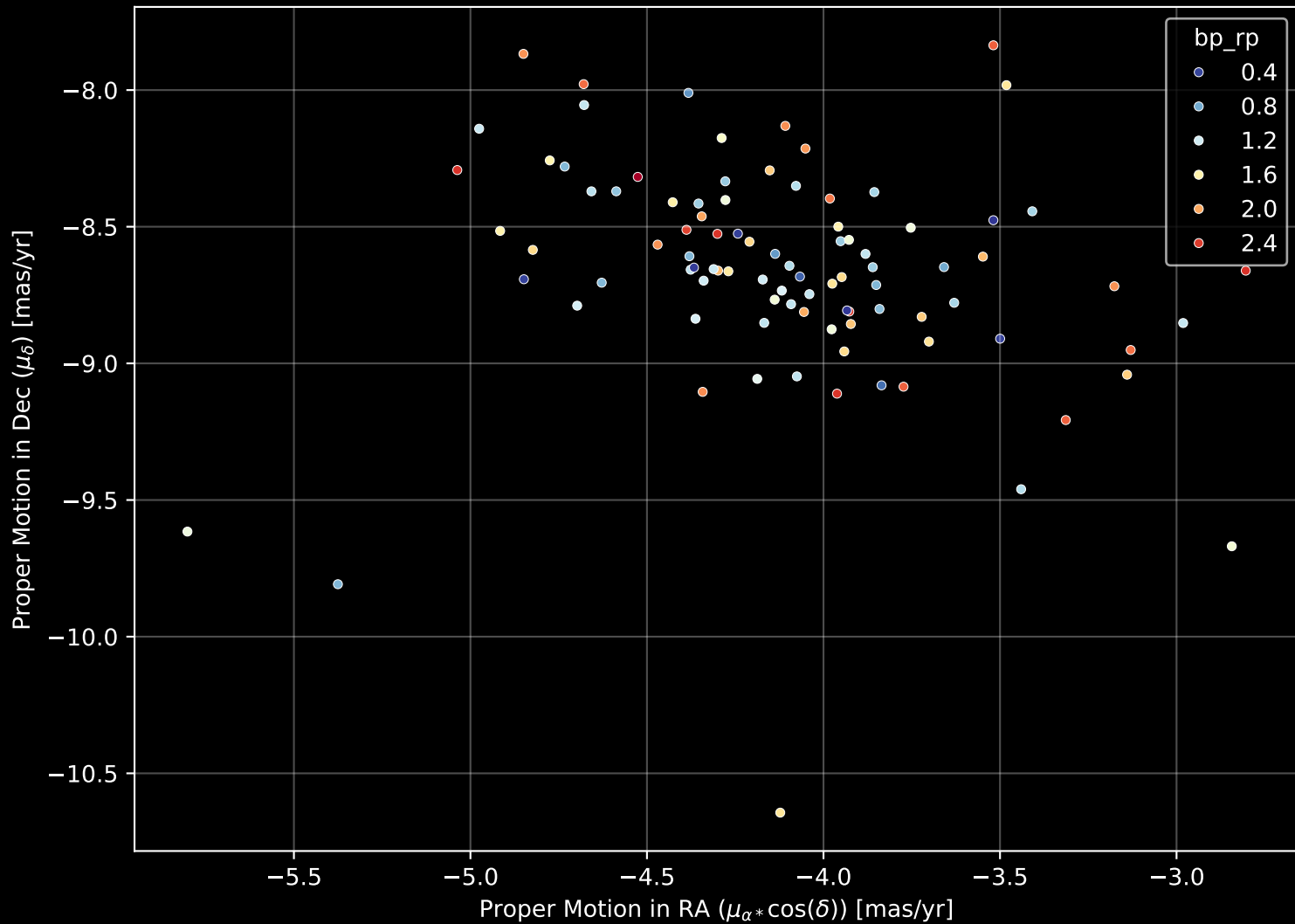
Gaia Cluster: [Ruprecht_98] Proper Motion Diagram (n= 93)
