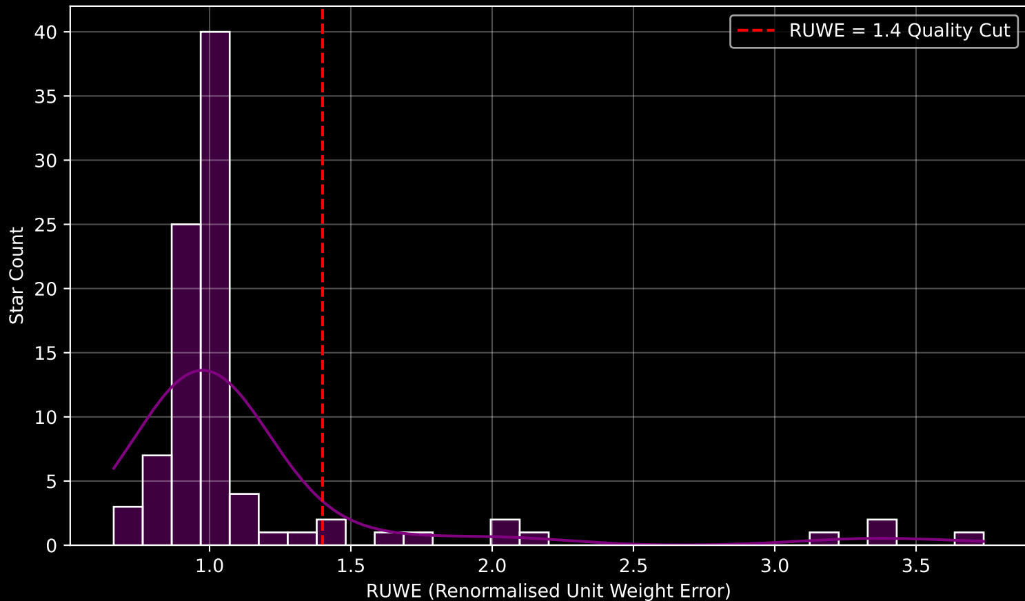
Gaia Cluster: [Ruprecht_98] RUWE Distribution (n= 92)
