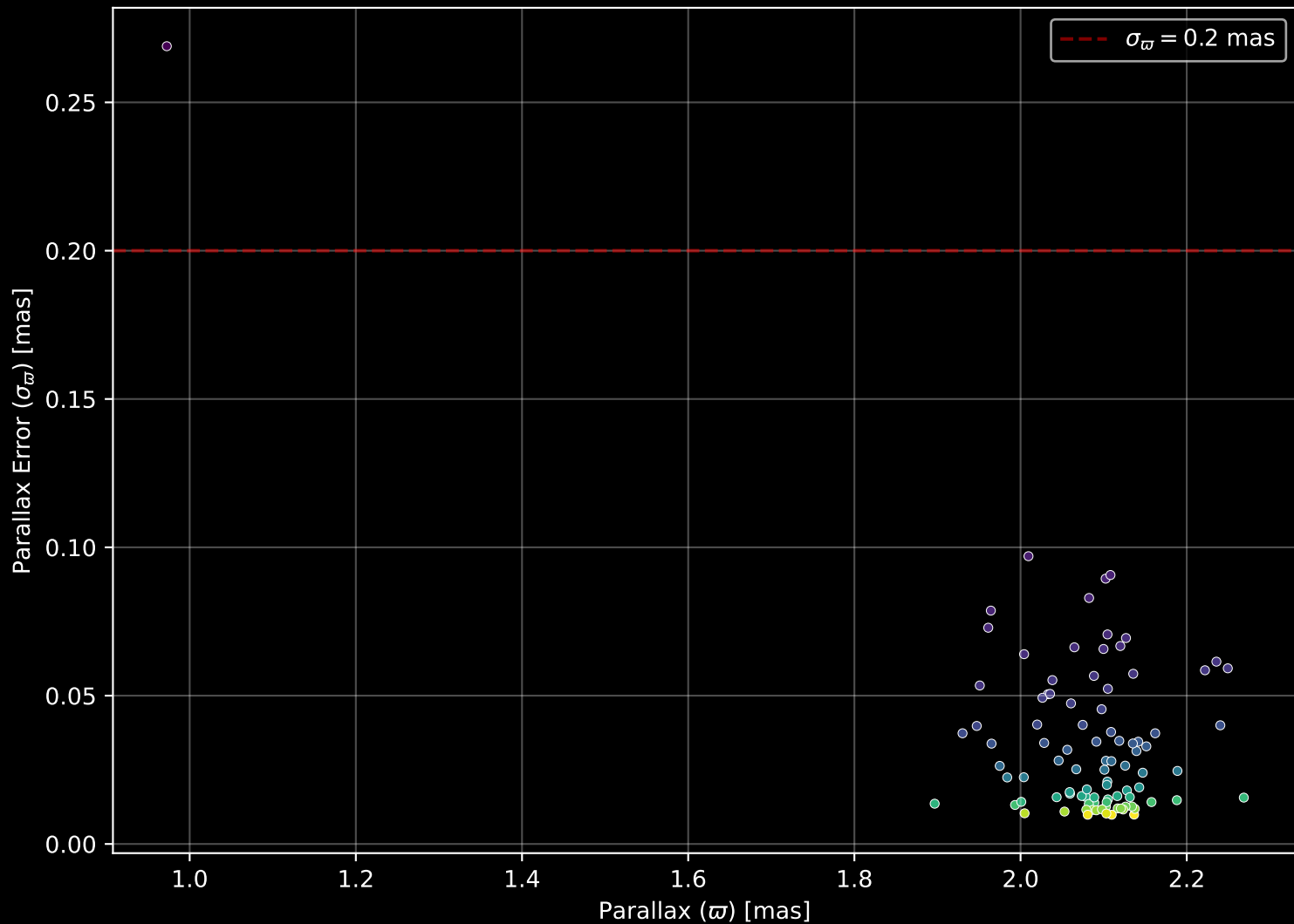
Gaia Cluster: [Ruprecht_98] Parallax Quality (n= 93)
