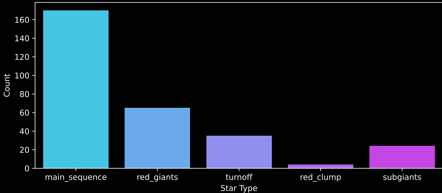
Gaia Cluster: [SAI_109] Count plot of Star Type
