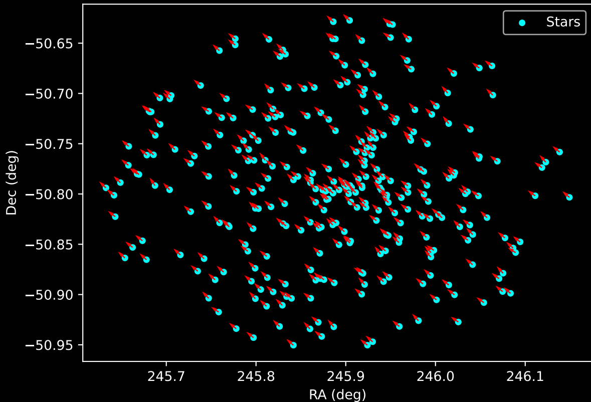
Gaia Cluster: [SAI_109] Proper Motion Vectors for Gaia Star Field (n= 298)
