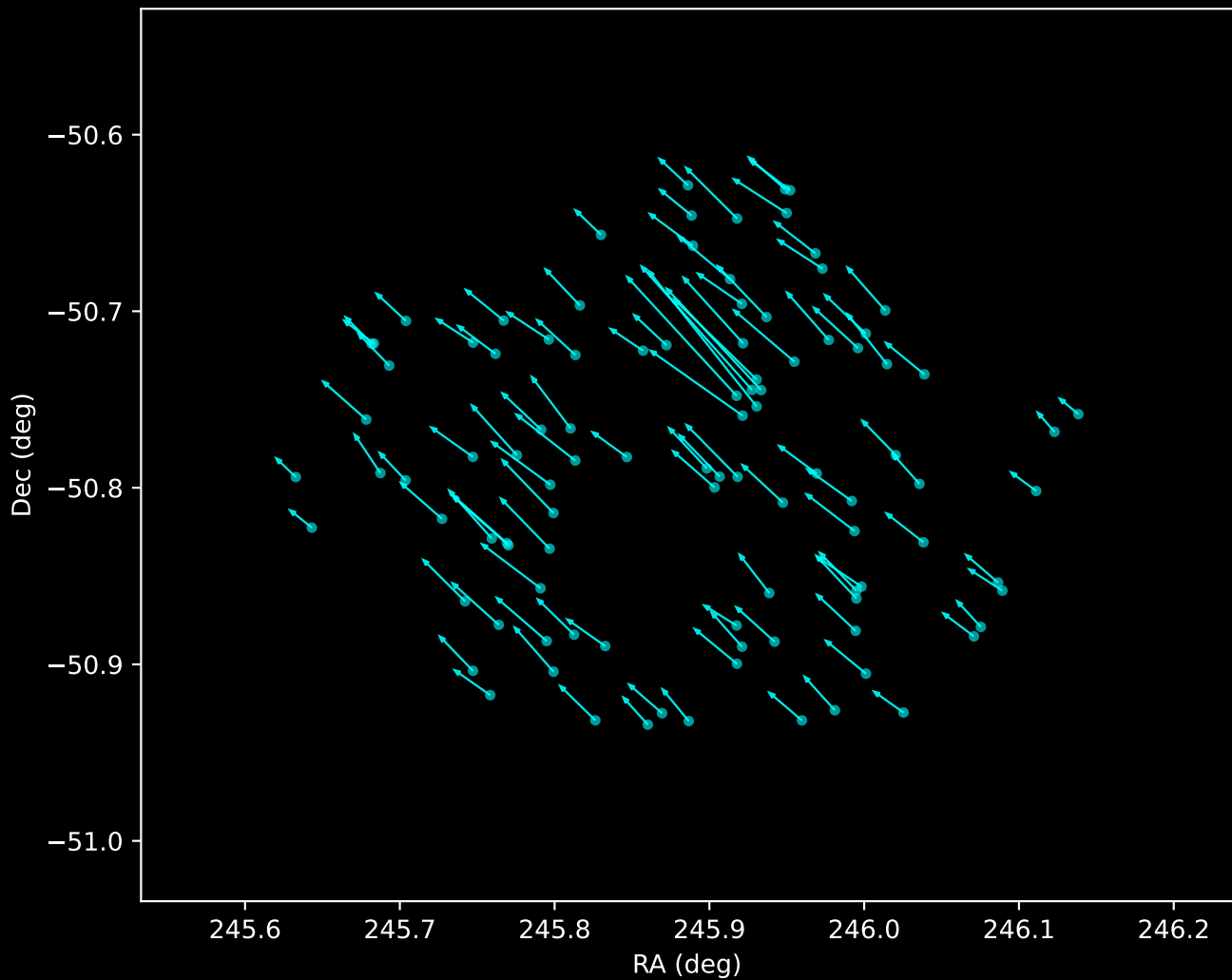
Gaia DR3 Noise Stream Proper Motion Vectors (n=101)
