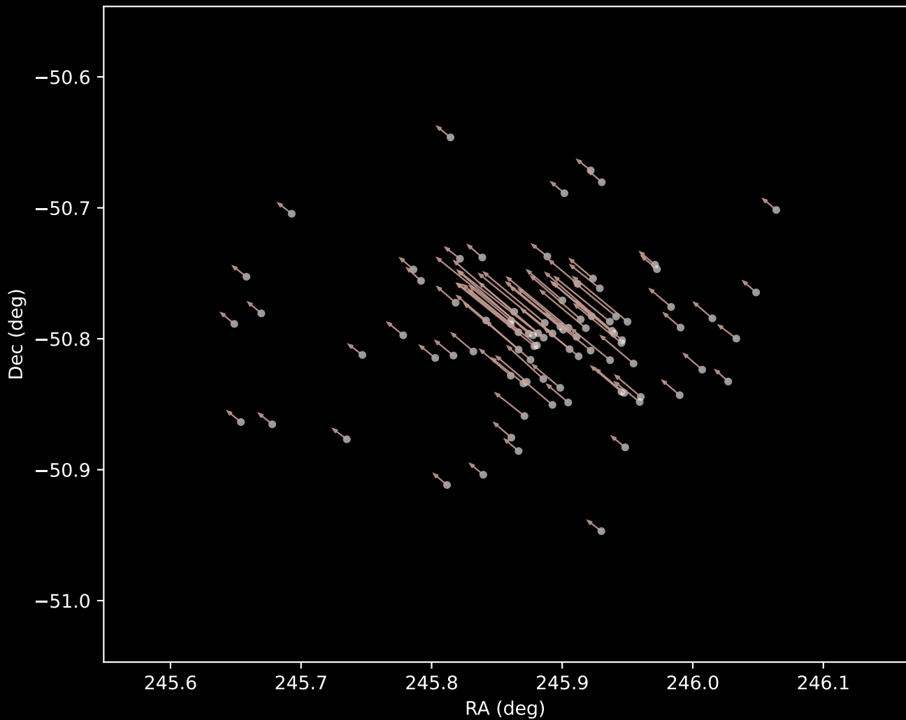
Gaia DR3 Cluster 11 Proper Motion Vectors (n=89)
