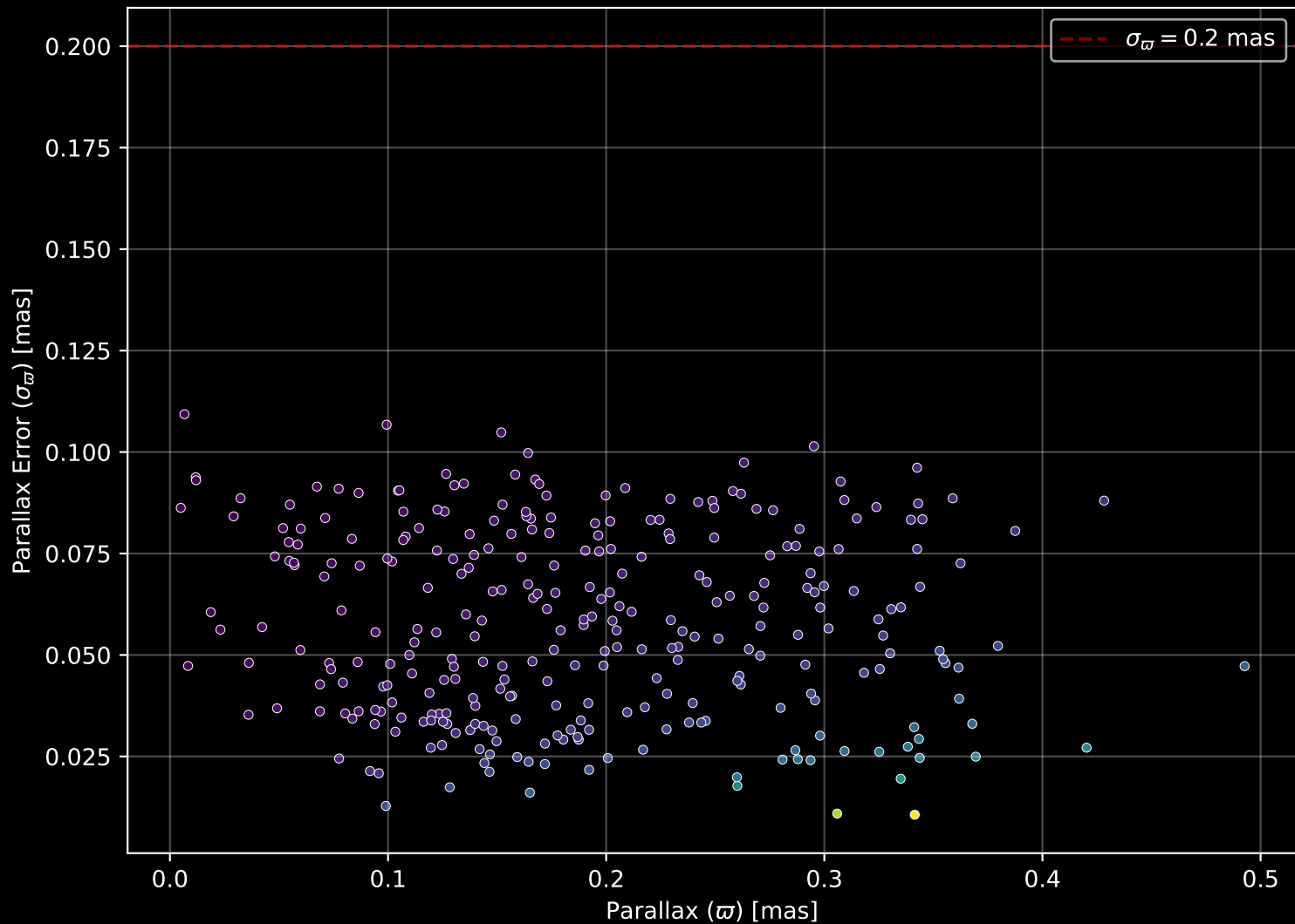
Gaia Cluster: [SAI_109] Parallax Quality (n= 298)
