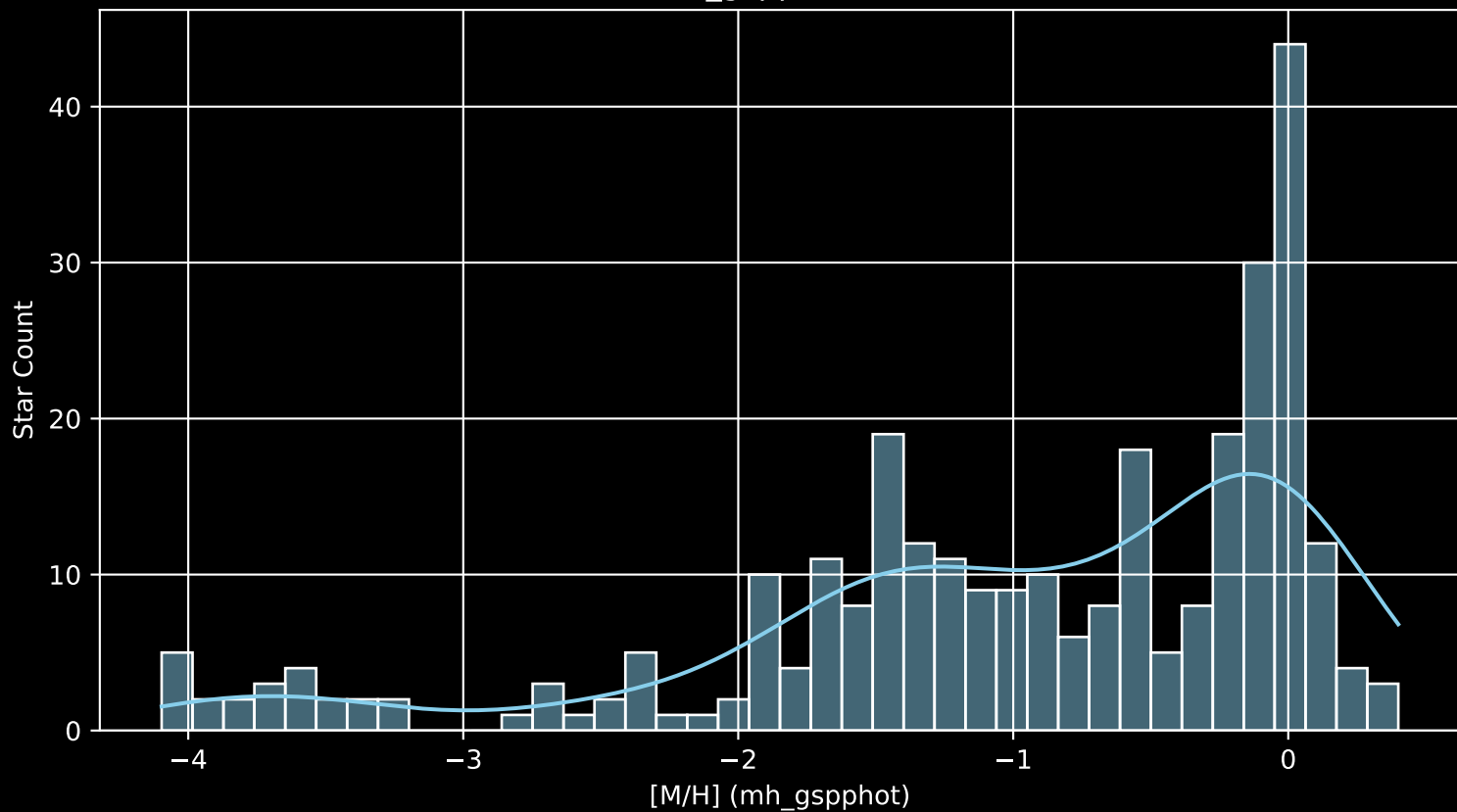
Gaia Cluster: [SAI_109 [M/H] (mh_gspphot) (n= 298)
