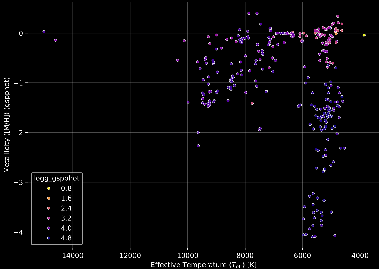
Gaia Cluster: [SAI_109] Stellar Population Parameters (n= 298)
