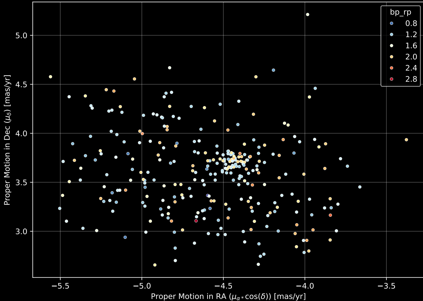
Gaia Cluster: [SAI_109] Proper Motion Diagram (n = 298)
