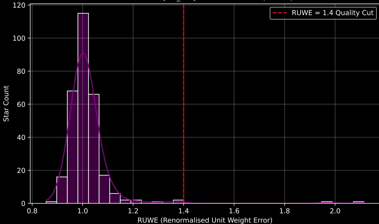
Gaia Cluster: [SAI_109] RUWE Distribution (n= 298)
