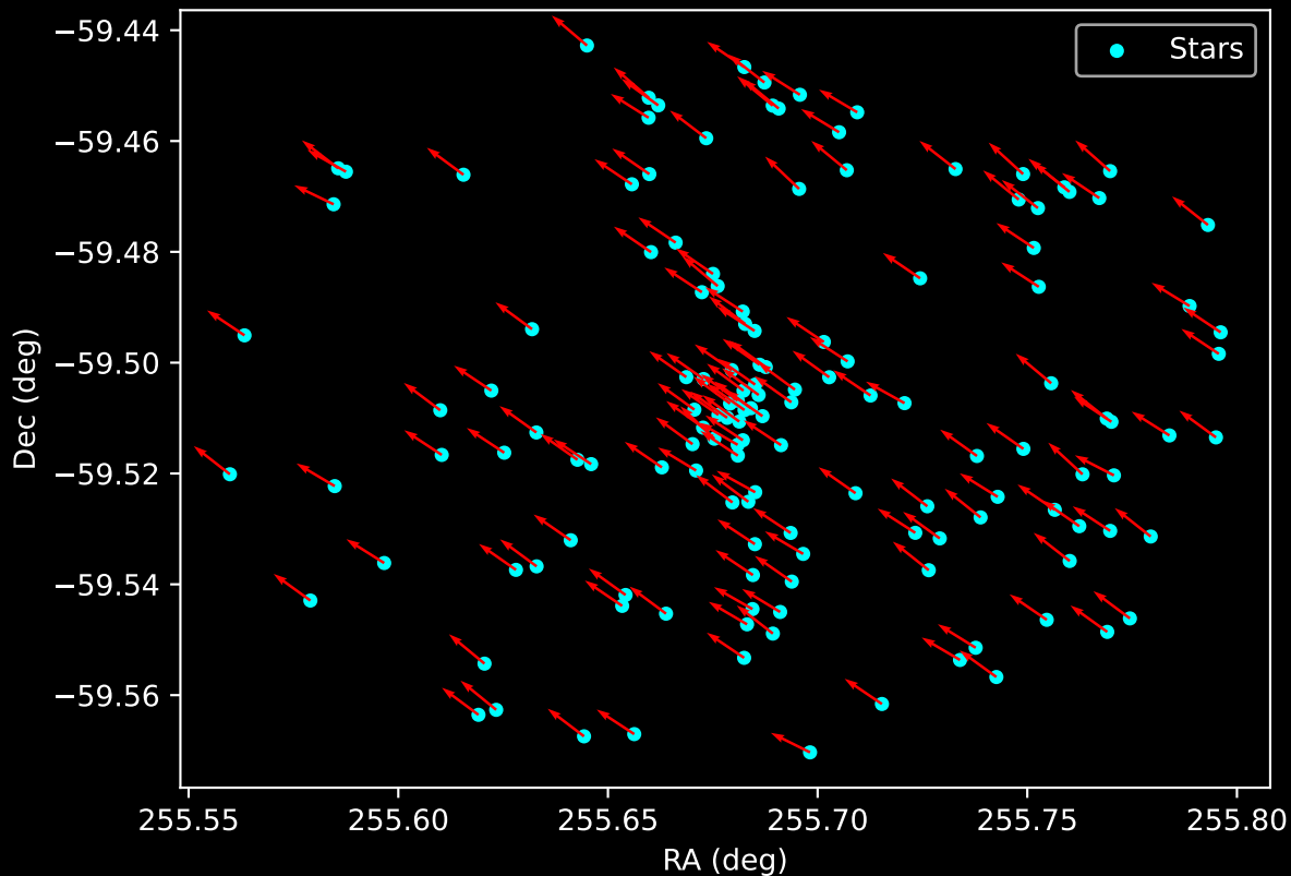
Gaia Cluster: [SAI_113] Proper Motion Vectors for Gaia Star Field (n= 142)
