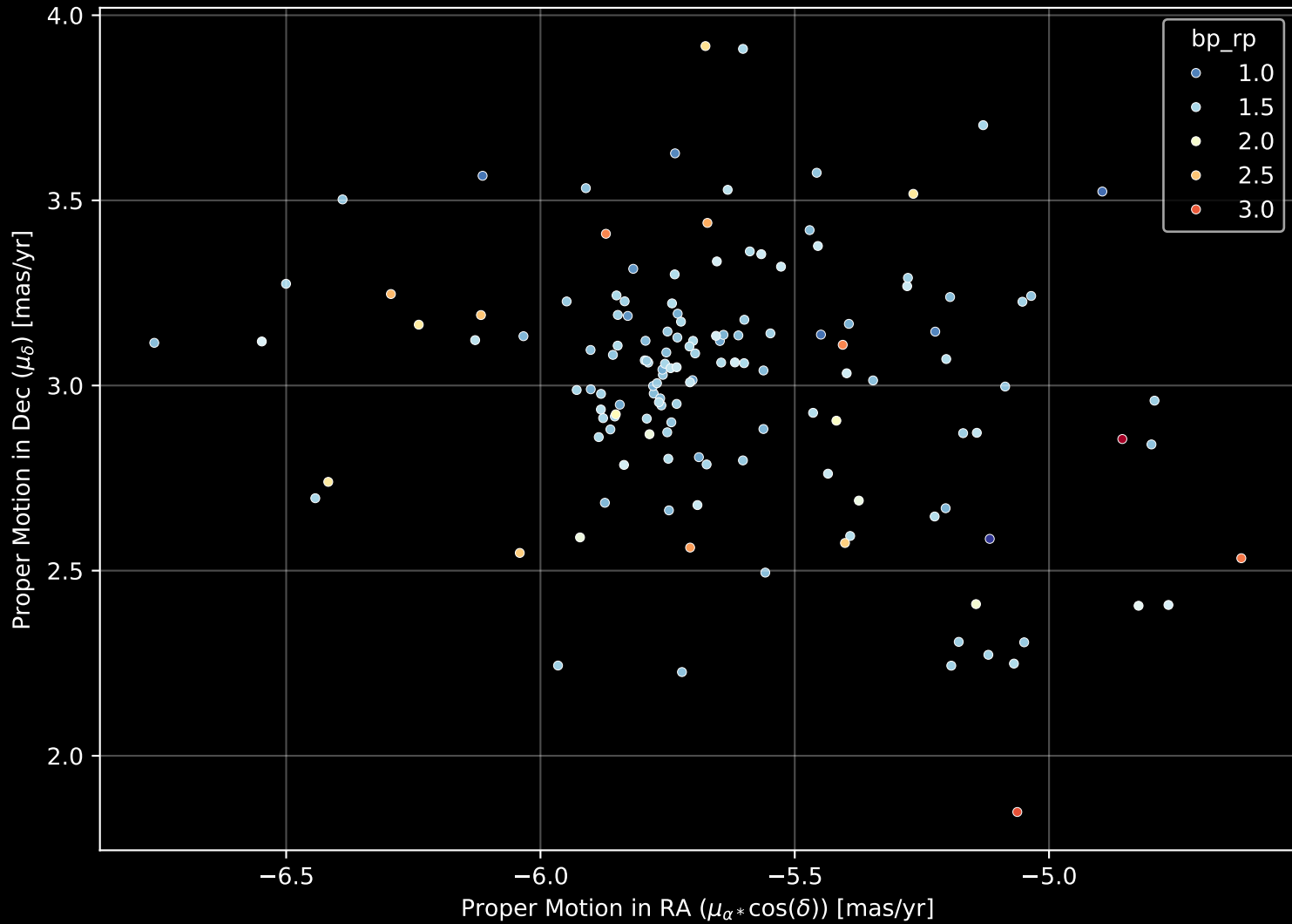
Gaia Cluster: [SAI_113] Proper Motion Diagram (n= 142)
