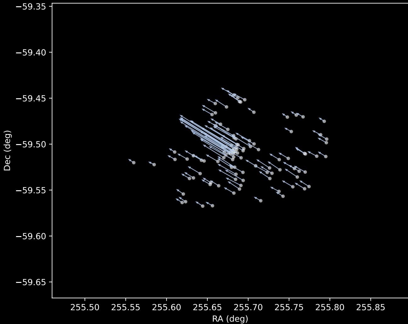
Gaia DR3 Cluster 1 Proper Motion Vectors (n=103)
