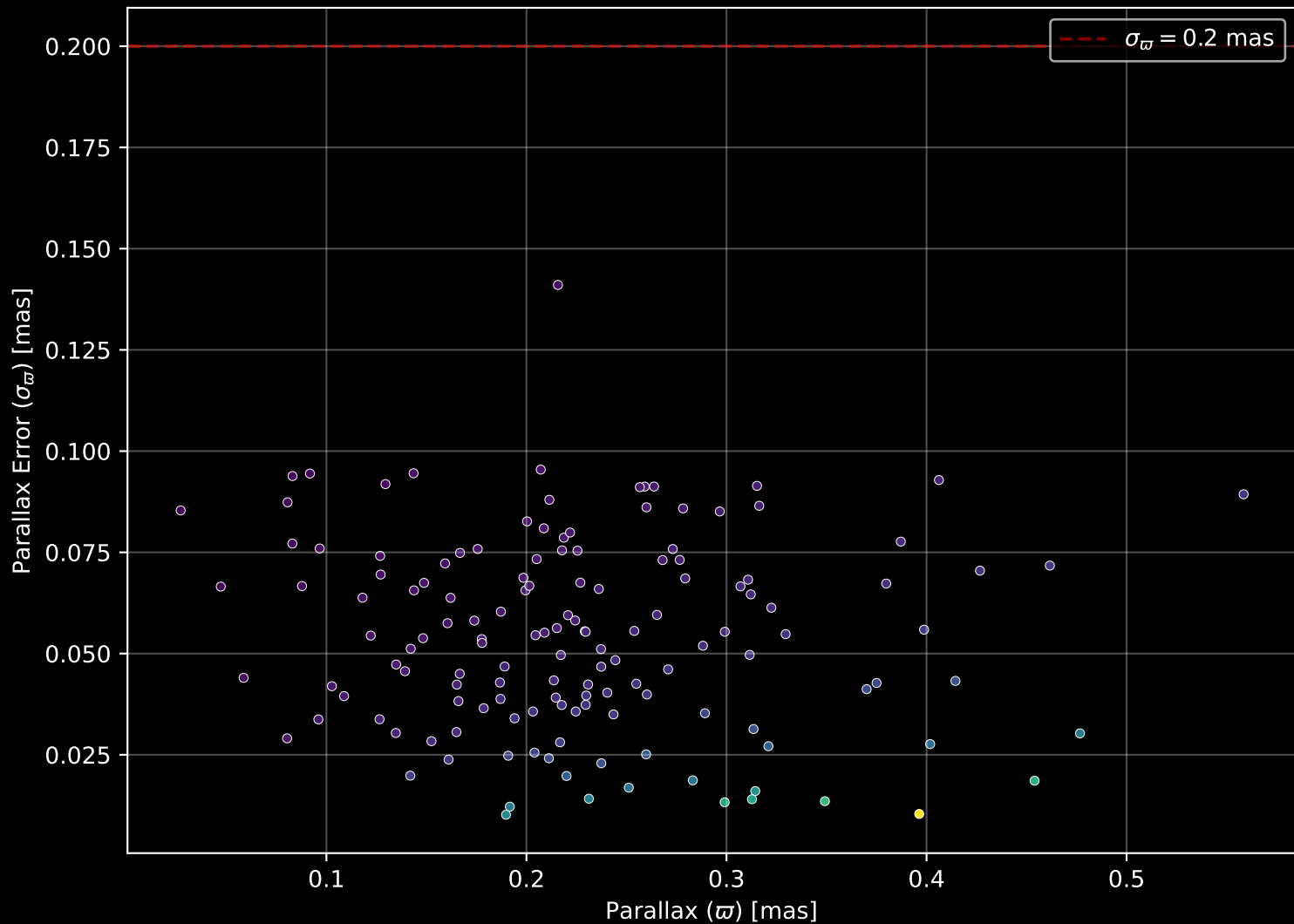
Gaia Cluster: [SAI_113] Parallax Quality (n= 142)
