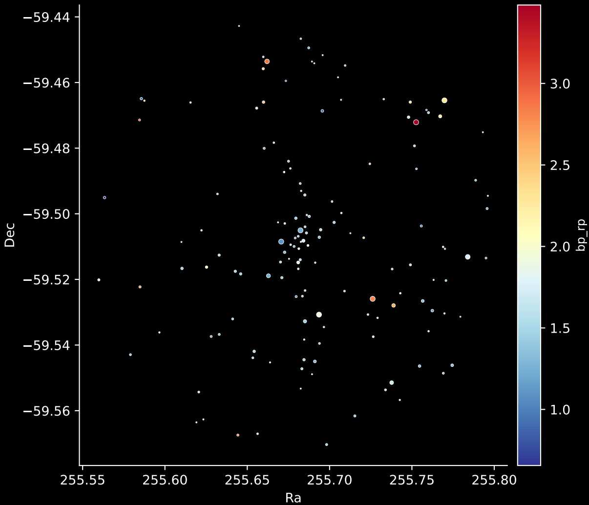
Gaia Cluster: [SAI_113] Stars: 142
