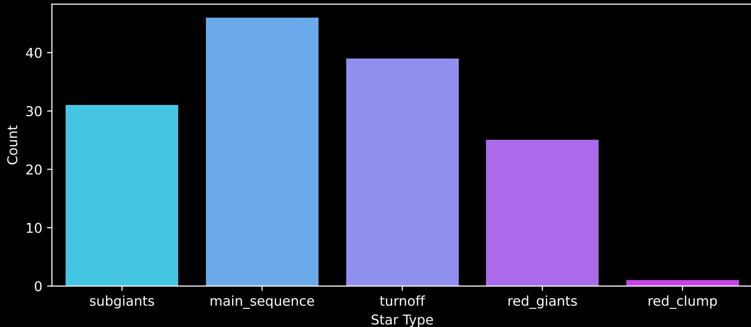
Gaia Cluster: [SAI_113] Count plot of Star Type
