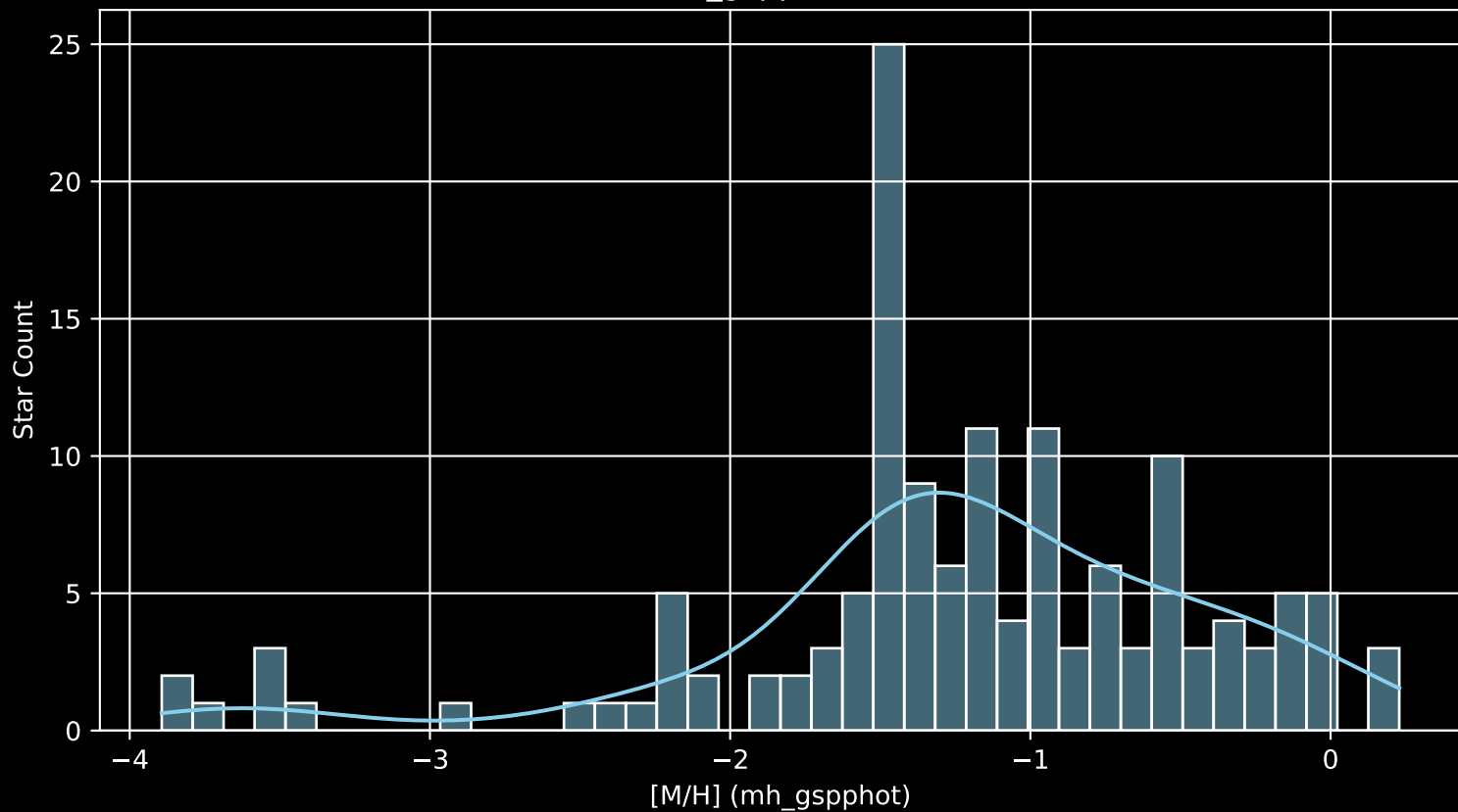
Gaia Cluster: [SAI_113 [M/H] (mh_gspphot) (n= 141)
