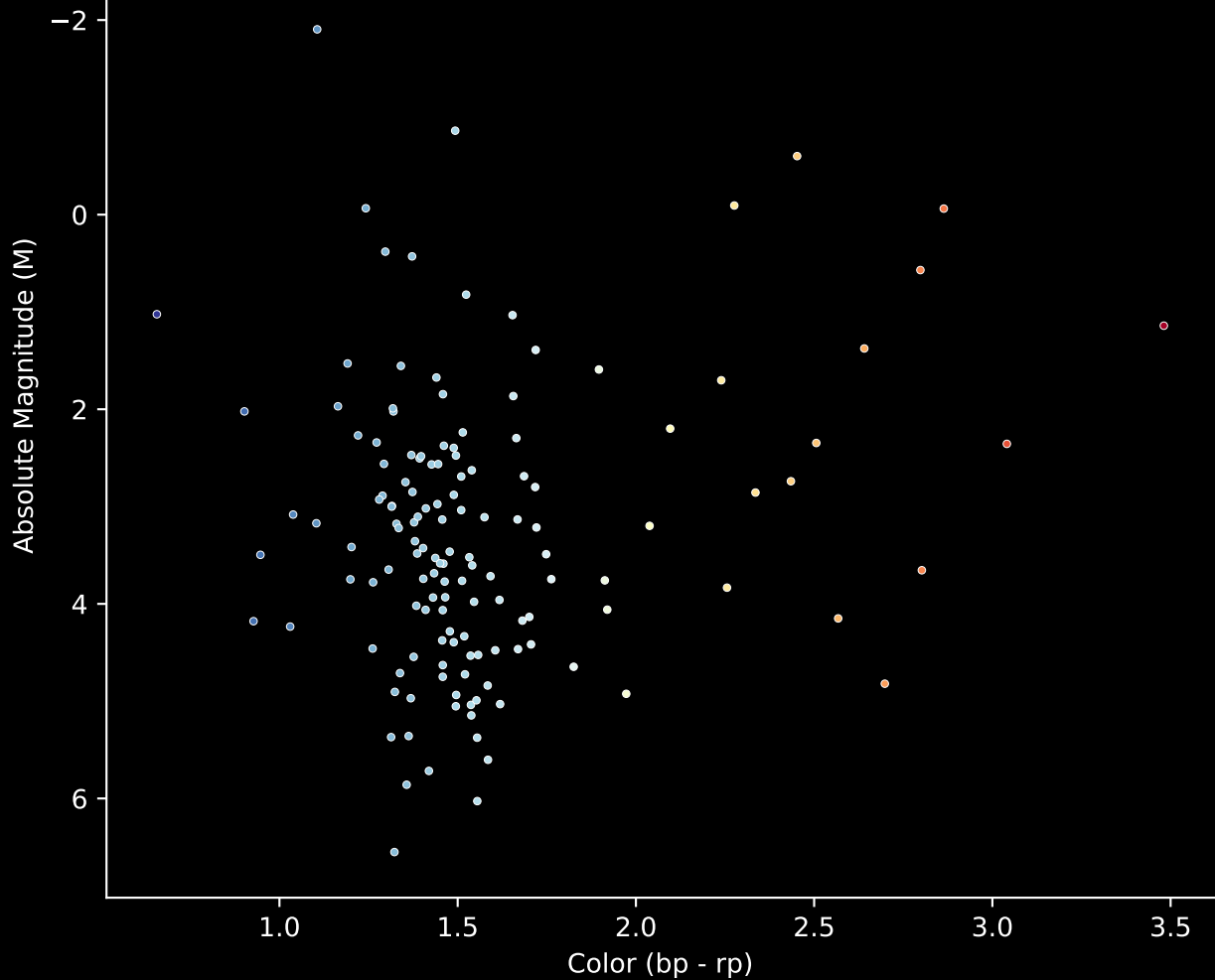
Gaia Cluster: [SAI_113] Stars (n= 142) Hertzsprung-Russel Diagram
