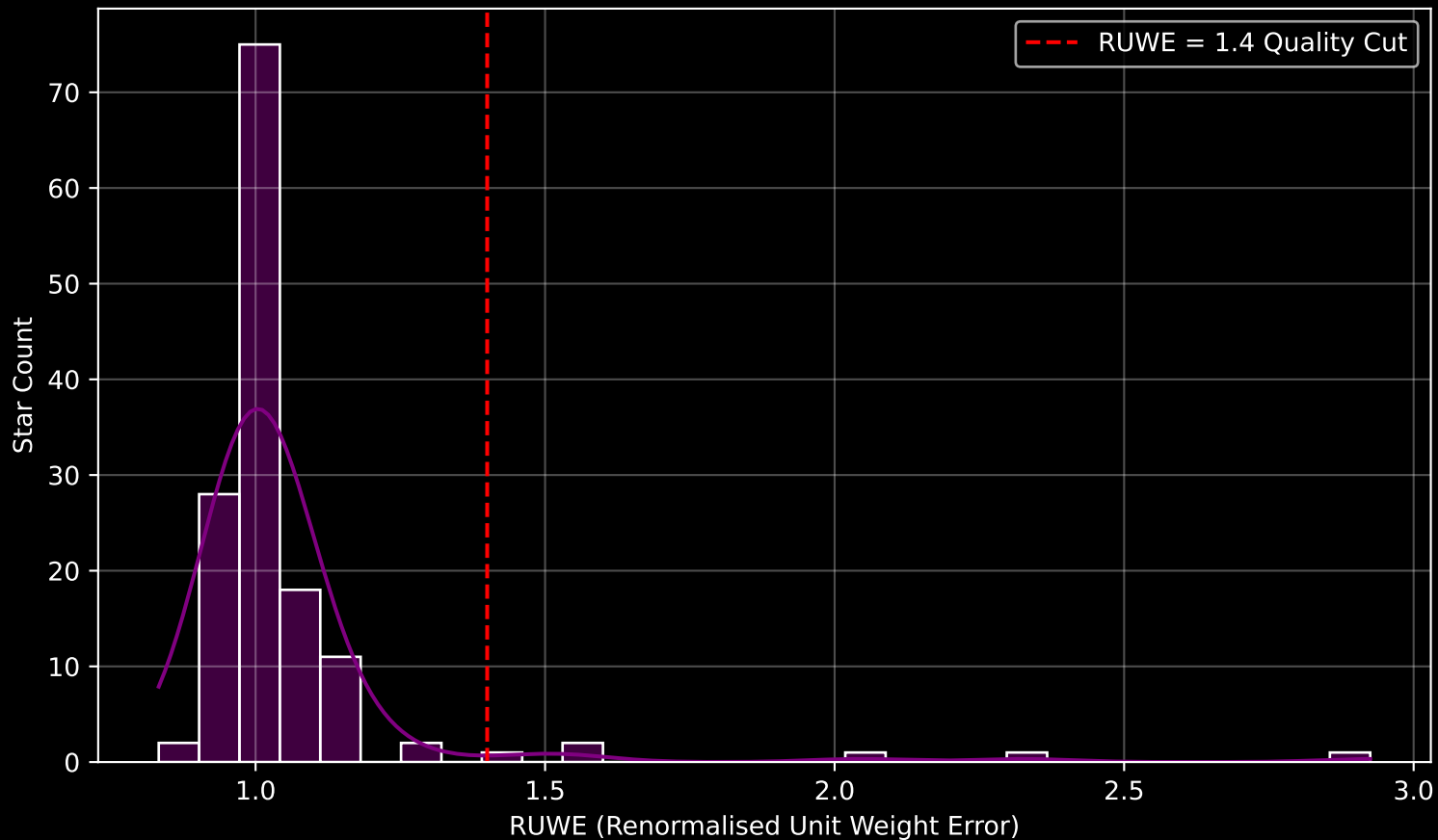
Gaia Cluster: [SAI_113] RUWE Distribution (n= 142)
