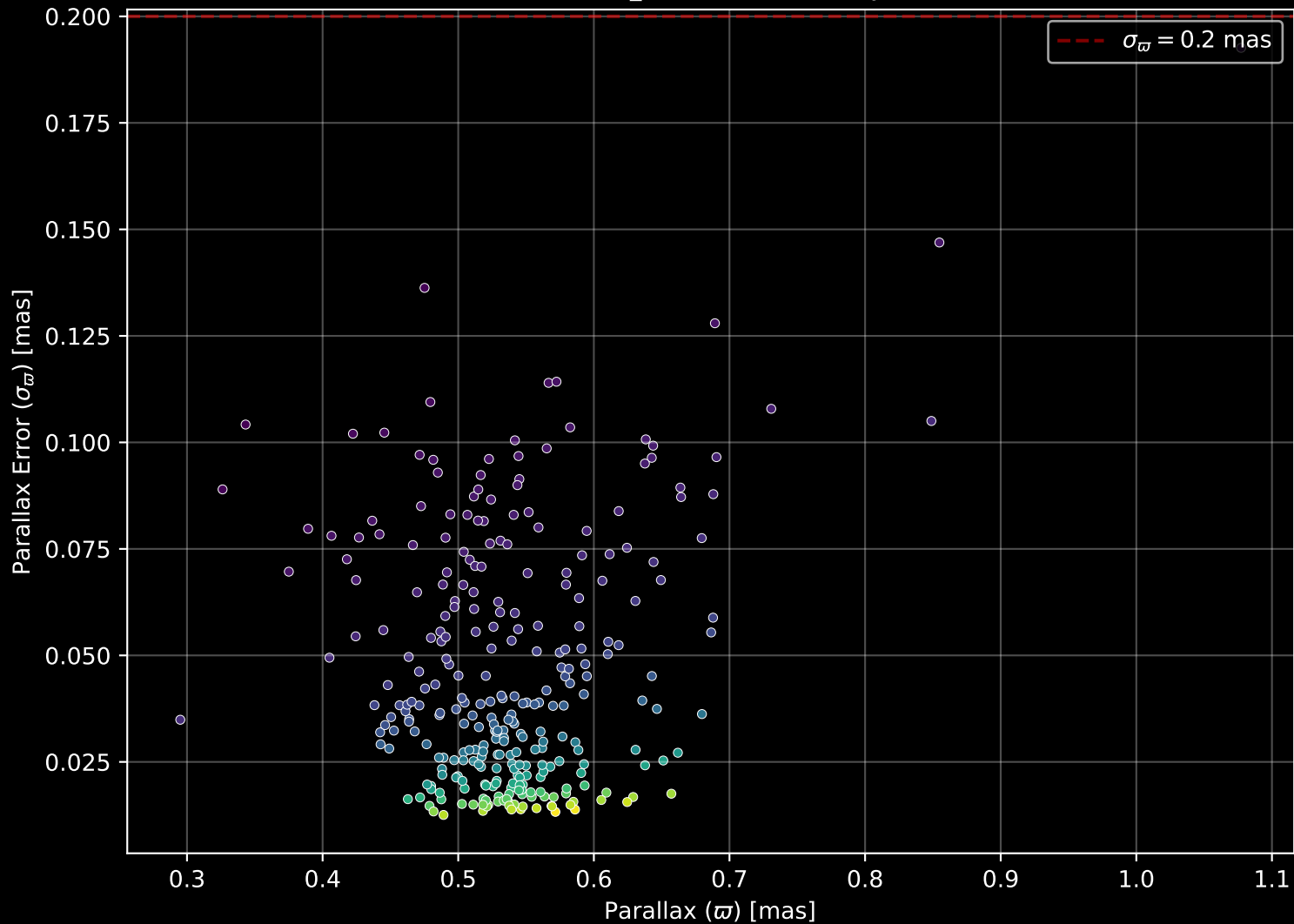
Gaia Cluster: [SAI_118] Parallax Quality (n= 293)
