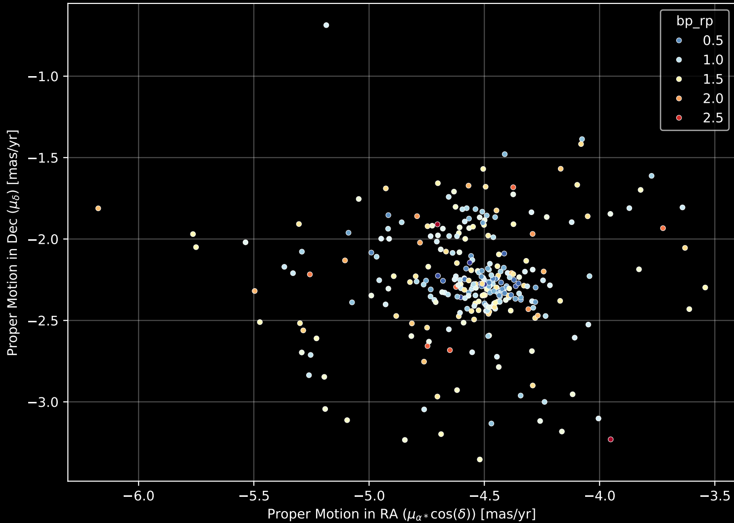
Gaia Cluster: [SAI_118] Proper Motion Diagram (n= 293)
