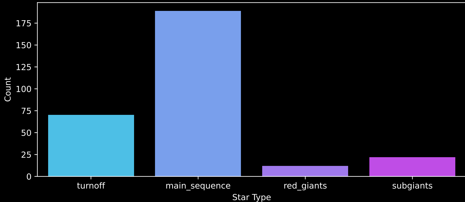
Gaia Cluster: [SAI_118] Count plot of Star Type
