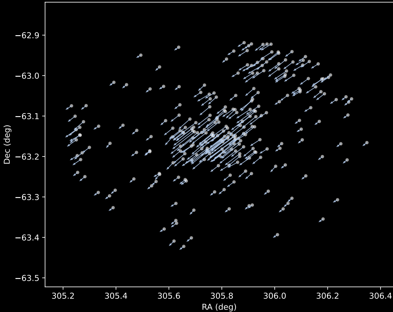
Gaia DR3 Cluster 1 Proper Motion Vectors (n=252)
