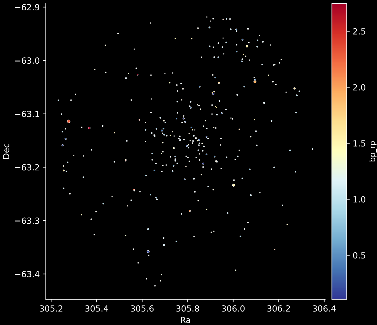
Gaia Cluster: [SAI_118] Stars: 293
