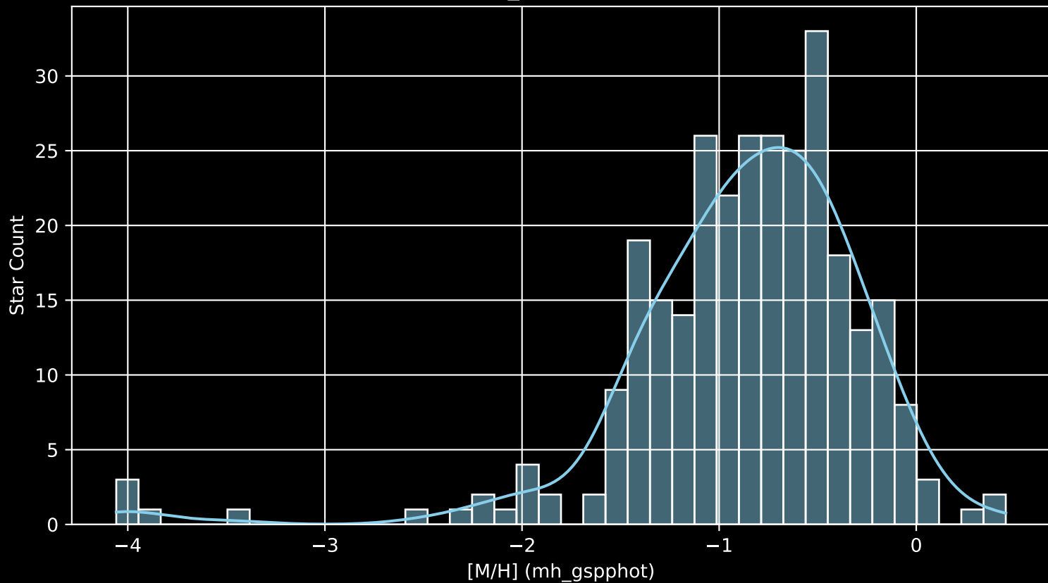
Gaia Cluster: [SAI_118 [M/H] (mh_gspphot) (n= 293)
