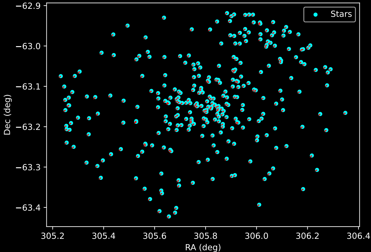
Gaia Cluster: [SAI_118] Proper Motion Vectors for Gaia Star Field (n= 293)
