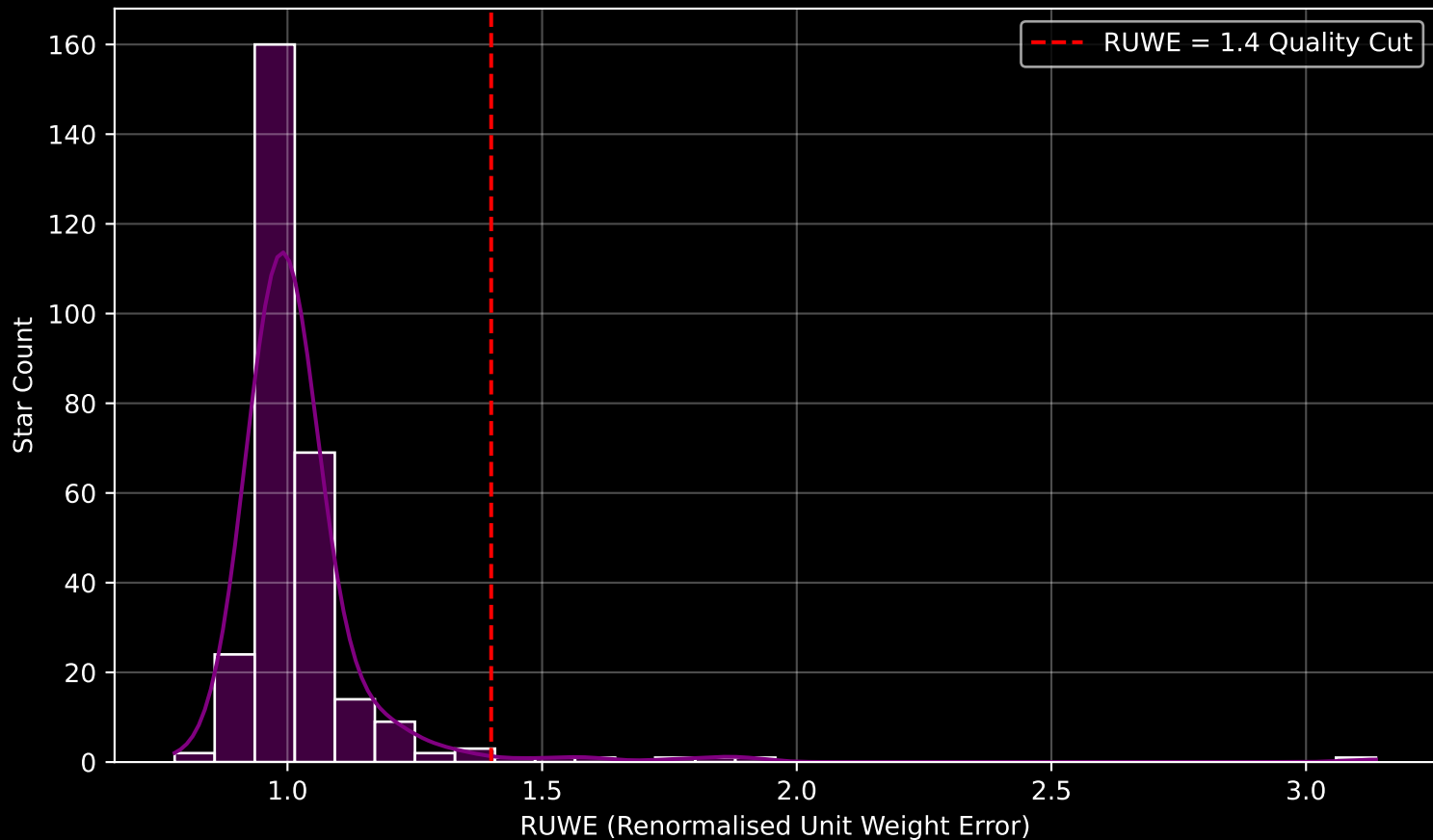
Gaia Cluster: [SAI_118] RUWE Distribution (n= 290)
