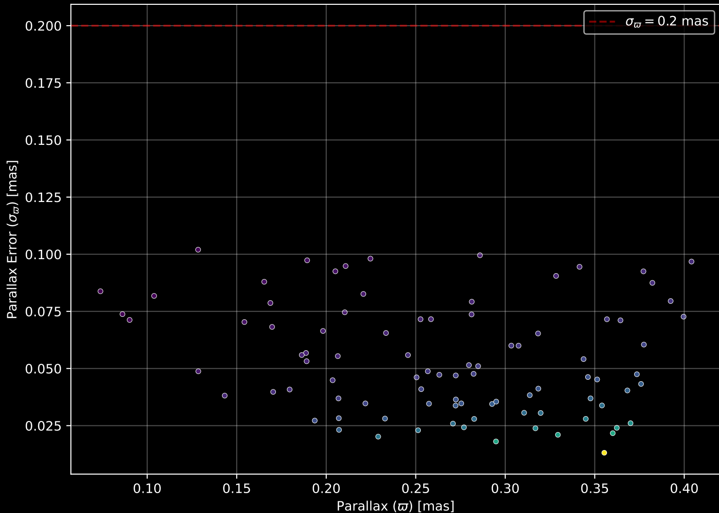
Gaia Cluster: [SAI_14] Parallax Quality (n= 90)
