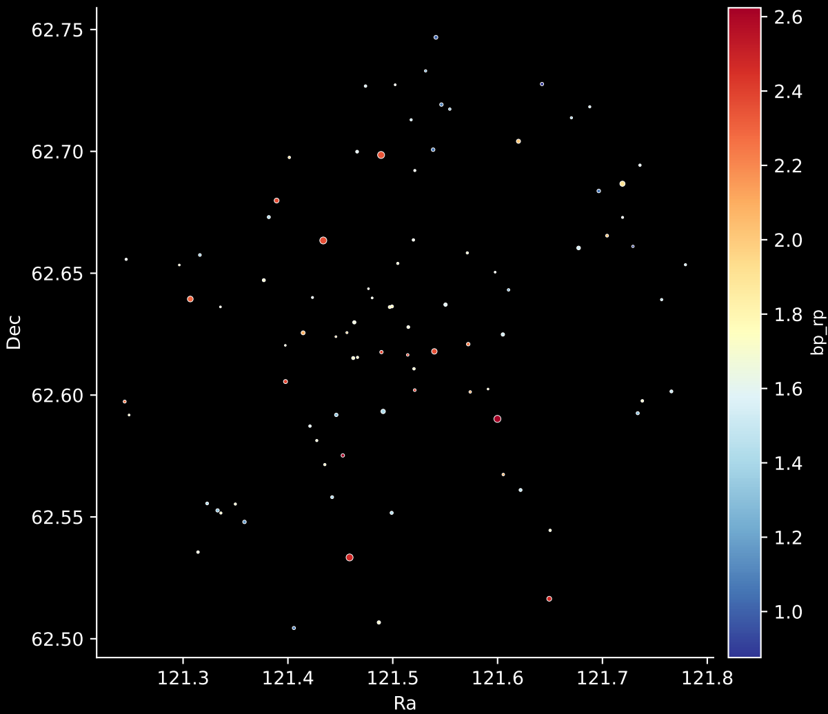
Gaia Cluster: [SAI_14] Stars: 90
