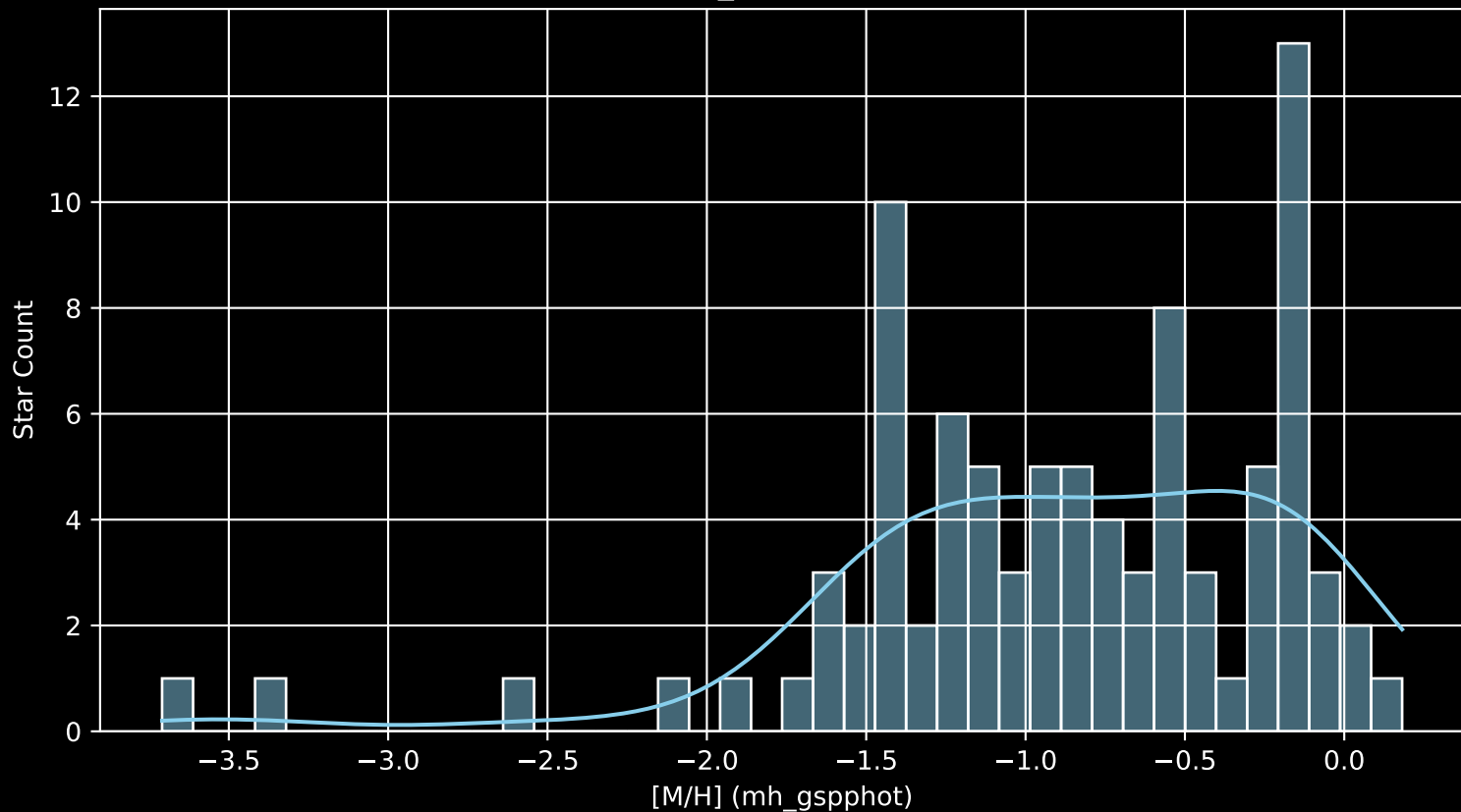
Gaia Cluster: [SAI_14 [M/H] (mh_gspphot) (n= 90)
