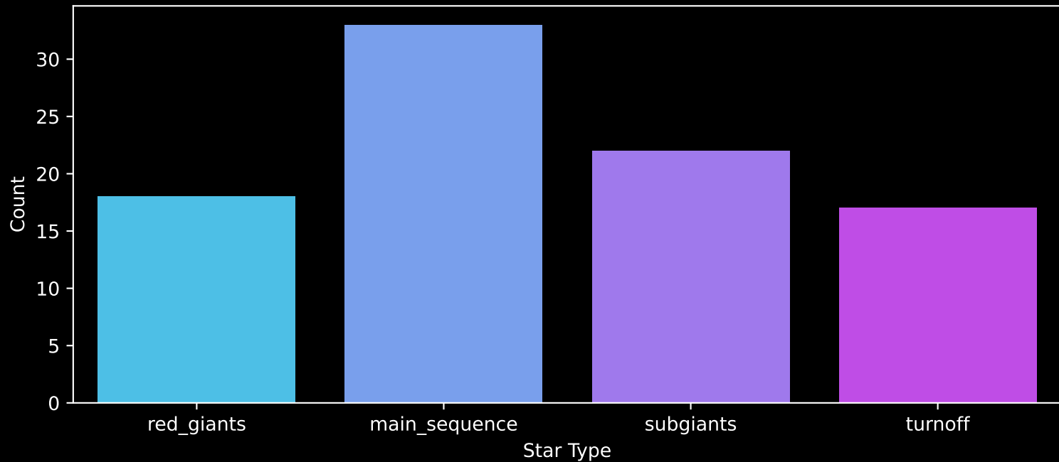
Gaia Cluster: [SAI_14] Count plot of Star Type
