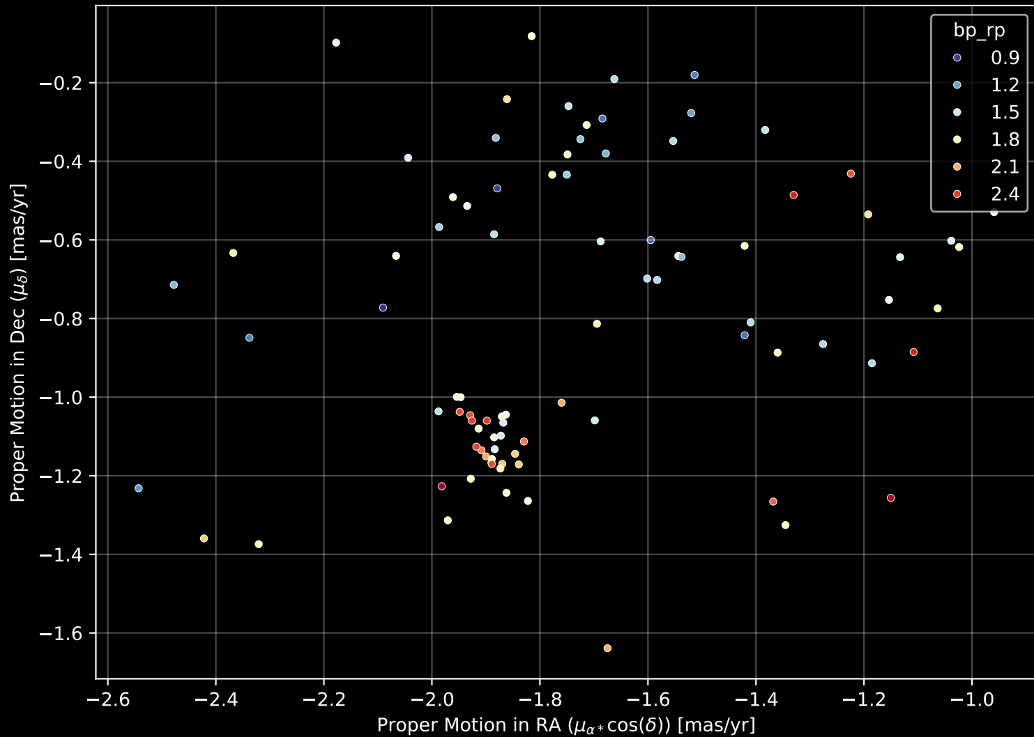
Gaia Cluster: [SAI_14] Proper Motion Diagram (n= 90)
