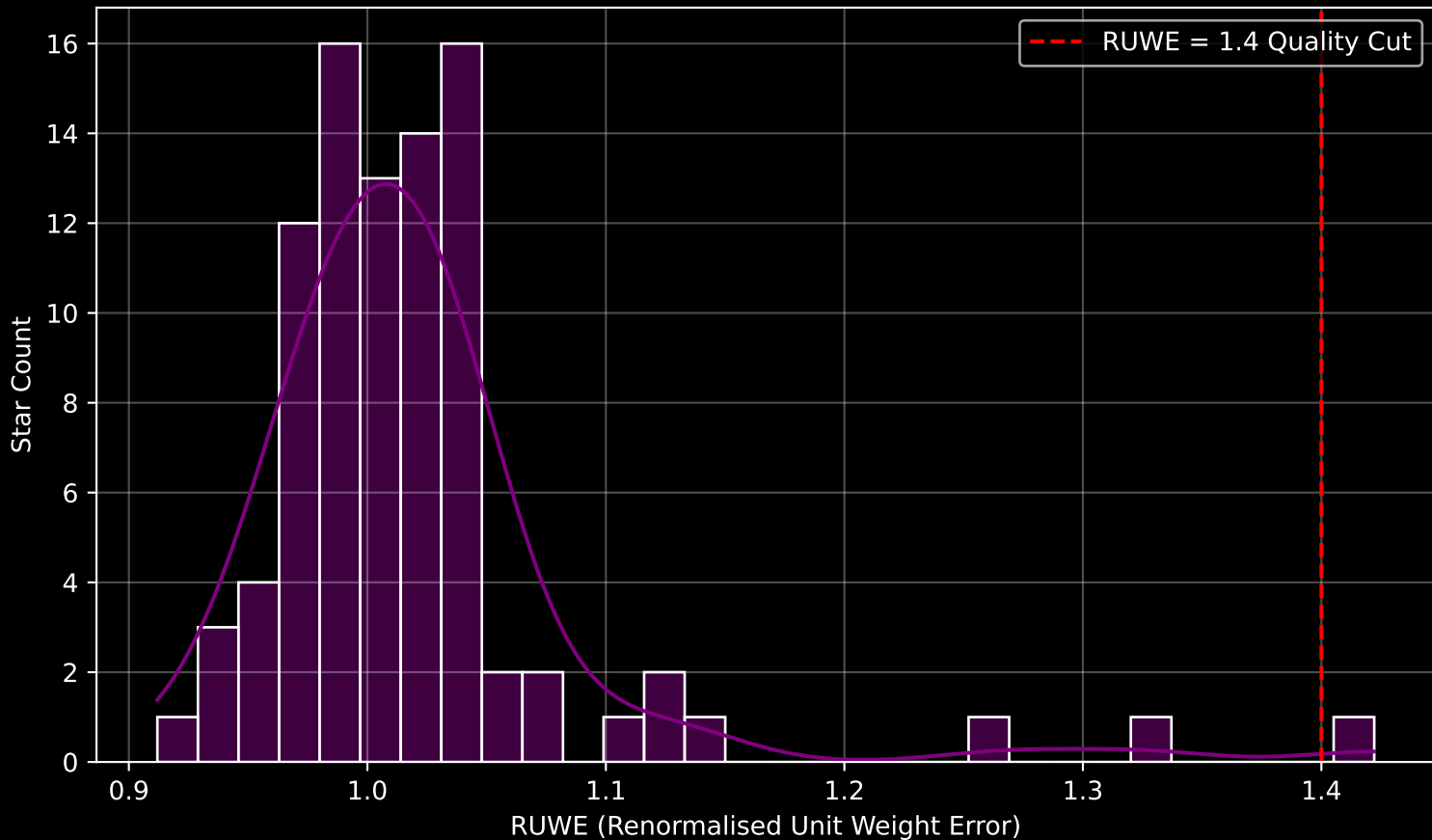
Gaia Cluster: [SAI_14] RUWE Distribution (n= 90)
