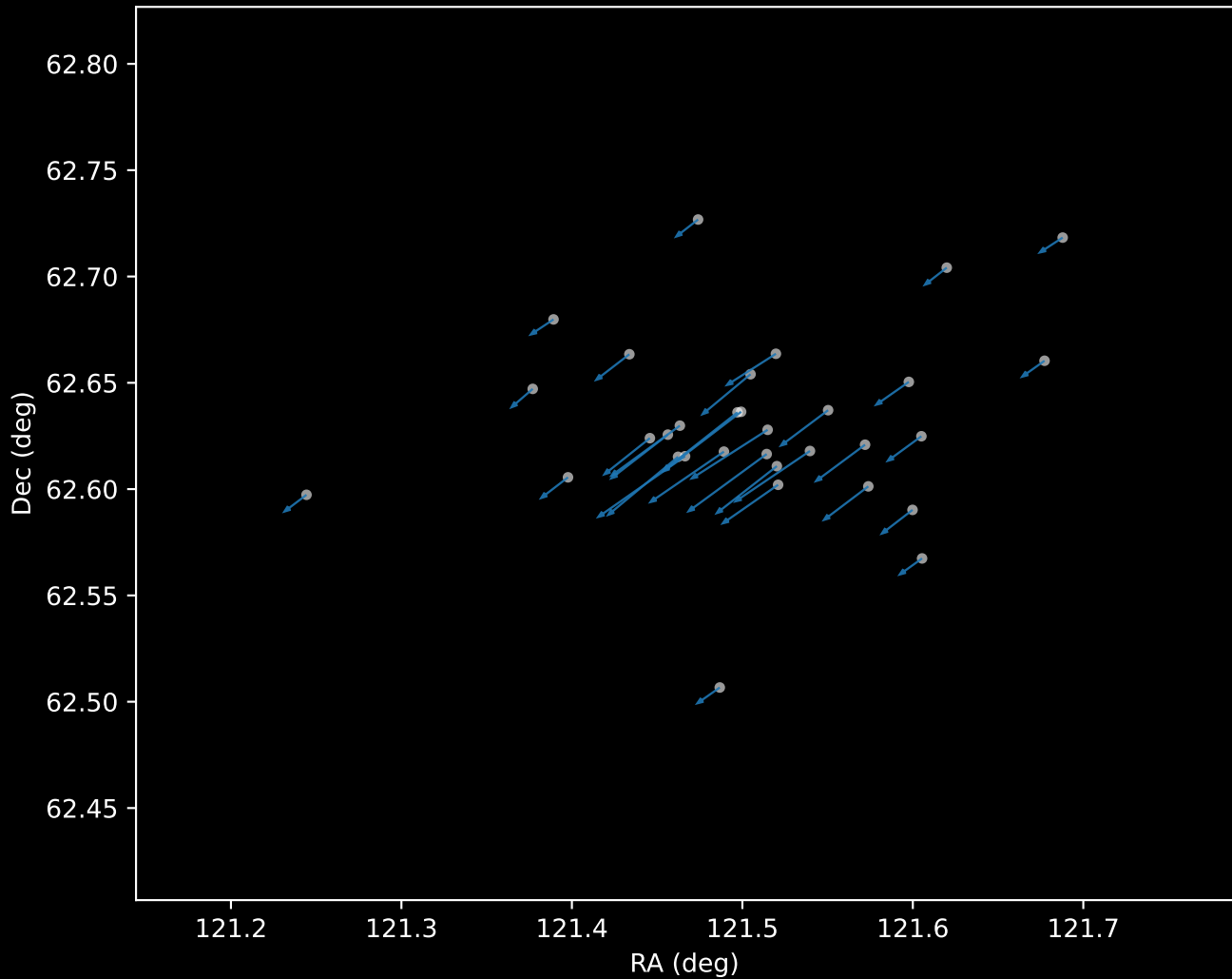
Gaia DR3 Cluster 0 Proper Motion Vectors (n=32)
