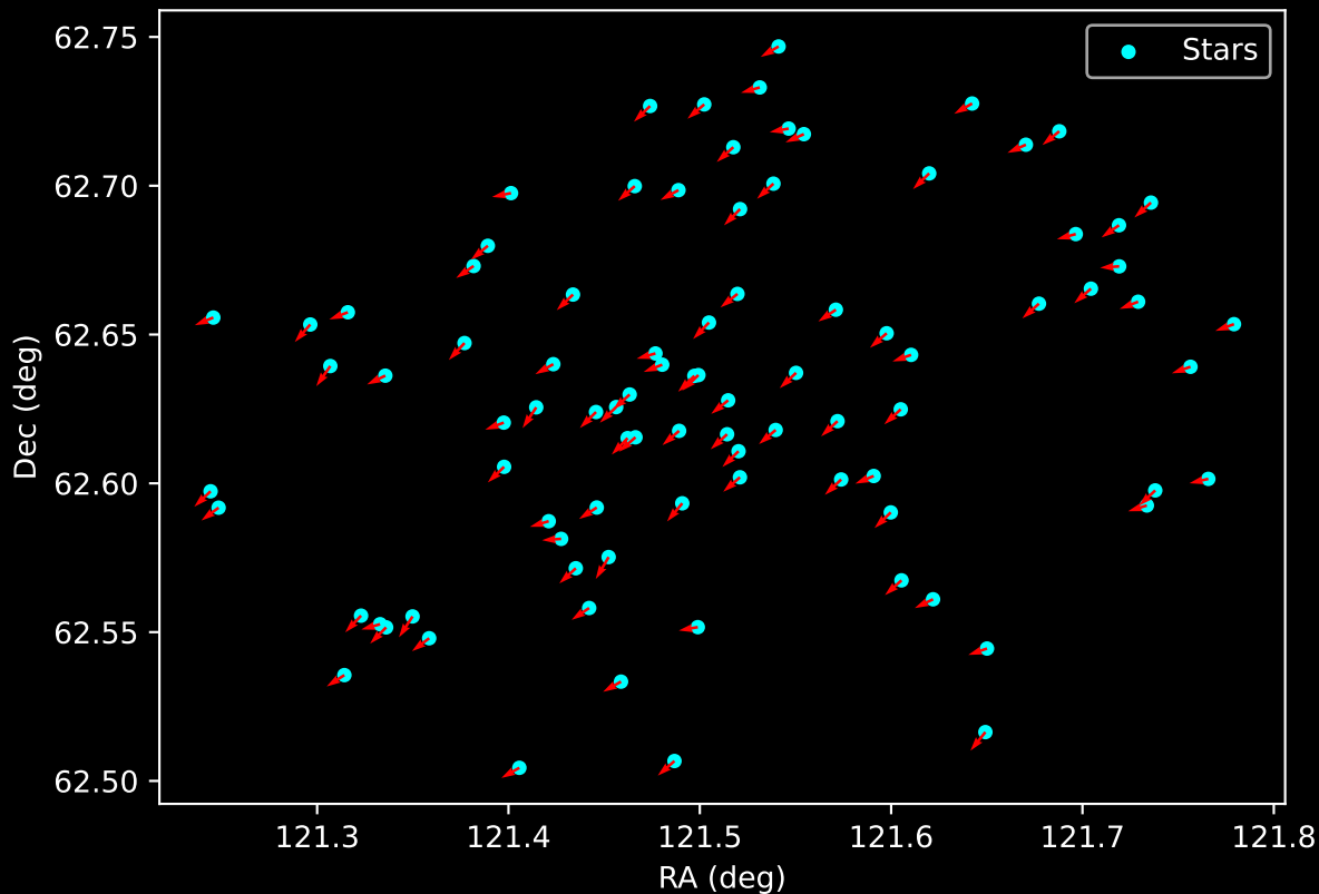
Gaia Cluster: [SAI_14] Proper Motion Vectors for Gaia Star Field (n= 90)
