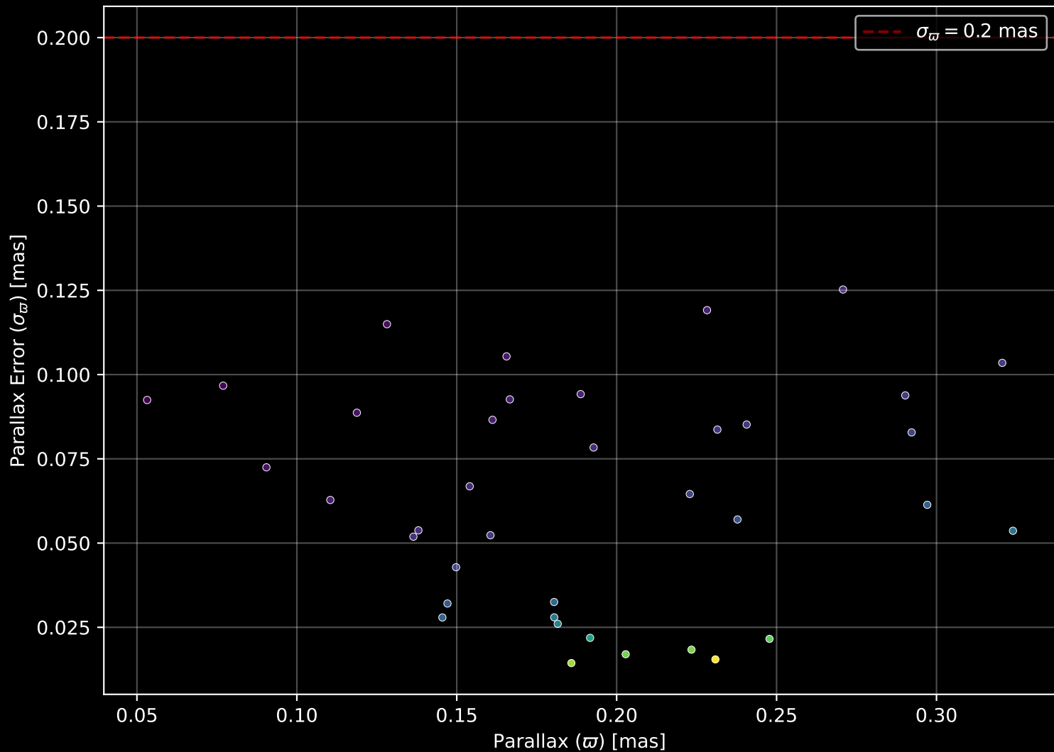
Gaia Cluster: [SAI_47] Parallax Quality (n= 38)
