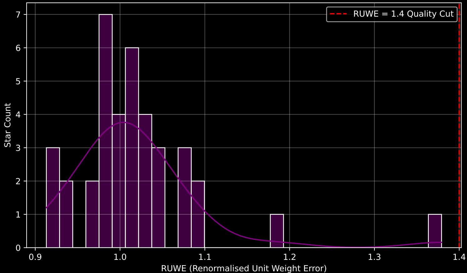
Gaia Cluster: [SAI_47] RUWE Distribution (n= 38)
