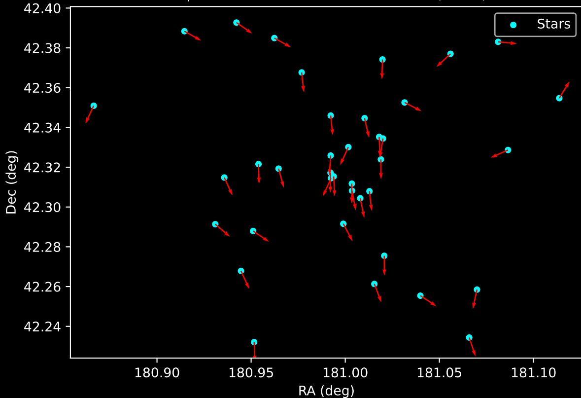
Gaia Cluster: [SAI_47] Proper Motion Vectors for Gaia Star Field (n= 38)
