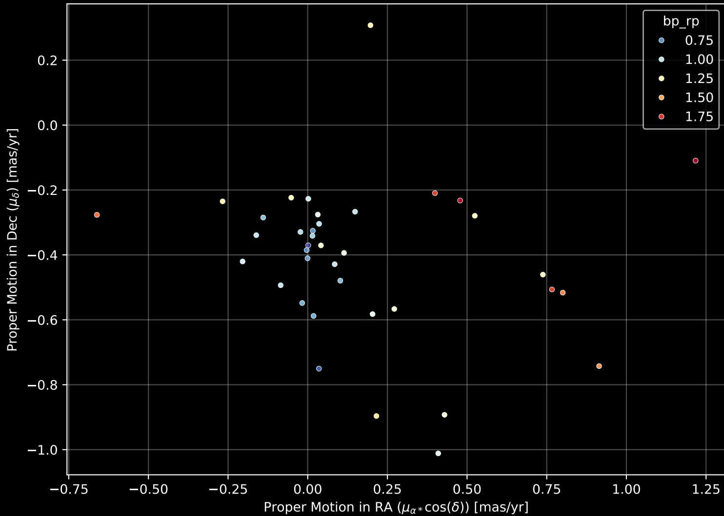
Gaia Cluster: [SAI_47] Proper Motion Diagram (n= 38)
