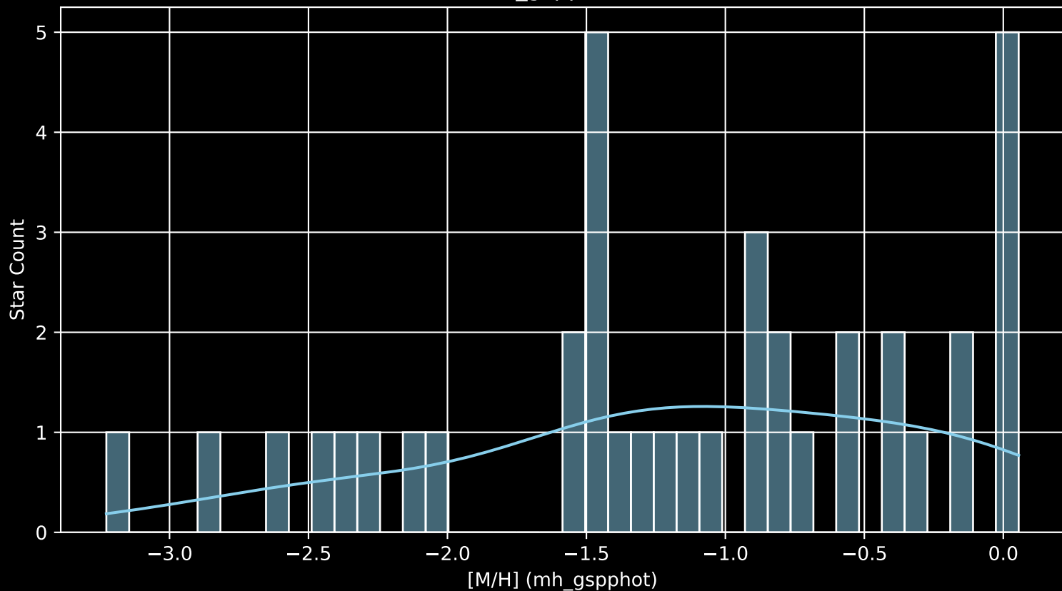
Gaia Cluster: [SAI_47 [M/H] (mh_gspphot) ( \bar{n}= 38 )
