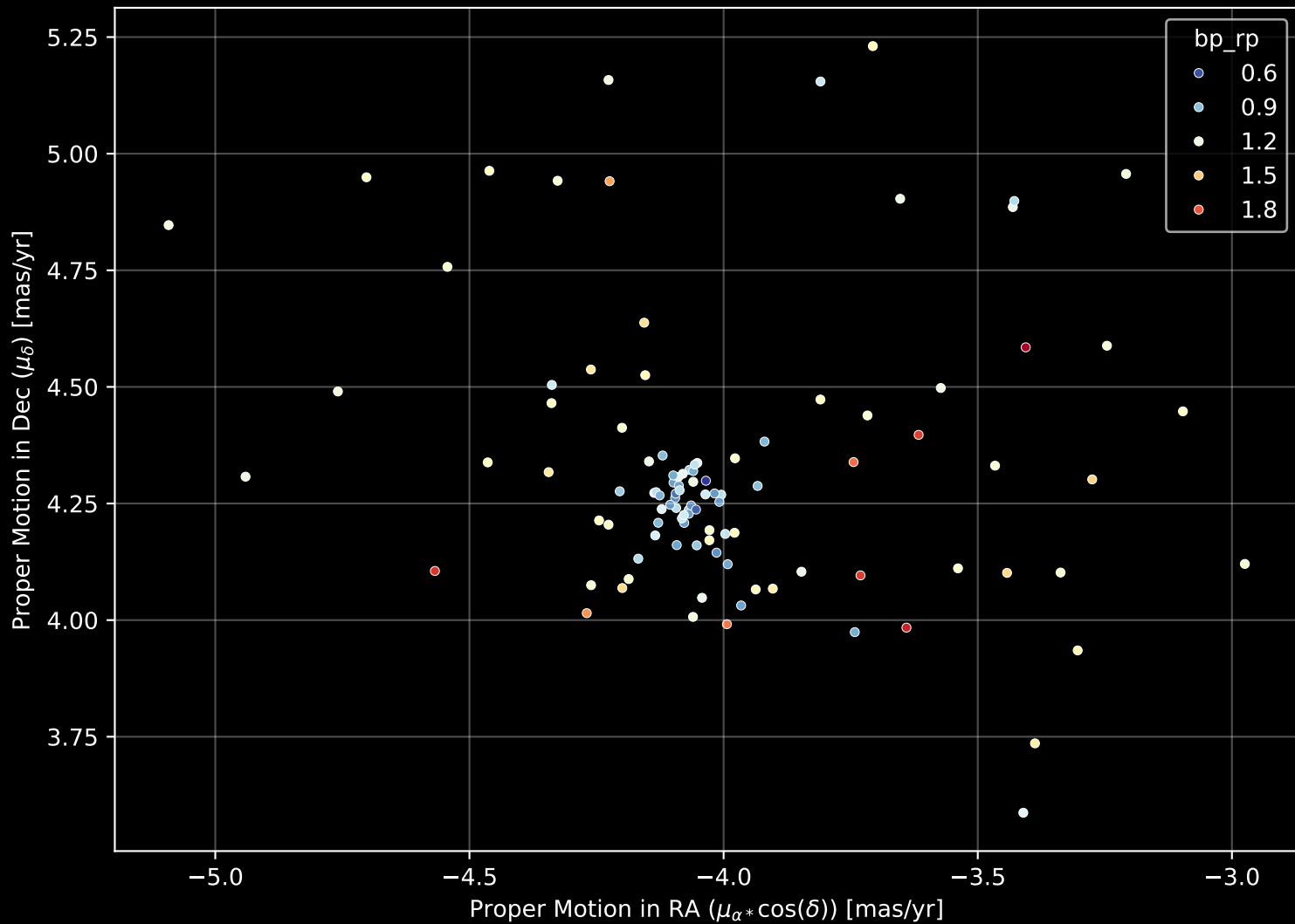
Gaia Cluster: [SAI_91] Proper Motion Diagram (n= 105)
