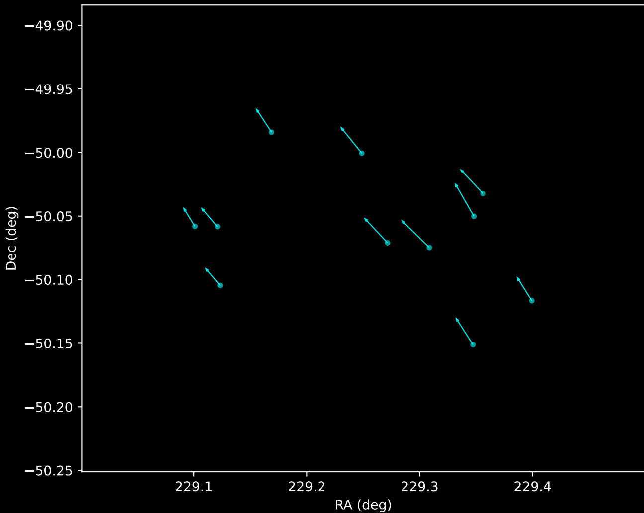
Gaia DR3 Noise Stream Proper Motion Vectors (n=11)
