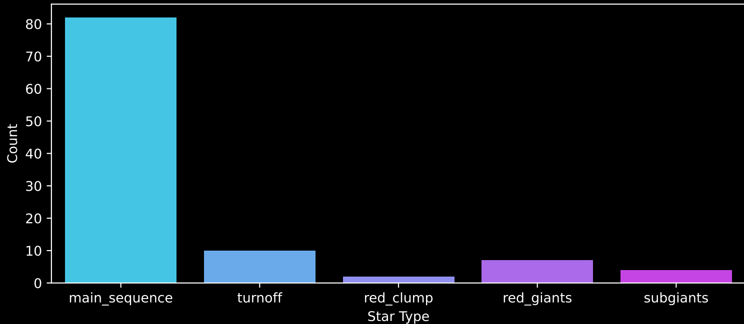
Gaia Cluster: [SAI_91] Count plot of Star Type
