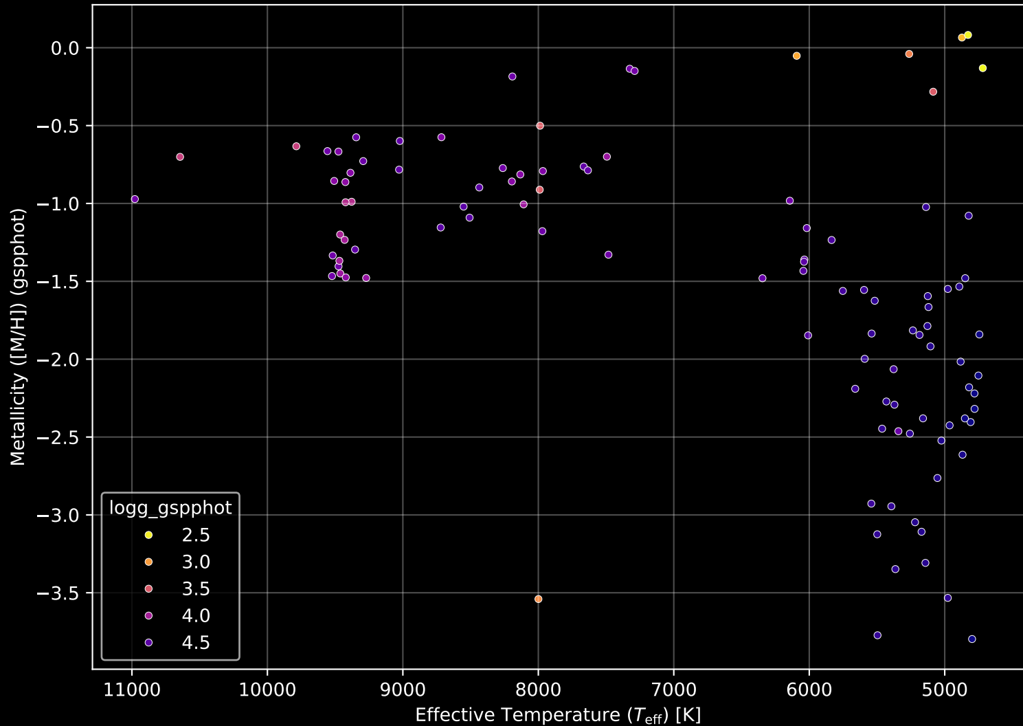
Gaia Cluster: [SAI_91] Stellar Population Parameters (n= 105)
