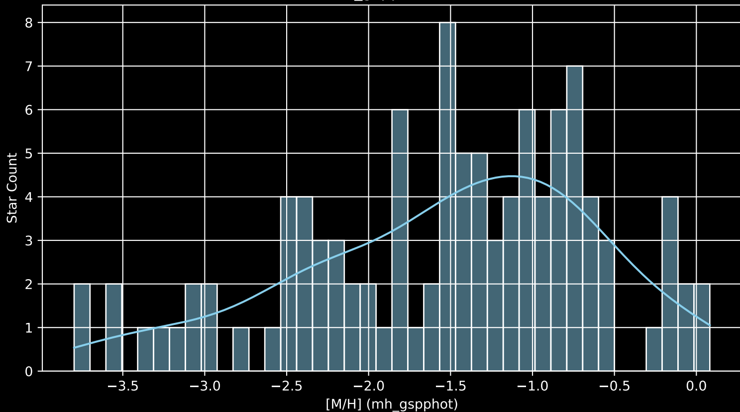
Gaia Cluster: [SAI_91 [M/H] (mh_gspphot) ( \bar{n}= 105 )
