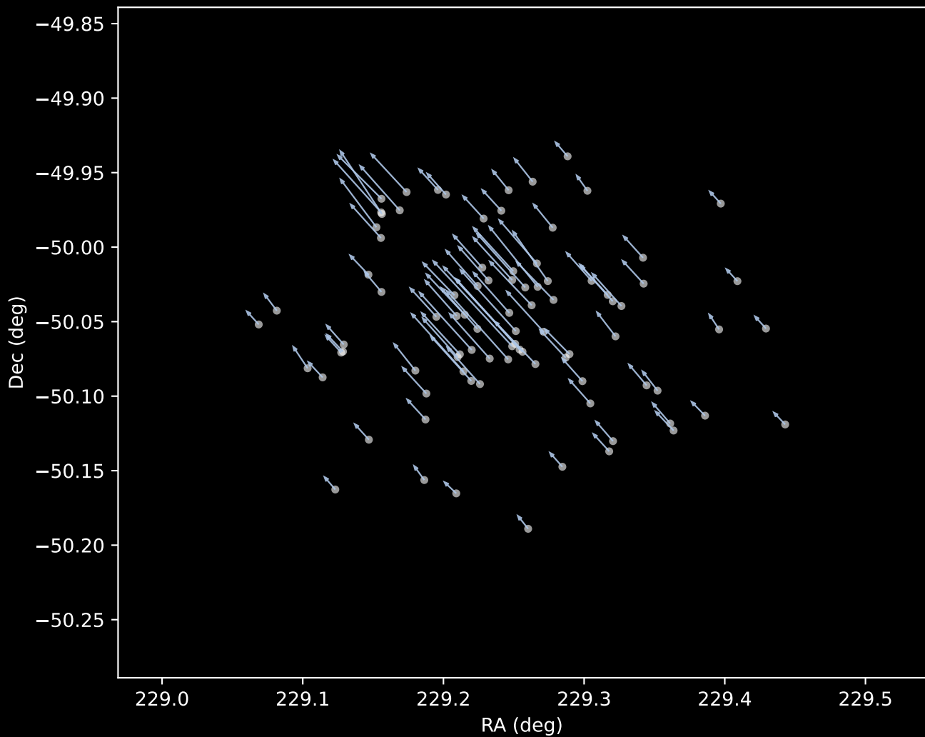
Gaia DR3 Cluster 1 Proper Motion Vectors (n=89)
