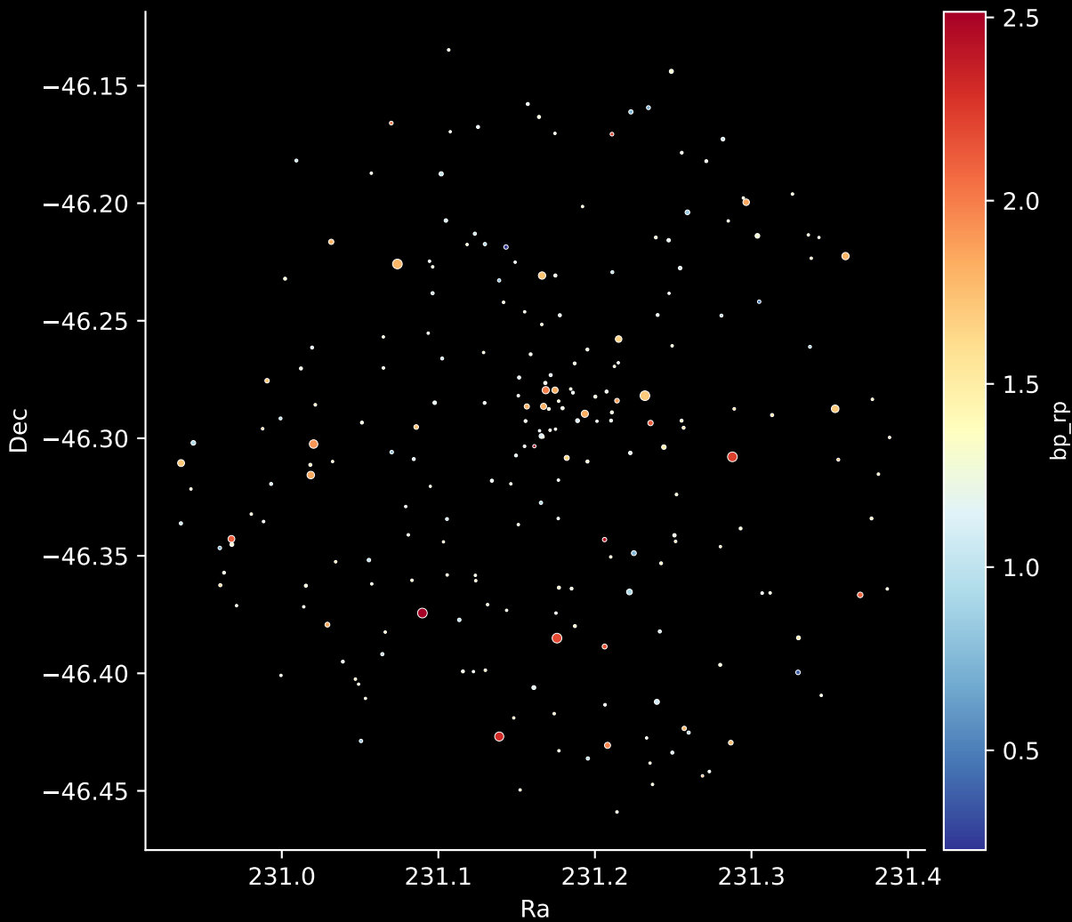
Gaia Cluster: [SAI_94] Stars: 225
