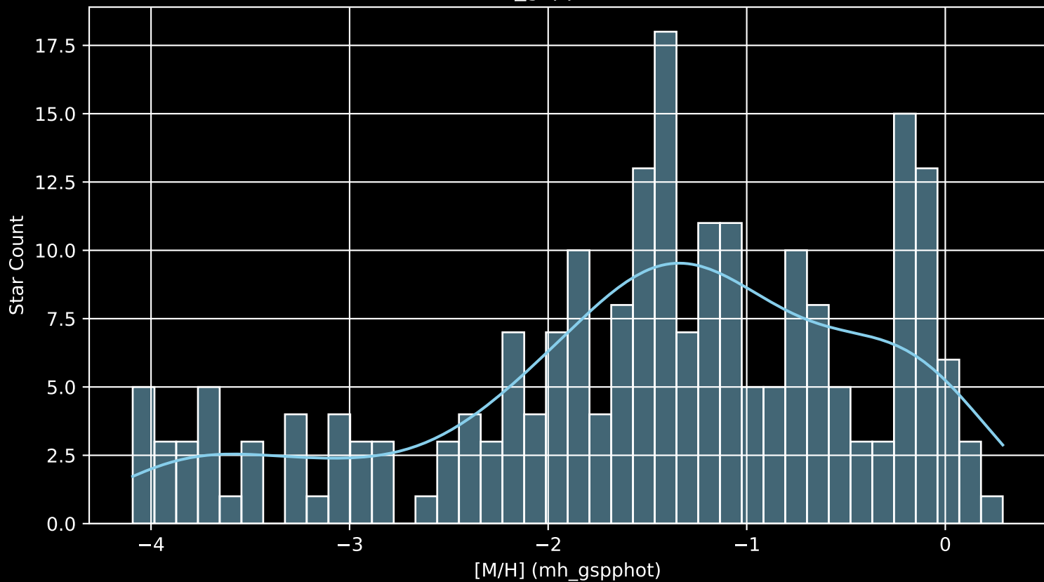
Gaia Cluster: [SAI_94 [M/H] (mh_gspphot) (n= 223)
