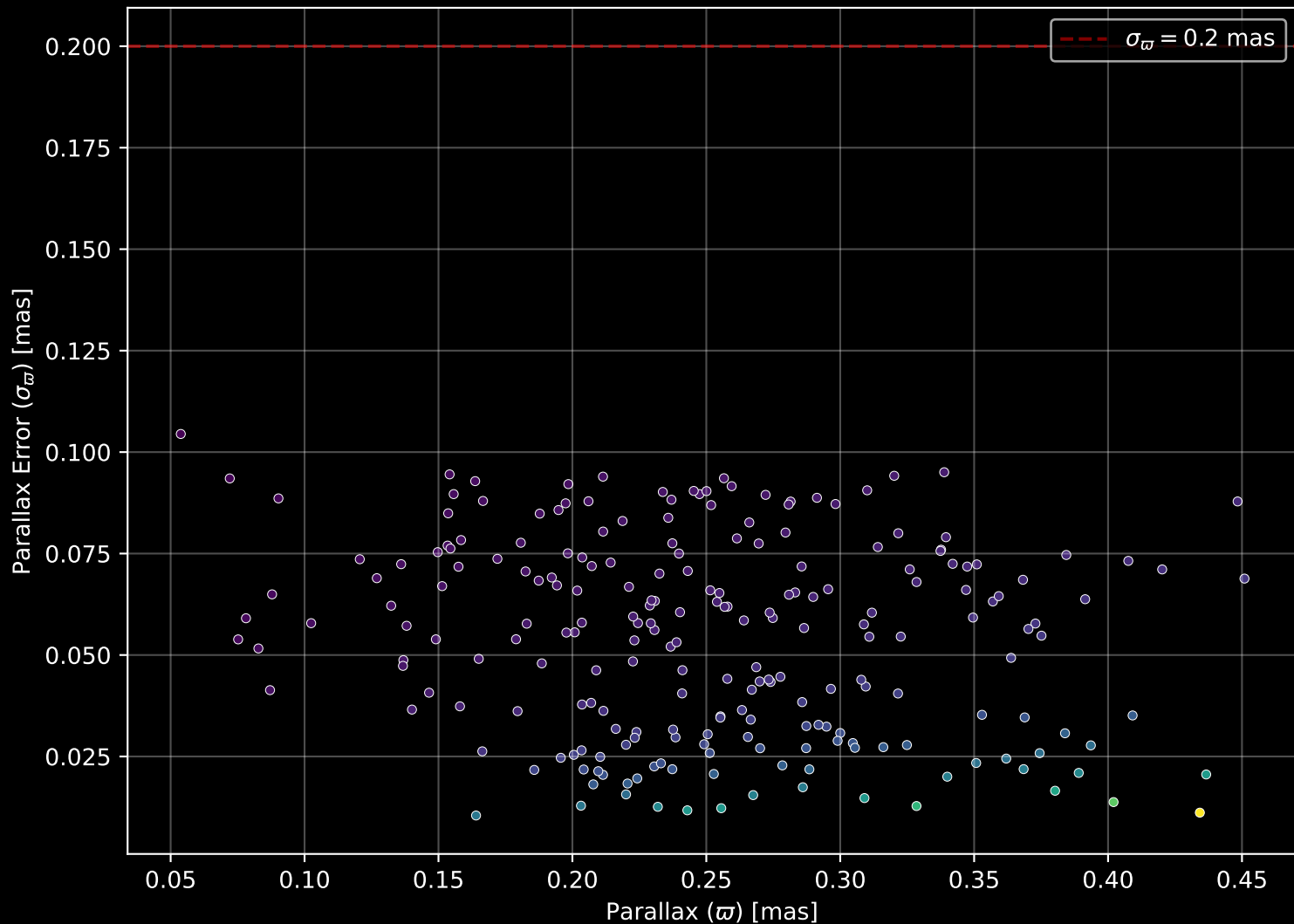
Gaia Cluster: [SAI_94] Parallax Quality (n= 225)
