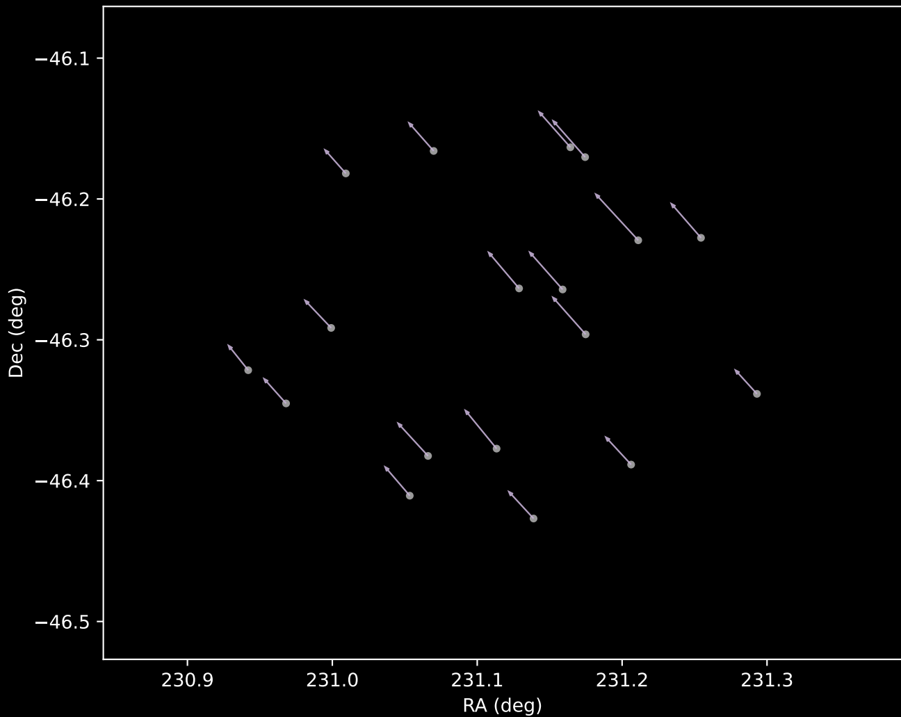
Gaia DR3 Cluster 9 Proper Motion Vectors (n=18)
