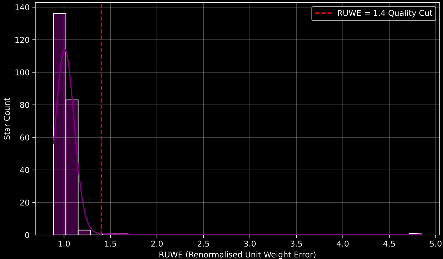
Gaia Cluster: [SAI_94] RUWE Distribution (n= 225)
