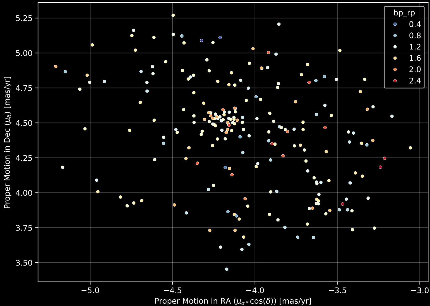
Gaia Cluster: [SAI_94] Proper Motion Diagram (n= 225)
