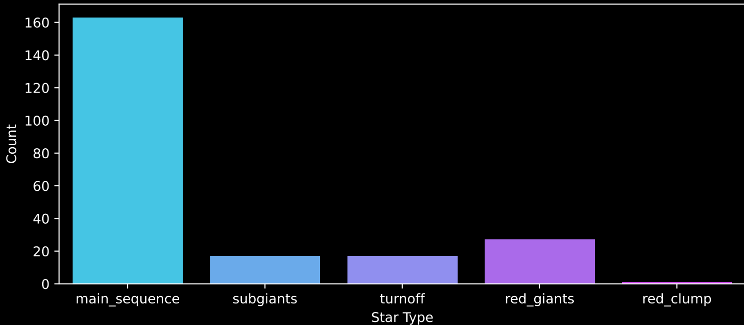
Gaia Cluster: [SAI_94] Count plot of Star Type
