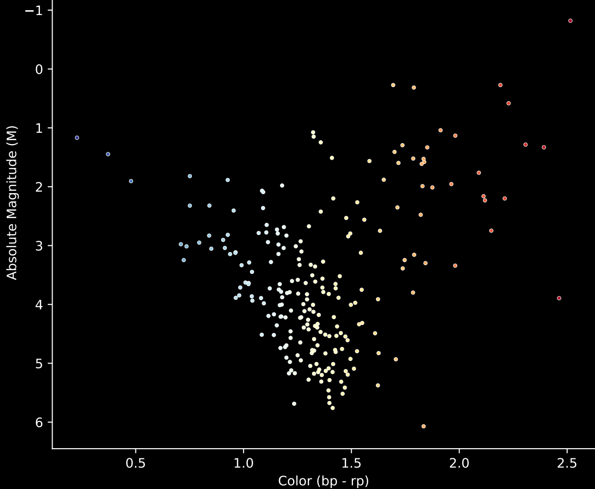
Gaia Cluster: [SAI_94] Stars (n= 225) Hertzsprung-Russel Diagram
