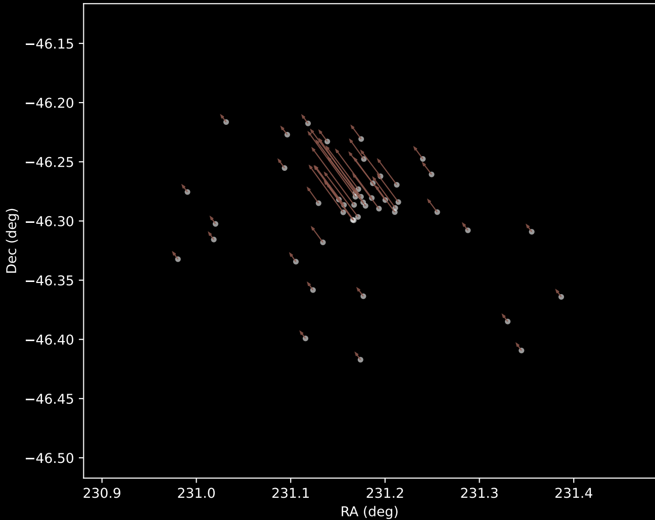
Gaia DR3 Cluster 10 Proper Motion Vectors (n=48)
