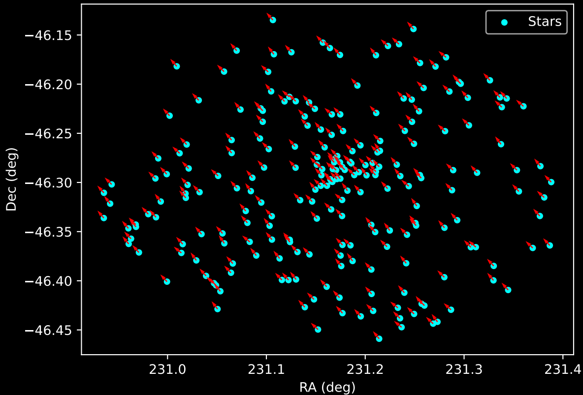
Gaia Cluster: [SAI_94] Proper Motion Vectors for Gaia Star Field (n= 225)
