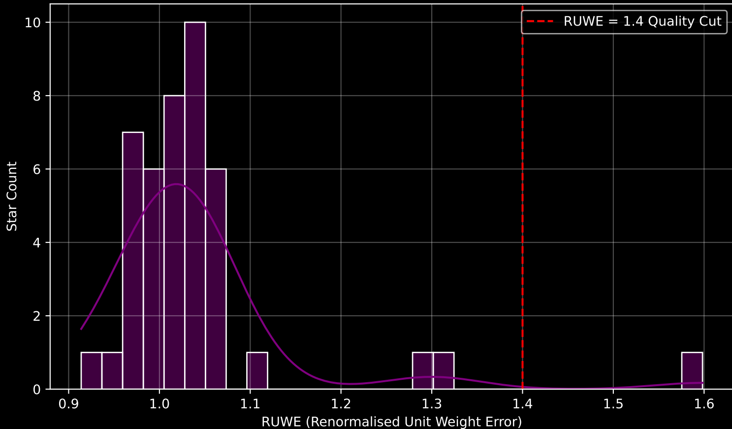
Gaia Cluster: [Shorlin_1] RUWE Distribution (n= 43)
