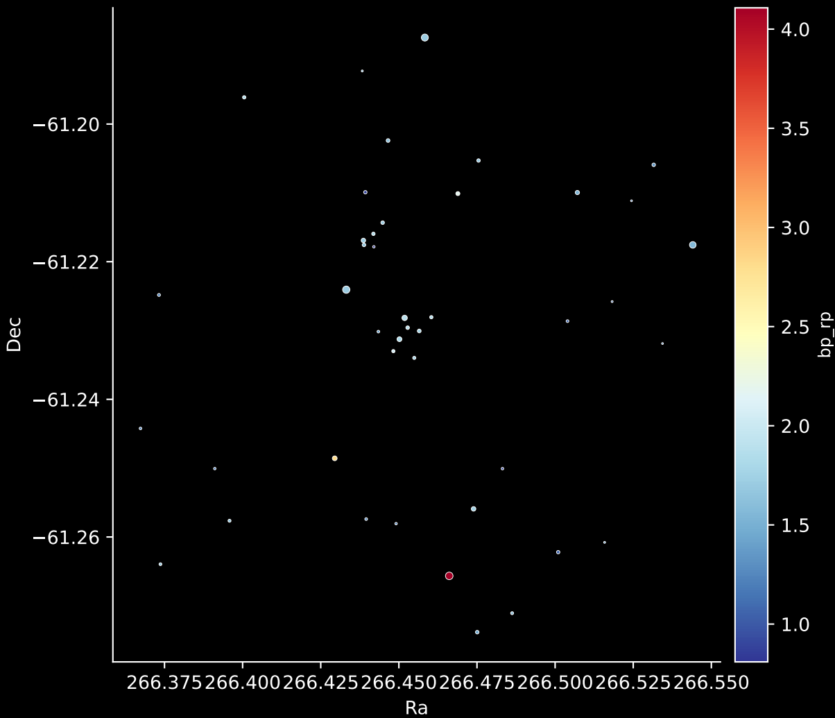
Gaia Cluster: [Shorlin_1] Stars: 43
