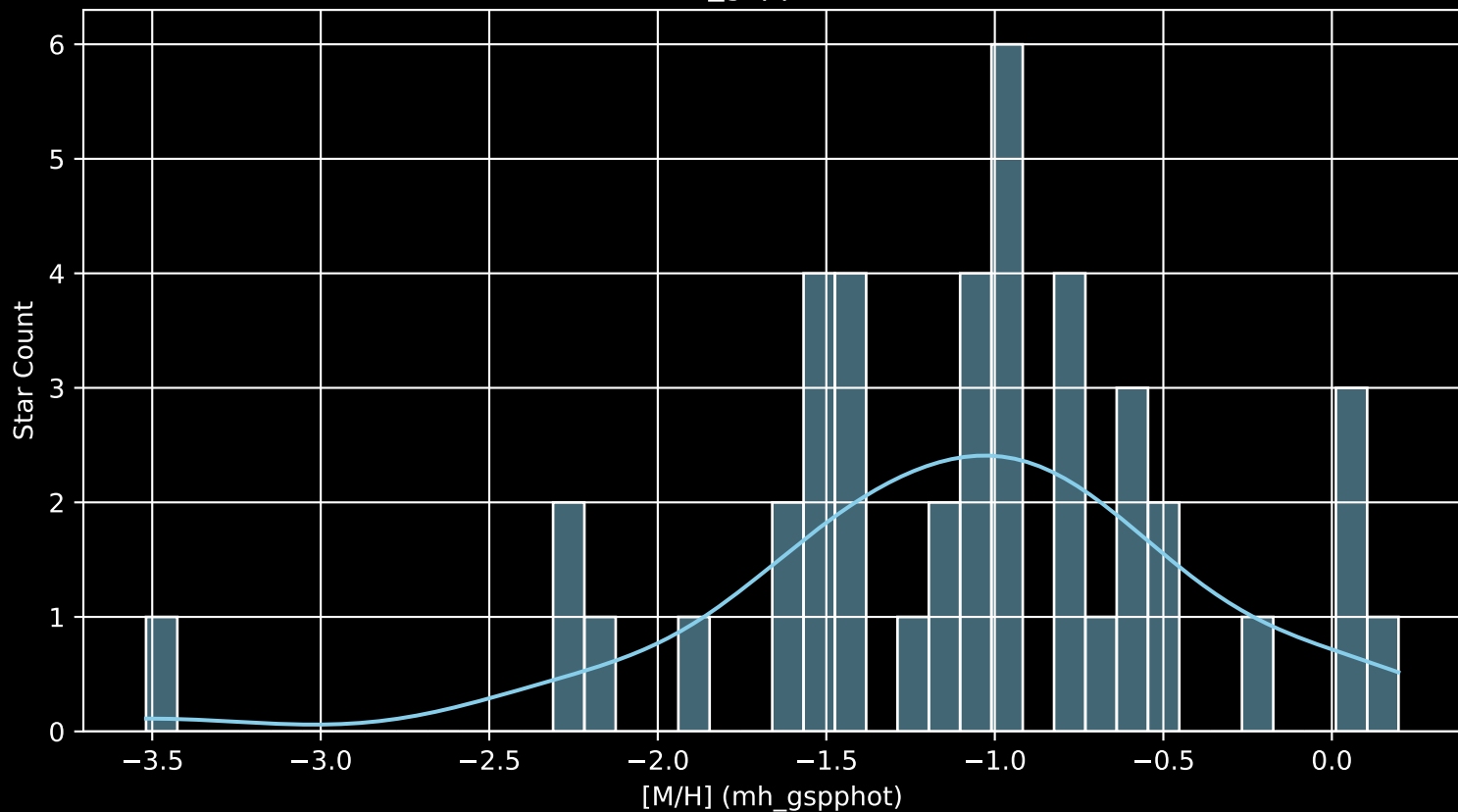
Gaia Cluster: [Shorlin_1 [M/H] (mh_gspphot) (n= 43)
