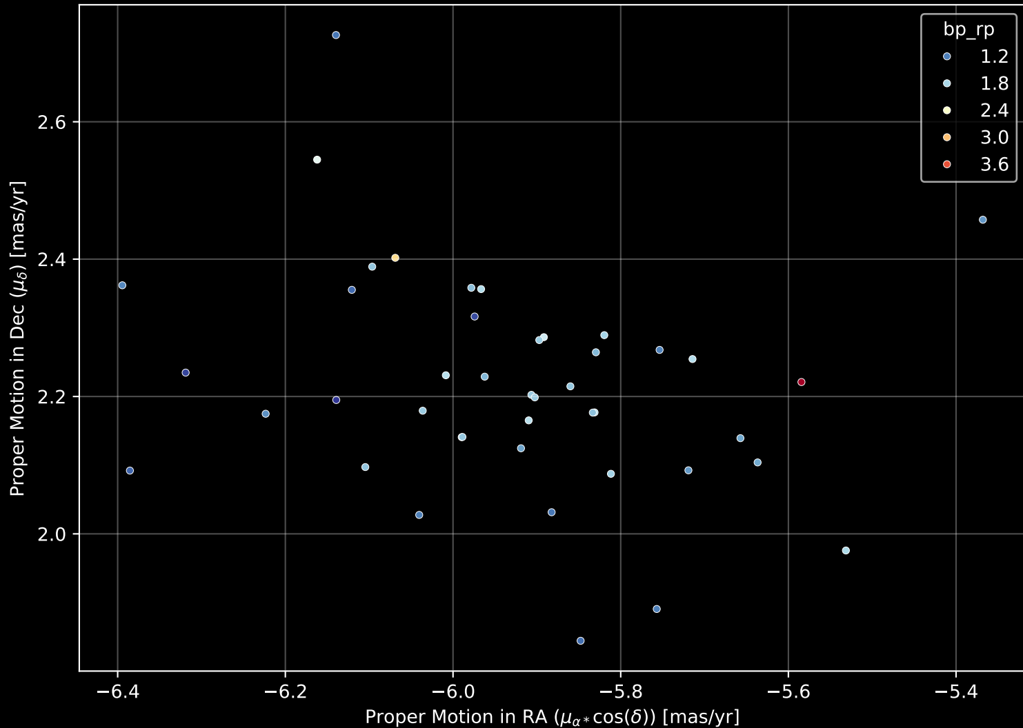
Gaia Cluster: [Shorlin_1] Proper Motion Diagram (n= 43)
