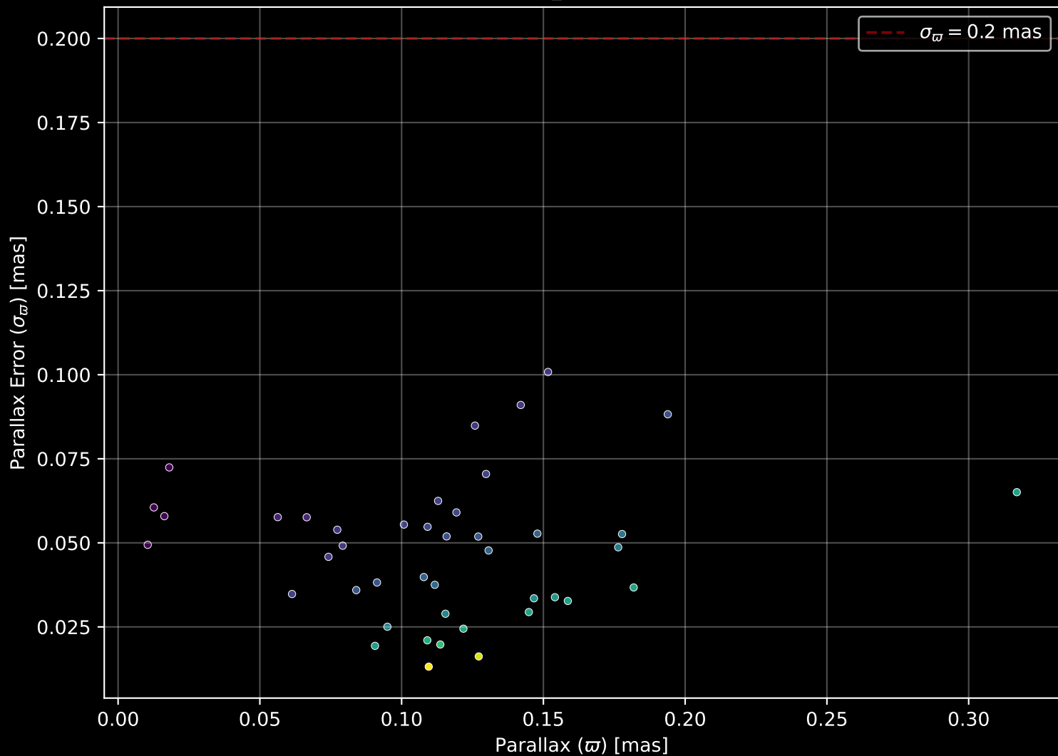
Gaia Cluster: [Shorlin_1] Parallax Quality (n= 43)
