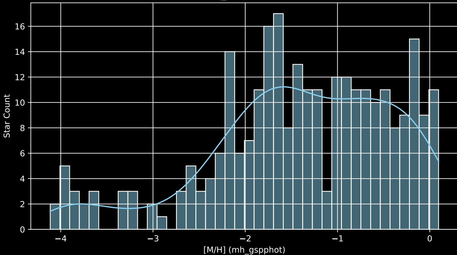
Gaia Cluster: [Skiff_J0458+43.0 [M/H] (mh_gspphot) (n= 281)
