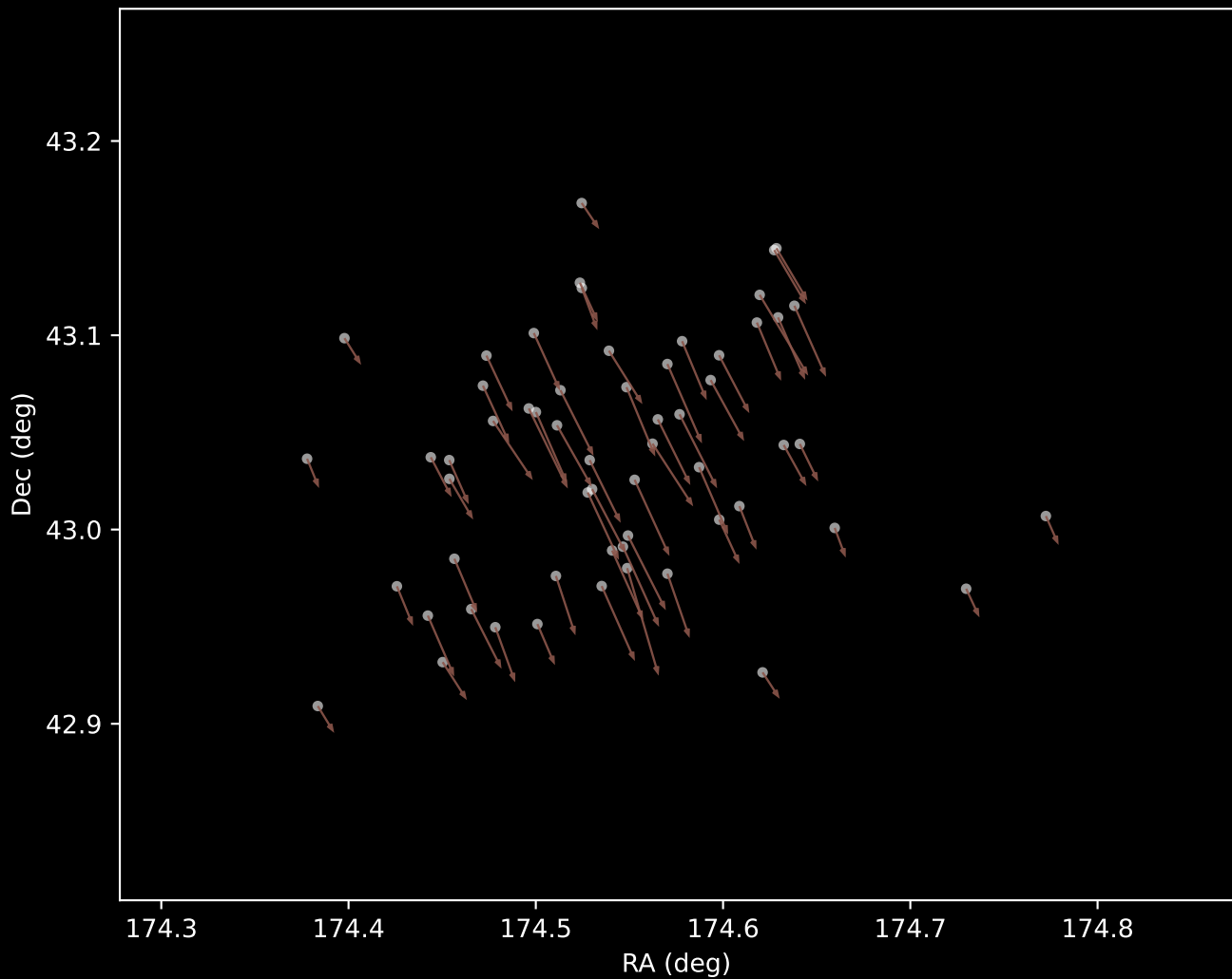
Gaia DR3 Cluster 10 Proper Motion Vectors (n=59)
