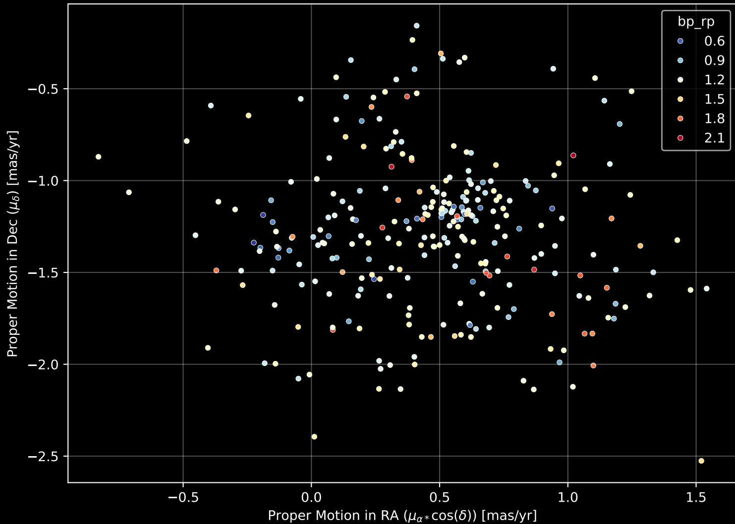
Gaia Cluster: [Skiff J0458+43.0] Proper Motion Diagram (n= 281)
