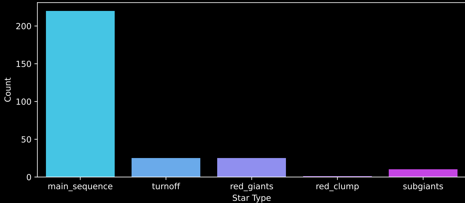
Gaia Cluster: [Skiff_J0458+43.0] Count plot of Star Type
