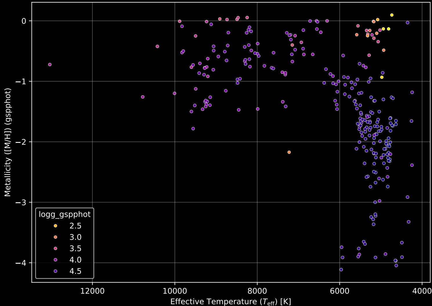
Gaia Cluster: [Skiff_J0458+43.0] Stellar Population Parameters (n= 281)
