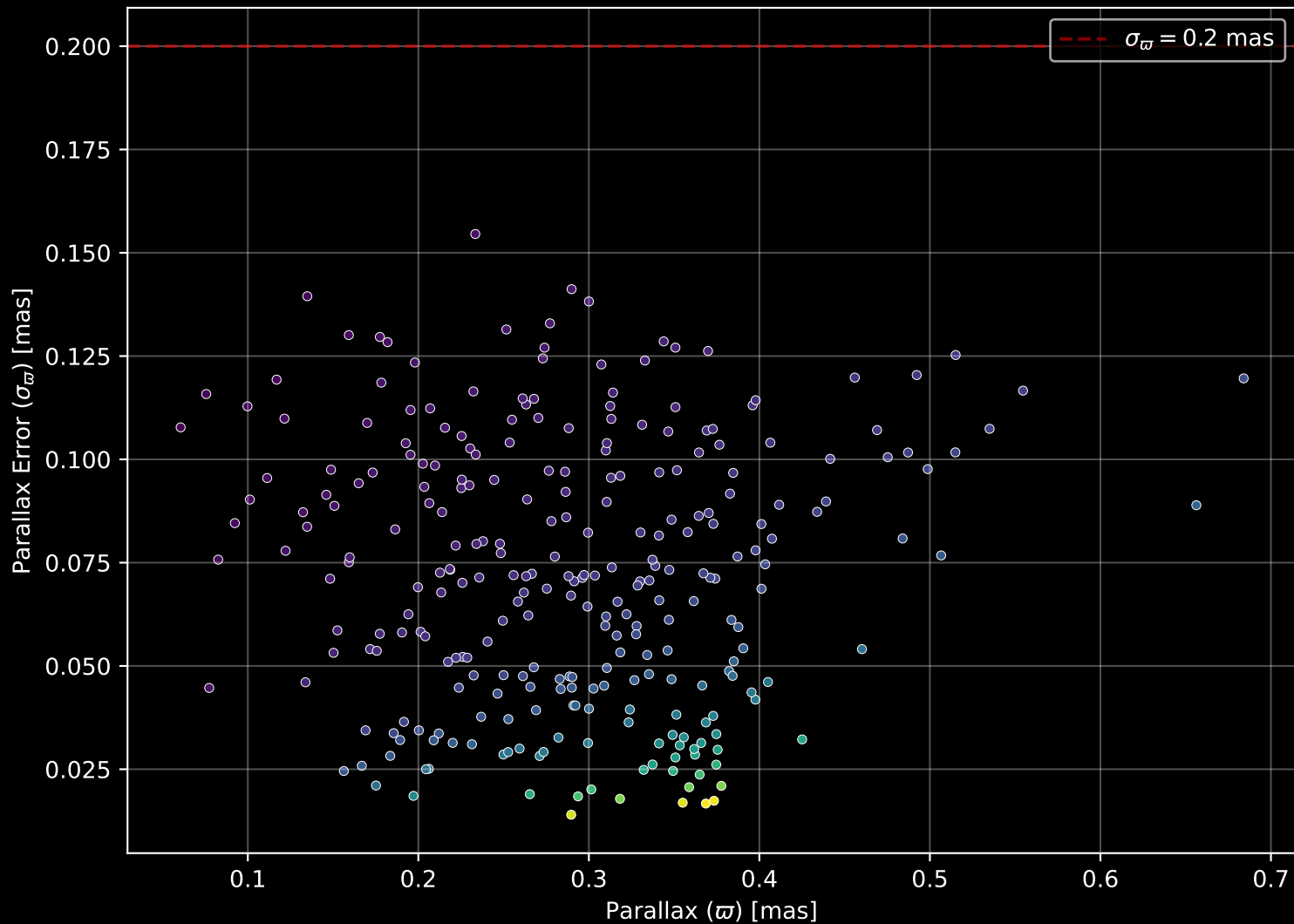
Gaia Cluster: [Skiff_J0458+43.0] Parallax Quality (n= 281)
