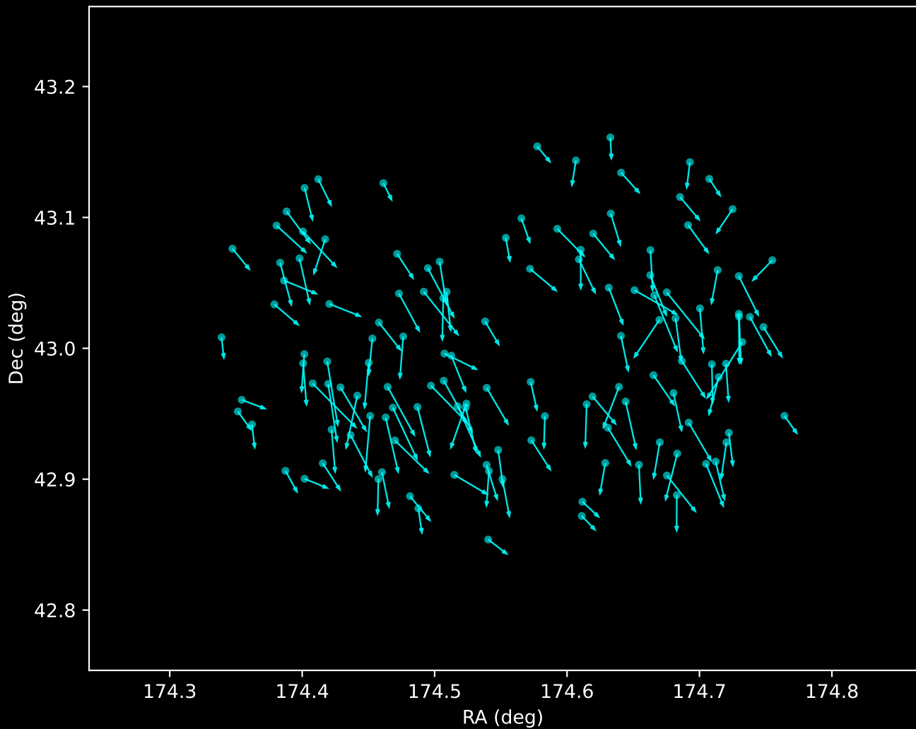
Gaia DR3 Noise Stream Proper Motion Vectors (n=128)
