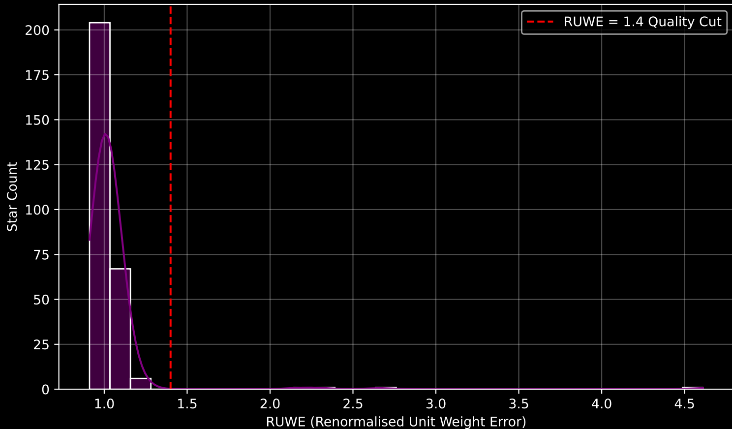
Gaia Cluster: [Skiff_J0458+43.0] RUWE Distribution (n= 281)
