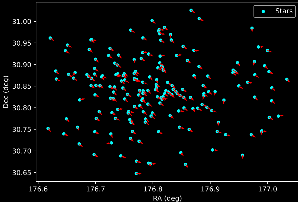
Gaia Cluster: [Skiff_J0507+30.8] Proper Motion Vectors for Gaia Star Field (n= 189)
