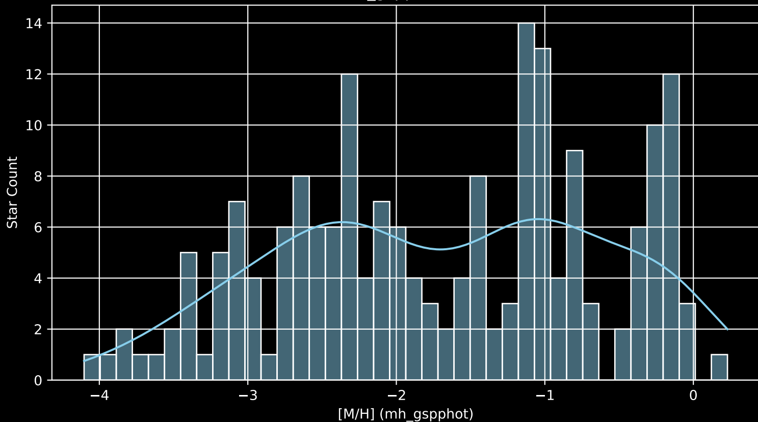
Gaia Cluster: [Skiff_J0507+30.8 [M/H] (mh_gspphot) (n= 189)
