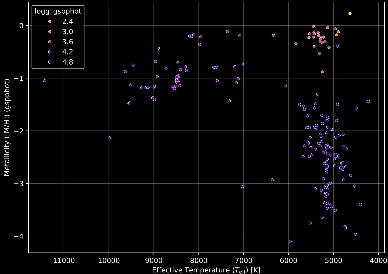
Gaia Cluster: [Skiff_J0507+30.8] Stellar Population Parameters (n= 189)
