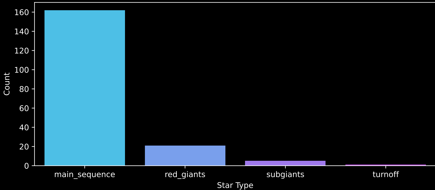
Gaia Cluster: [Skiff_J0507+30.8] Count plot of Star Type
