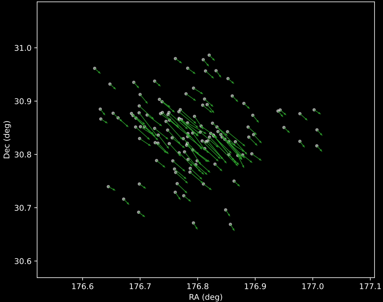
Gaia DR3 Cluster 4 Proper Motion Vectors (n=121)
