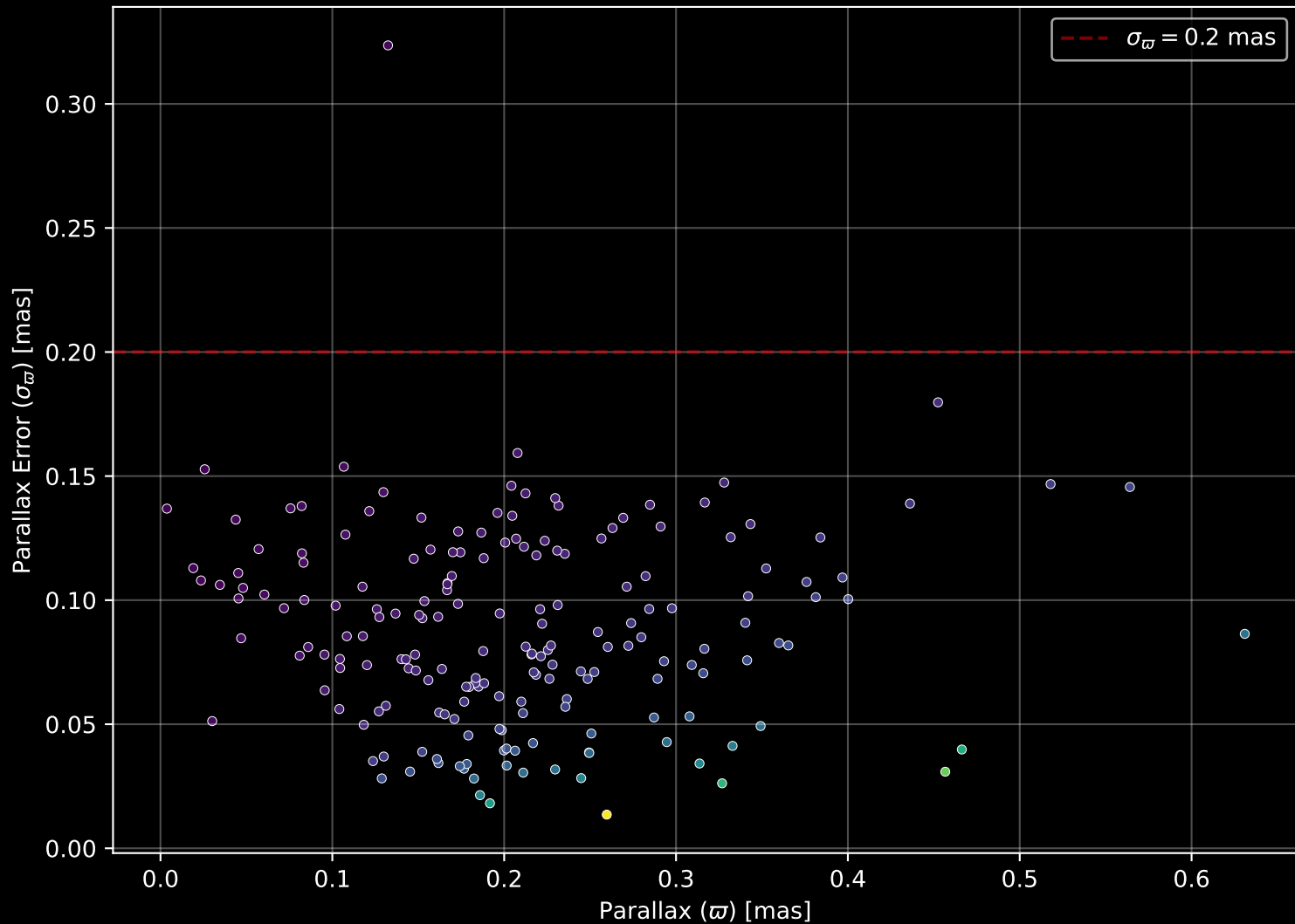
Gaia Cluster: [Skiff_J0507+30.8] Parallax Quality (n= 189)
