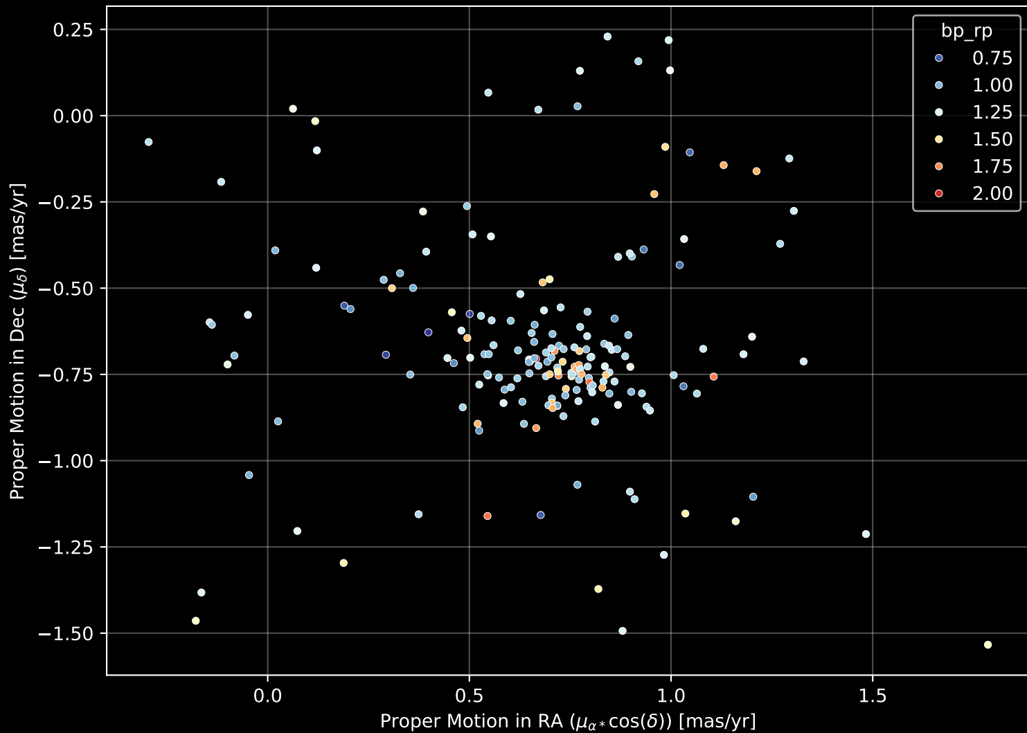
Gaia Cluster: [Skiff_J0507+30.8] Proper Motion Diagram (n= 189)
