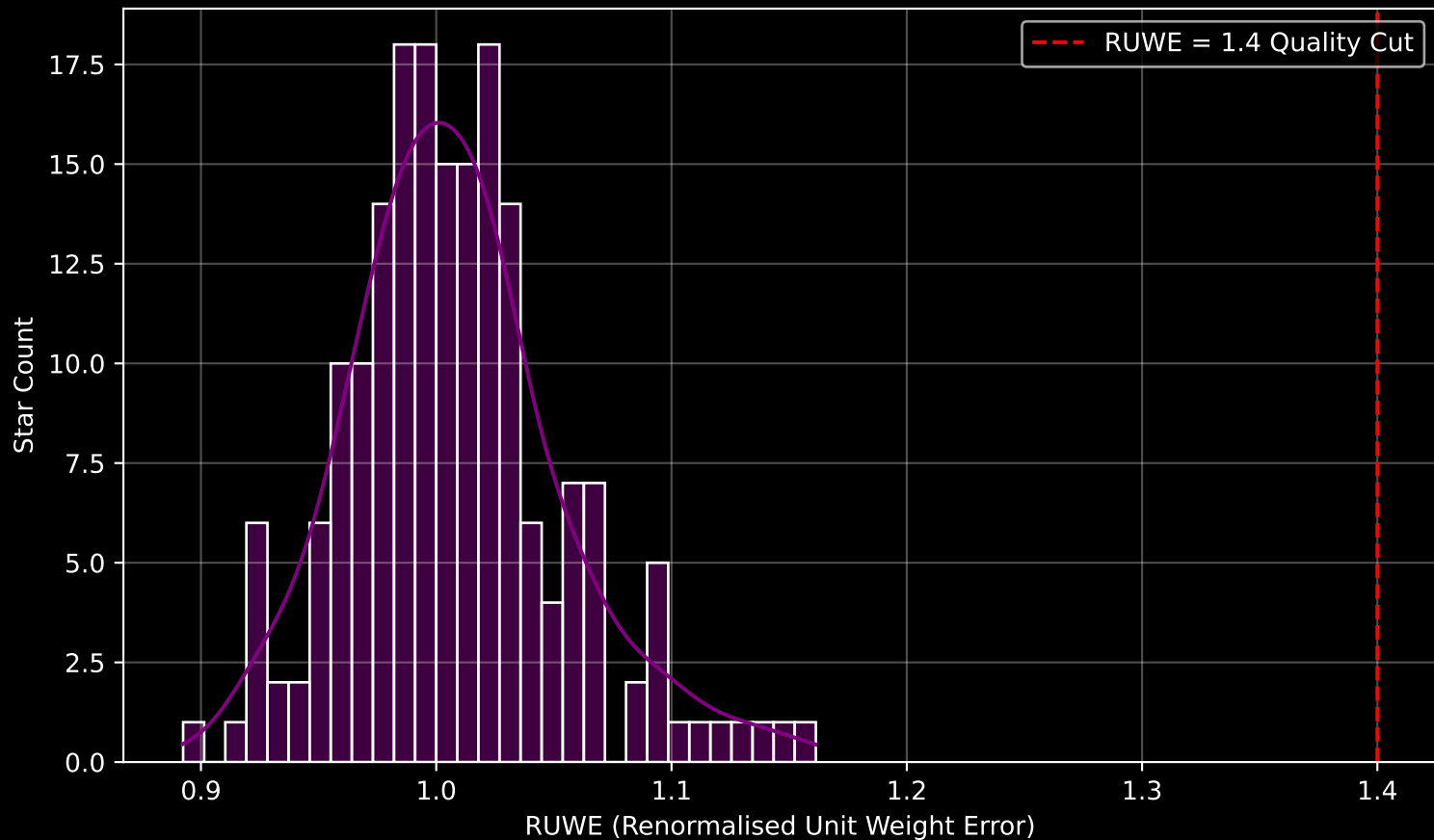
Gaia Cluster: [Skiff_J0507+30.8] RUWE Distribution (n= 188)
