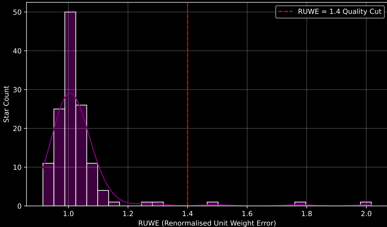
Gaia Cluster: [Skiff_J1942+38.6] RUWE Distribution (n= 133)
