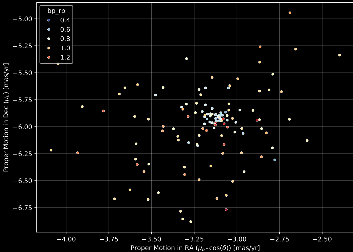
Gaia Cluster: [Skiff_J1942+38.6] Proper Motion Diagram (n= 133)
