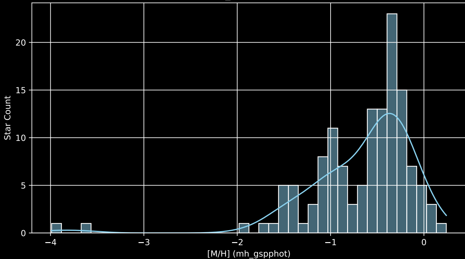
Gaia Cluster: [Skiff_J1942+38.6 [M/H] (mh_gspphot) (n= 133)
