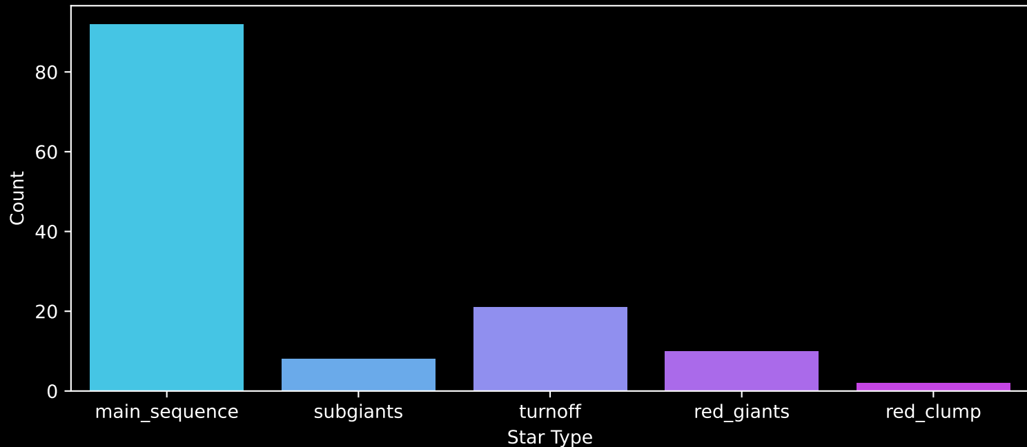
Gaia Cluster: [Skiff_J1942+38.6] Count plot of Star Type
