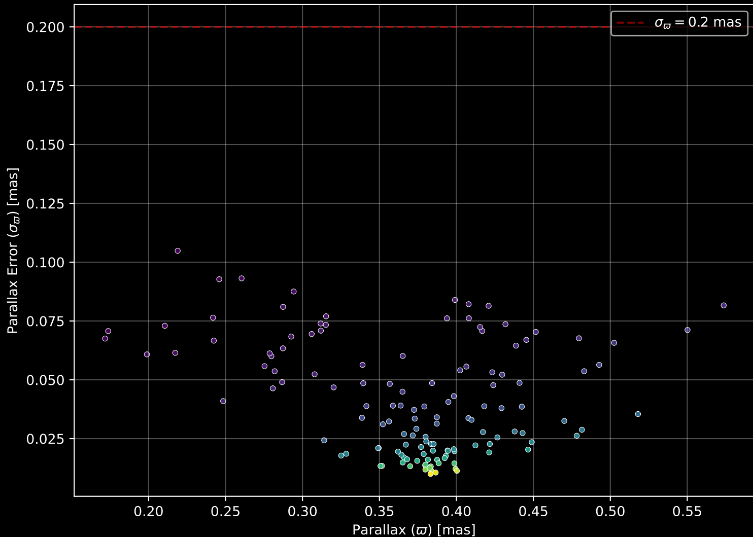
Gaia Cluster: [Skiff_J1942+38.6] Parallax Quality (n= 133)
