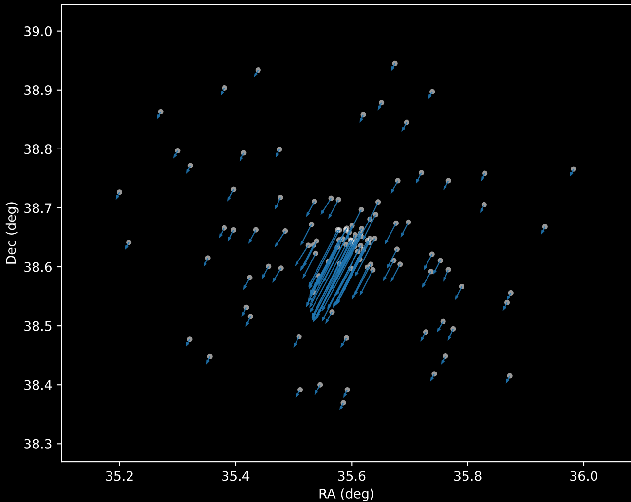
Gaia DR3 Cluster 0 Proper Motion Vectors (n=108)
