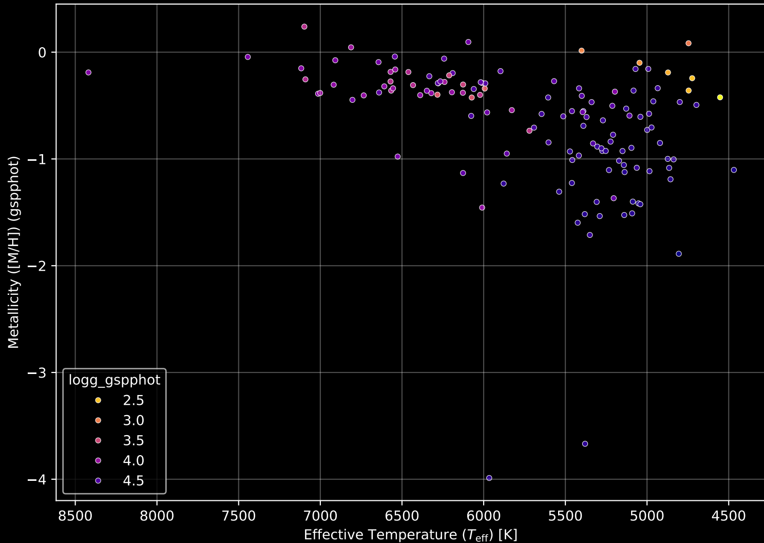
Gaia Cluster: [Skiff_J1942+38.6] Stellar Population Parameters (n= 133)
