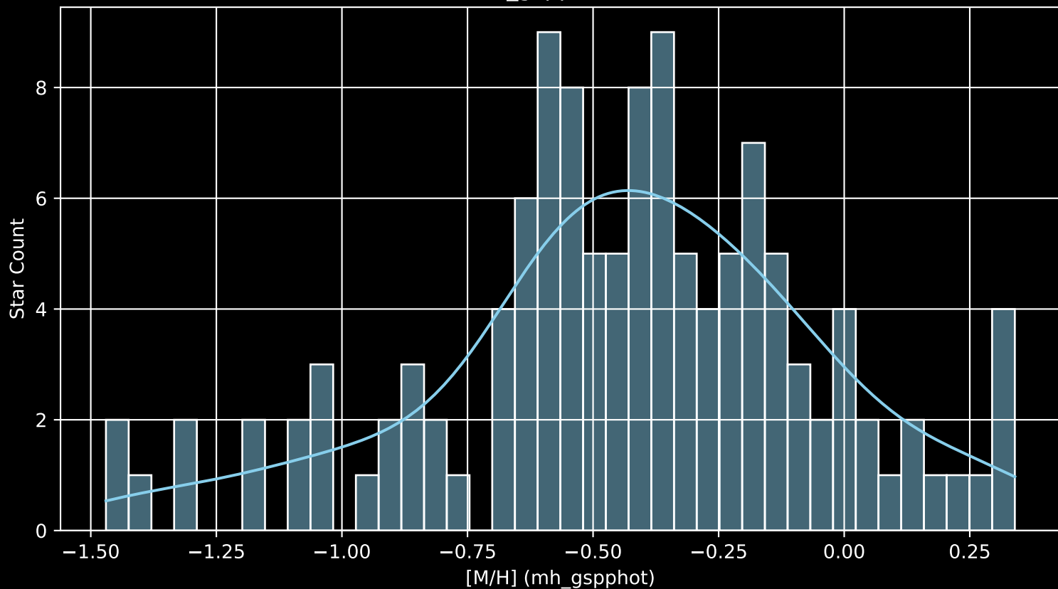
Gaia Cluster: [Stock_10 [M/H] (mh_gspphot) (n= 122)
