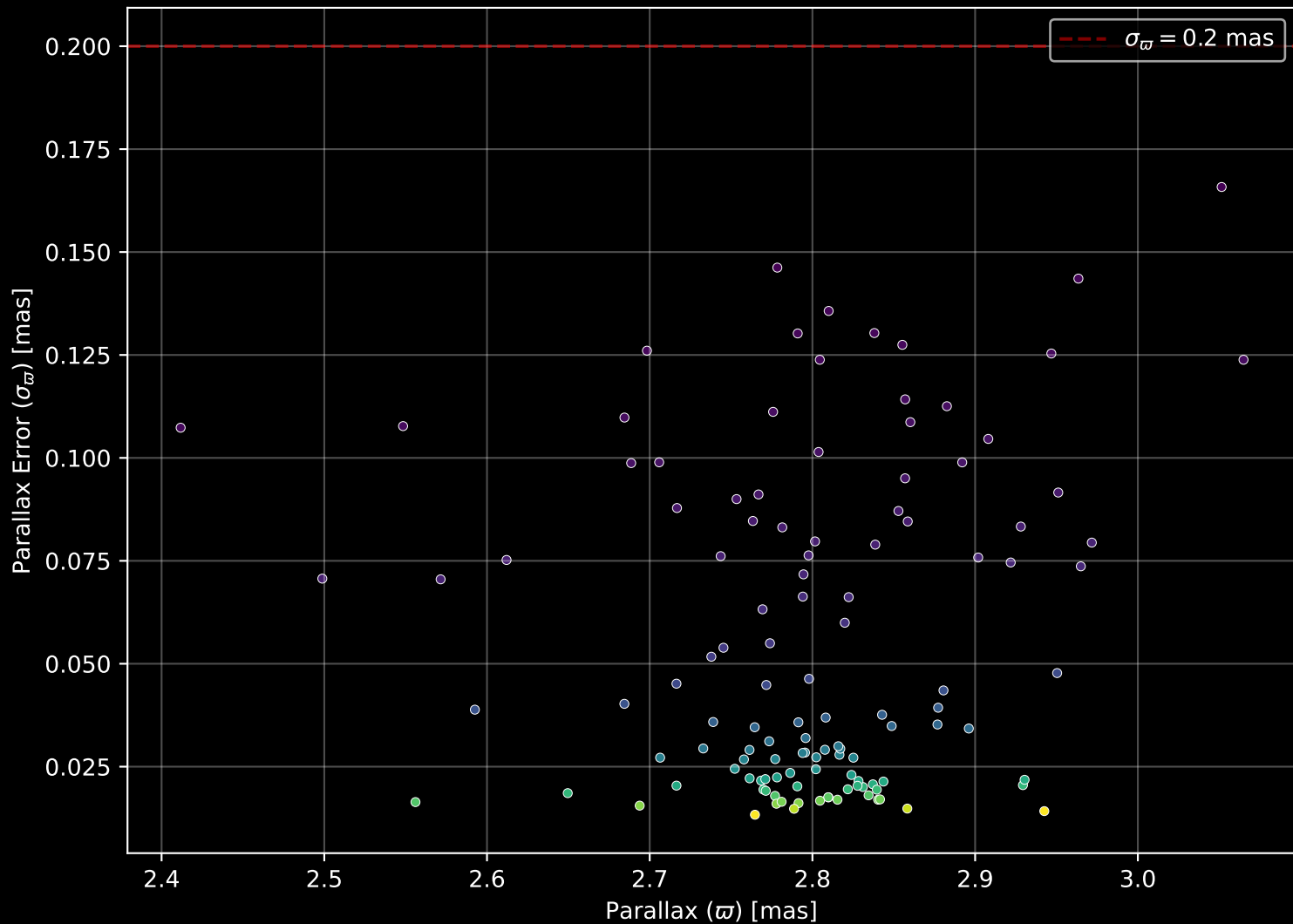
Gaia Cluster: [Stock_10] Parallax Quality (n= 122)
