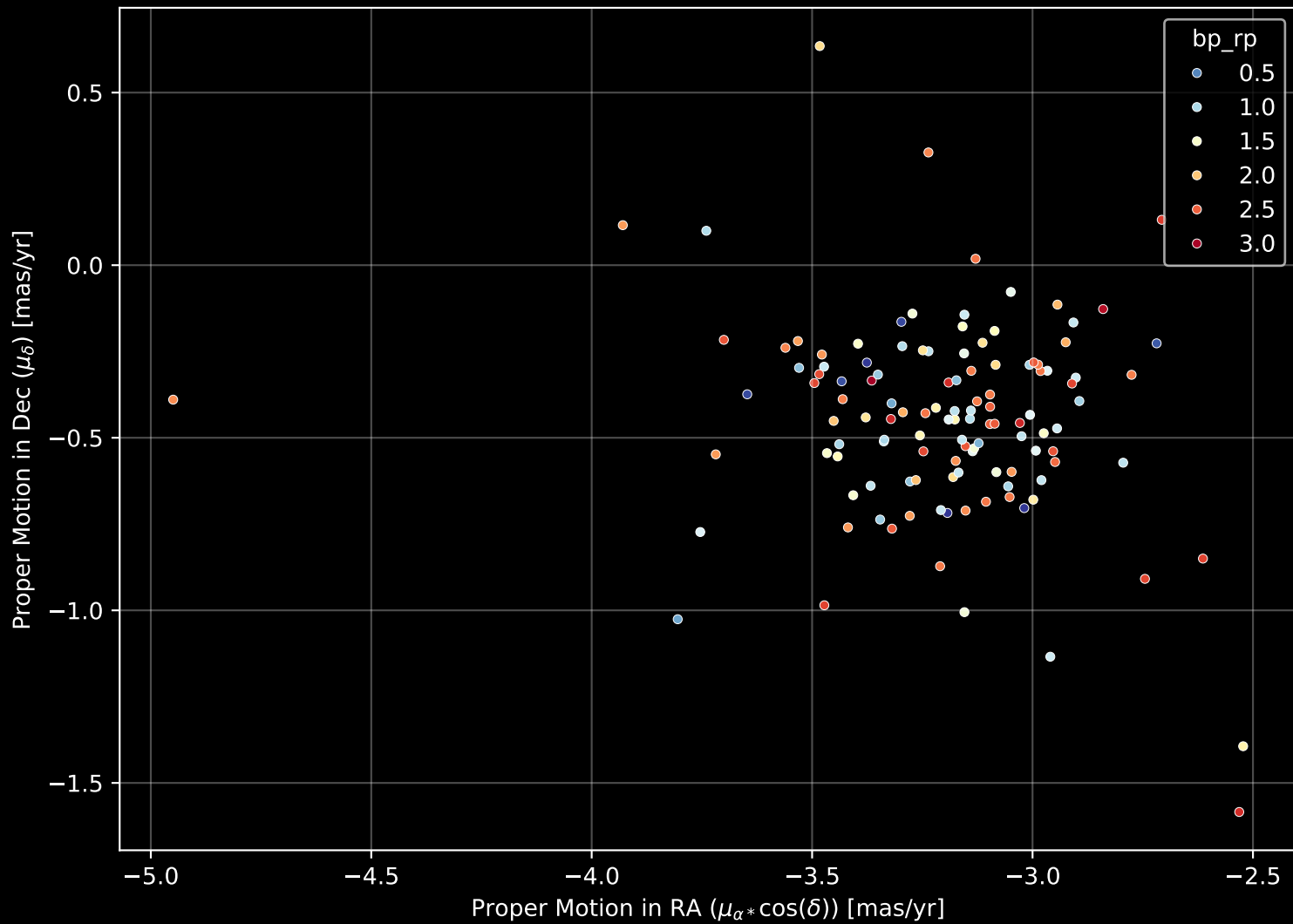
Gaia Cluster: [Stock_10] Proper Motion Diagram (n= 122)
