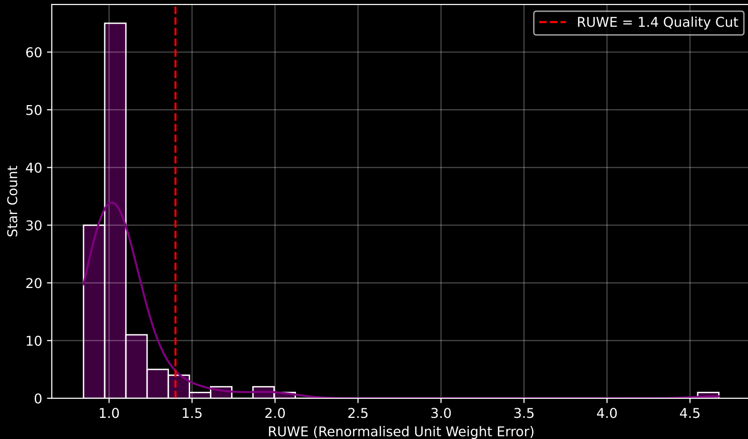
Gaia Cluster: [Stock_10] RUWE Distribution (n= 122)
