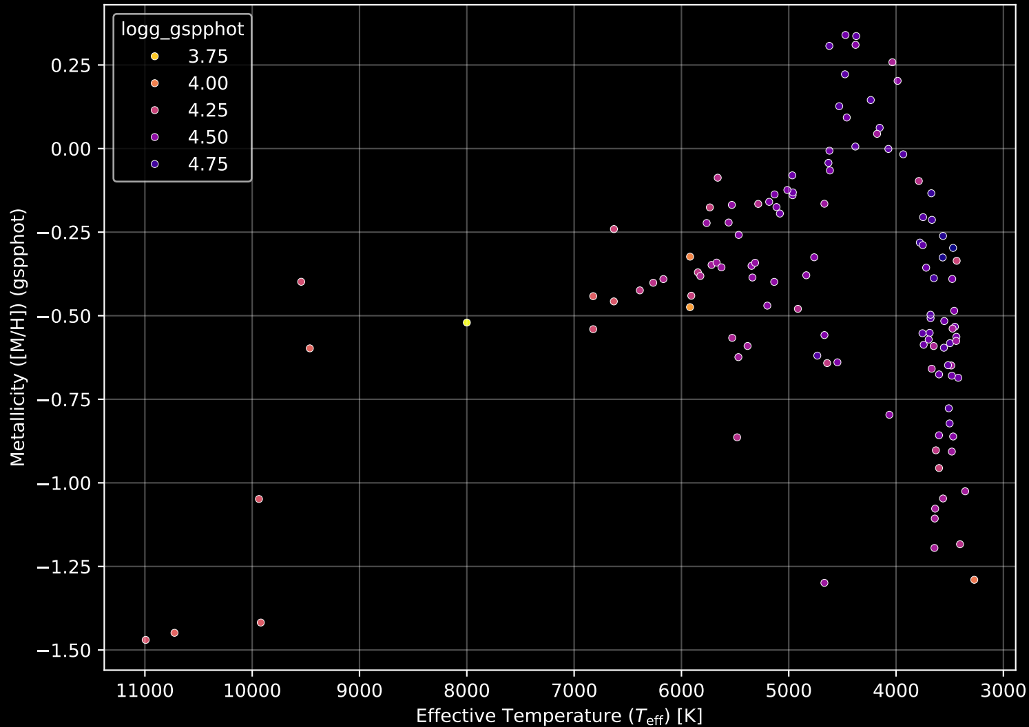
Gaia Cluster: [Stock_10] Stellar Population Parameters (n= 122)
