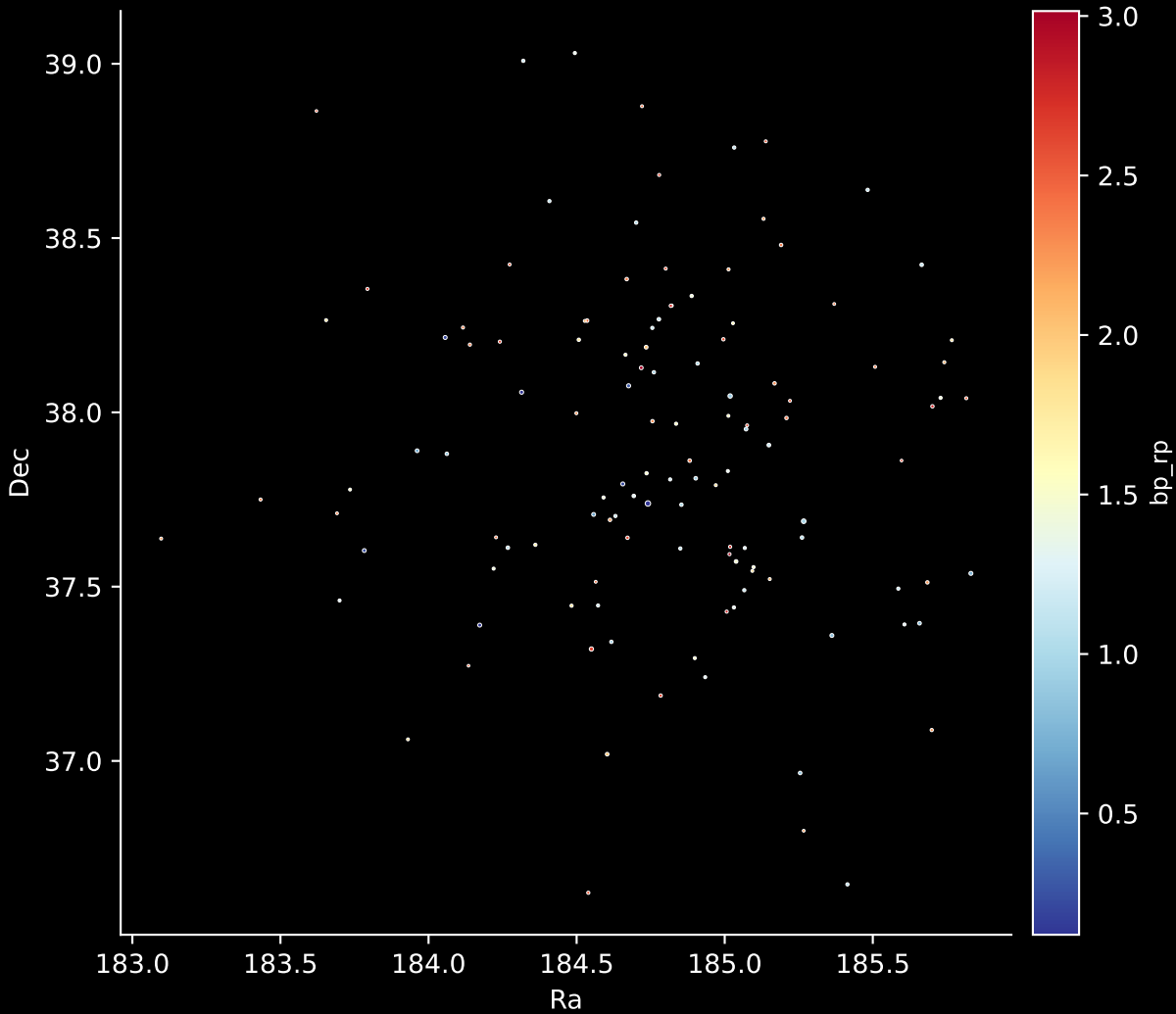
Gaia Cluster: [Stock_10] Stars: 122
