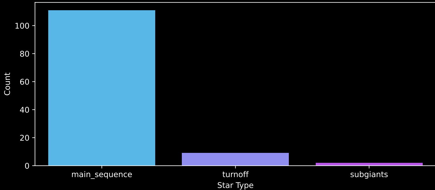
Gaia Cluster: [Stock_10] Count plot of Star Type
