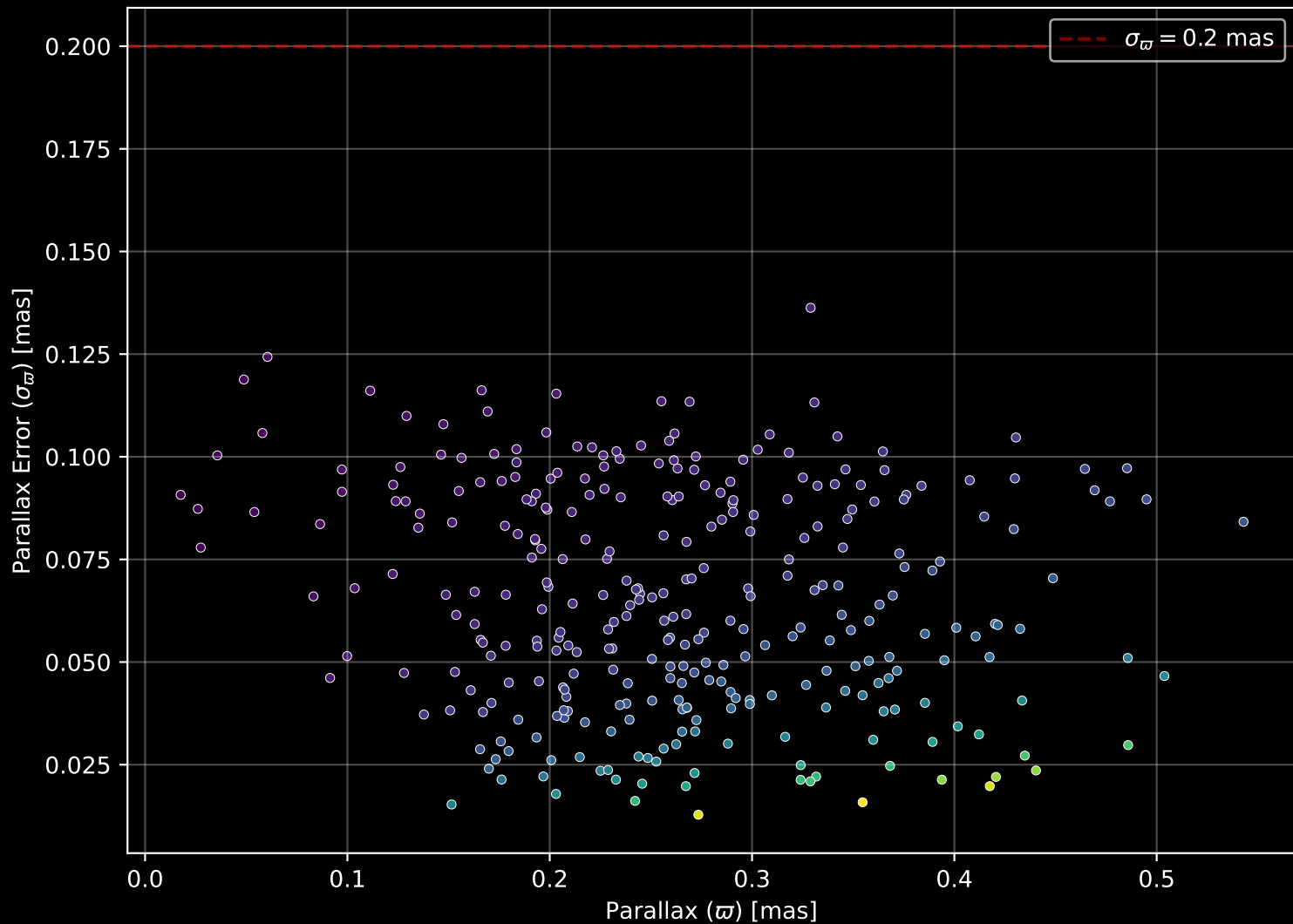
Gaia Cluster: [Stock_16] Parallax Quality (n= 313)
