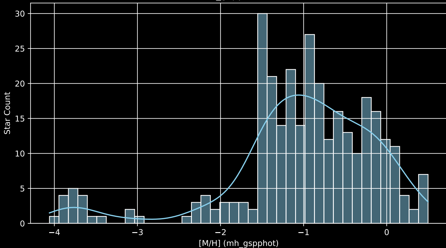
Gaia Cluster: [Stock_16 [M/H] (mh_gspphot) (n= 309)
