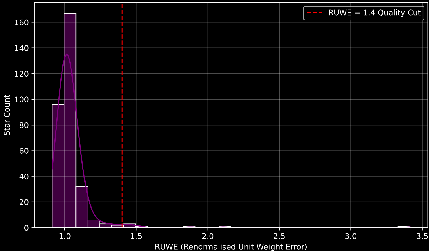
Gaia Cluster: [Stock_16] RUWE Distribution (n= 313)
