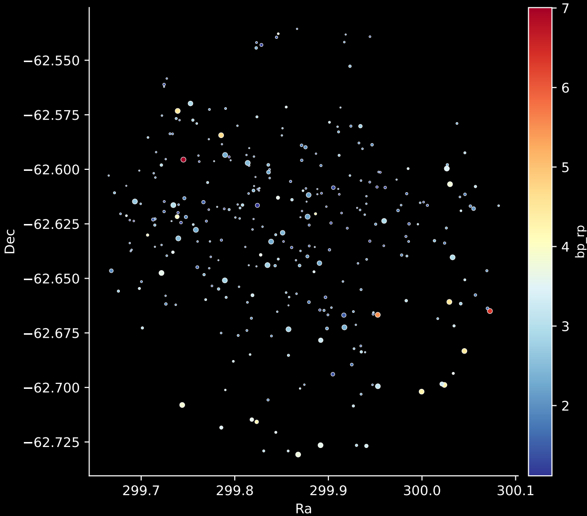
Gaia Cluster: [Stock_16] Stars: 313
