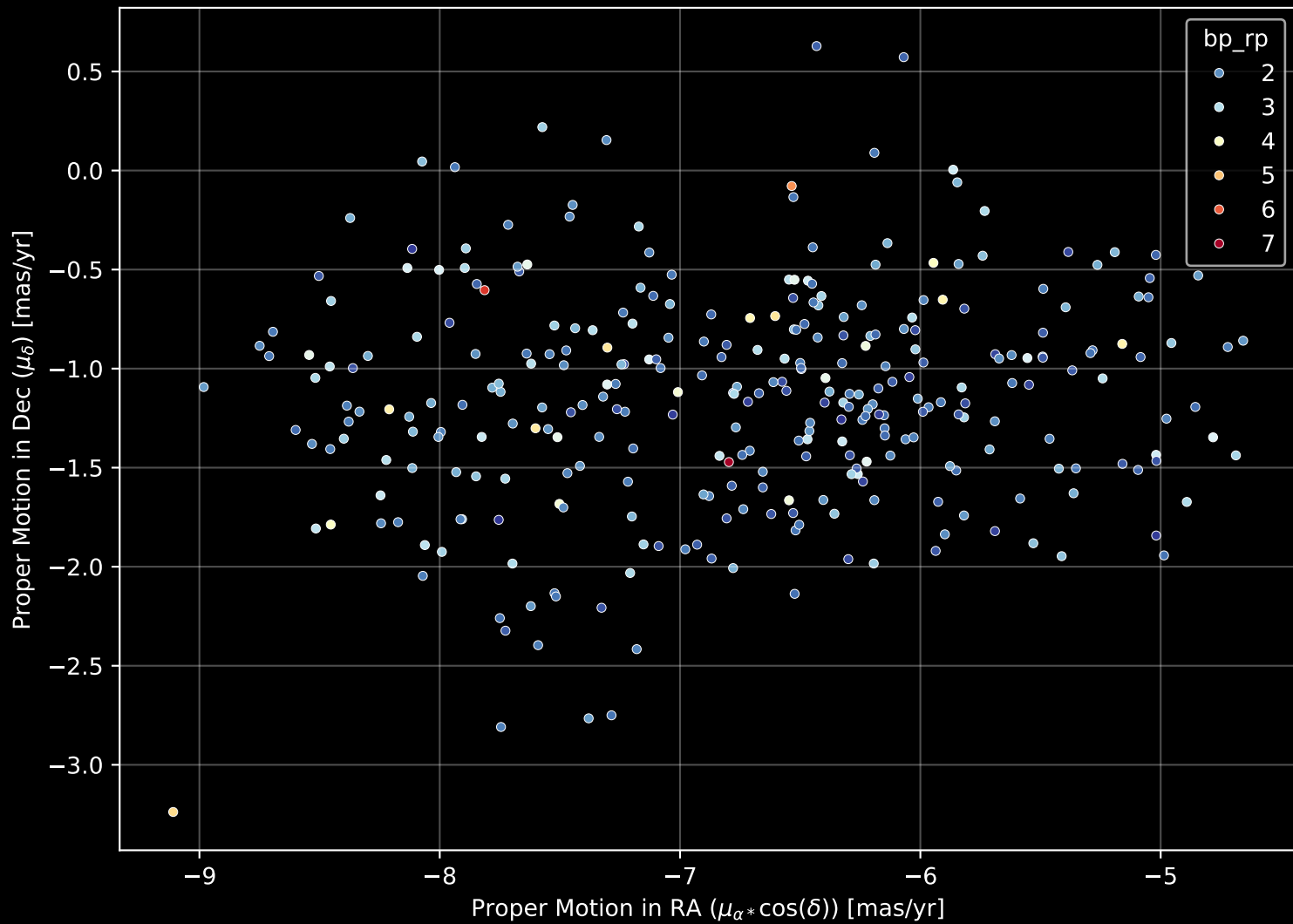
Gaia Cluster: [Stock_16] Proper Motion Diagram (n= 313)
