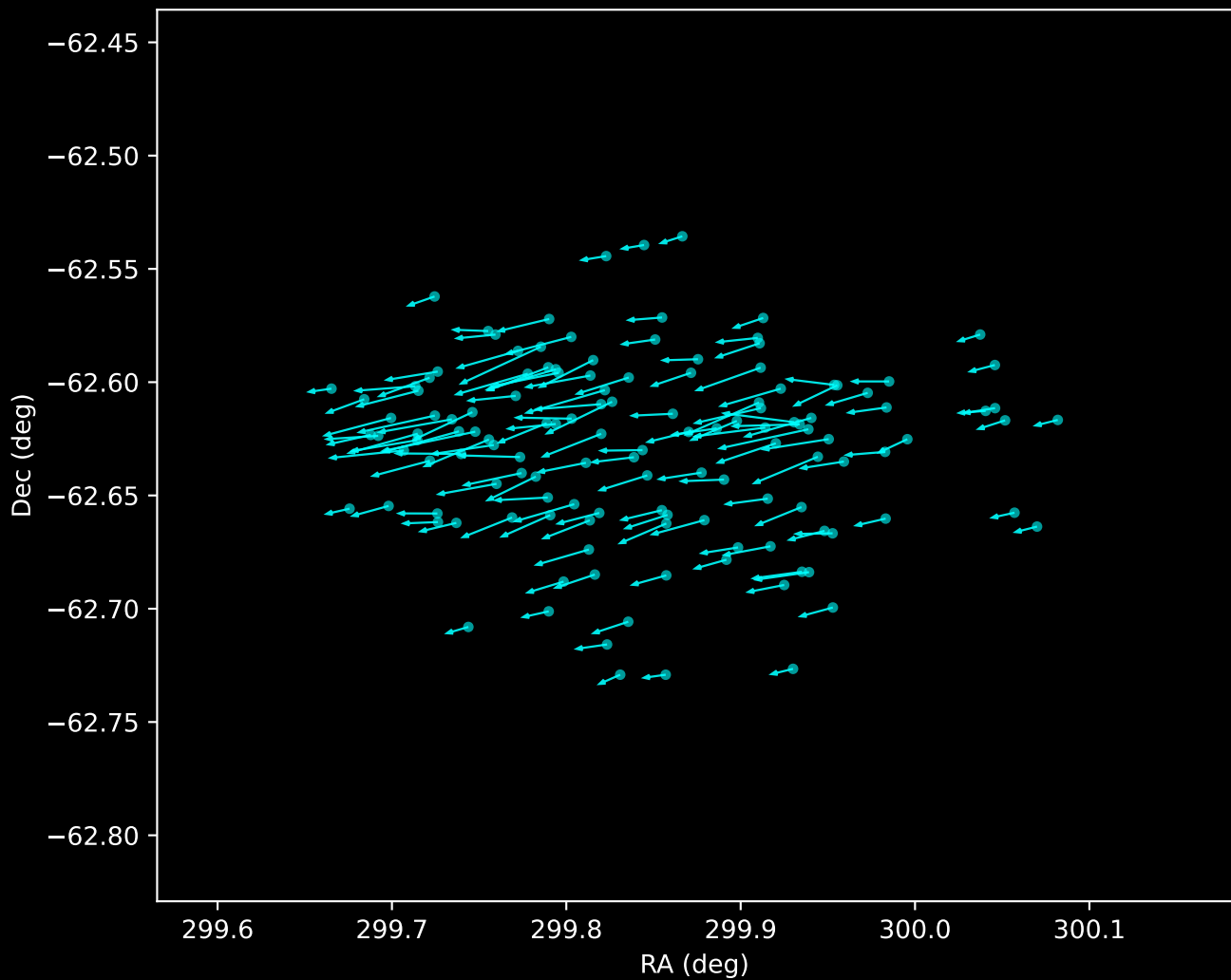
Gaia DR3 Noise Stream Proper Motion Vectors (n=133)
