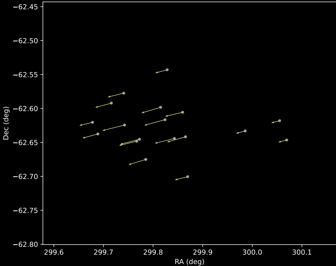
Gaia DR3 Cluster 17 Proper Motion Vectors (n=18)
