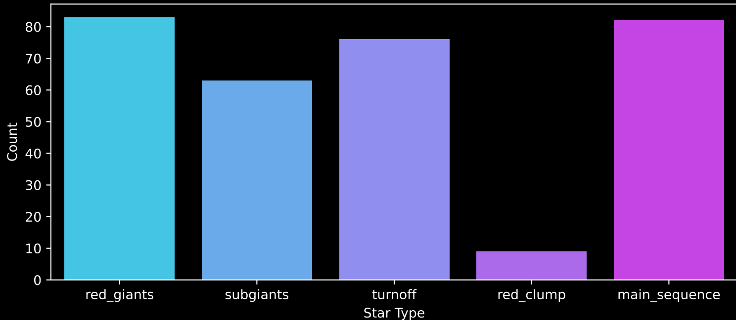
Gaia Cluster: [Stock_16] Count plot of Star Type
