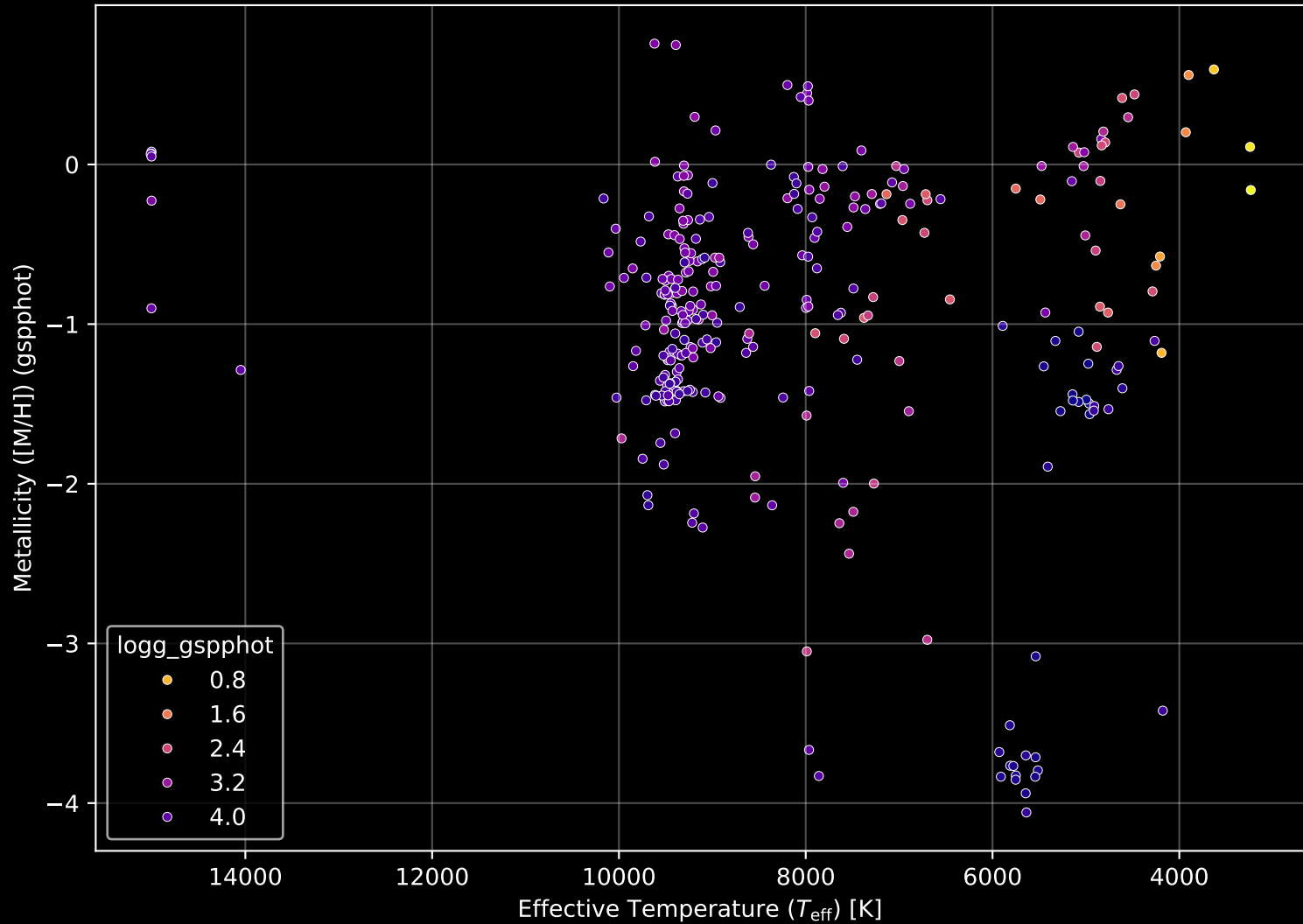
Gaia Cluster: [Stock_16] Stellar Population Parameters (n= 313)
