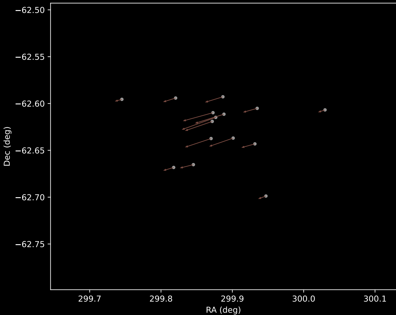
Gaia DR3 Cluster 10 Proper Motion Vectors (n=15)
