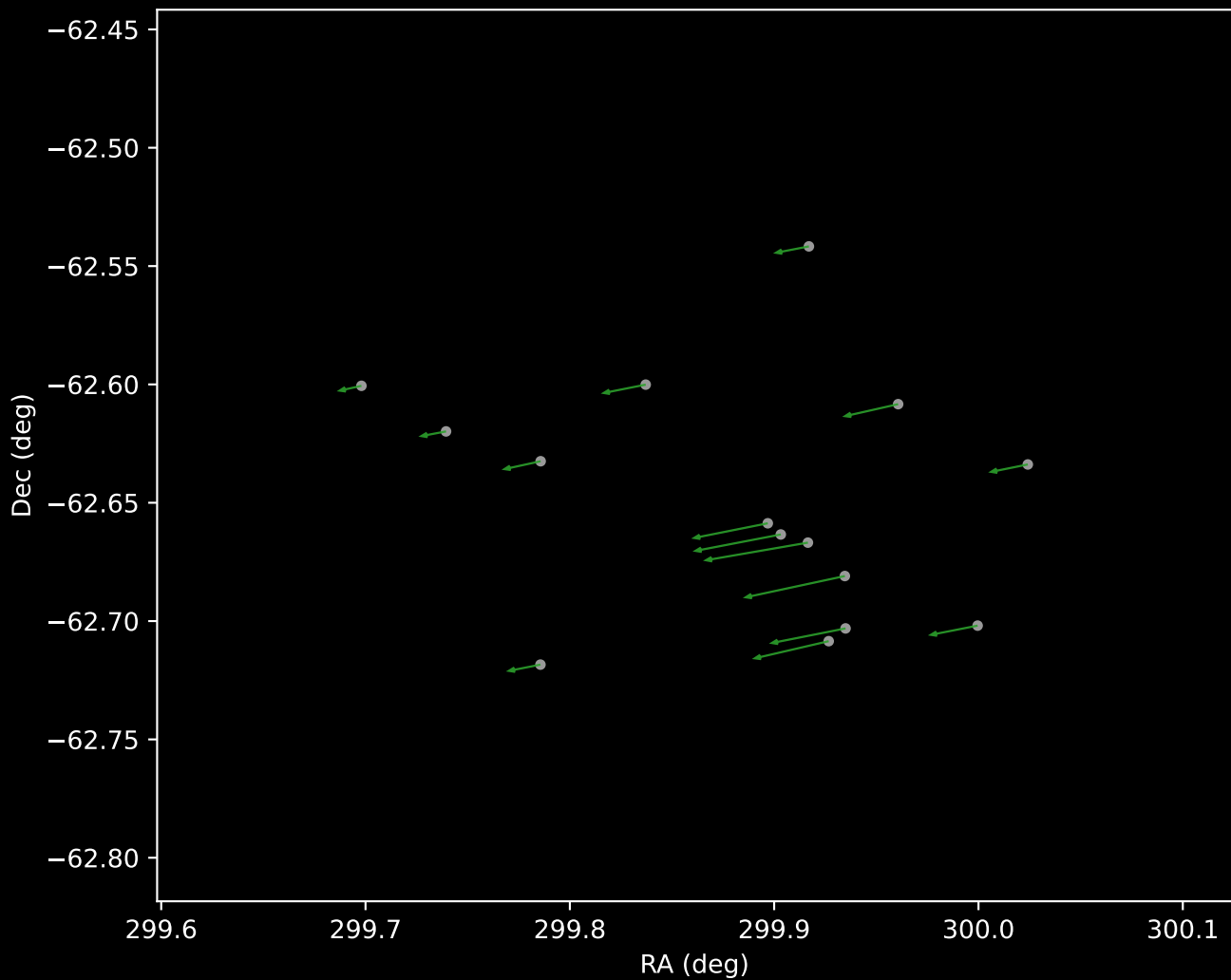
Gaia DR3 Cluster 4 Proper Motion Vectors (n=15)
