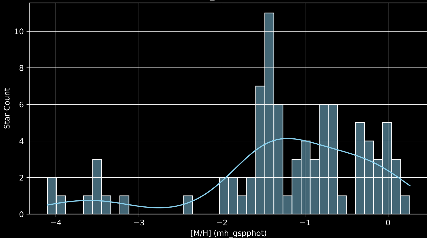
Gaia Cluster: [Stock_18 [M/H] (mh_gspphot) (n= 86)
