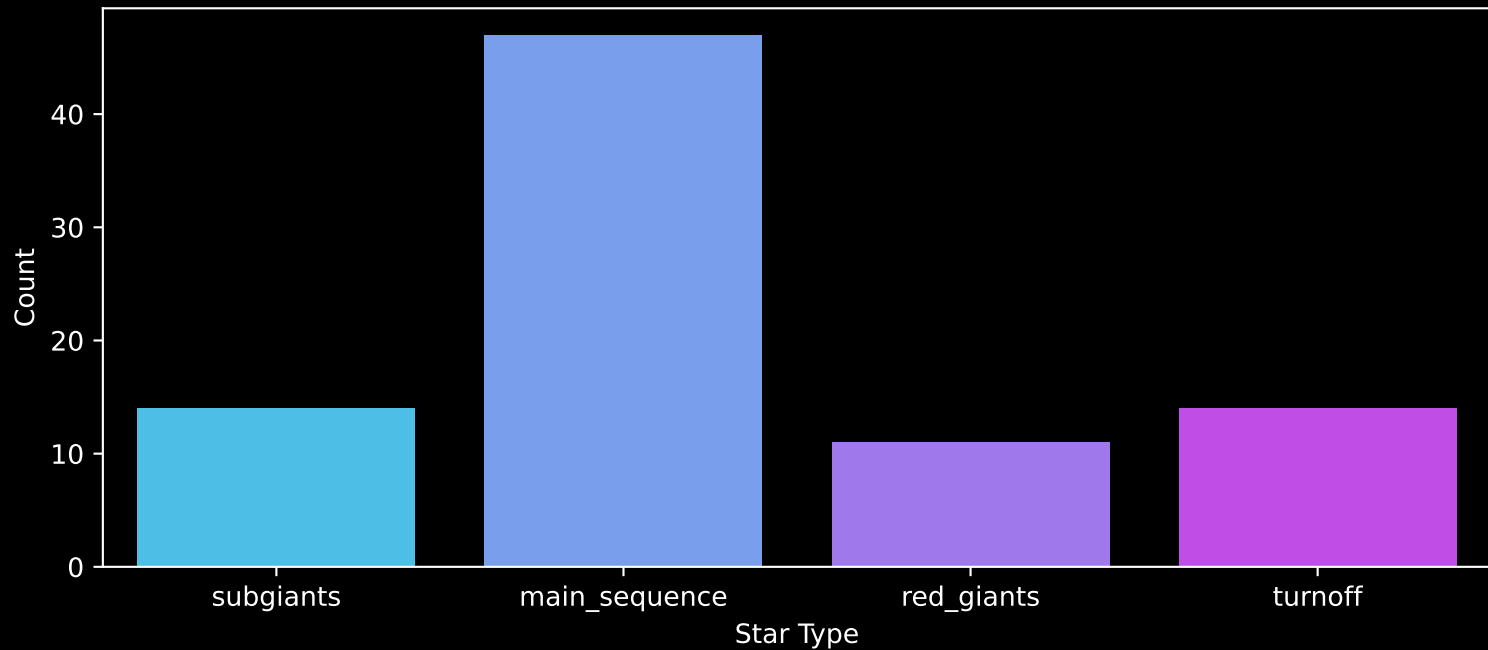
Gaia Cluster: [Stock_18] Count plot of Star Type
