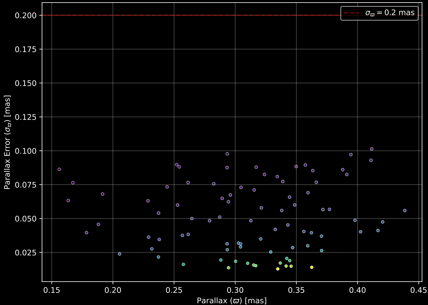
Gaia Cluster: [Stock_18] Parallax Quality (n= 86)
