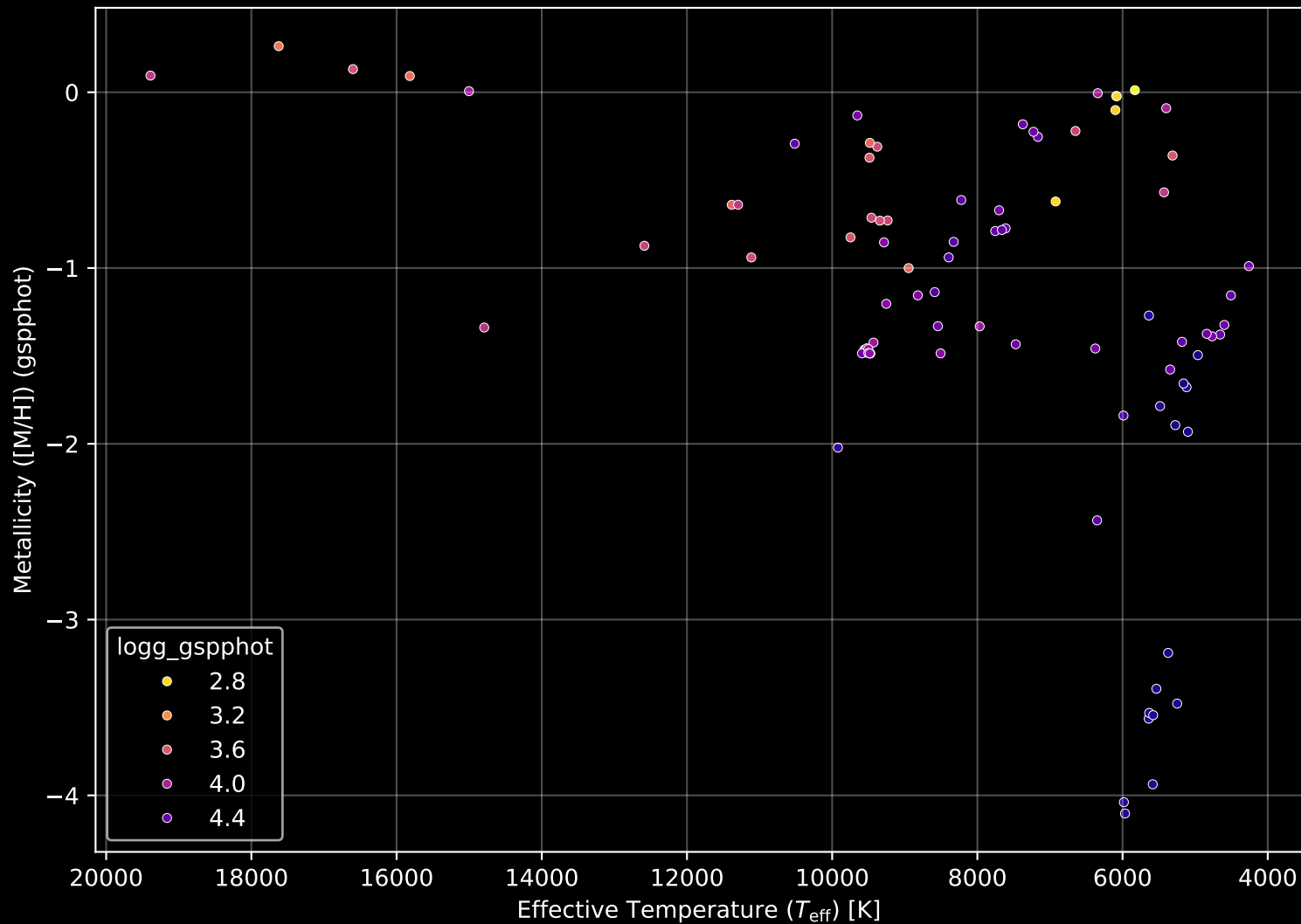
Gaia Cluster: [Stock_18] Stellar Population Parameters (n= 86)
