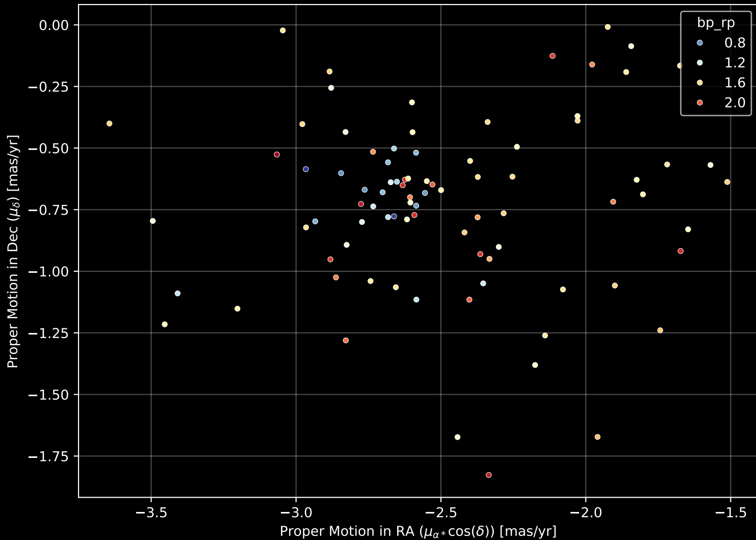
Gaia Cluster: [Stock_18] Proper Motion Diagram (n= 86)
