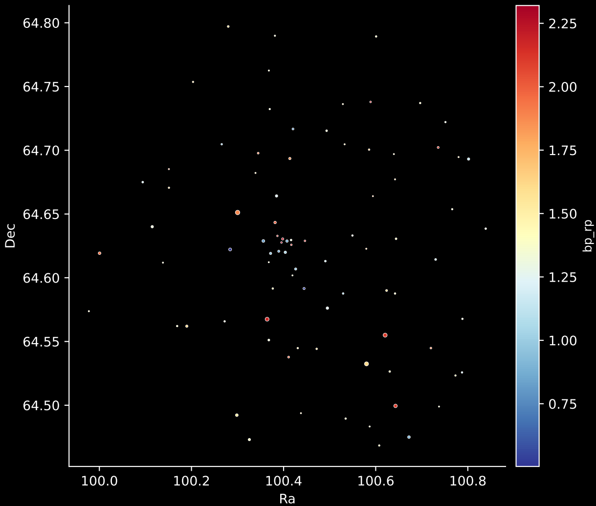
Gaia Cluster: [Stock_18] Stars: 86
