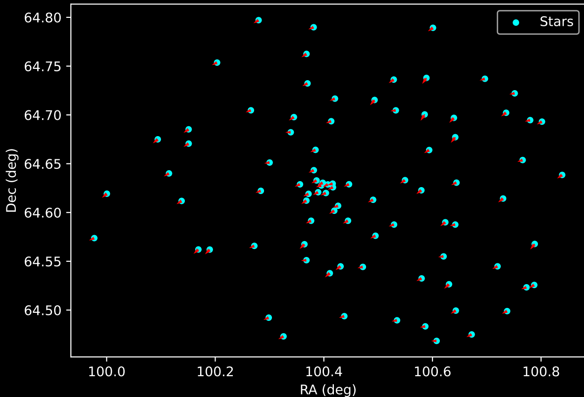
Gaia Cluster: [Stock_18] Proper Motion Vectors for Gaia Star Field (n= 86)
