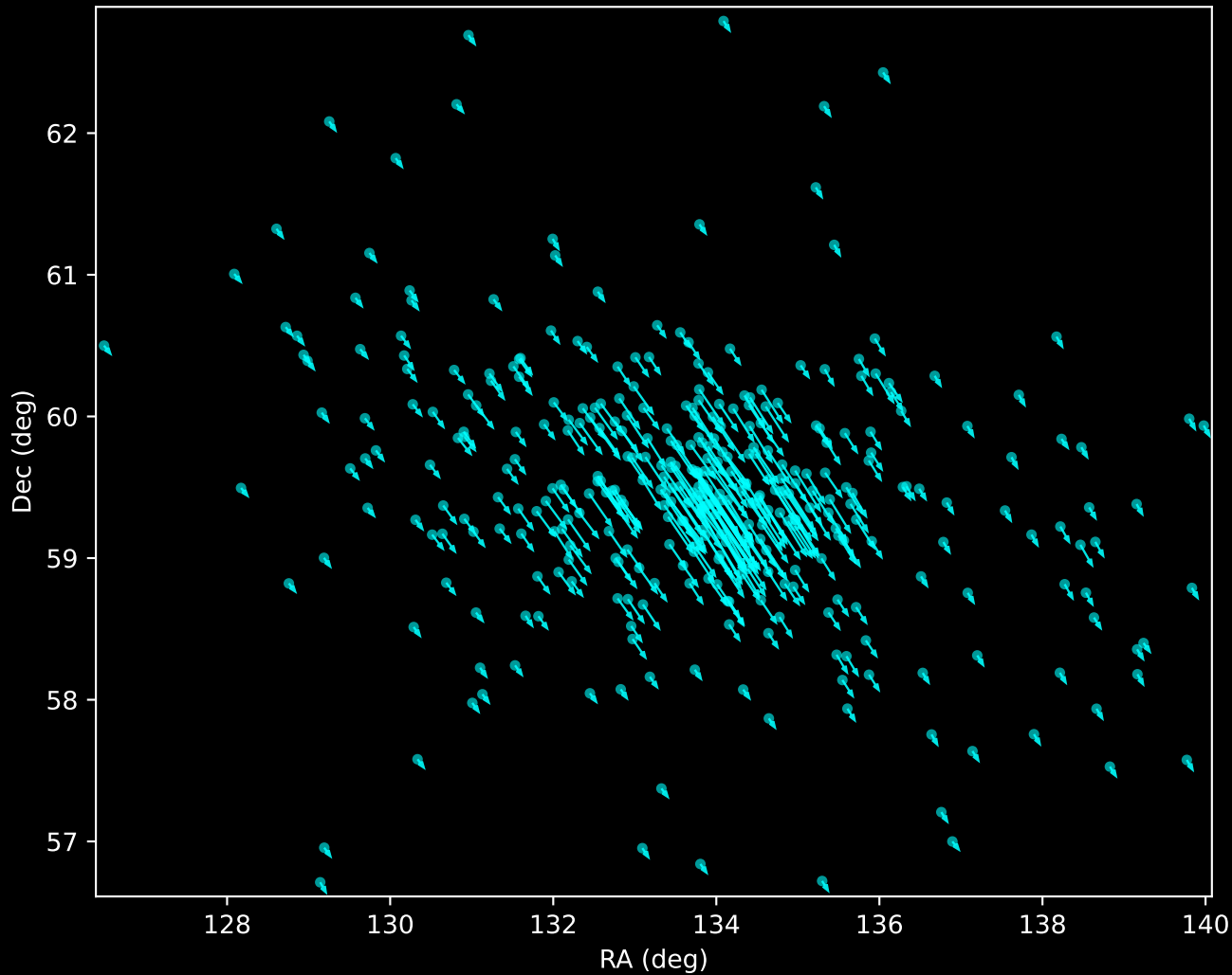
Gaia DR3 Noise Stream Proper Motion Vectors (n=360)
