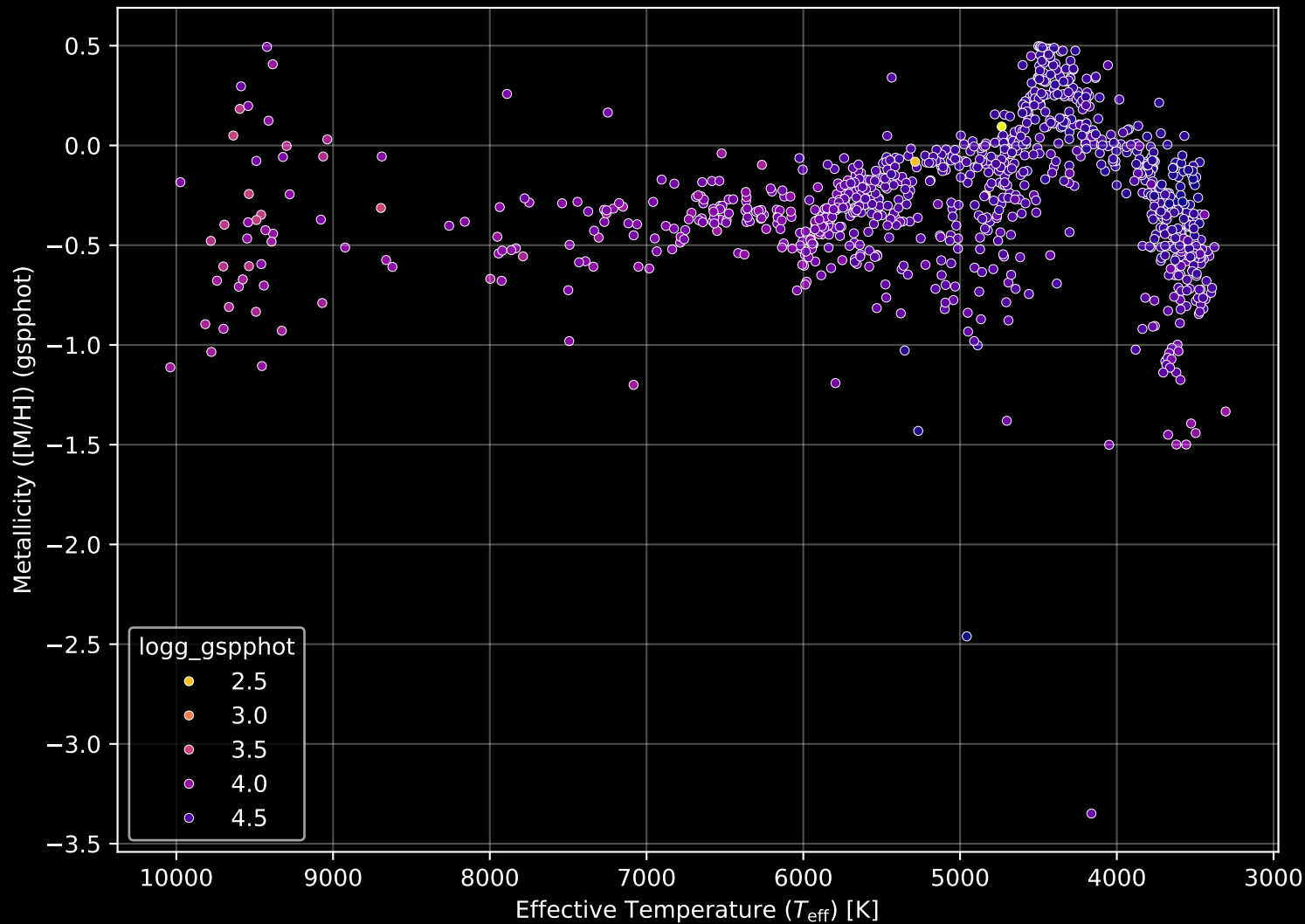
Gaia Cluster: [Stock_2] Stellar Population Parameters (n= 995)
