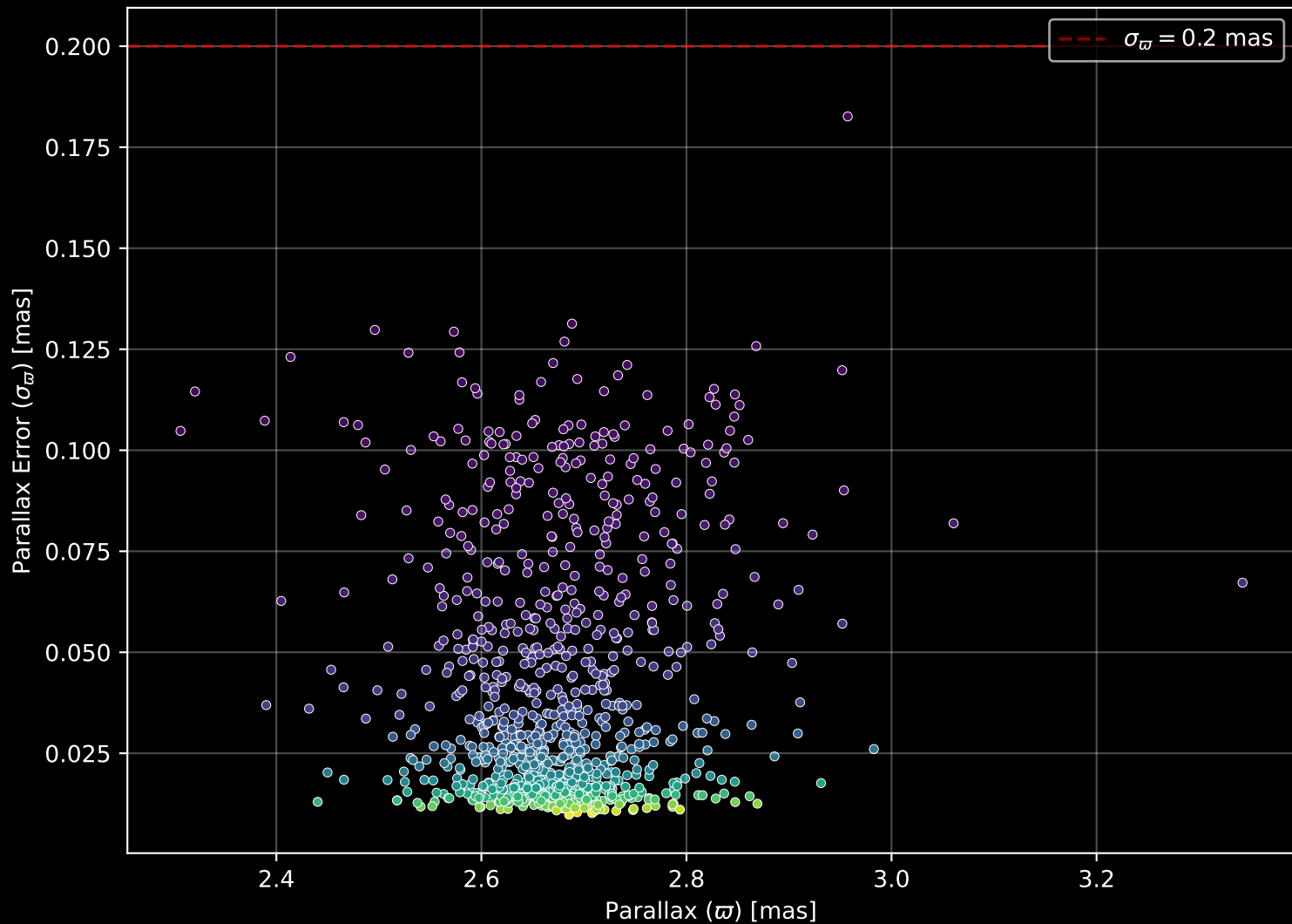
Gaia Cluster: [Stock_2] Parallax Quality (n= 995)
