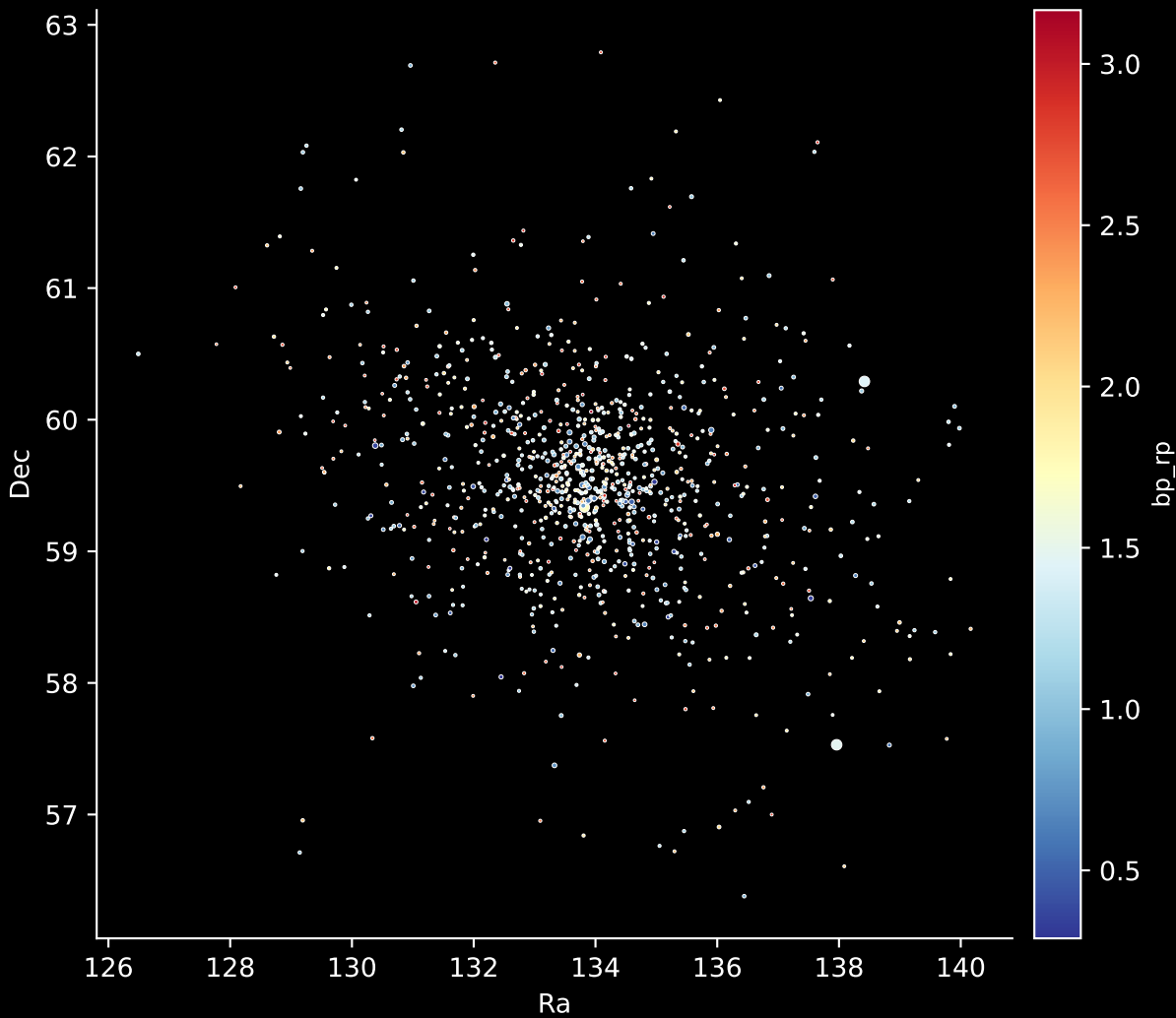
Gaia Cluster: [Stock_2] Stars: 995
