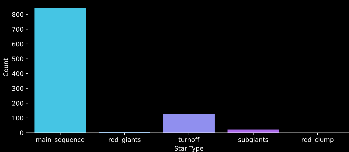
Gaia Cluster: [Stock_2] Count plot of Star Type
