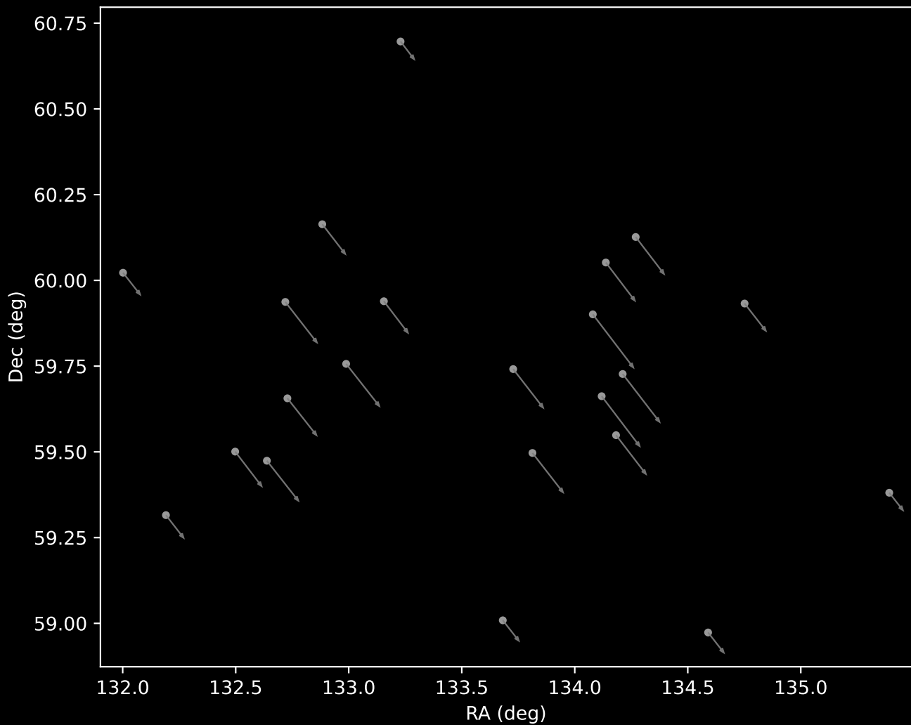
Gaia DR3 Cluster 34 Proper Motion Vectors (n=22)
