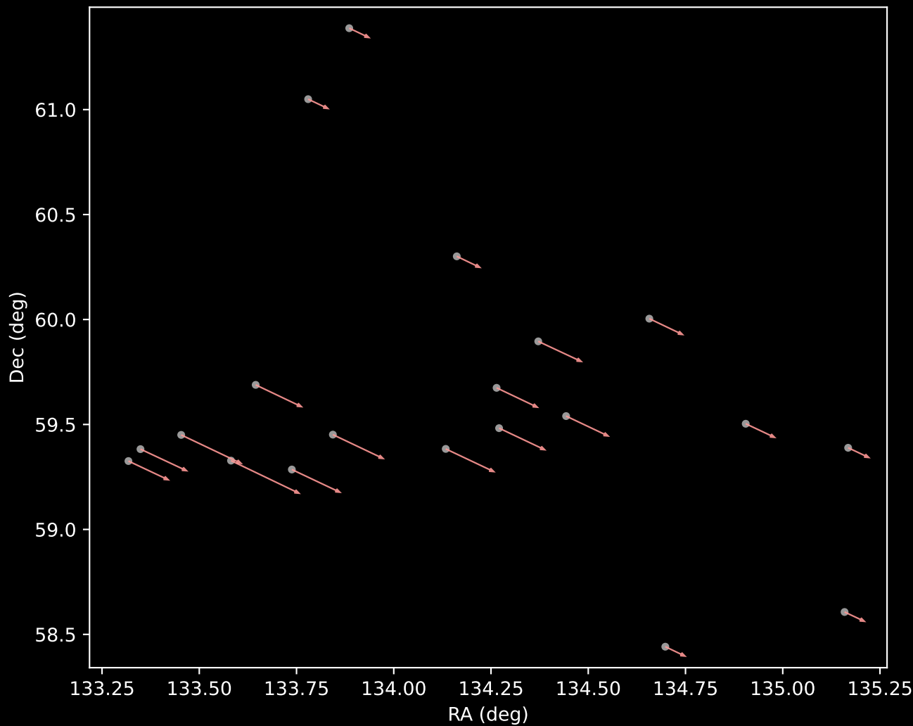
Gaia DR3 Cluster 27 Proper Motion Vectors (n=20)
