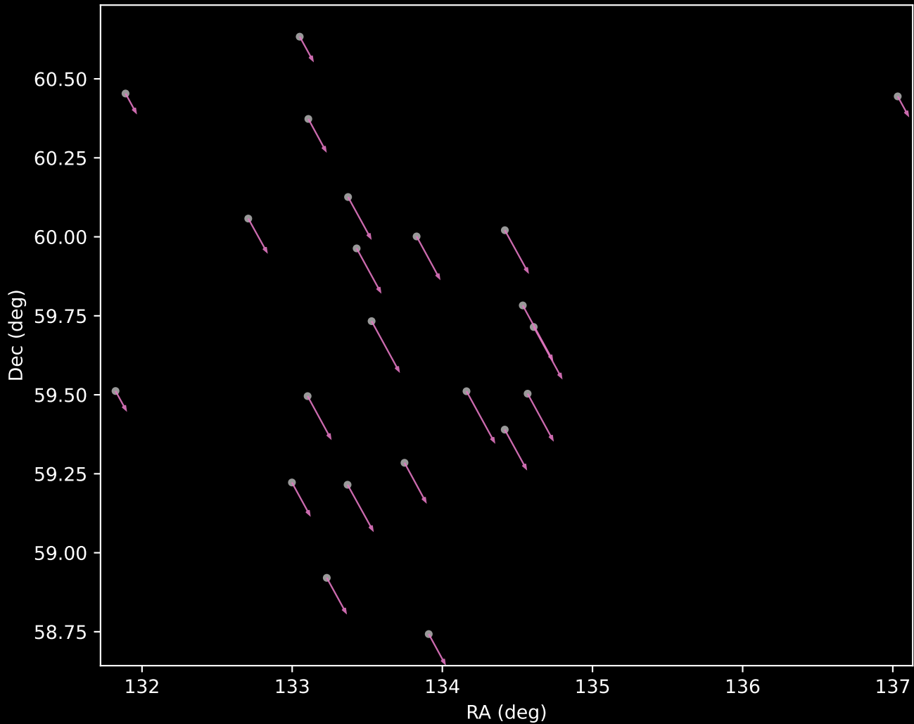
Gaia DR3 Cluster 52 Proper Motion Vectors (n=22)
