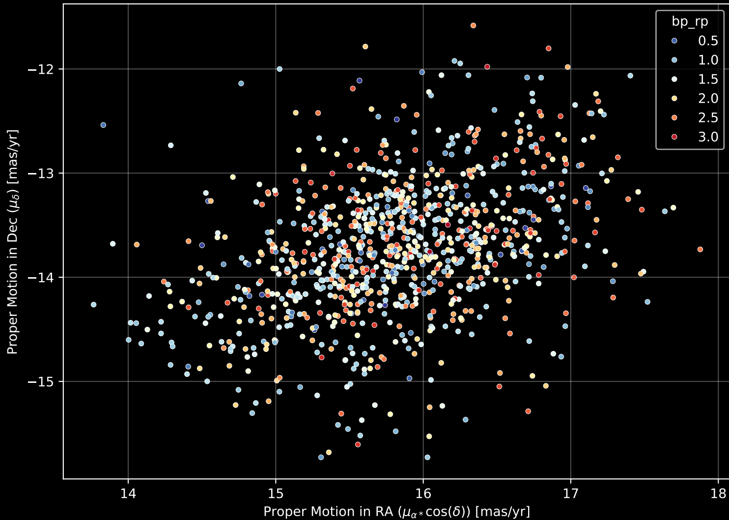
Gaia Cluster: [Stock_2] Proper Motion Diagram (n= 995)
