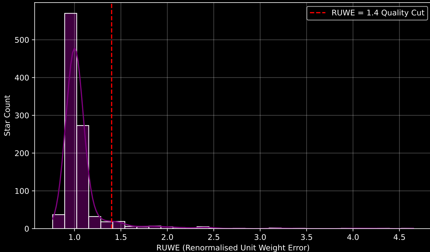
Gaia Cluster: [Stock_2] RUWE Distribution (n= 990)
