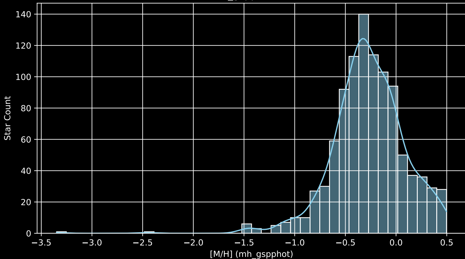
Gaia Cluster: [Stock_2 [M/H] (mh_gspphot) (n= 995)
