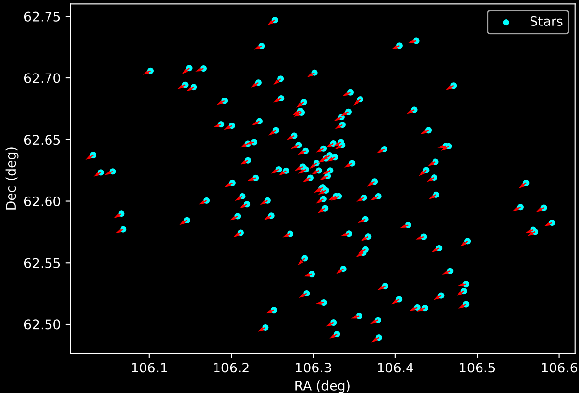
Gaia Cluster: [Stock_20] Proper Motion Vectors for Gaia Star Field (n= 121)
