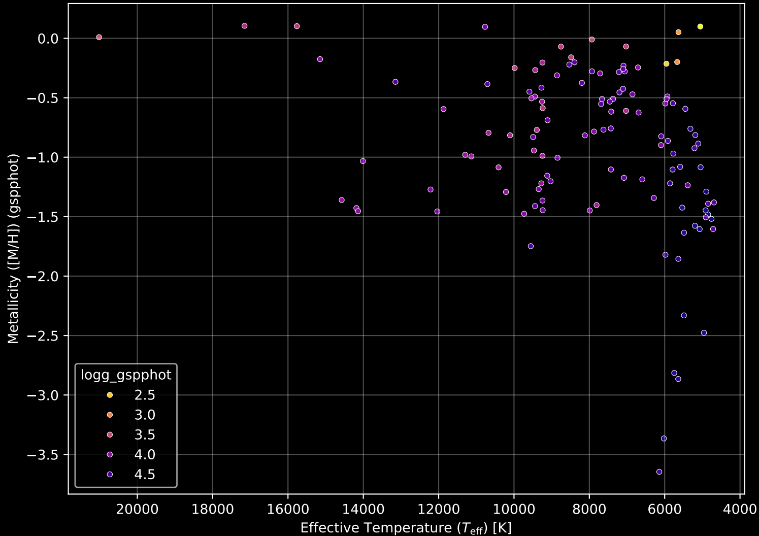
Gaia Cluster: [Stock_20] Stellar Population Parameters (n= 121)
