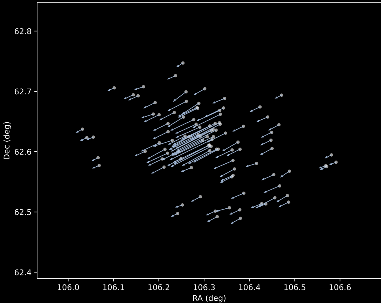
Gaia DR3 Cluster 1 Proper Motion Vectors (n=100)
