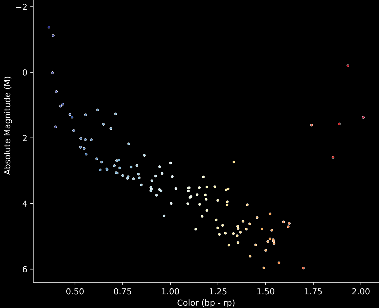
Gaia Cluster: [Stock_20] Stars (n= 121) Hertzprung-Russel Diagram
