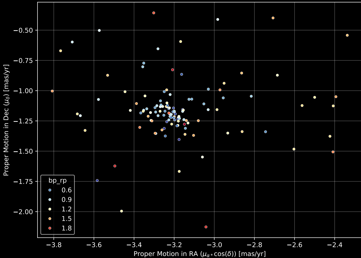
Gaia Cluster: [Stock_20] Proper Motion Diagram (n= 121)
