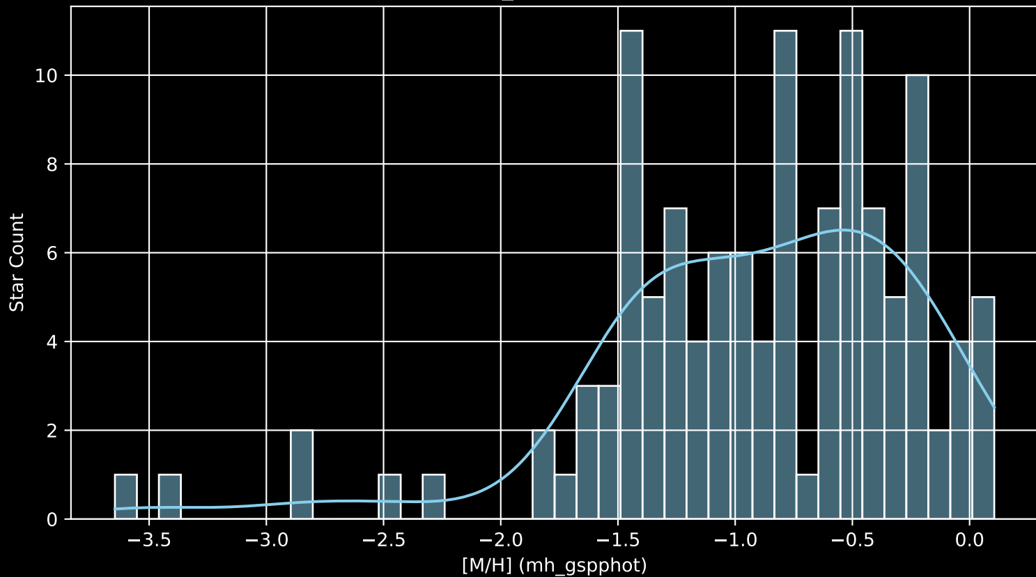
Gaia Cluster: [Stock_20 [M/H] (mh_gspphot) (n= 121)
