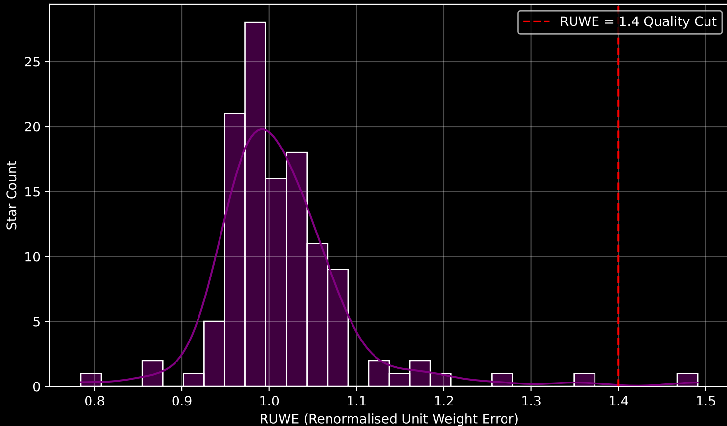
Gaia Cluster: [Stock_20] RUWE Distribution (n= 121)
