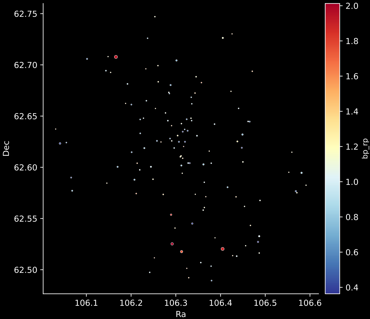
Gaia Cluster: [Stock_20] Stars: 121
