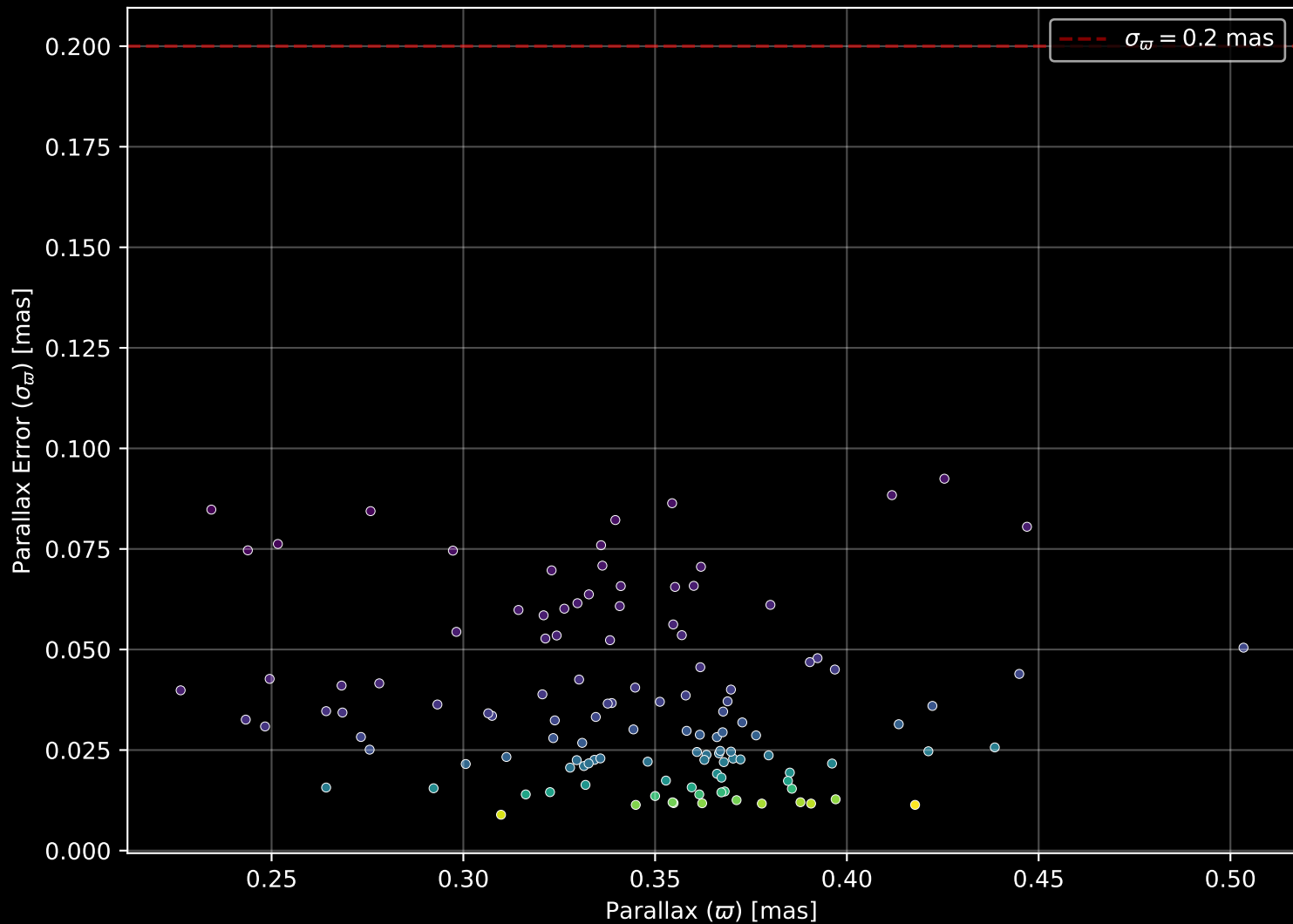
Gaia Cluster: [Stock_20] Parallax Quality (n= 121)
