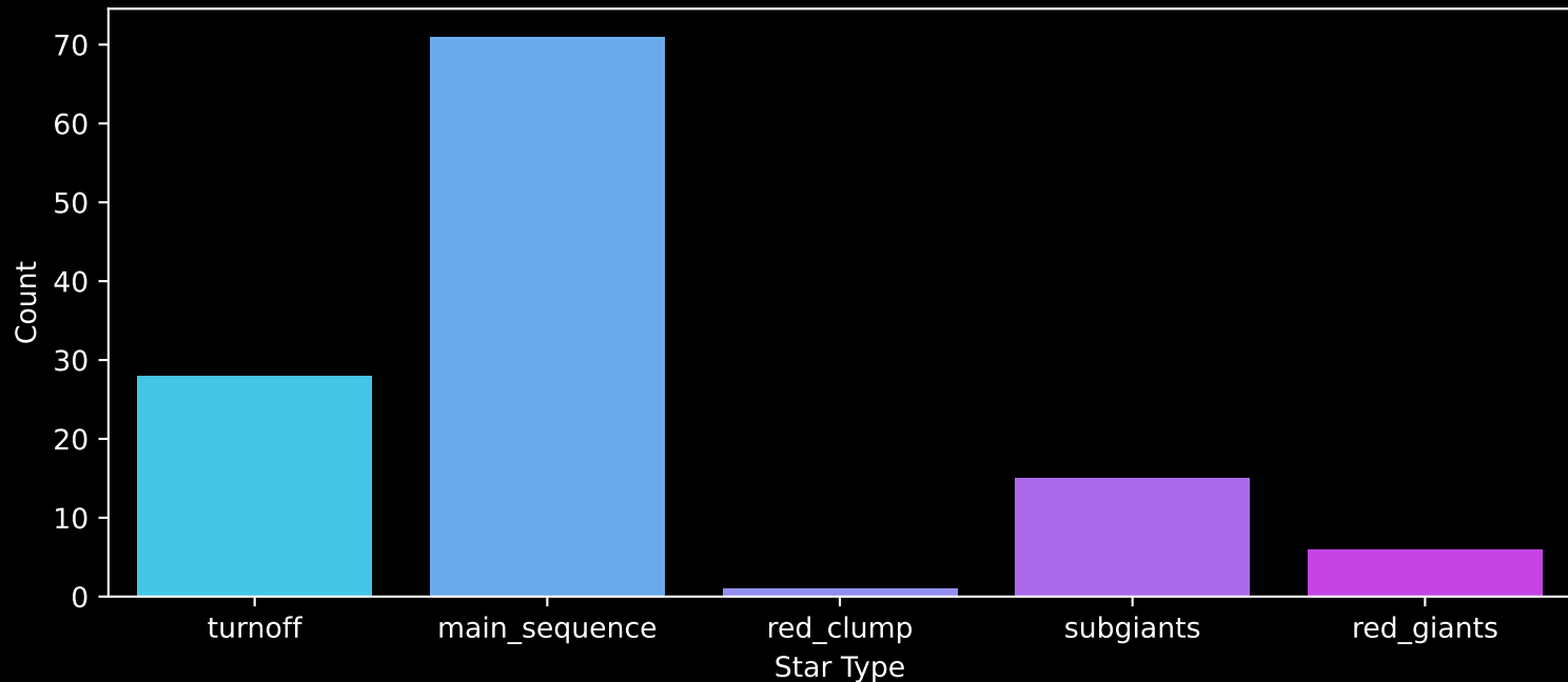
Gaia Cluster: [Stock_20] Count plot of Star Type
