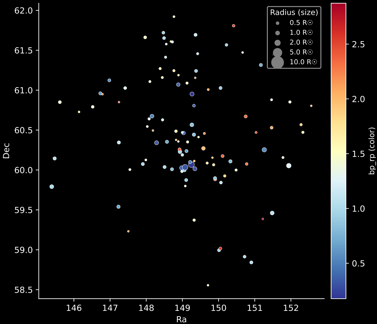
Gaia Cluster: [Stock_23] Stars: 111
