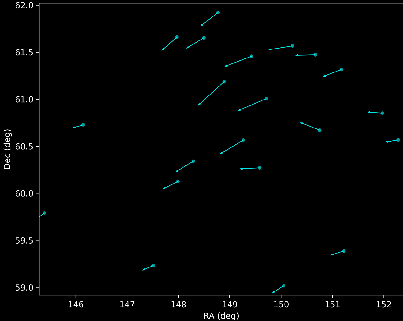
Gaia DR3 Noise Stream Proper Motion Vectors (n=21)
