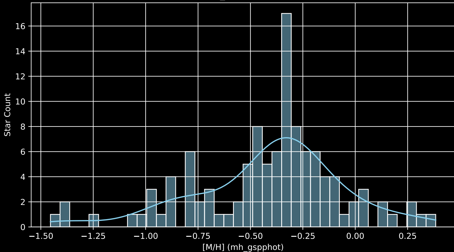
Gaia Cluster: [Stock_23 [M/H] (mh_gspphot) (n= 111)
