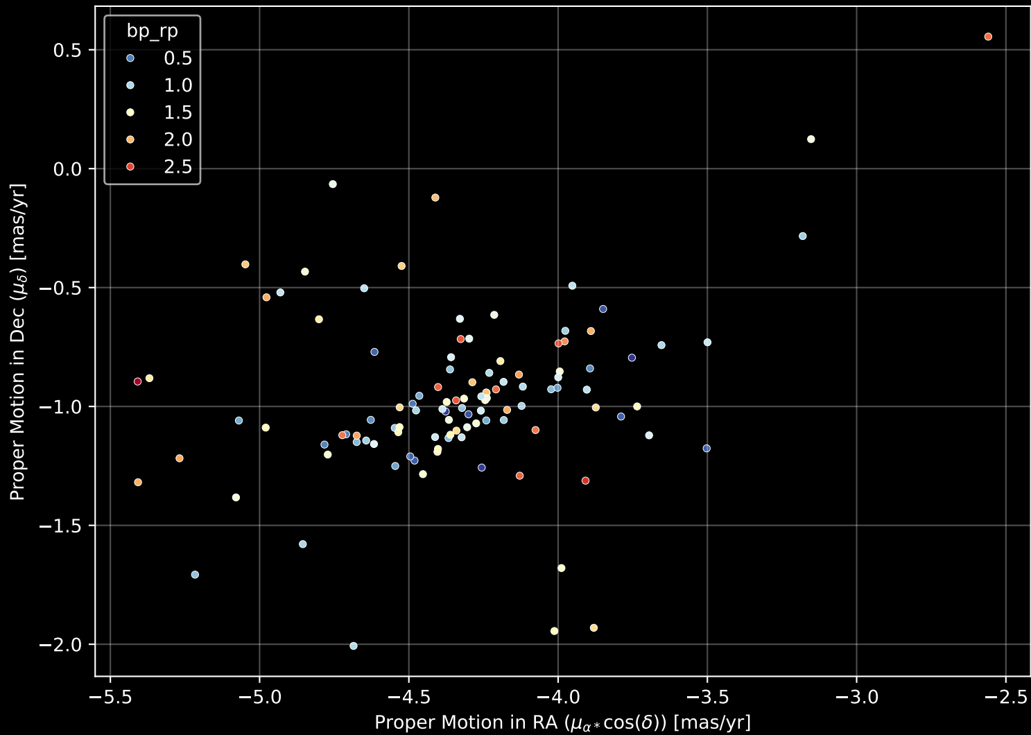
Gaia Cluster: [Stock_23] Proper Motion Diagram (n= 111)
