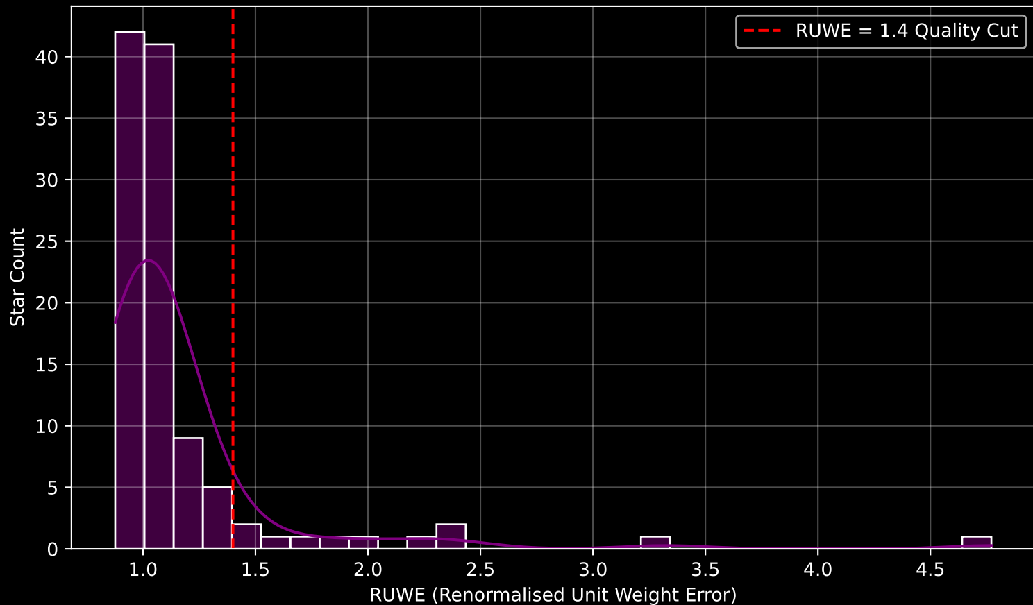
Gaia Cluster: [Stock_23] RUWE Distribution (n= 108)
