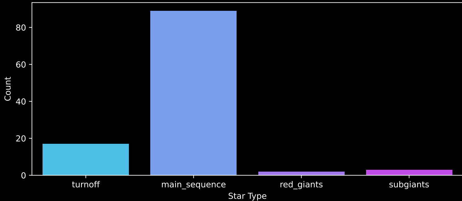
Gaia Cluster: [Stock_23] Count plot of Star Type
