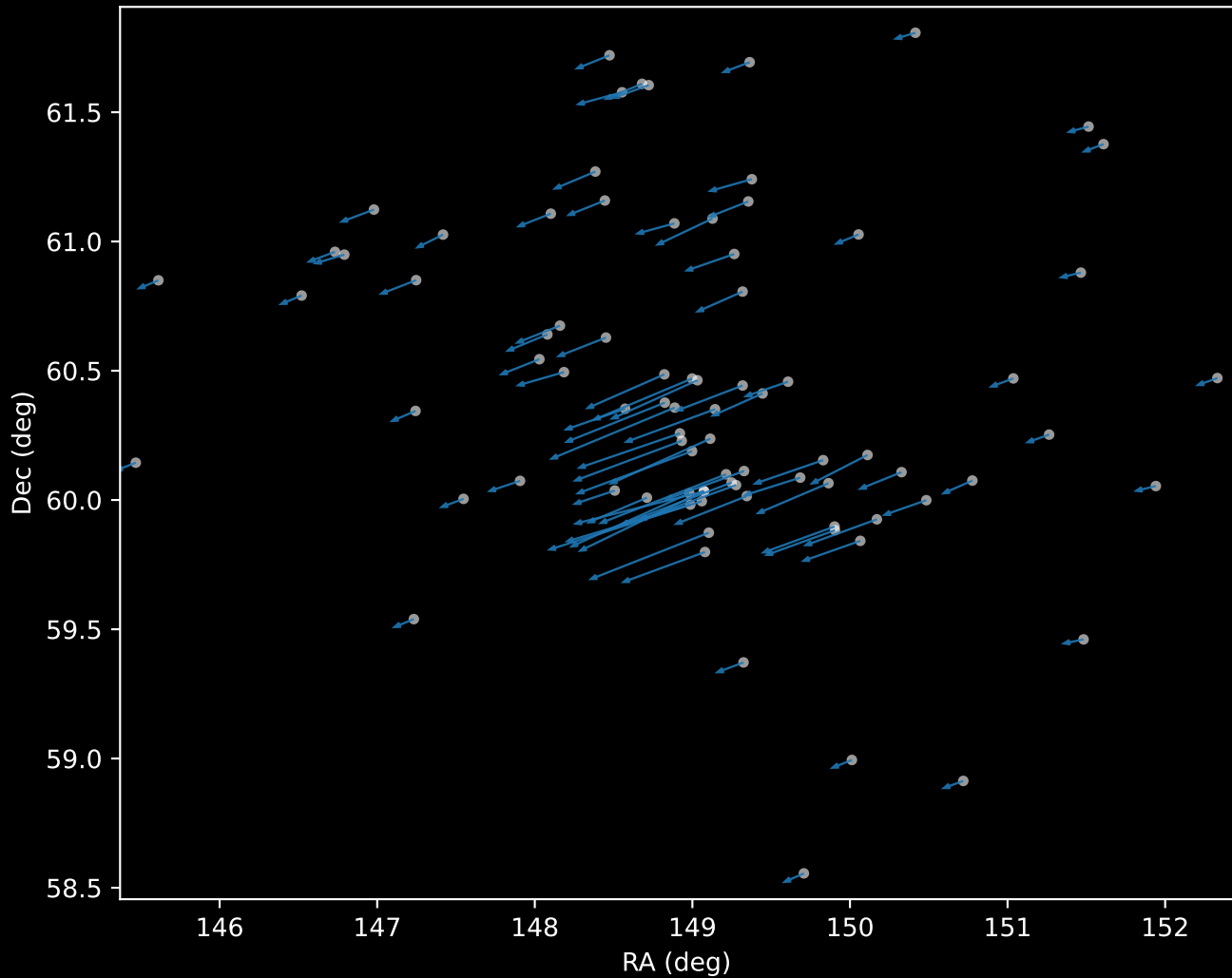
Gaia DR3 Cluster 0 Proper Motion Vectors (n=84)
