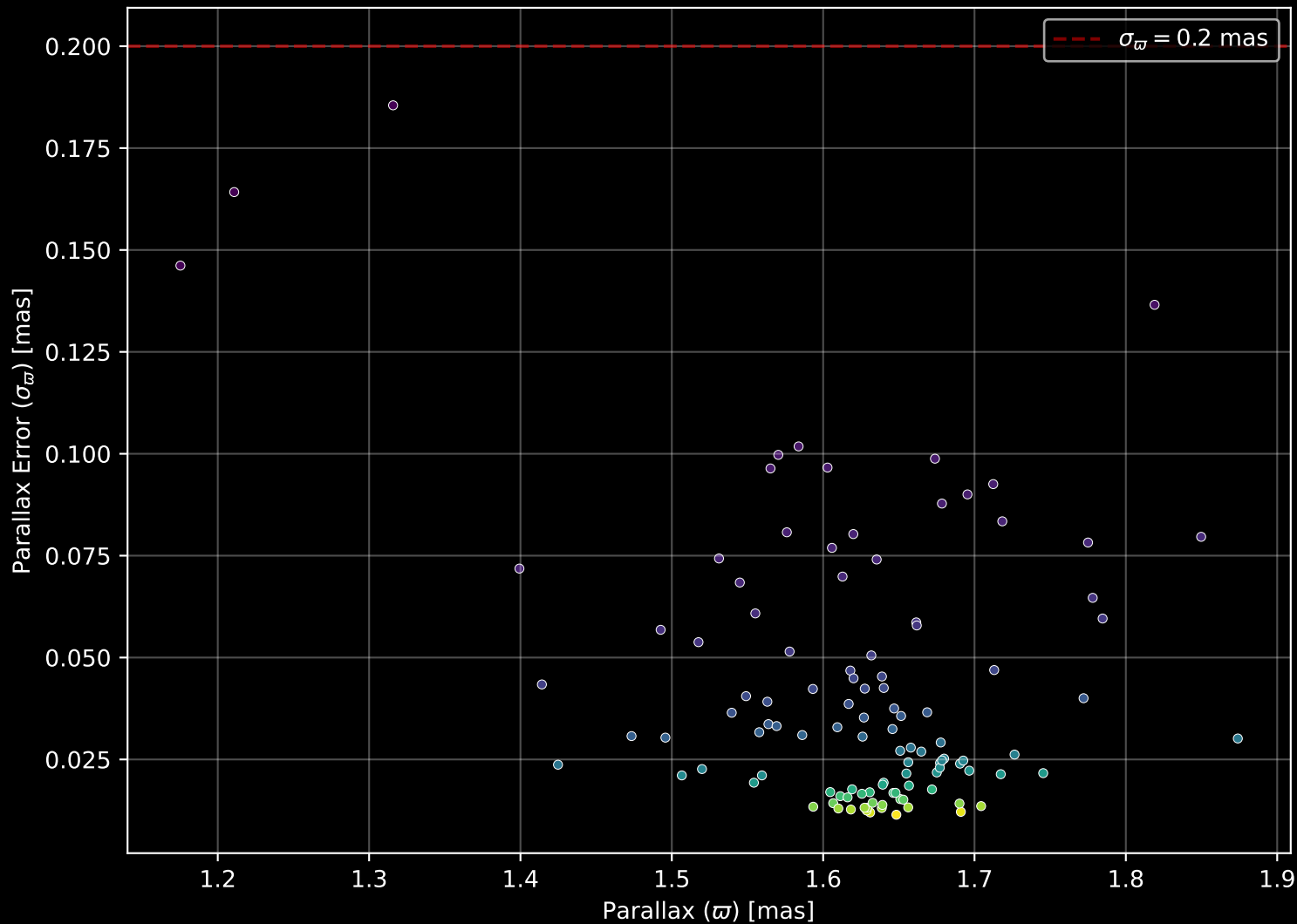
Gaia Cluster: [Stock_23] Parallax Quality (n= 111)
