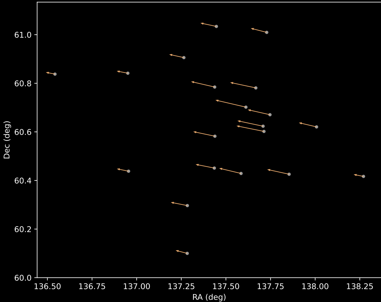
Gaia DR3 Cluster 3 Proper Motion Vectors (n=20)
