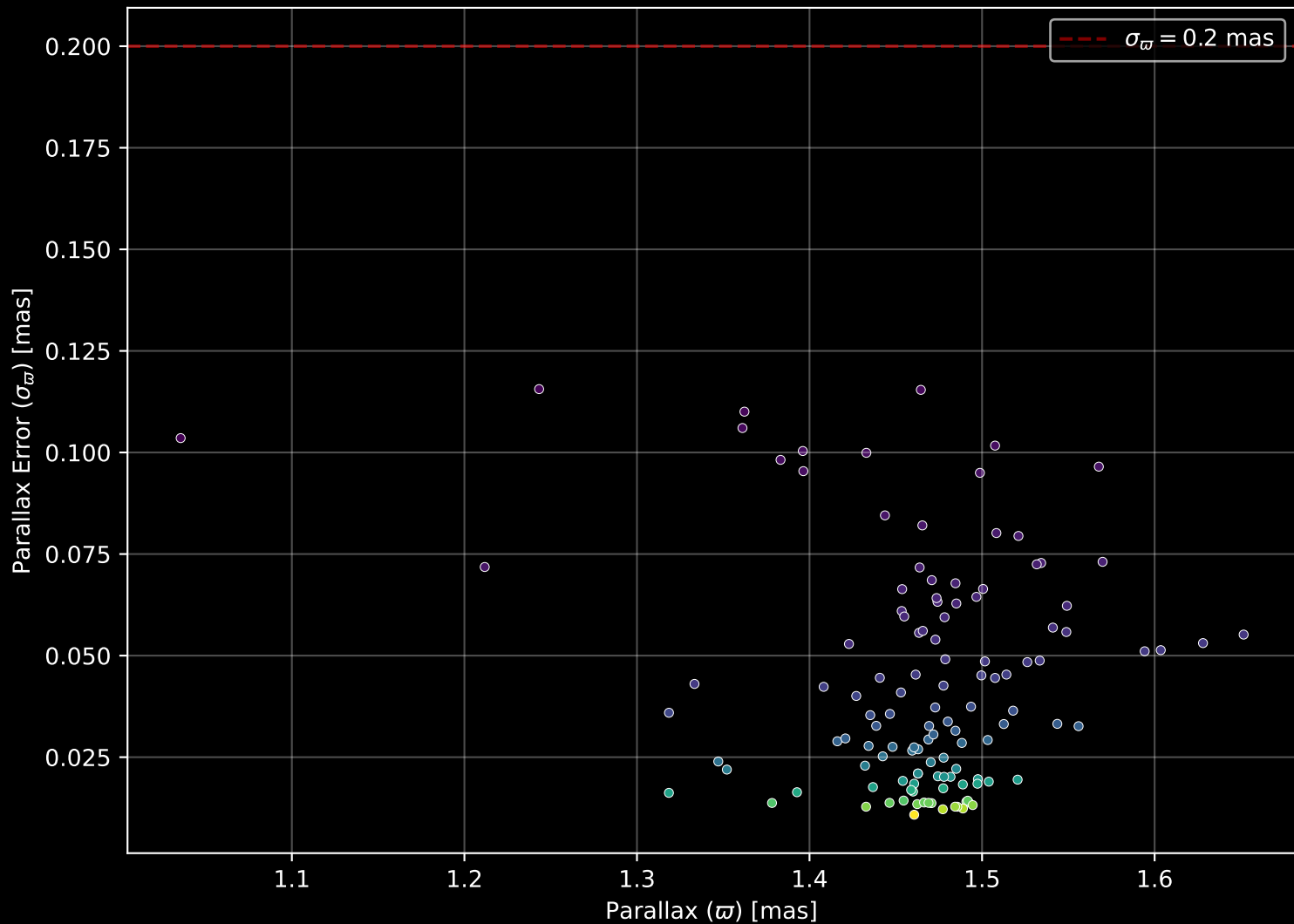
Gaia Cluster: [Stock_7] Parallax Quality (n= 123)
