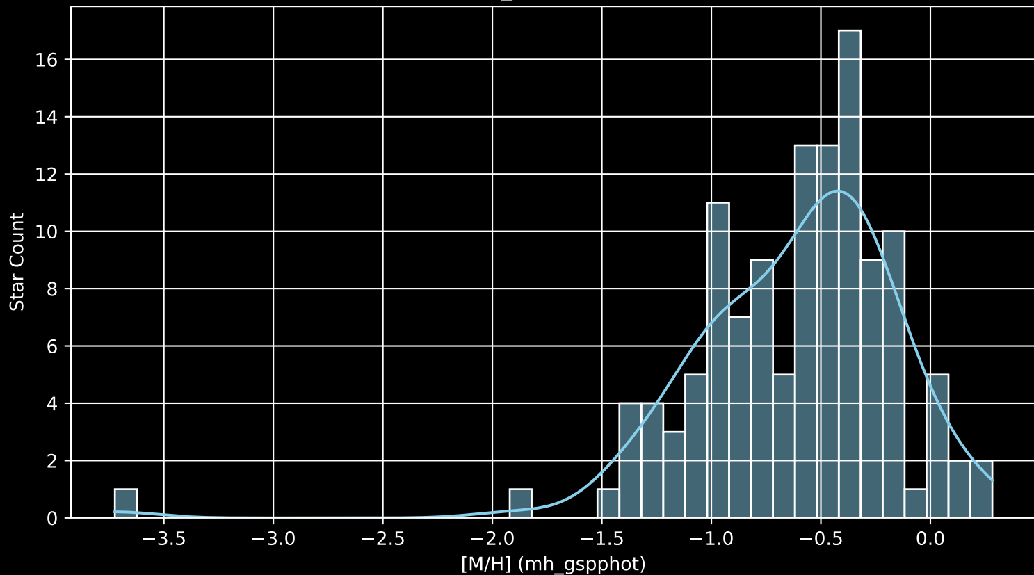
Gaia Cluster: [Stock_7 [M/H] (mh_gspphot) (n= 123)
