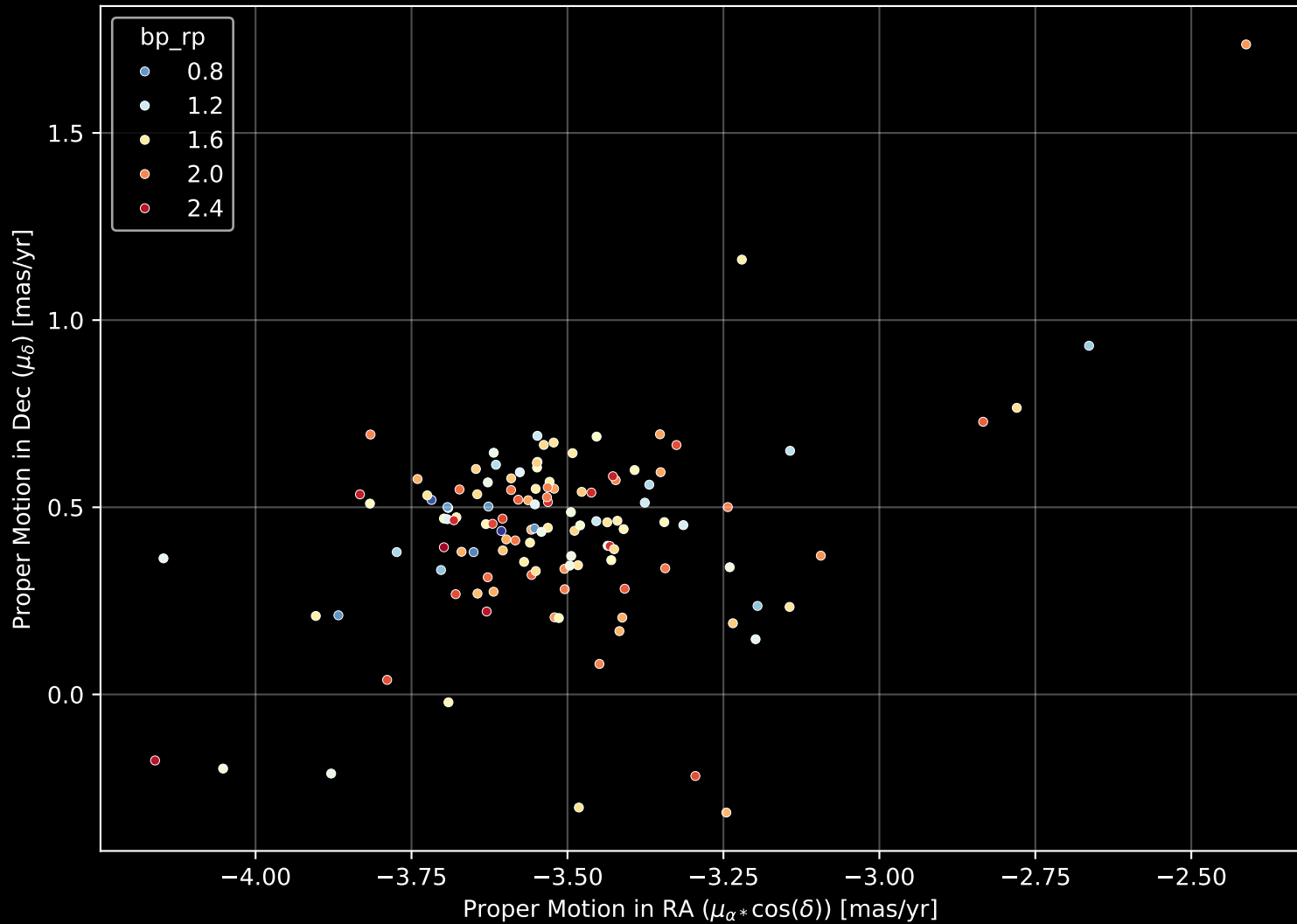
Gaia Cluster: [Stock_7] Proper Motion Diagram (n= 123)
