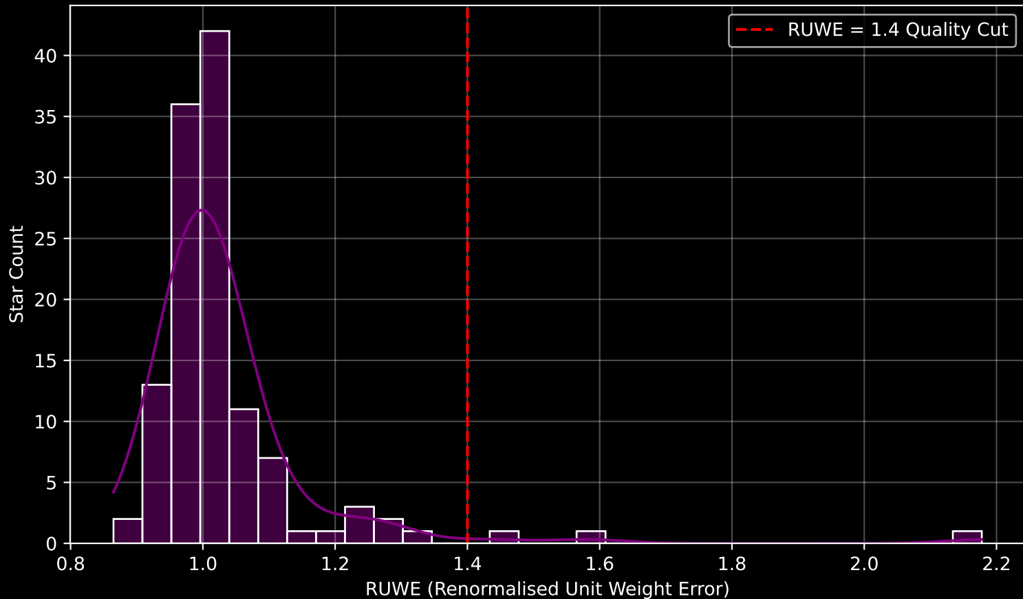
Gaia Cluster: [Stock_7] RUWE Distribution (n= 122)
