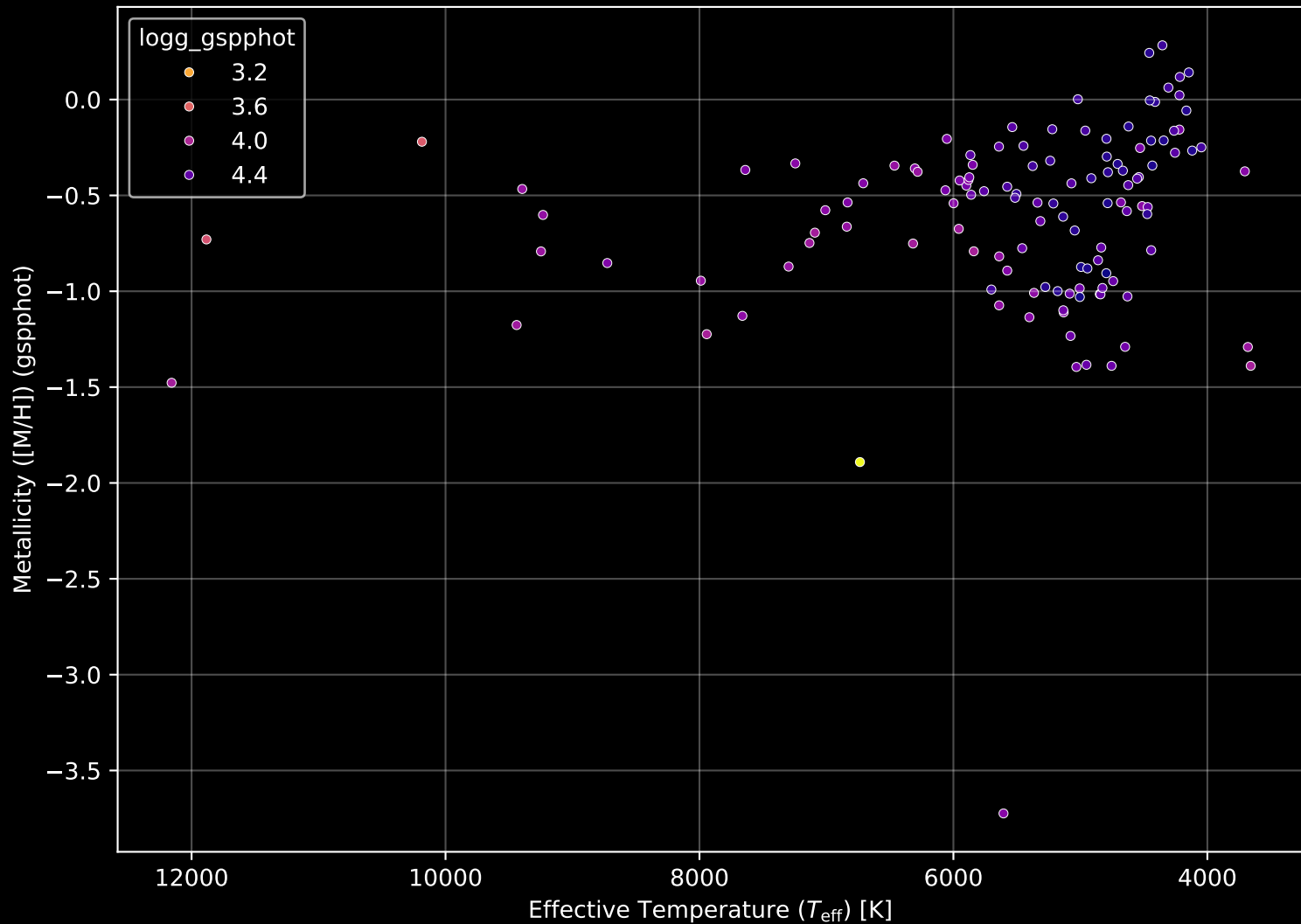
Gaia Cluster: [Stock_7] Stellar Population Parameters (n= 123)
