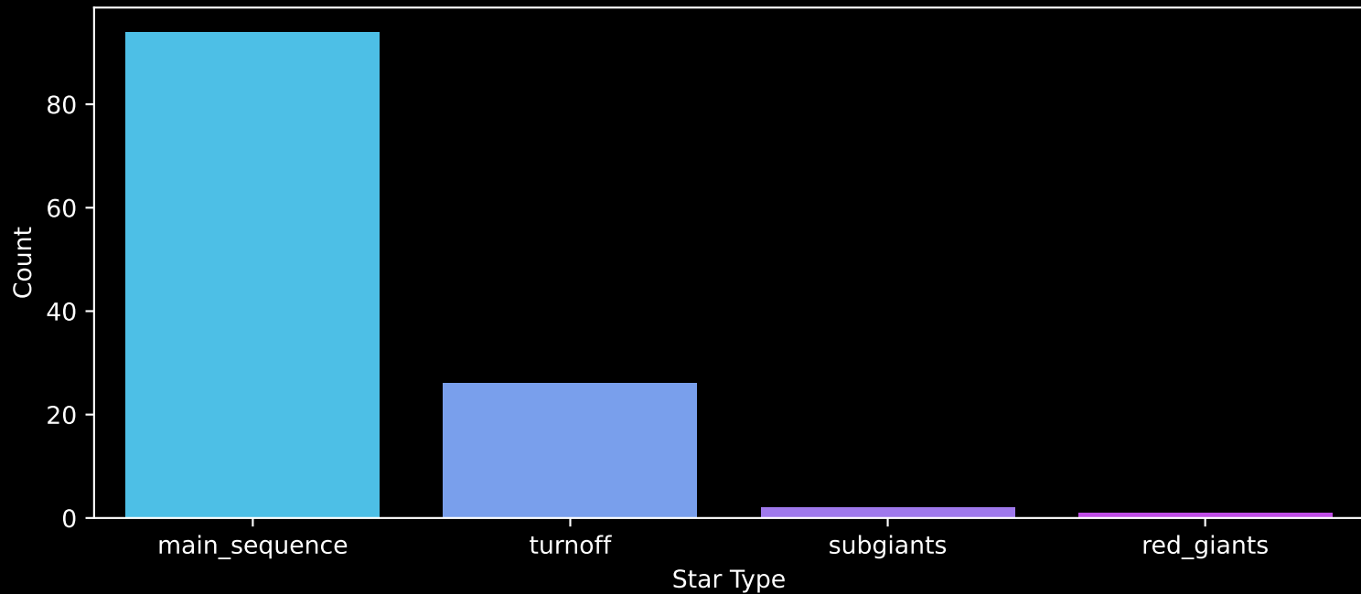
Gaia Cluster: [Stock_7] Count plot of Star Type
