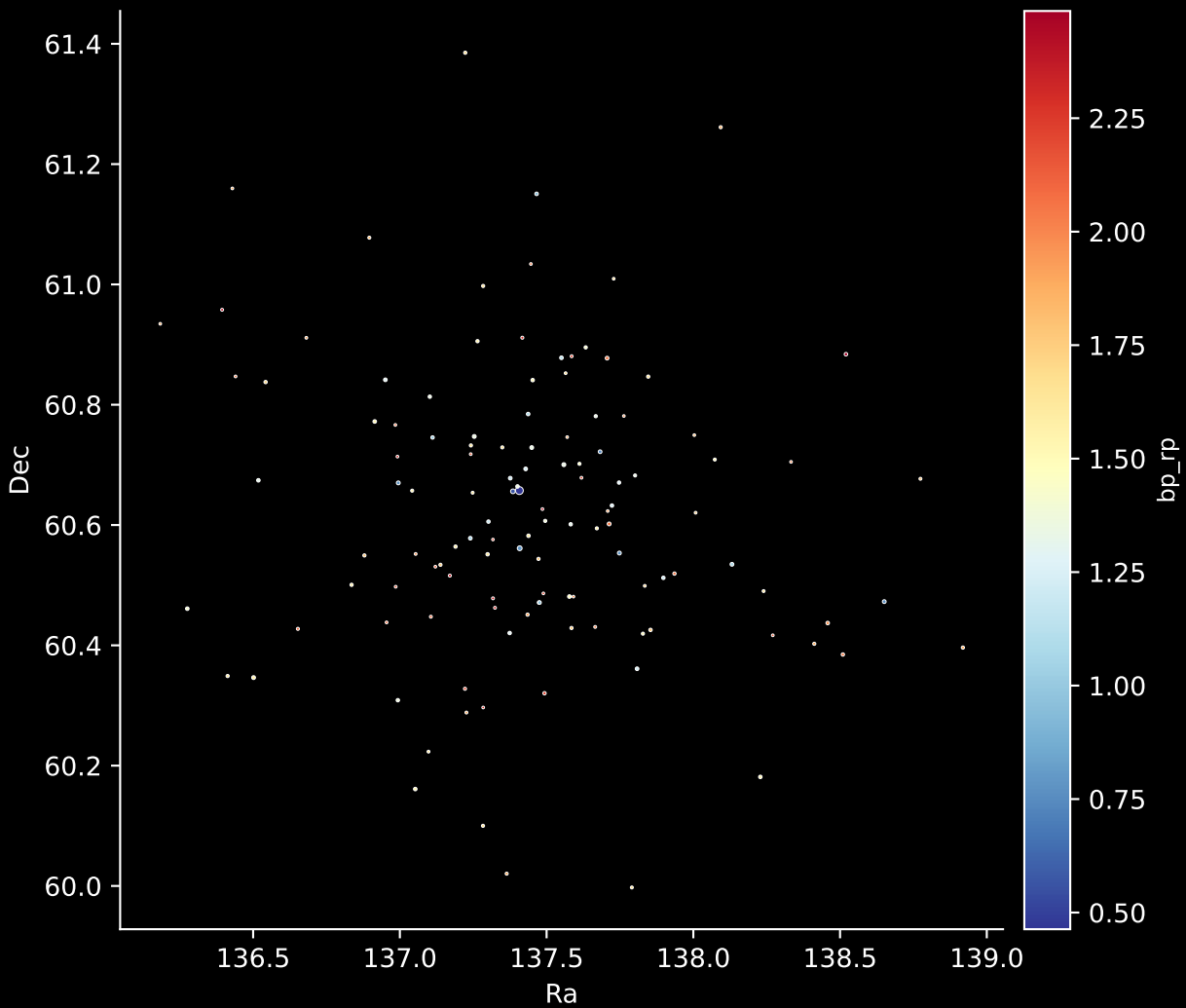
Gaia Cluster: [Stock_7] Stars: 123
