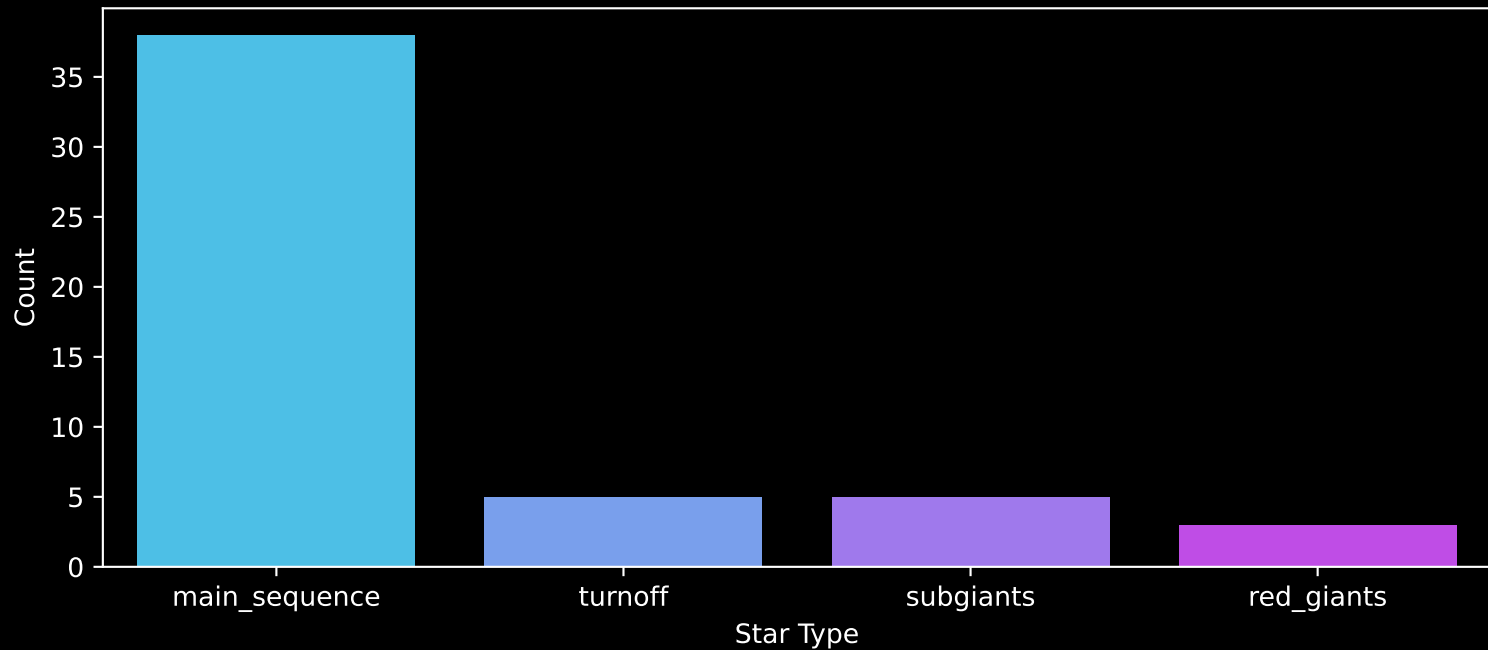
Gaia Cluster: [Teutsch_1] Count plot of Star Type
