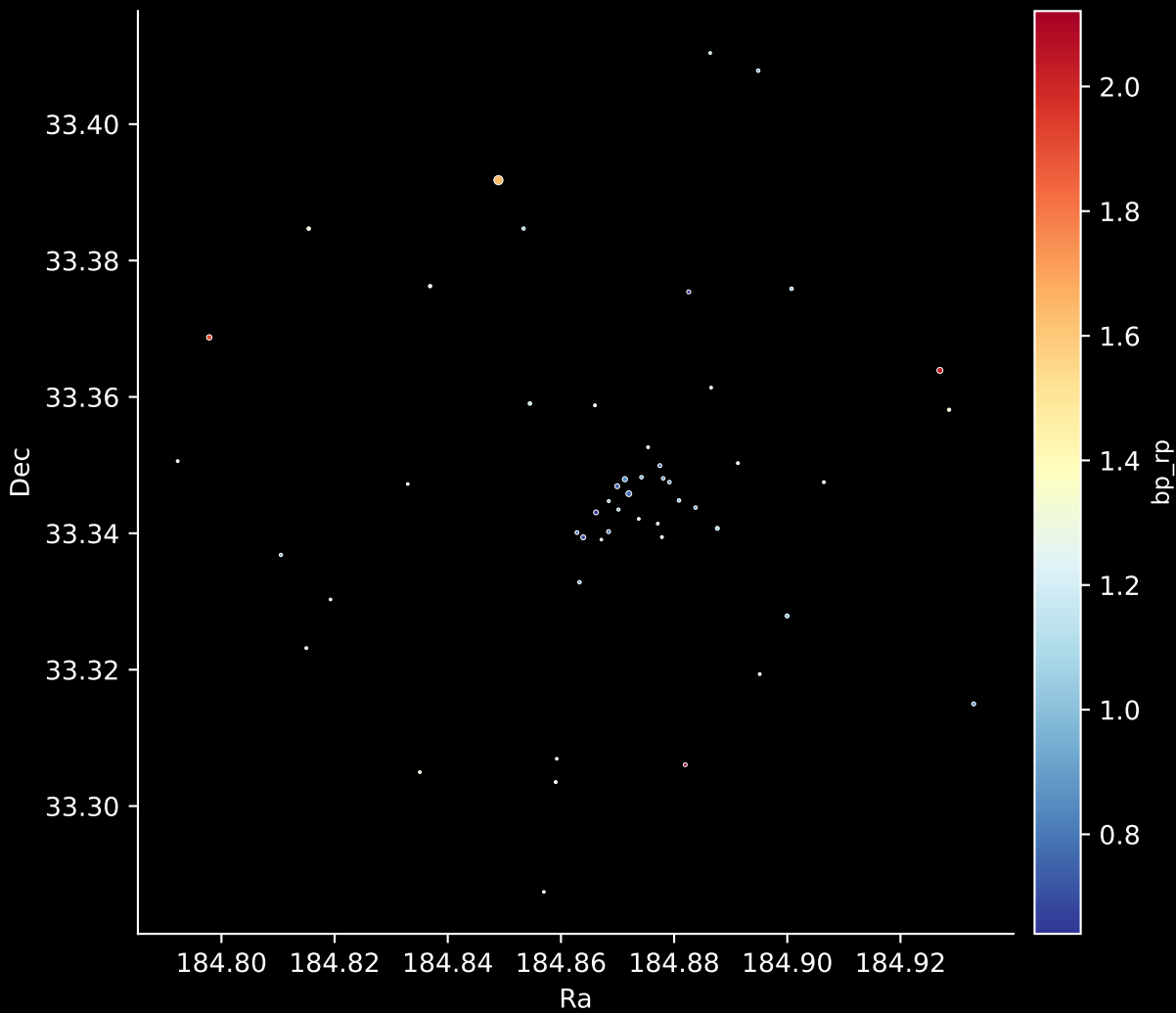
Gaia Cluster: [Teutsch_1] Stars: 51
