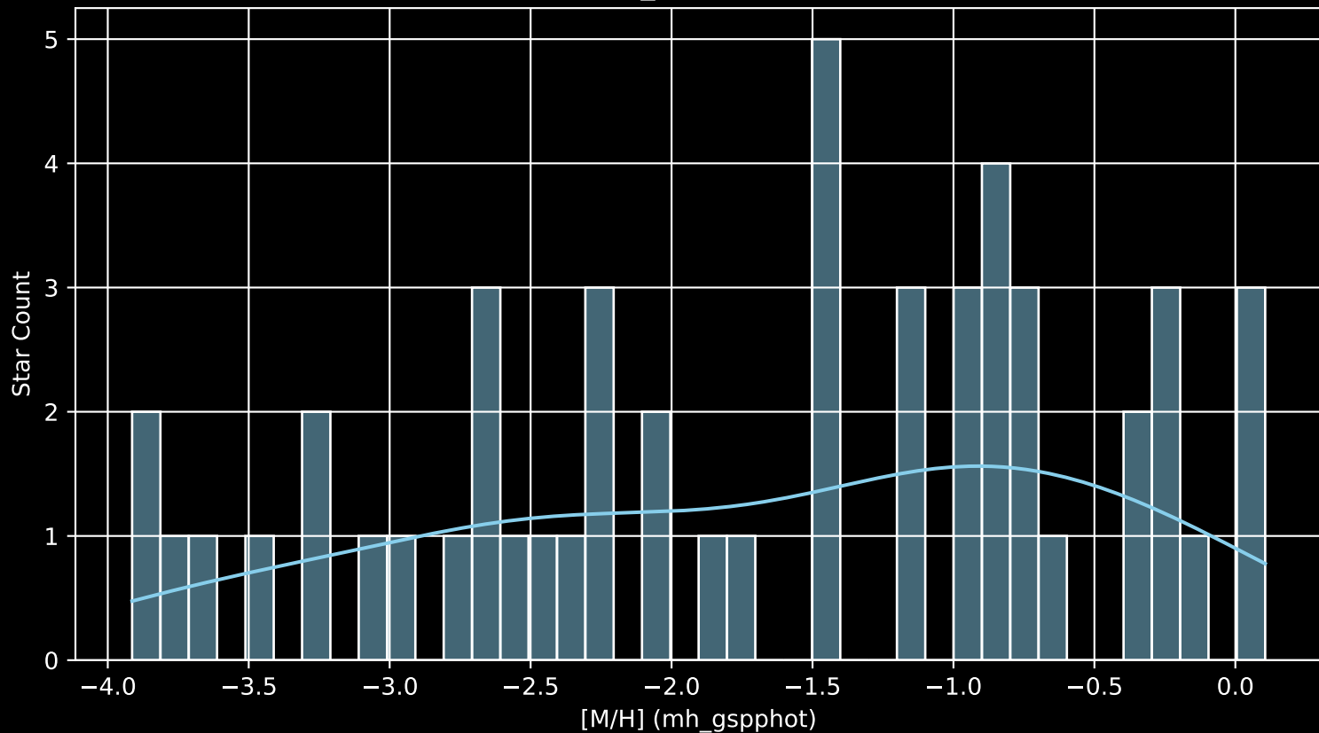
Gaia Cluster: [Deutsch_1 [M/H] (mh_gspphot) (n= 51)
