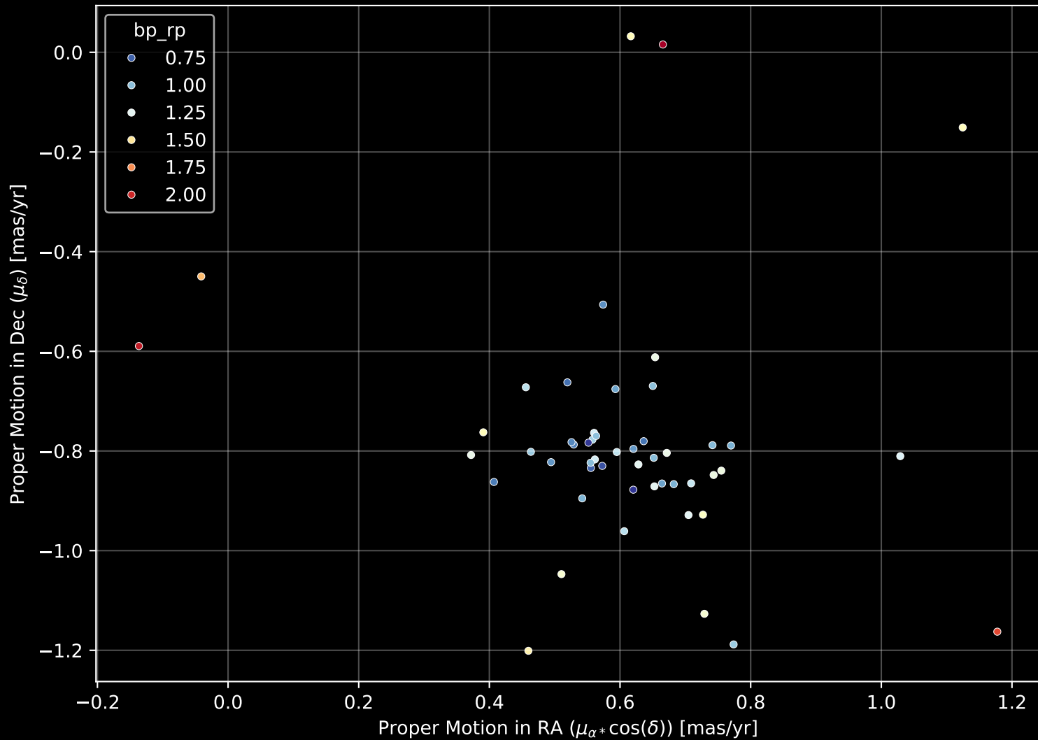
Gaia Cluster: [Teutsch_1] Proper Motion Diagram (n= 51)
