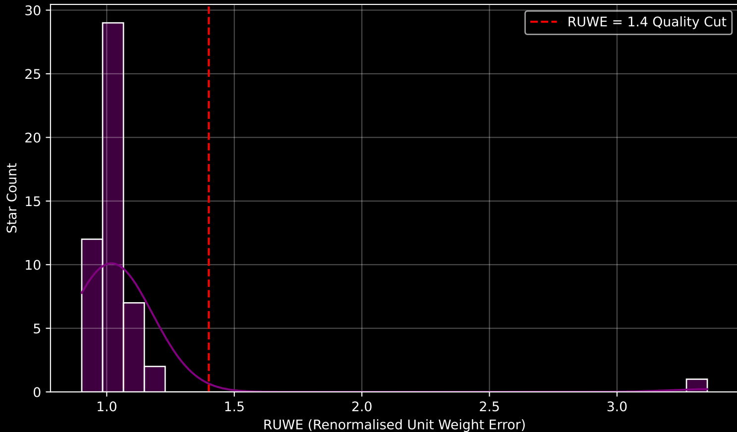
Gaia Cluster: [Teutsch_1] RUWE Distribution (n= 51)
