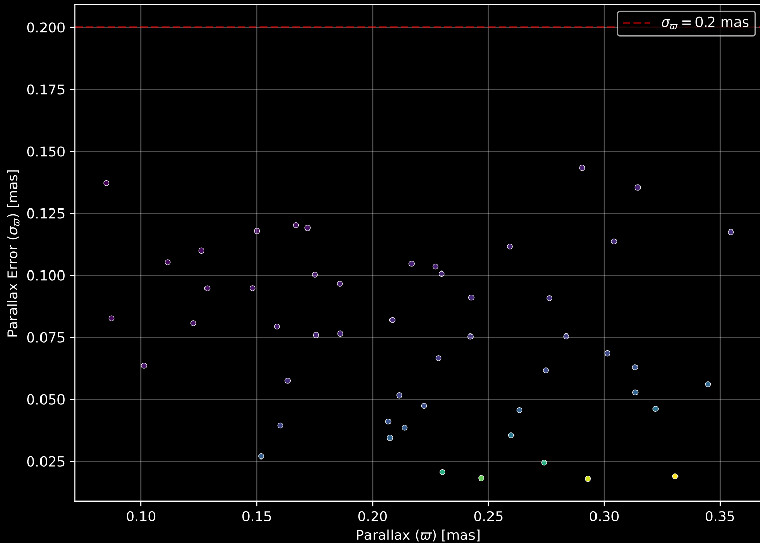
Gaia Cluster: [Teutsch_1] Parallax Quality (n= 51)
