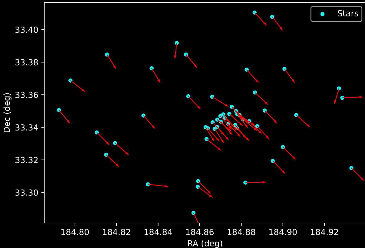
Gaia Cluster: [Teutsch_1] Proper Motion Vectors for Gaia Star Field (n= 51)
