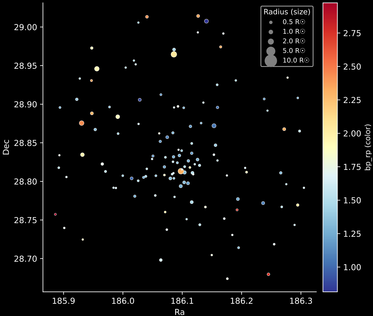
Gaia Cluster: [Teutsch_10] Stars: 128
