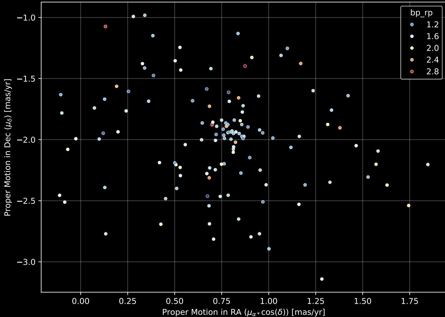
Gaia Cluster: [Deutsch_10] Proper Motion Diagram (n= 128)
