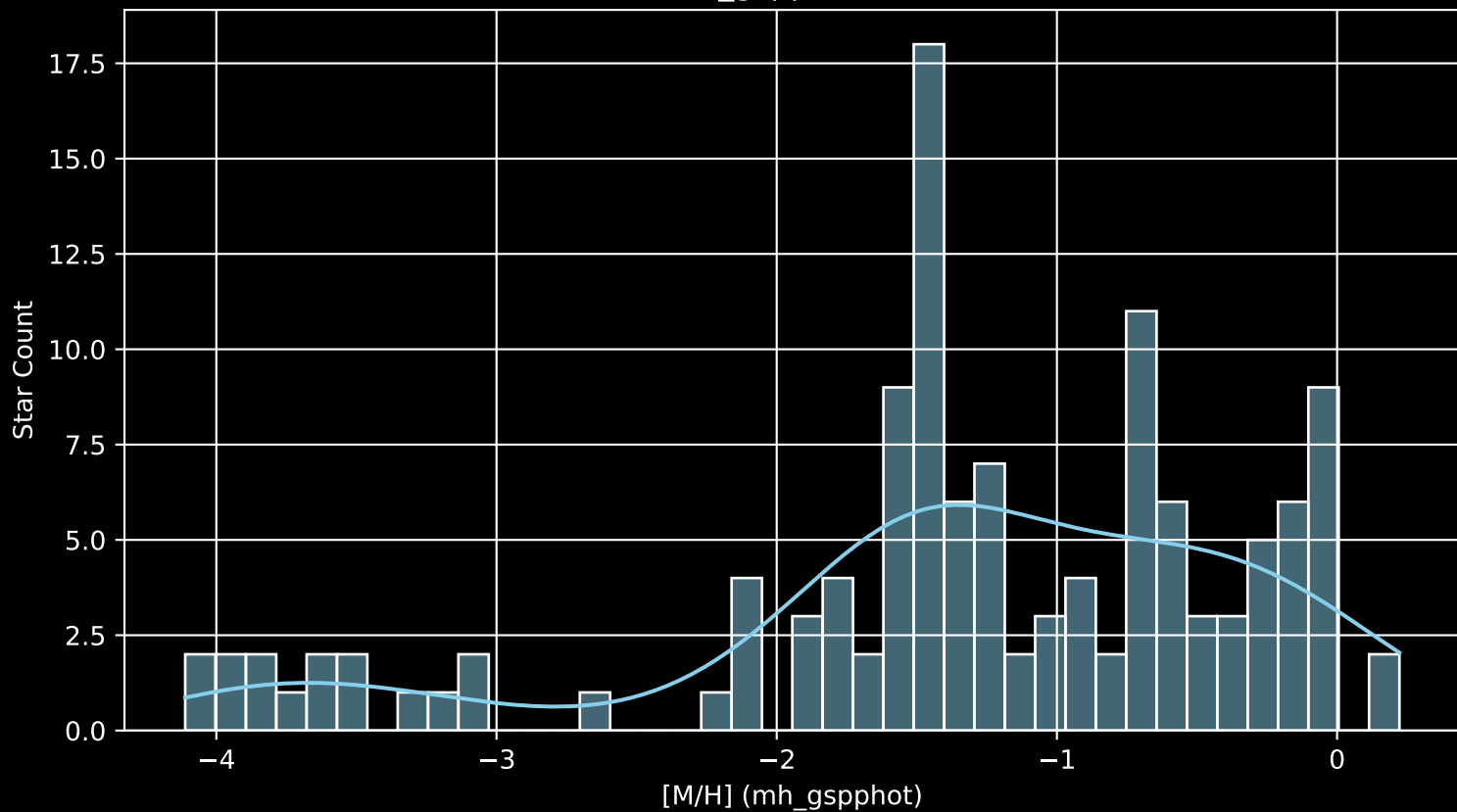
Gaia Cluster: [Deutsch_10 [M/H] (mh_gspphot) (n= 126)
