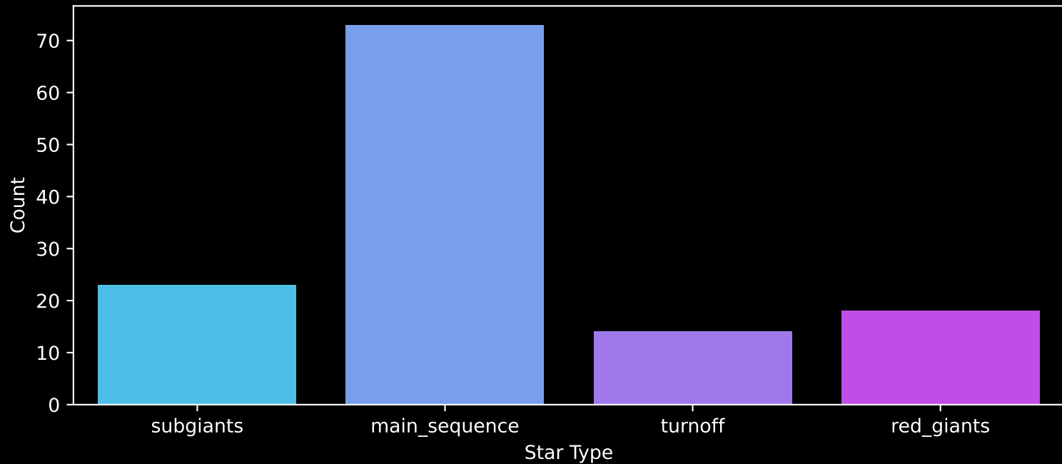
Gaia Cluster: [Teutsch_10] Count plot of Star Type
