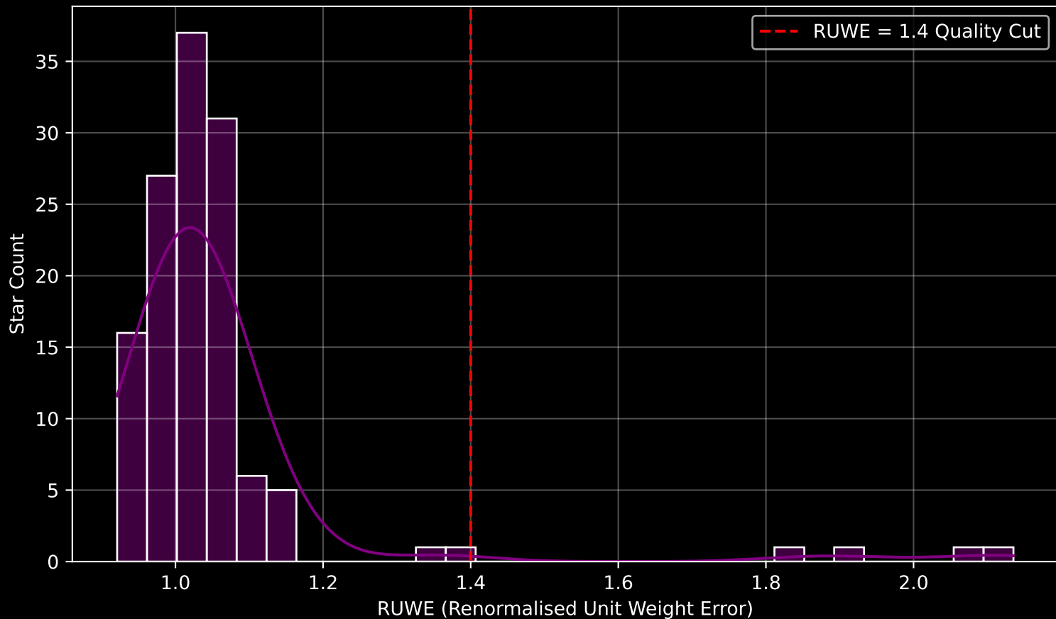
Gaia Cluster: [Teutsch_10] RUWE Distribution (n= 128)
