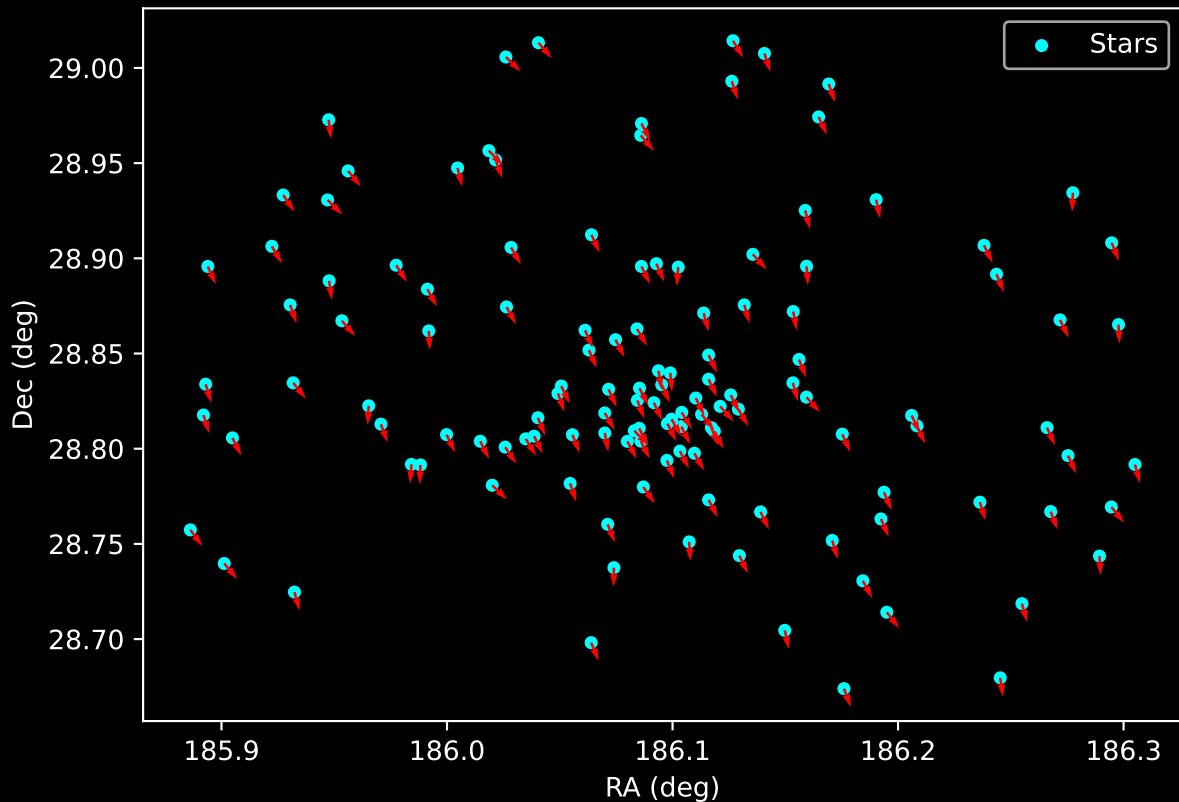
Gaia Cluster: [Teutsch_10] Proper Motion Vectors for Gaia Star Field (n= 128)
