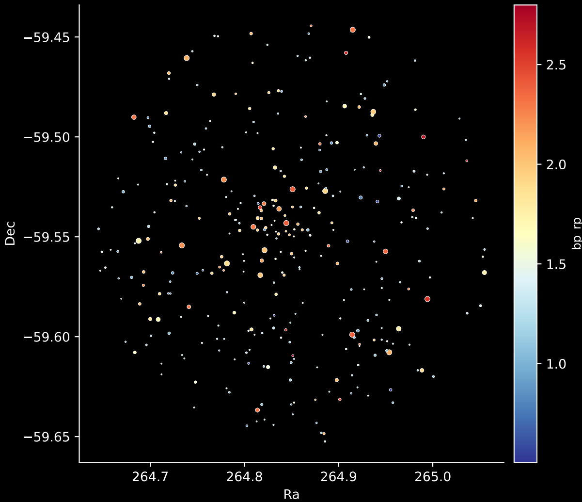
Gaia Cluster: [Teutsch_106] Stars: 332
