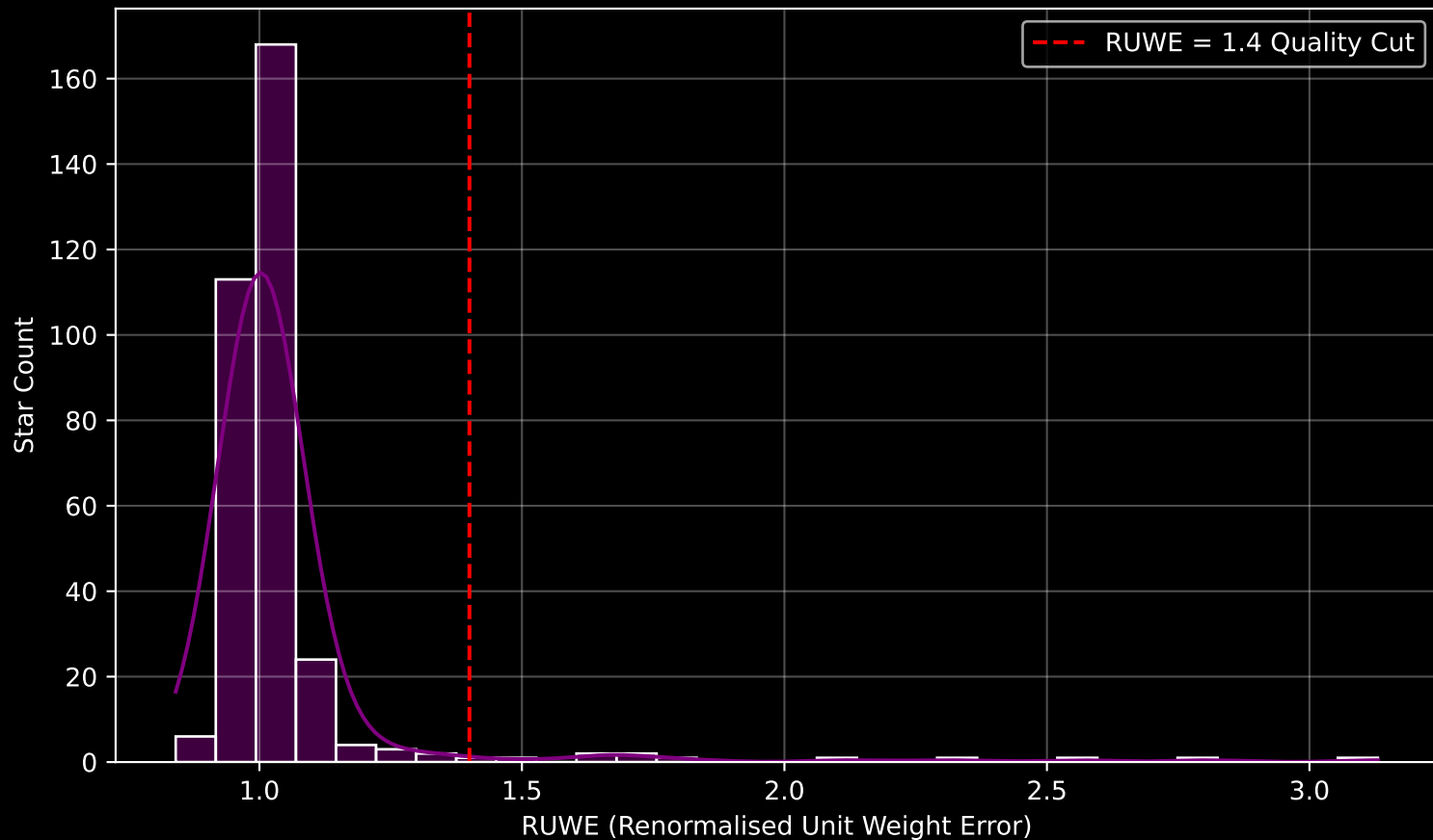
Gaia Cluster: [Teutsch_106] RUWE Distribution (n= 332)
