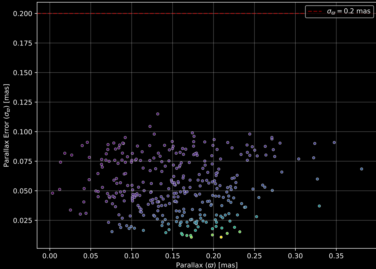
Gaia Cluster: [Teutsch_106] Parallax Quality (n= 332)
