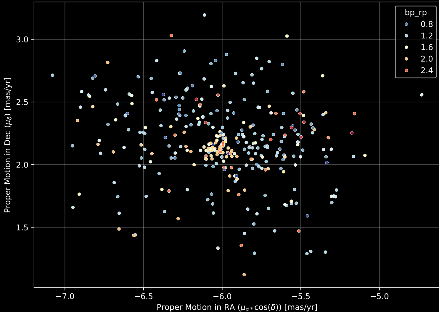
Gaia Cluster: [Teutsch_106] Proper Motion Diagram (n= 332)
