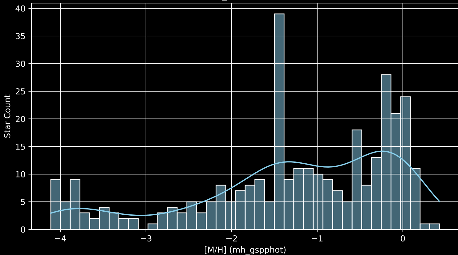
Gaia Cluster: [Teutsch_106 [M/H] (mh_gspphot) (n= 331)
