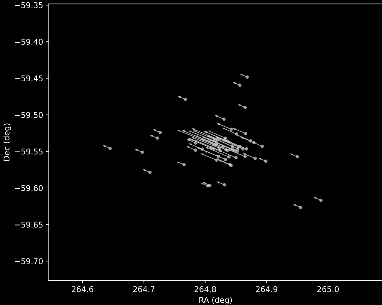
Gaia DR3 Cluster 15 Proper Motion Vectors (n=59)
