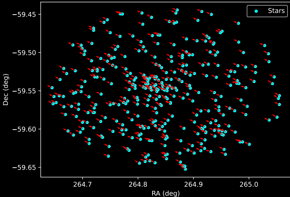
Gaia Cluster: [Teutsch_106] Proper Motion Vectors for Gaia Star Field (n= 332)
