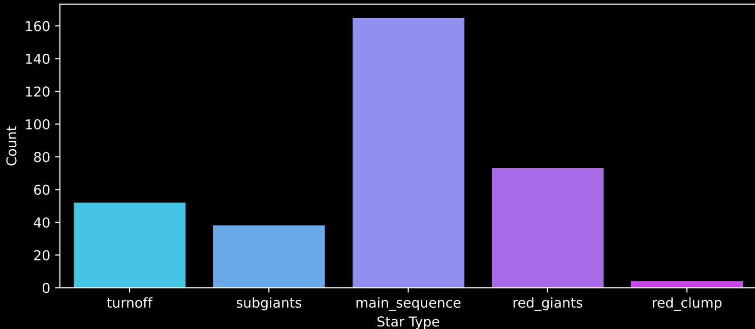
Gaia Cluster: [Teutsch_106] Count plot of Star Type
