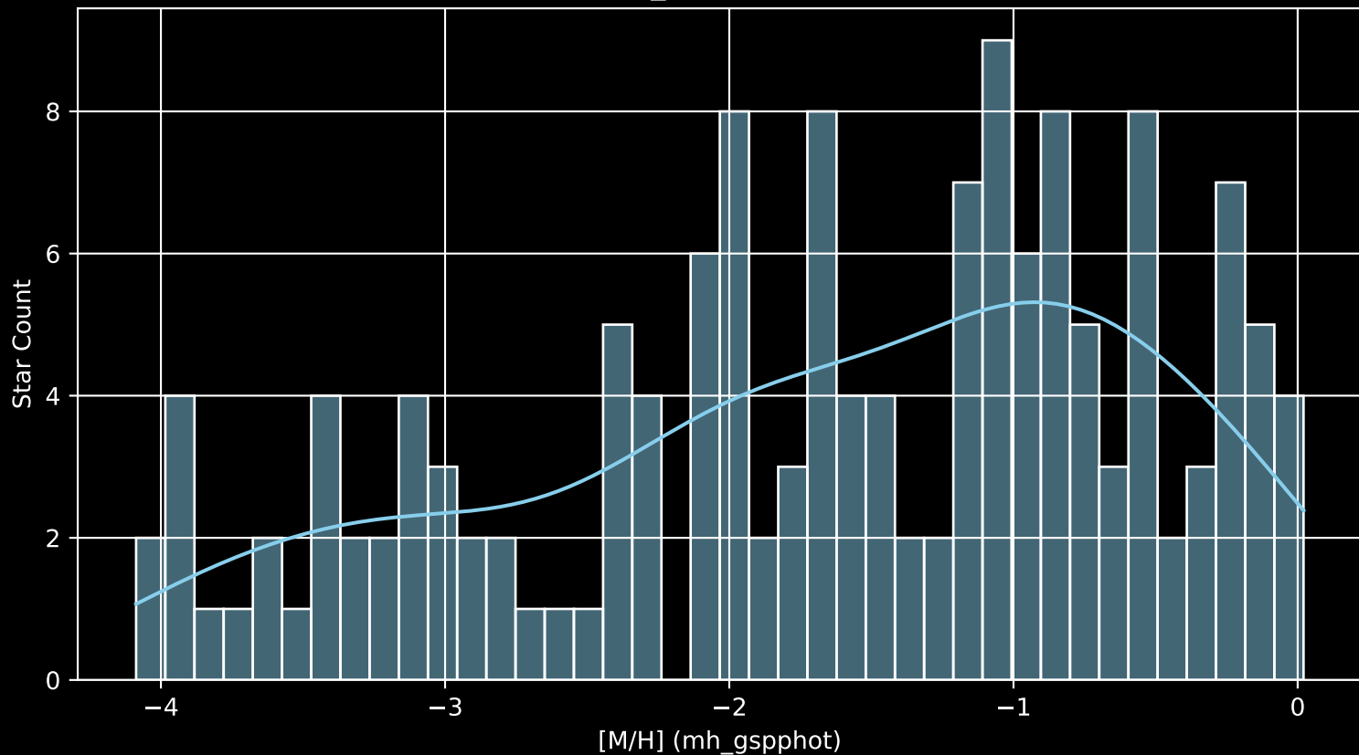
Gaia Cluster: [Teutsch_11 [M/H] (mh_gspphot) (n= 148)
