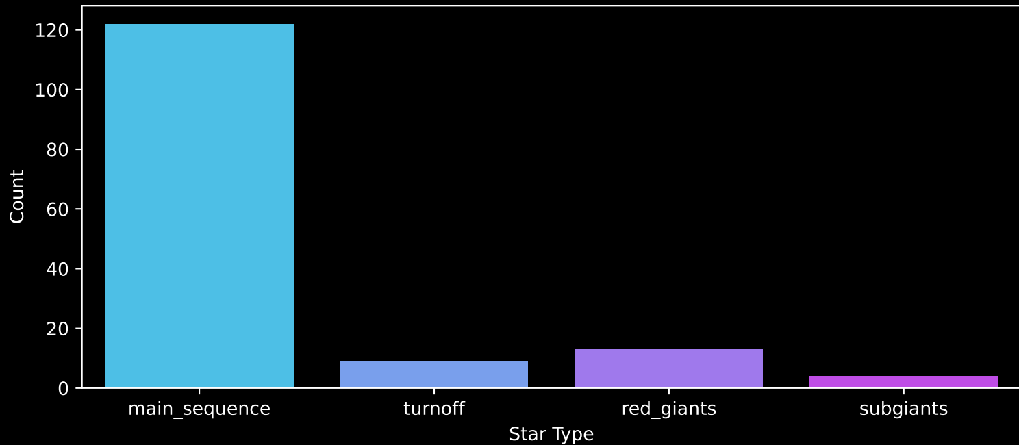
Gaia Cluster: [Teutsch_11] Count plot of Star Type
