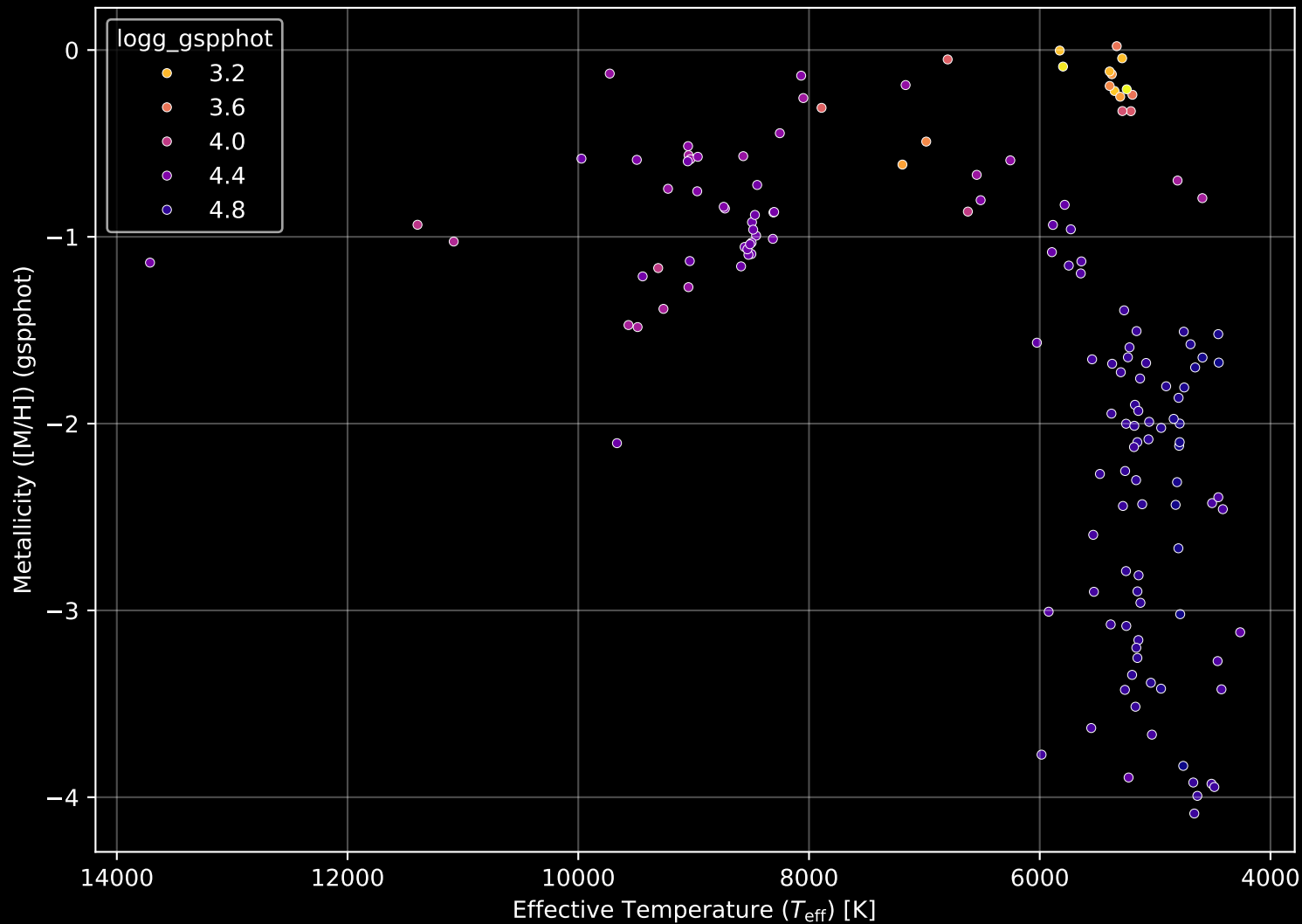
Gaia Cluster: [Teusch_11] Stellar Population Parameters (n= 148)
