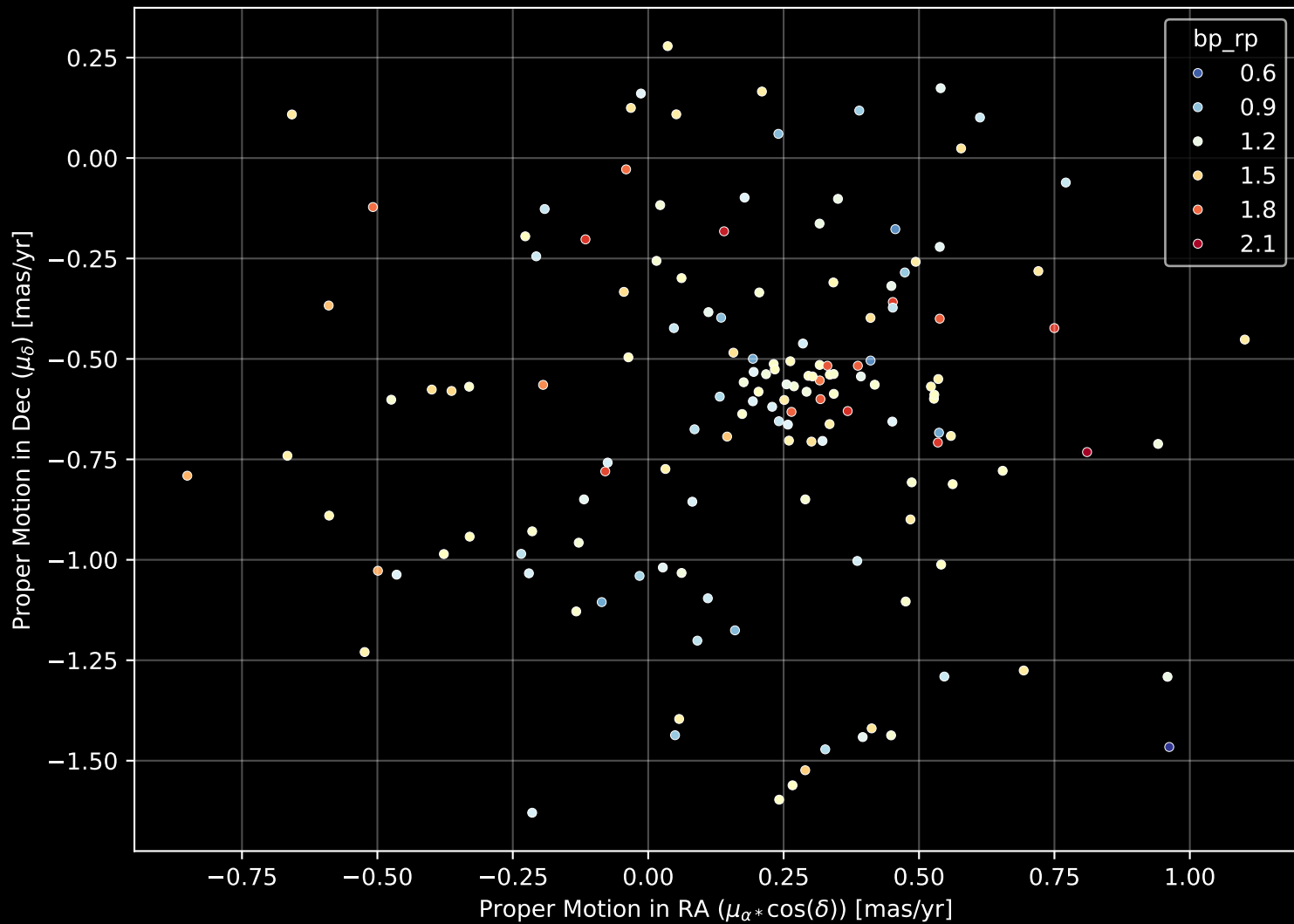
Gaia Cluster: [Teutsch_11] Proper Motion Diagram (n= 148)
