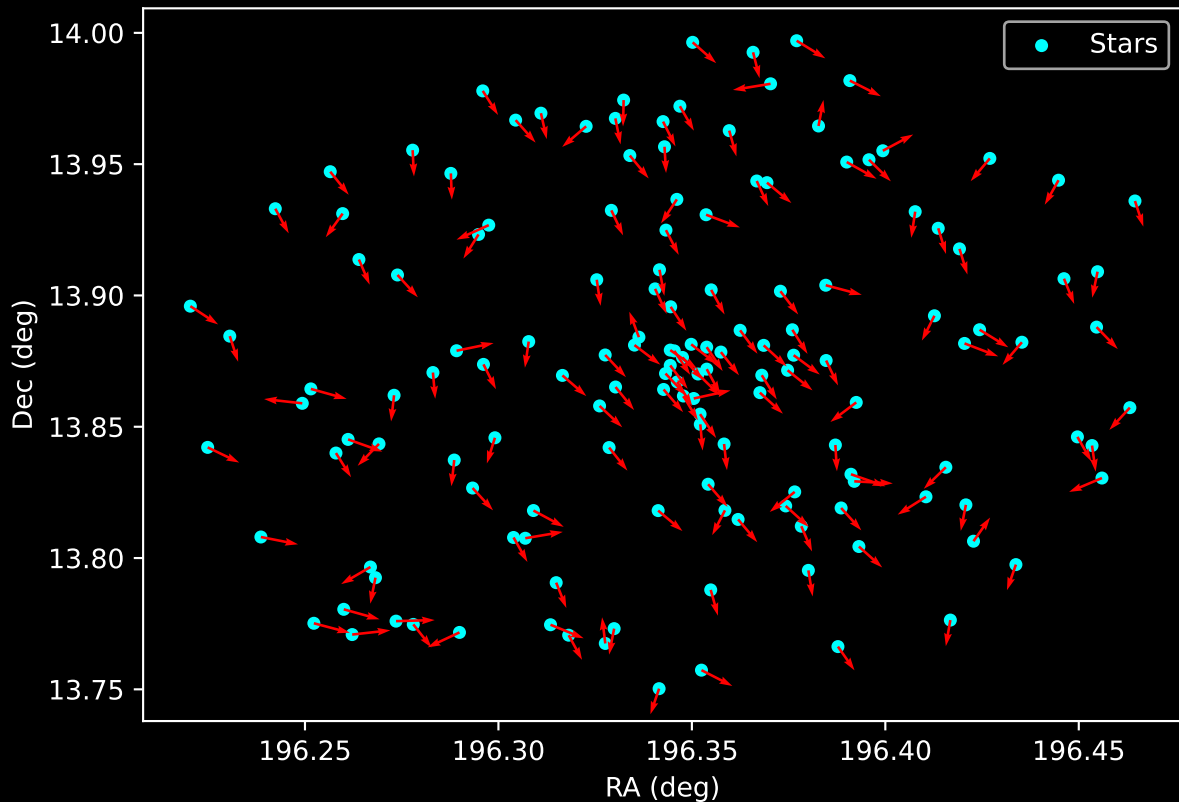
Gaia Cluster: [Teutsch_11] Proper Motion Vectors for Gaia Star Field (n= 148)
