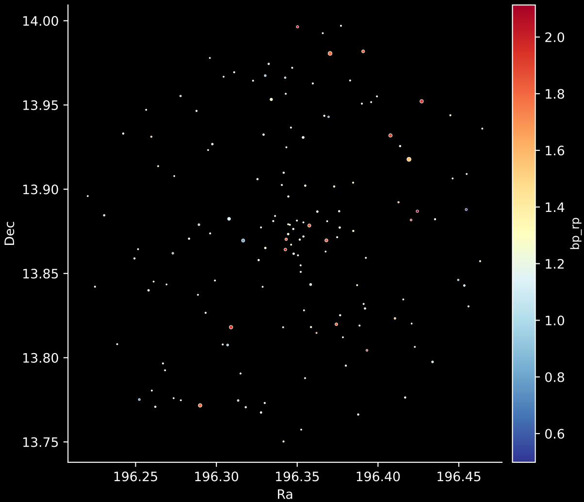
Gaia Cluster: [Teutsch_11] Stars: 148
