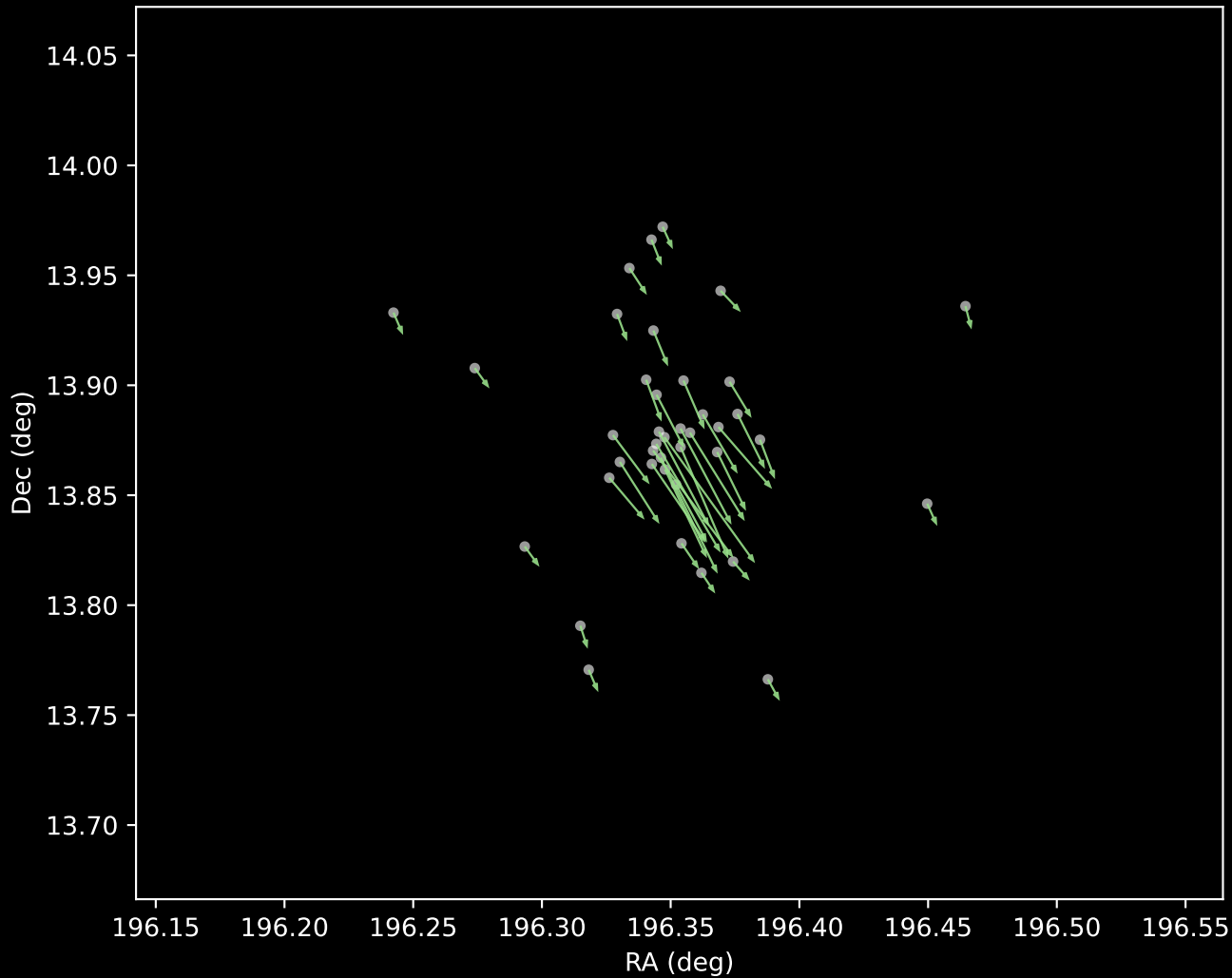
Gaia DR3 Cluster 5 Proper Motion Vectors (n=40)
