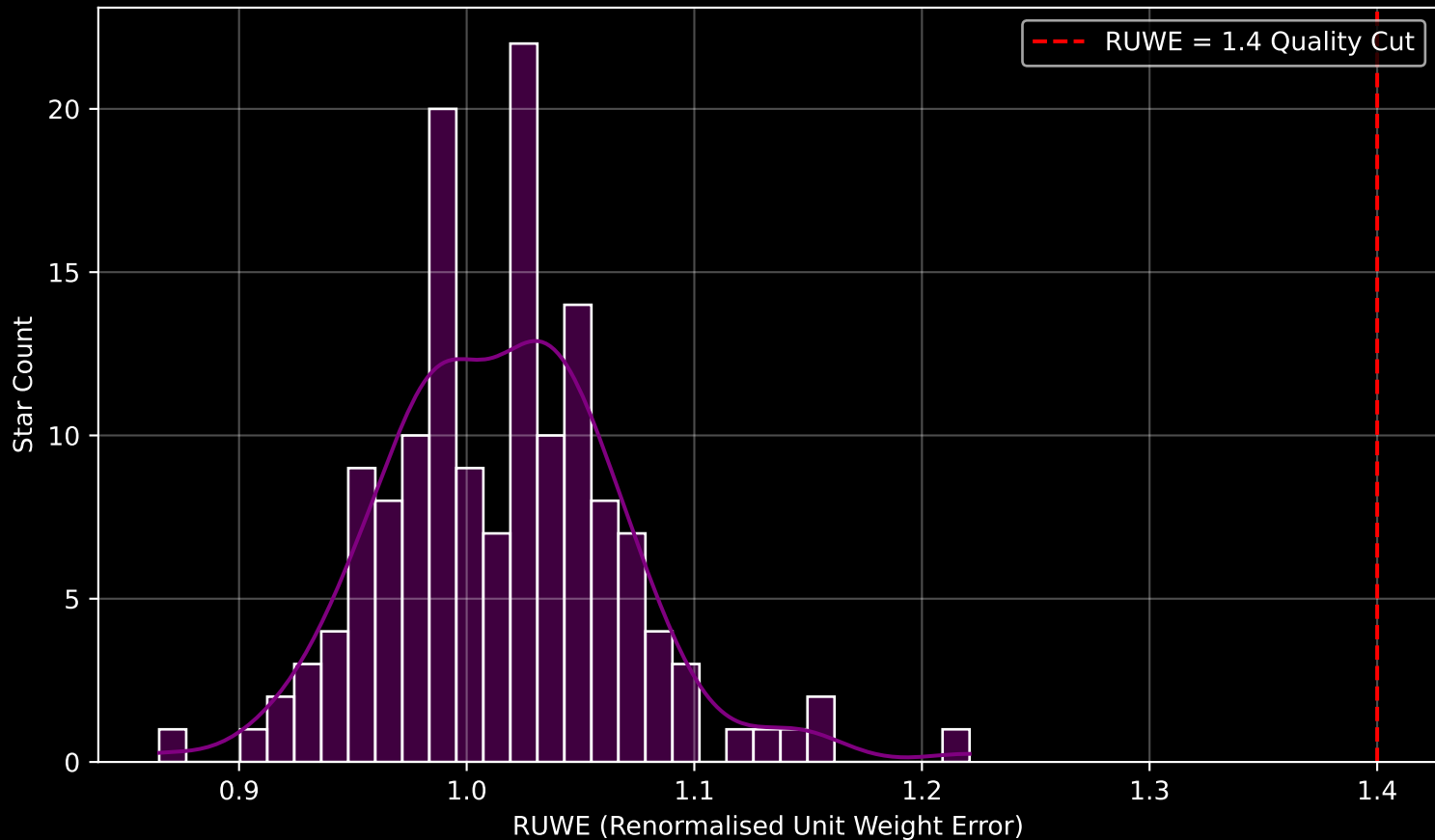
Gaia Cluster: [Teutsch_11] RUWE Distribution (n= 148)
