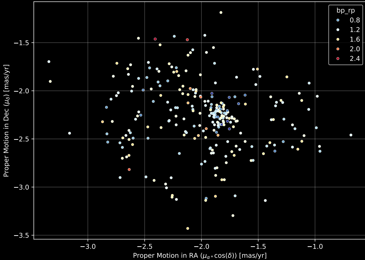
Gaia Cluster: [Deutsch_126] Proper Motion Diagram (n= 268)
