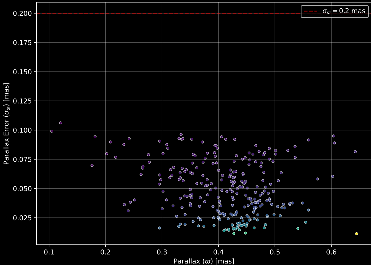
Gaia Cluster: [Teutsch_126] Parallax Quality (n= 268)
