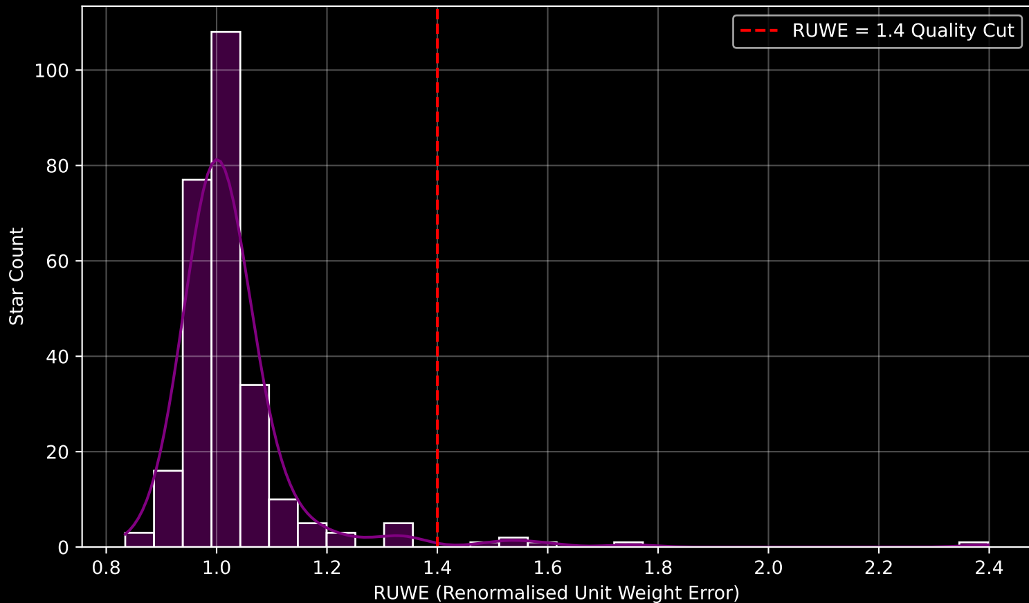
Gaia Cluster: [Teutsch_126] RUWE Distribution (n= 267)
