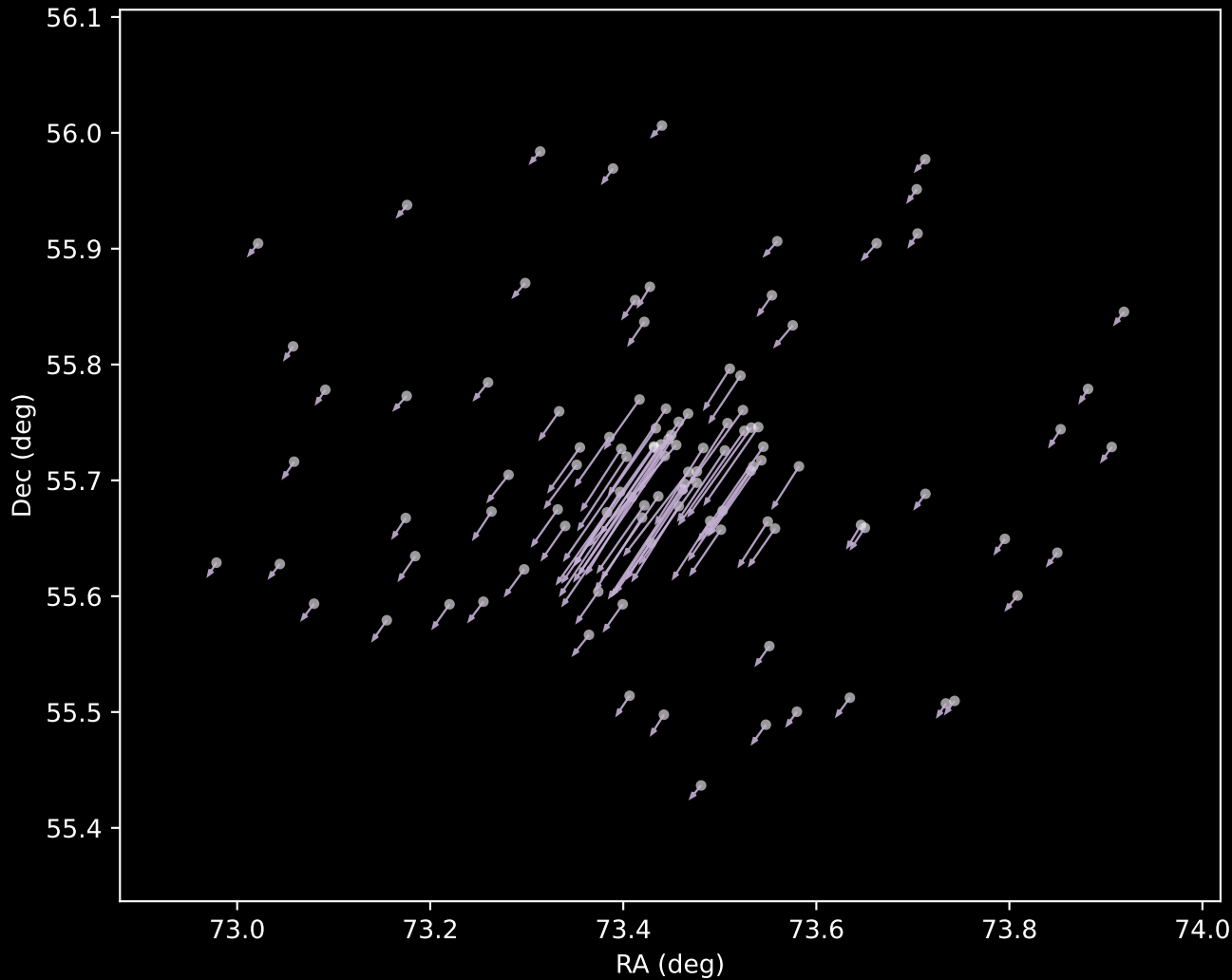
Gaia DR3 Cluster 9 Proper Motion Vectors (n=106)
