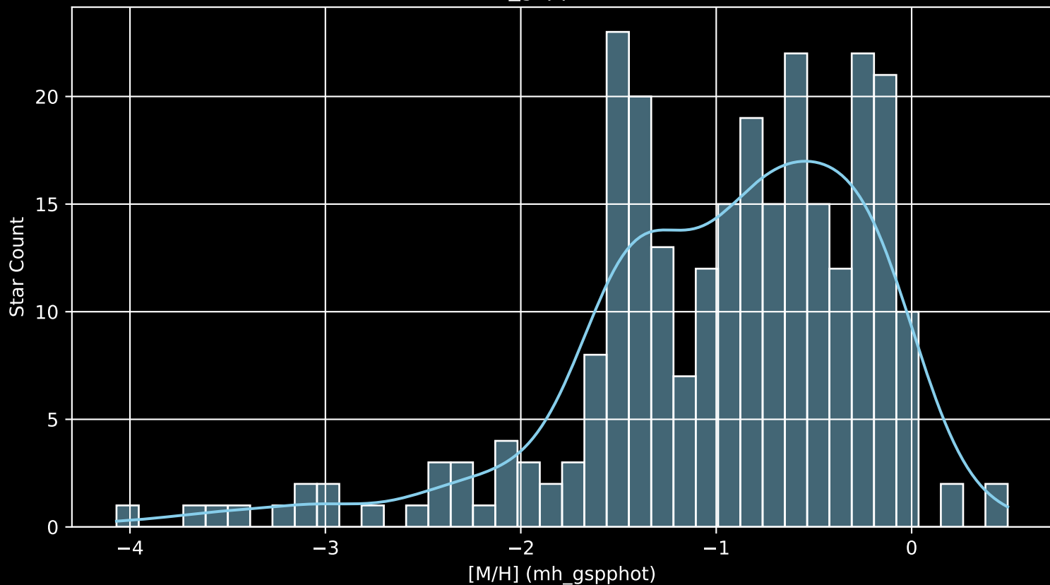
Gaia Cluster: [Deutsch_126 [M/H] (mh_gspphot) (n= 268)
