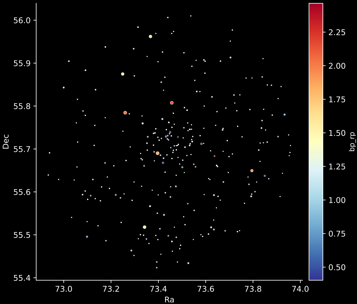
Gaia Cluster: [Teutsch_126] Stars: 268
