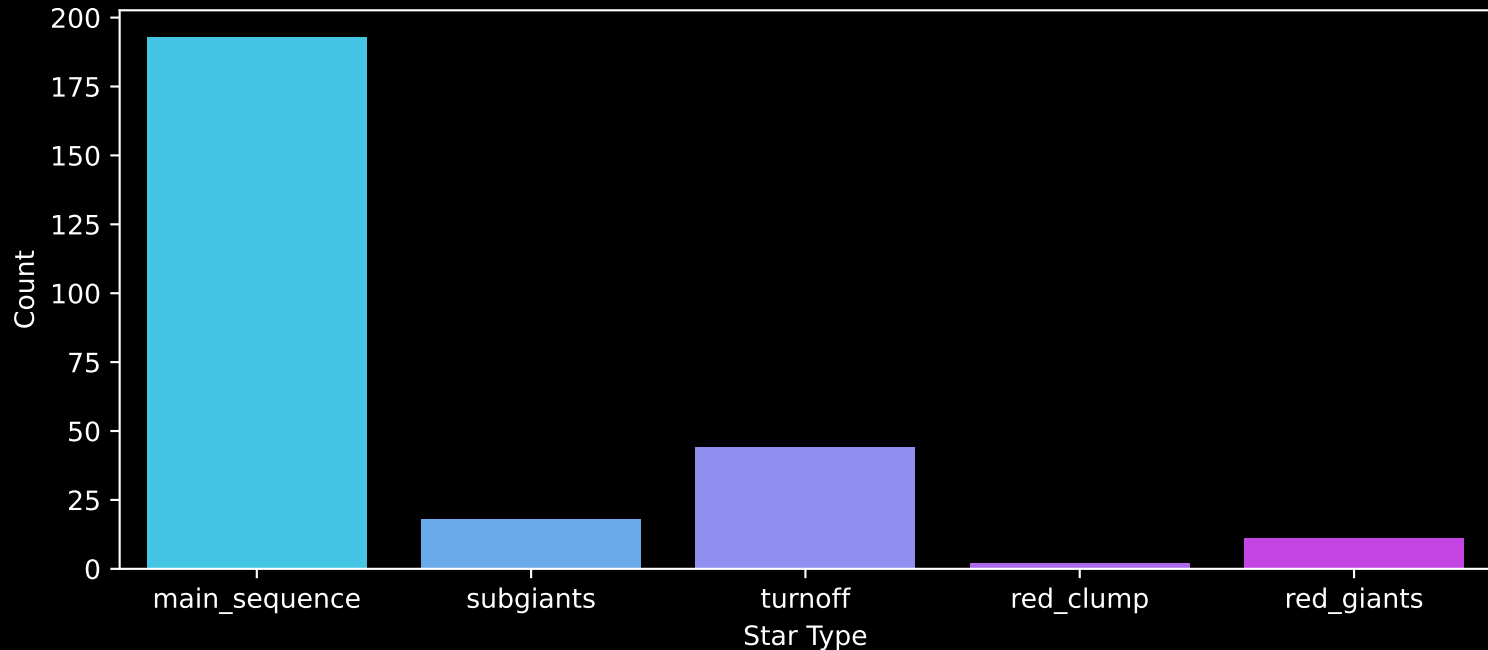
Gaia Cluster: [Teutsch_126] Count plot of Star Type
