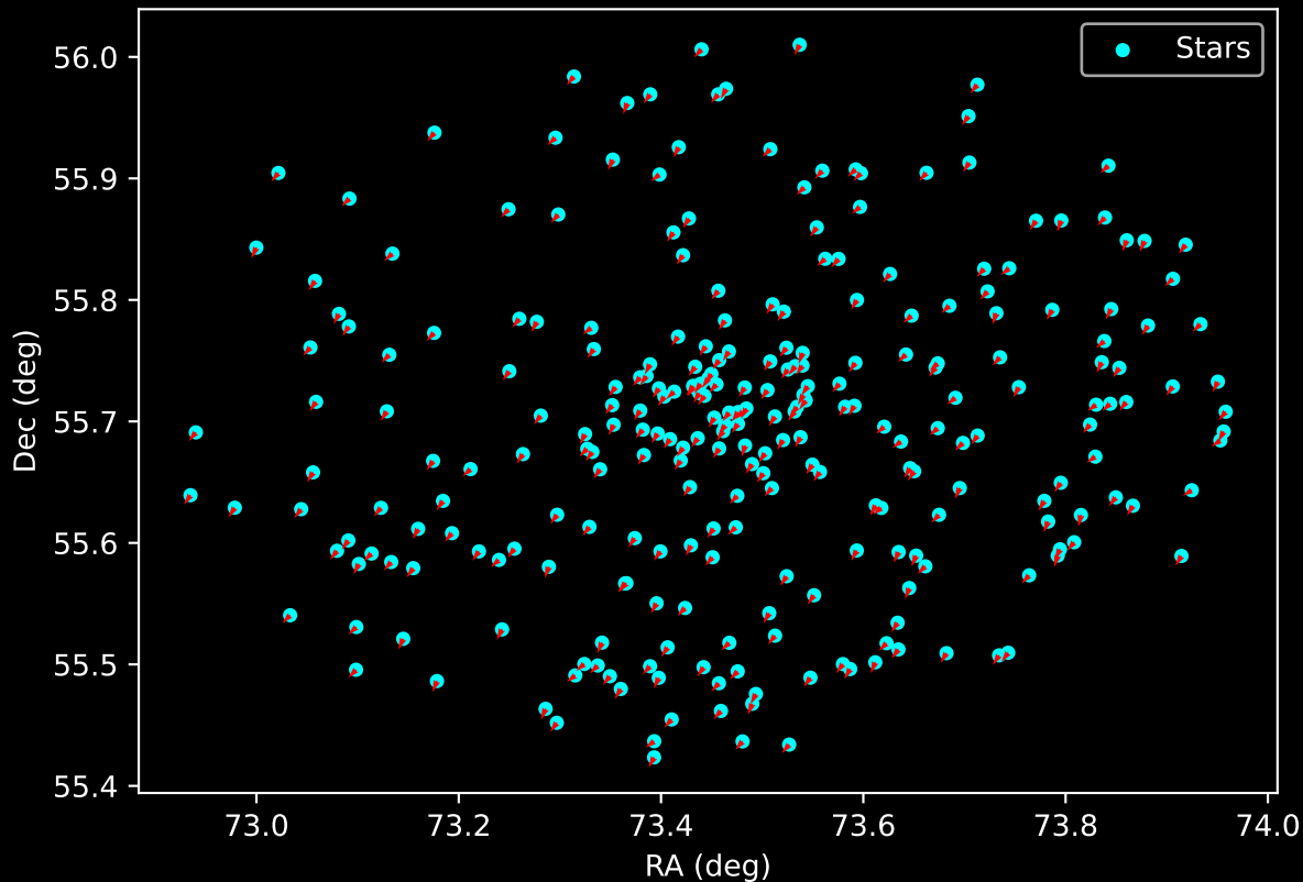
Gaia Cluster: [Deutsch_126] Proper Motion Vectors for Gaia Star Field (n= 268)
